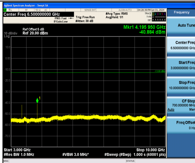
Band12_1.4MHz_QPSK_23017_1RB#0_3000~10000_3000~10000
