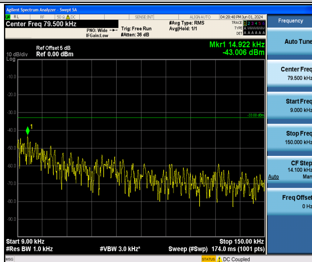
Band12_1.4MHz_16QAM_23017_1RB#0_0.009~0.15_0.009~0.15
