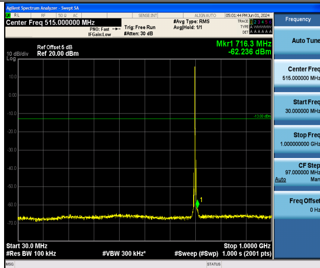
Band12_3MHz_QPSK_23095_1RB#0_30~1000_30~1000
