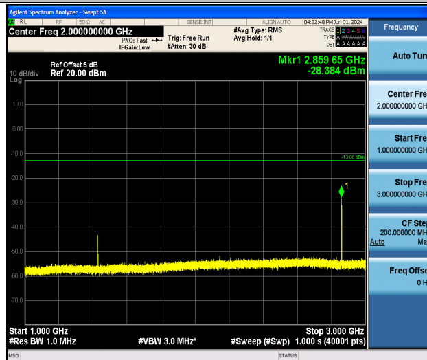
Band12_1.4MHz_16QAM_23173_1RB#0_1000~3000_1000~3000
