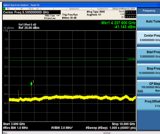
Band12_3MHz_QPSK_23095_1RB#0_3000~10000_3000~10000
