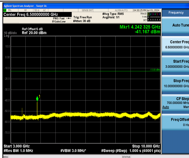
Band12_1.4MHz_QPSK_23095_1RB#0_3000~10000_3000~10000
