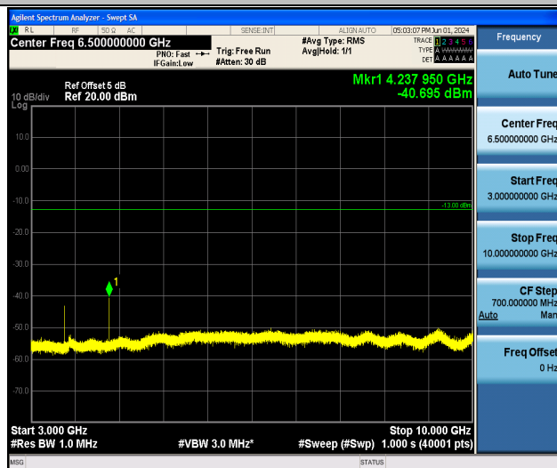
Band12_3MHz_16QAM_23095_1RB#0_3000~10000_3000~10000
