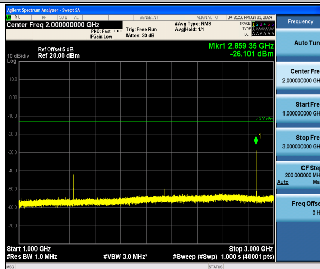
Band12_1.4MHz_QPSK_23173_1RB#0_1000~3000_1000~3000
