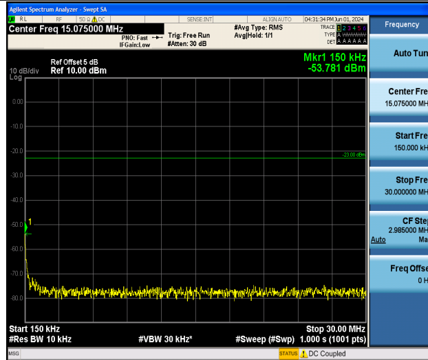
Band12_1.4MHz_QPSK_23173_1RB#0_0.15~30_0.15~30
