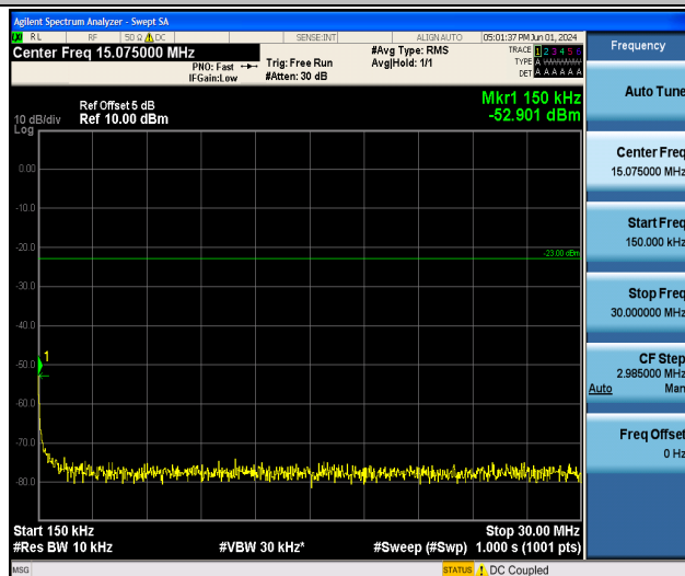
Band12_3MHz_QPSK_23095_1RB#0_0.15~30_0.15~30
