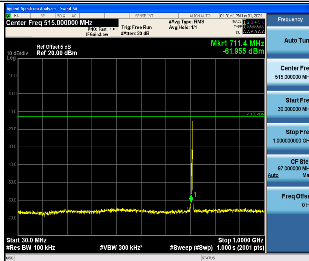
Band12_1.4MHz_QPSK_23173_1RB#0_30~1000_30~1000
