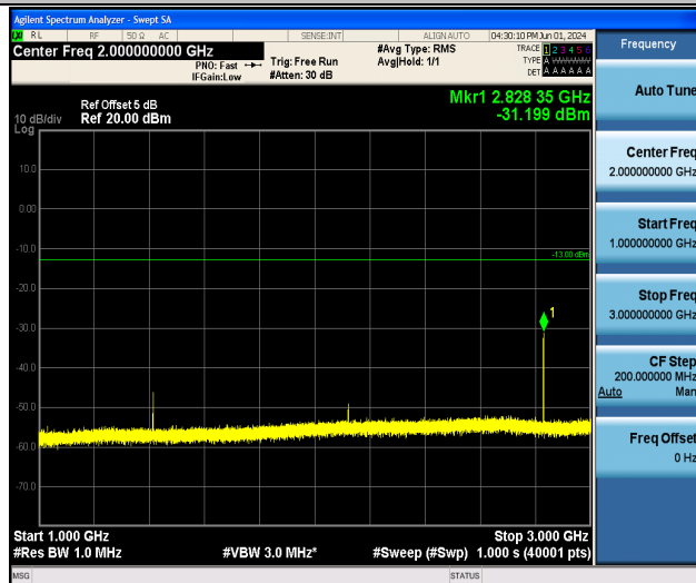
Band12_1.4MHz_QPSK_23095_1RB#0_1000~3000_1000~3000
