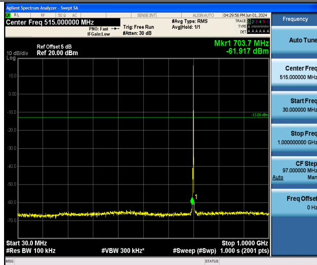
Band12_1.4MHz_QPSK_23095_1RB#0_30~1000_30~1000
