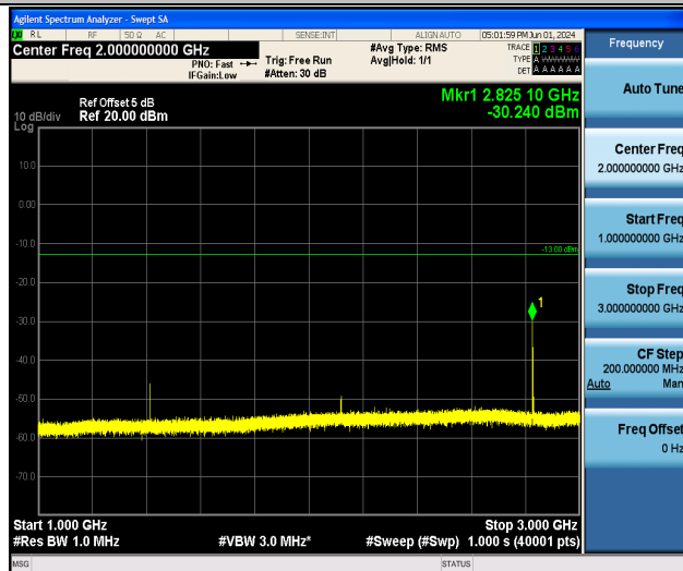
Band12_3MHz_QPSK_23095_1RB#0_1000~3000_1000~3000
