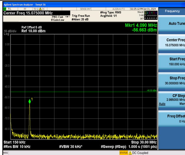
Band7_5MHz_QPSK_21425_1RB#0_0.15~30_0.15~30
