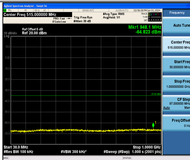
Band7_10MHz_QPSK_21400_1RB#0_30~1000_30~1000
