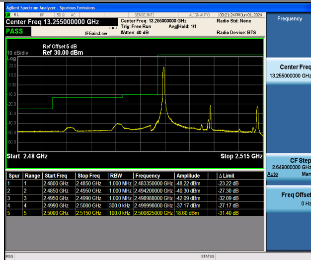
Band7_15MHz_QPSK_20825_1RB#0
