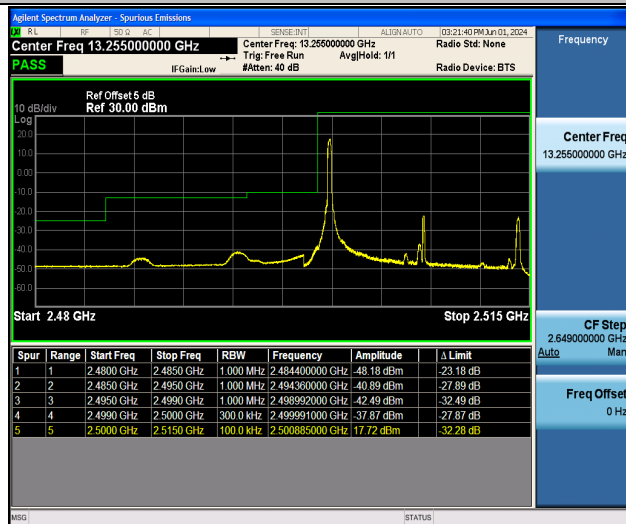
Band7_15MHz_16QAM_20825_1RB#0
