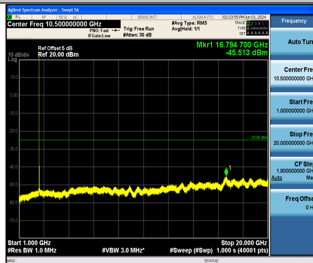
Band7_5MHz_QPSK_21100_1RB#0_1000~20000_1000~20000
