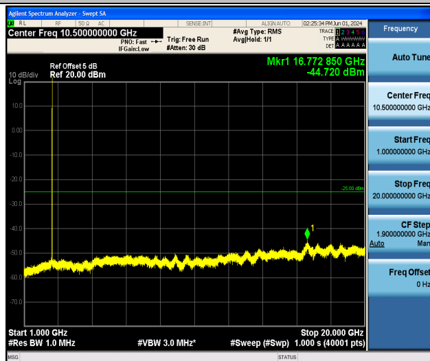
Band7_5MHz_QPSK_21425_1RB#0_1000~20000_1000~20000
