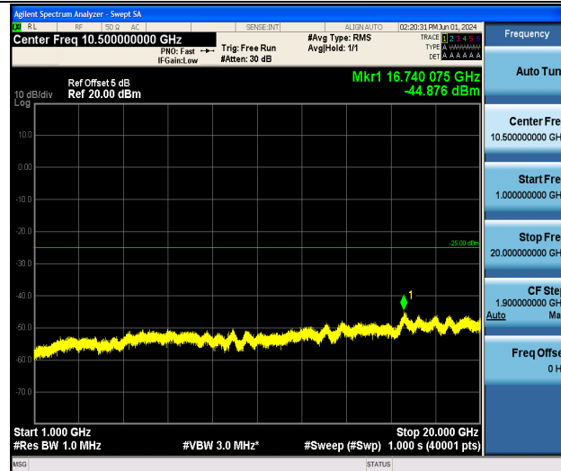
Band7_5MHz_QPSK_20775_1RB#0_1000~20000_1000~20000
