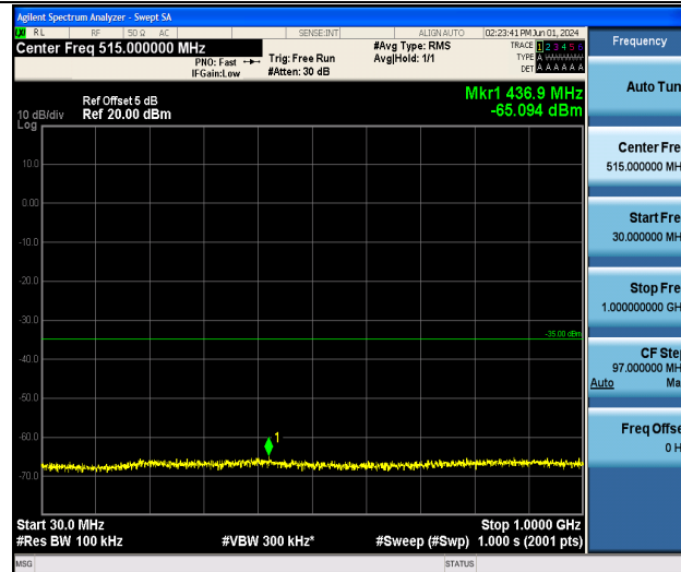
Band7_5MHz_QPSK_21100_1RB#0_30~1000_30~1000
