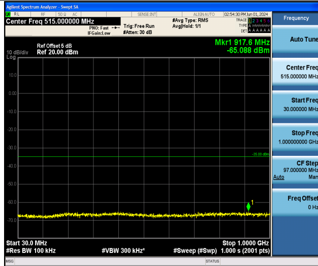
Band7_10MHz_QPSK_21100_1RB#0_30~1000_30~1000
