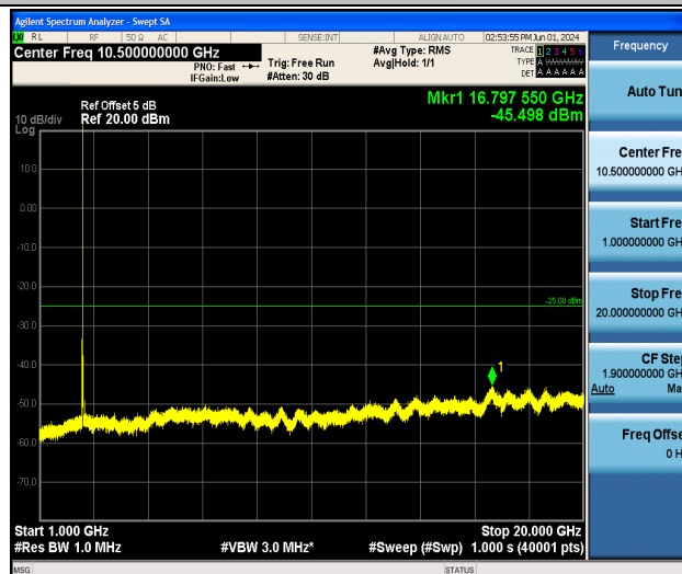
Band7_10MHz_16QAM_20800_1RB#0_1000~20000_1000~20000
