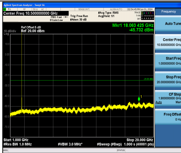
Band7_10MHz_QPSK_21100_1RB#0_1000~20000_1000~20000
