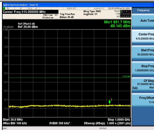
Band7_5MHz_QPSK_21425_1RB#0_30~1000_30~1000
