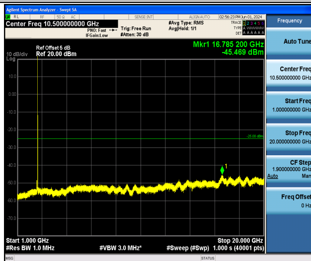
Band7_10MHz_QPSK_21400_1RB#0_1000~20000_1000~20000
