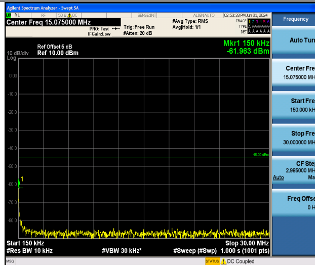
Band7_10MHz_16QAM_20800_1RB#0_0.15~30_0.15~30
