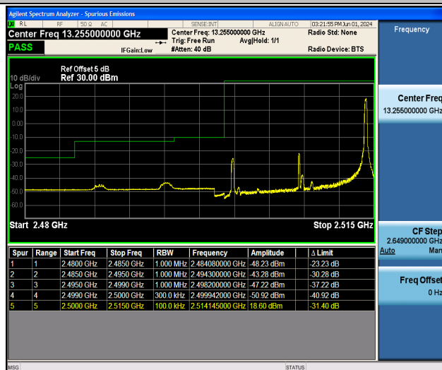
Band7_15MHz_QPSK_20825_1RB#74
