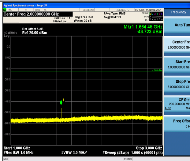
Band5_10MHz_QPSK_20525_1RB#0_1000~3000_1000~3000
