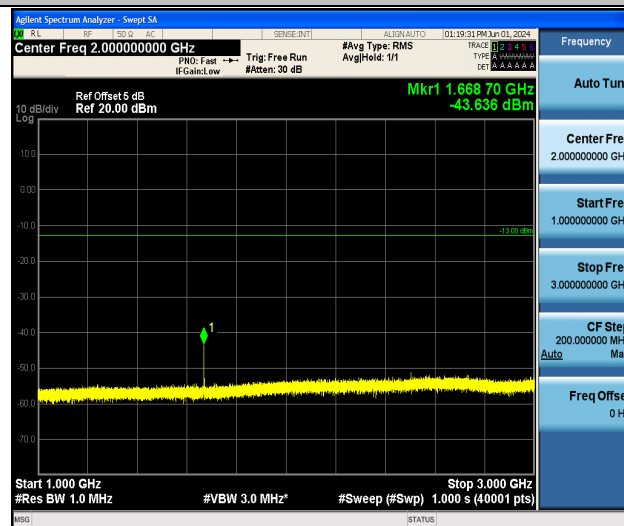
Band5_5MHz_QPSK_20525_1RB#0_1000~3000_1000~3000
