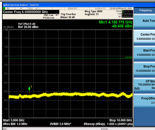
Band5_10MHz_QPSK_20525_1RB#0_3000~10000_3000~10000
