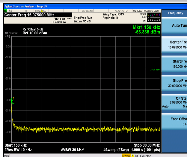
Band5_10MHz_QPSK_20525_1RB#0_0.15~30_0.15~30
