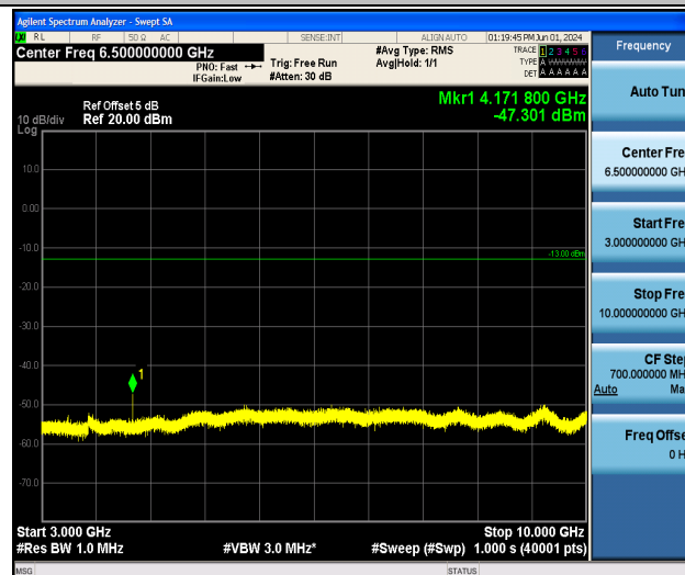
Band5_5MHz_QPSK_20525_1RB#0_3000~10000_3000~10000
