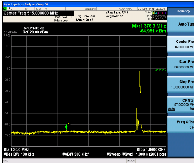
Band5_10MHz_QPSK_20525_1RB#0_30~1000_30~1000
