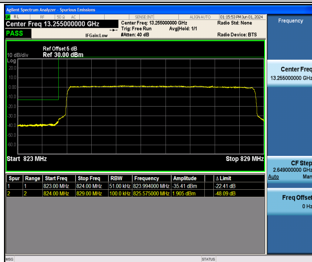
Band5_5MHz_16QAM_20425_25RB#0
