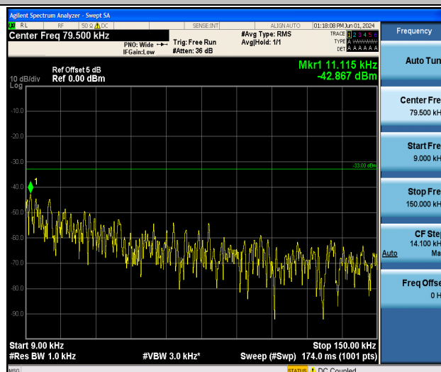
Band5_5MHz_16QAM_20425_1RB#0_0.009~0.15_0.009~0.15
