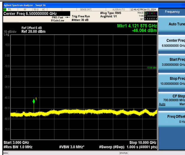
Band5_3MHz_QPSK_20415_1RB#0_3000~10000_3000~10000
