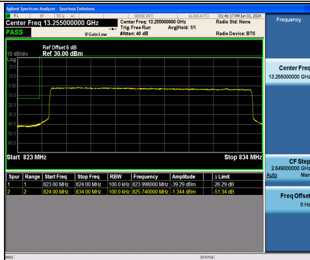
Band5_10MHz_16QAM_20450_50RB#0
