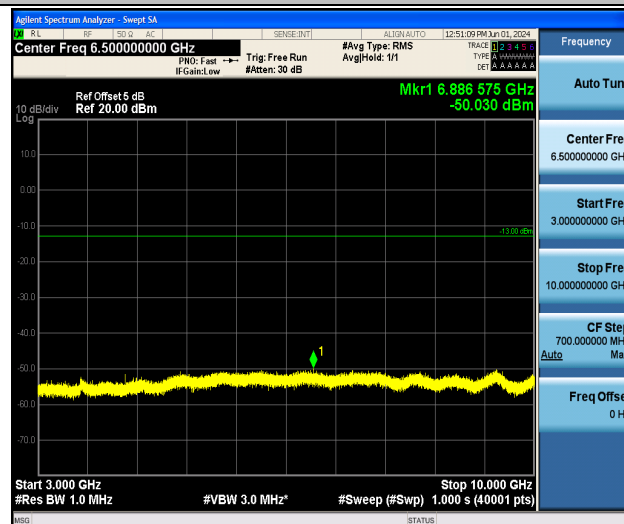
Band5_3MHz_16QAM_20635_1RB#0_3000~10000_3000~10000
