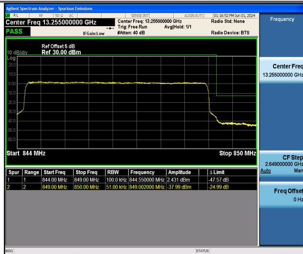
Band5_5MHz_QPSK_20625_25RB#0
