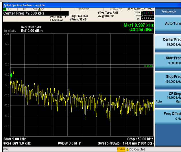
Band5_3MHz_16QAM_20635_1RB#0_0.009~0.15_0.009~0.15
