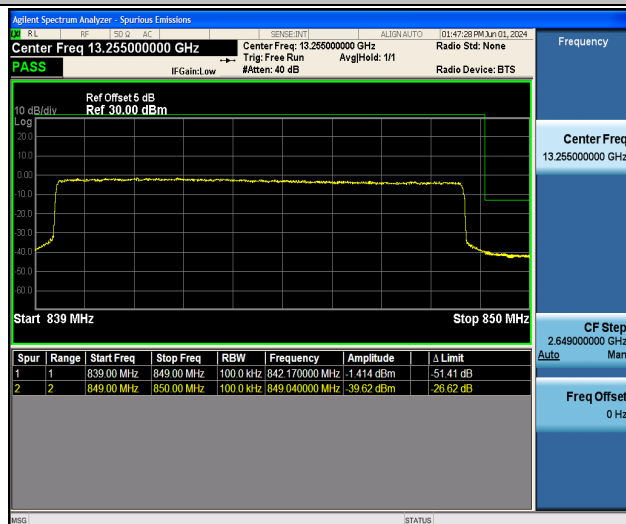
Band5_10MHz_16QAM_20600_50RB#0
