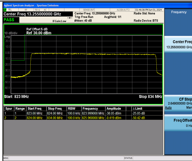
Band5_10MHz_QPSK_20450_50RB#0
