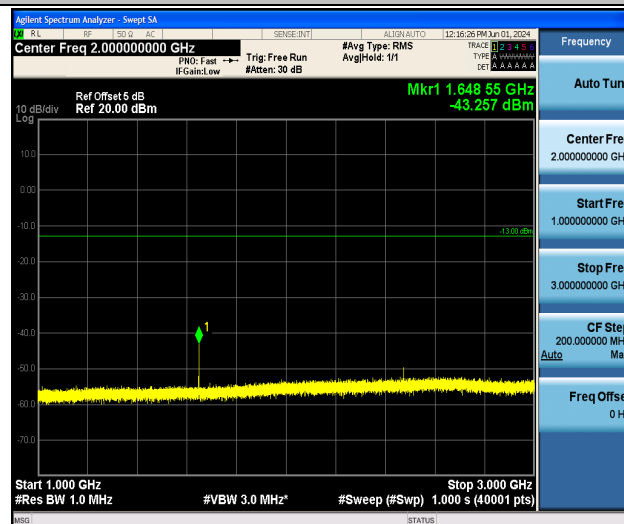
Band5_1.4MHz_16QAM_20407_1RB#0_1000~3000_1000~3000
