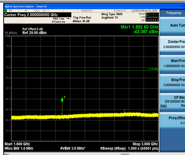
Band5_3MHz_QPSK_20635_1RB#0_1000~3000_1000~3000
