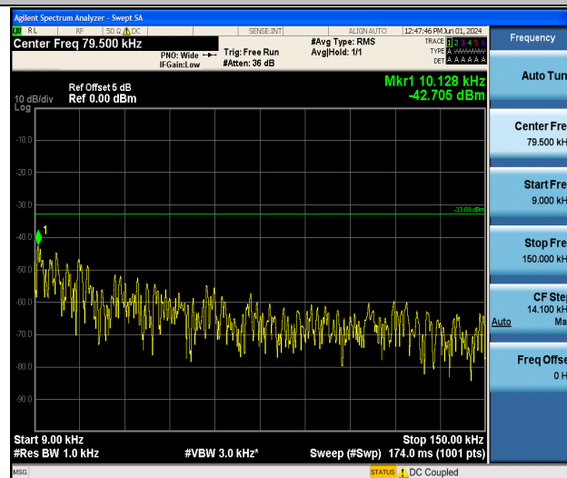
Band5_3MHz_QPSK_20525_1RB#0_0.009~0.15_0.009~0.15
