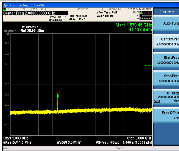
Band5_3MHz_QPSK_20525_1RB#0_1000~3000_1000~3000
