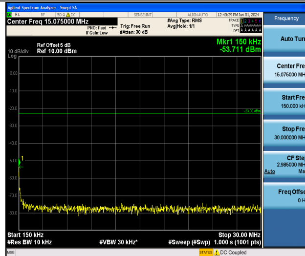
Band5_3MHz_QPSK_20635_1RB#0_0.15~30_0.15~30
