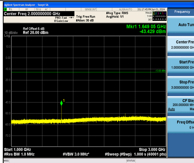
Band5_5MHz_QPSK_20425_1RB#0_1000~3000_1000~3000
