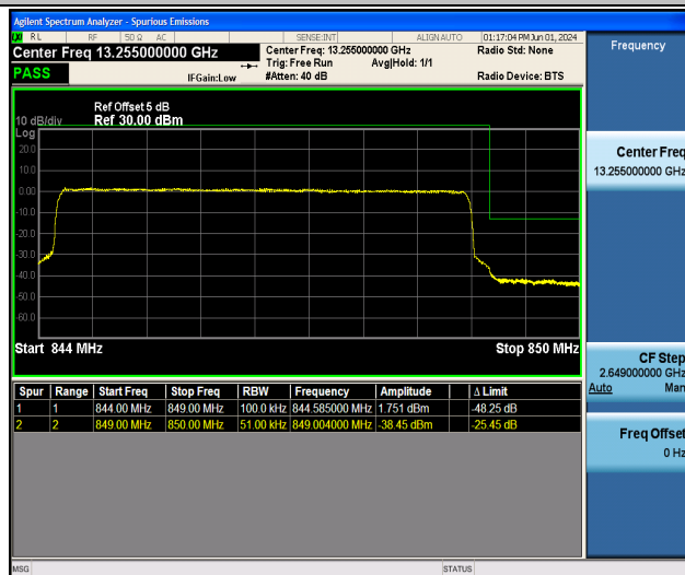
Band5_5MHz_16QAM_20625_25RB#0
