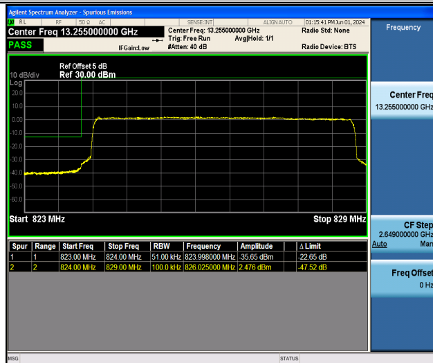
Band5_5MHz_QPSK_20425_25RB#0
