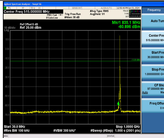
Band5_3MHz_16QAM_20635_1RB#0_30~1000_30~1000
