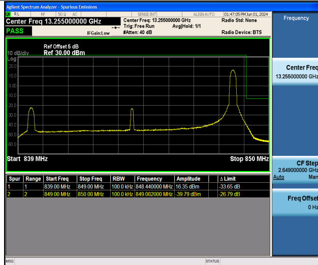
Band5_10MHz_16QAM_20600_1RB#49
