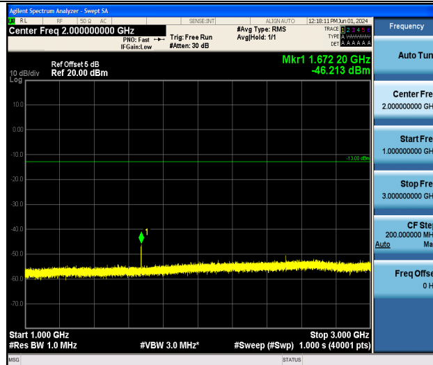
Band5_1.4MHz_16QAM_20525_1RB#0_1000~3000_1000~3000
