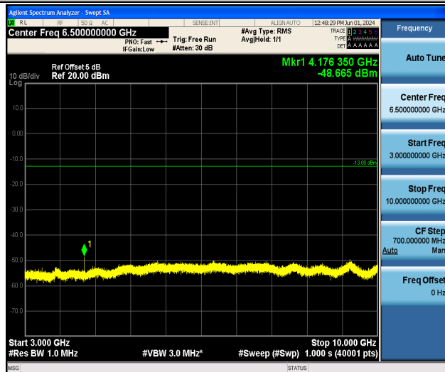
Band5_3MHz_QPSK_20525_1RB#0_3000~10000_3000~10000
