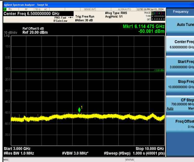
Band5_3MHz_QPSK_20635_1RB#0_3000~10000_3000~10000
