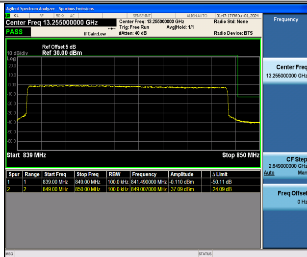
Band5_10MHz_QPSK_20600_50RB#0
