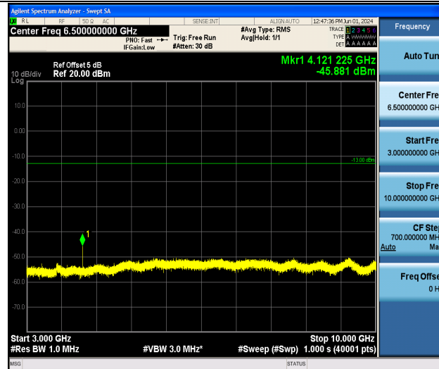
Band5_3MHz_16QAM_20415_1RB#0_3000~10000_3000~10000
