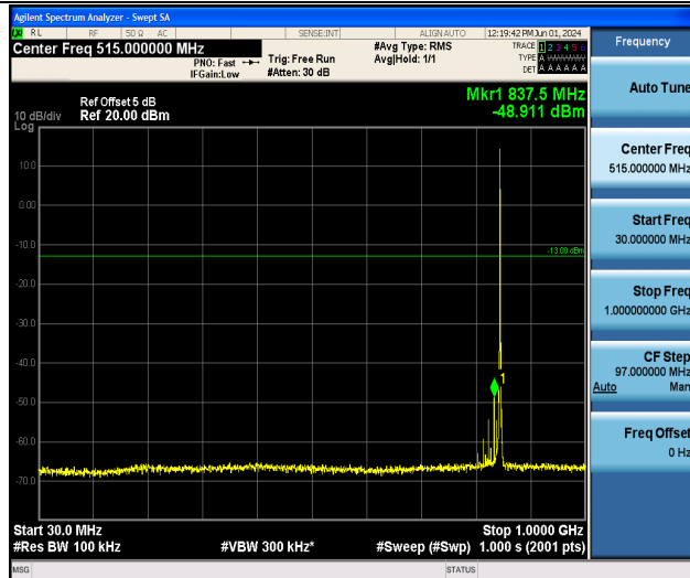
Band5_1.4MHz_16QAM_20643_1RB#0_30~1000_30~1000
