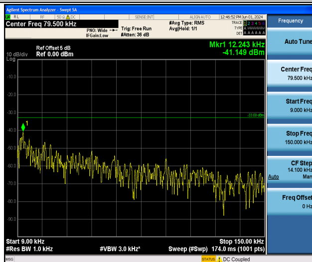
Band5_3MHz_16QAM_20415_1RB#0_0.009~0.15_0.009~0.15
