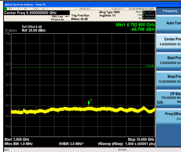
Band5_1.4MHz_QPSK_20643_1RB#0_3000~10000_3000~10000
