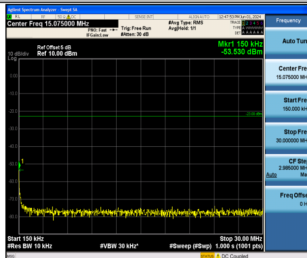
Band5_3MHz_QPSK_20525_1RB#0_0.15~30_0.15~30
