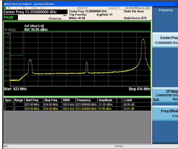
Band5_10MHz_16QAM_20450_1RB#49
