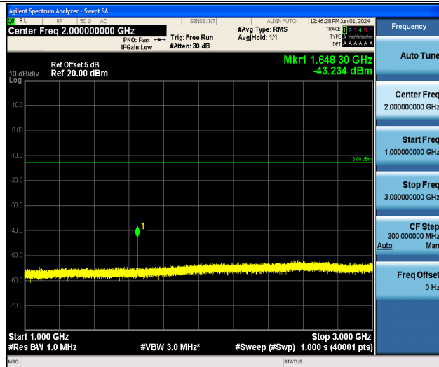
Band5_3MHz_QPSK_20415_1RB#0_1000~3000_1000~3000
