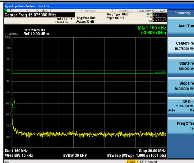
Band5_1.4MHz_16QAM_20643_1RB#0_0.15~30_0.15~30
