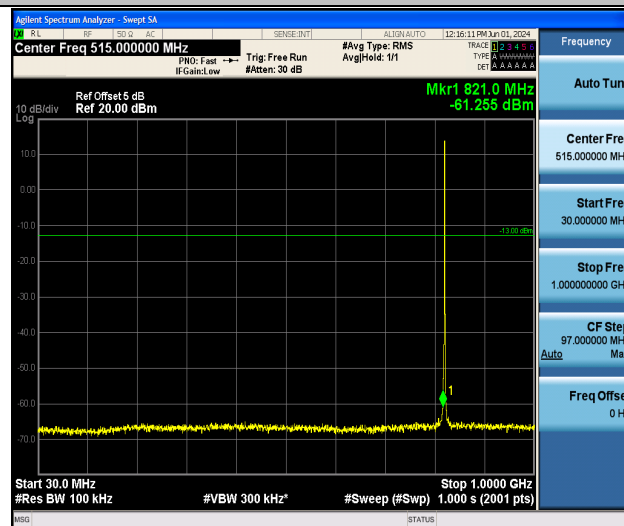
Band5_1.4MHz_16QAM_20407_1RB#0_30~1000_30~1000
