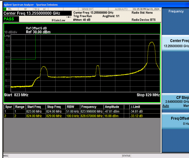
Band5_5MHz_16QAM_20425_1RB#24
