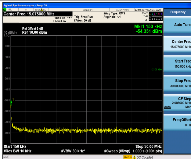
Band5_3MHz_16QAM_20635_1RB#0_0.15~30_0.15~30
