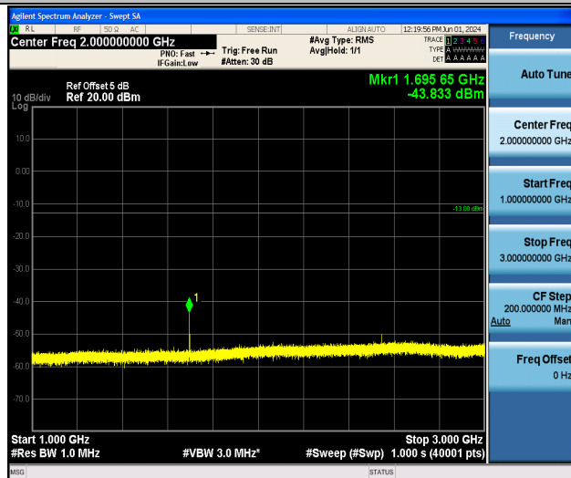
Band5_1.4MHz_16QAM_20643_1RB#0_1000~3000_1000~3000
