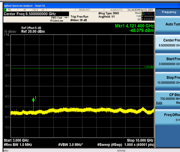
Band5_5MHz_QPSK_20425_1RB#0_3000~10000_3000~10000
