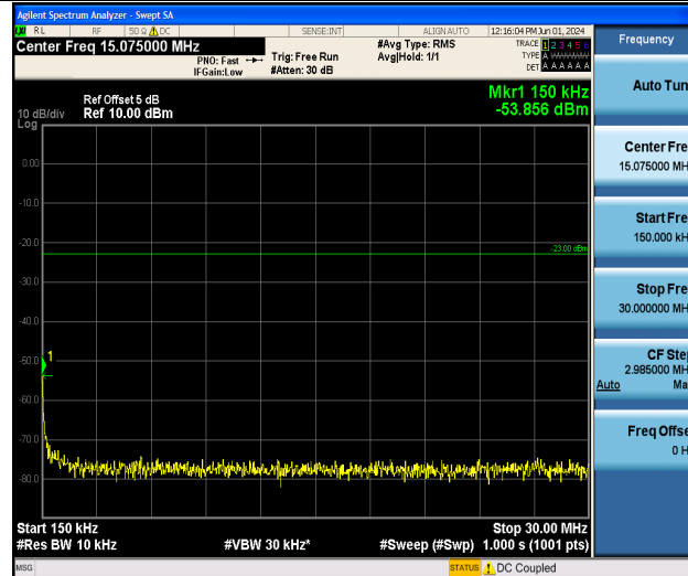
Band5_1.4MHz_16QAM_20407_1RB#0_0.15~30_0.15~30
