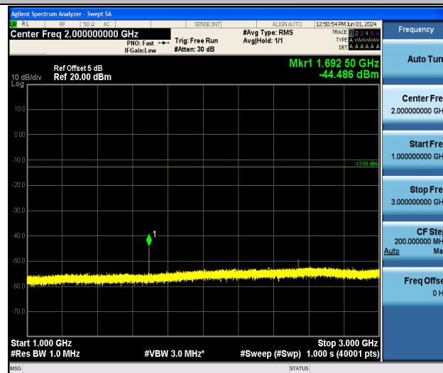
Band5_3MHz_16QAM_20635_1RB#0_1000~3000_1000~3000
