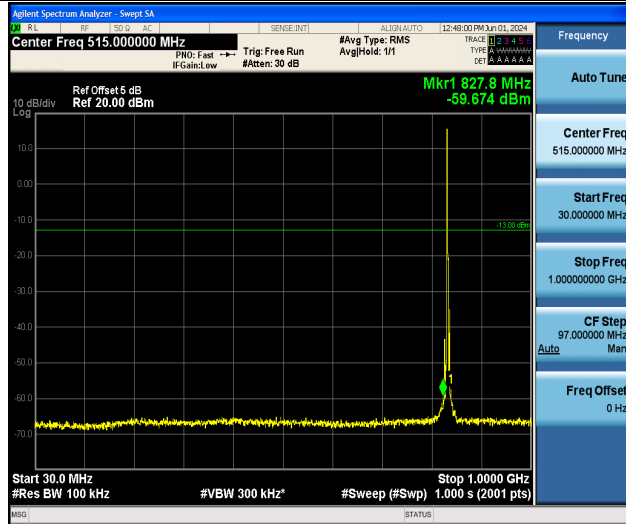
Band5_3MHz_QPSK_20525_1RB#0_30~1000_30~1000
