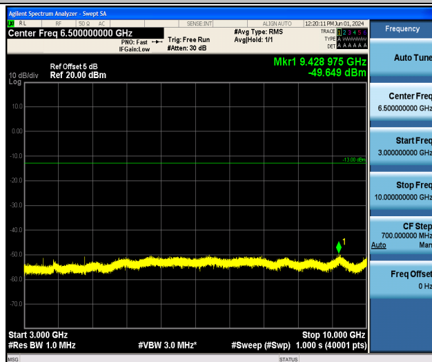
Band5_1.4MHz_16QAM_20643_1RB#0_3000~10000_3000~10000
