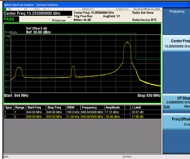
Band5_5MHz_16QAM_20625_1RB#24
