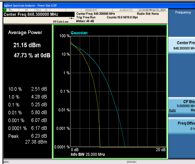
Band5-1.4MHz-QPSK-20643-6RB#0-PASS
