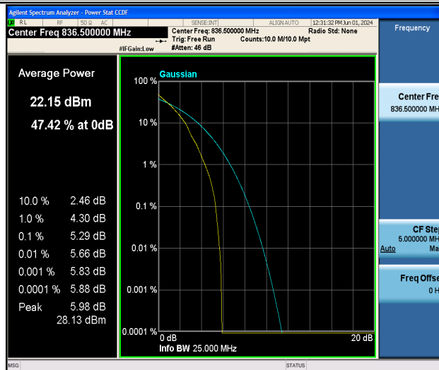
Band5-1.4MHz-QPSK-20525-1RB#0-PASS
