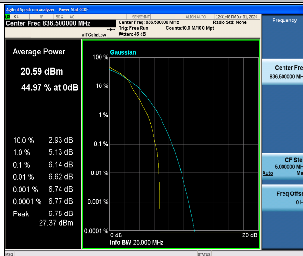
Band5-1.4MHz-16QAM-20525-1RB#0-PASS
