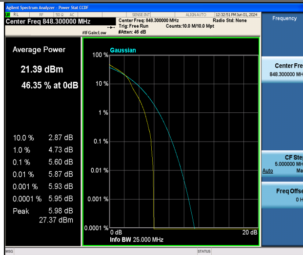
Band5-1.4MHz-16QAM-20643-1RB#0-PASS
