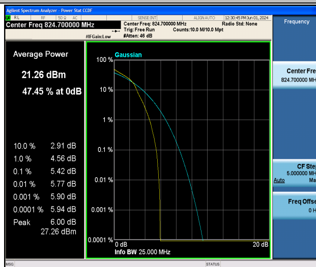
Band5-1.4MHz-16QAM-20407-1RB#0-PASS
