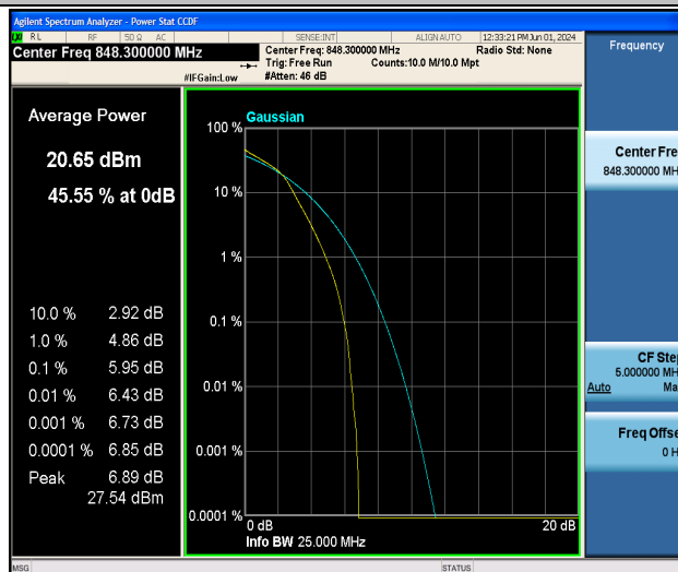
Band5-1.4MHz-16QAM-20643-6RB#0-PASS
