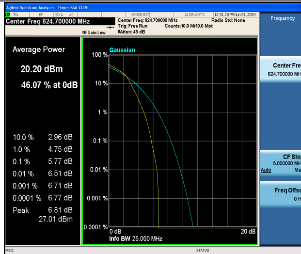
Band5-1.4MHz-16QAM-20407-6RB#0-PASS
