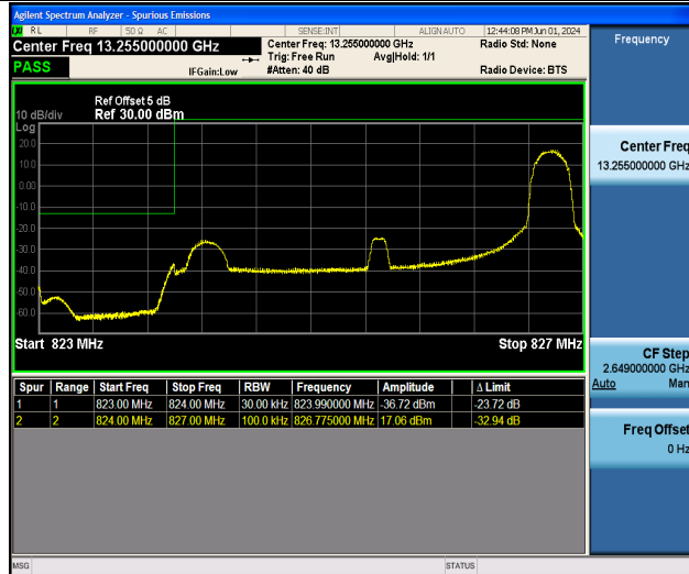
Band5_3MHz_16QAM_20415_1RB#14
