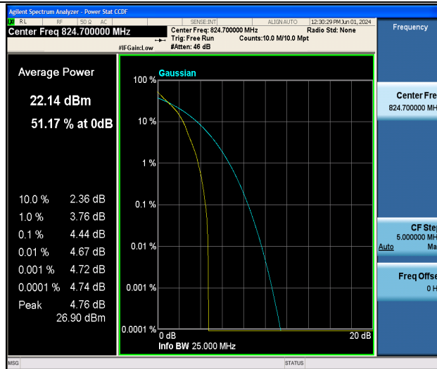
Band5-1.4MHz-QPSK-20407-1RB#0-PASS
