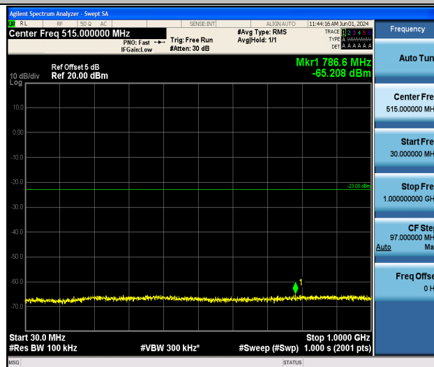
Band4_20MHz_16QAM_20050_1RB#0_30~1000_30~1000
