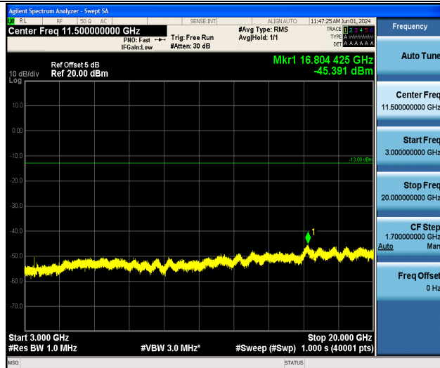
Band4_20MHz_QPSK_20300_1RB#0_3000~20000_3000~20000
