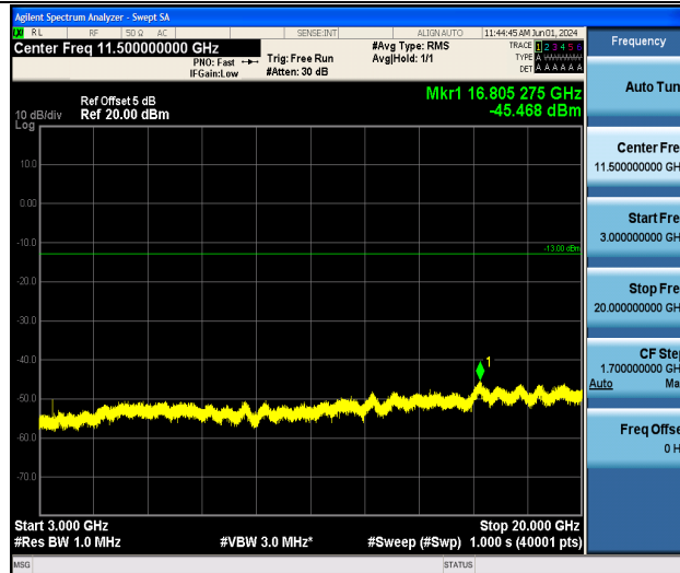
Band4_20MHz_16QAM_20050_1RB#0_3000~20000_3000~20000
