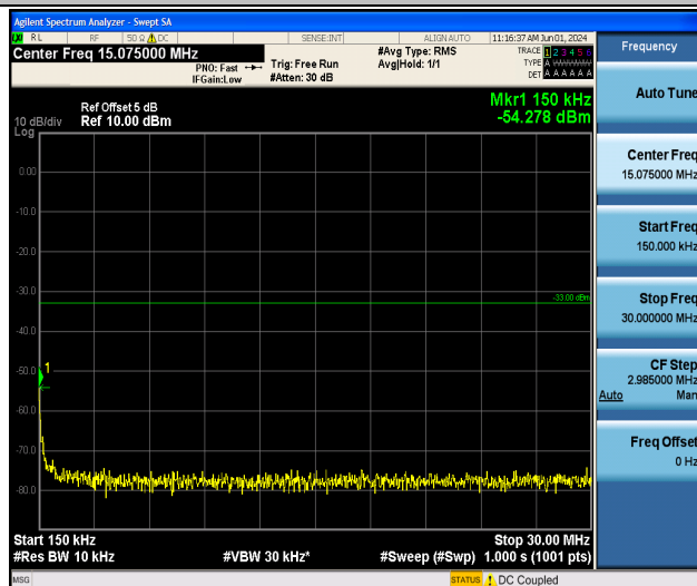
Band4_15MHz_16QAM_20325_1RB#0_0.15~30_0.15~30
