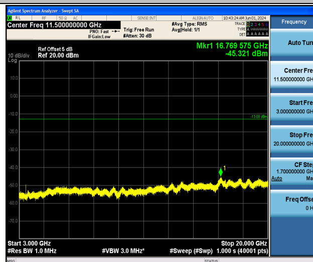
Band4_10MHz_QPSK_20175_1RB#0_3000~20000_3000~20000
