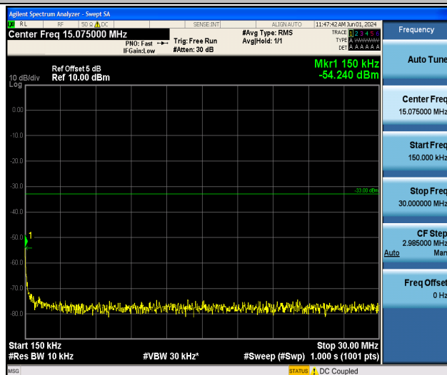
Band4_20MHz_16QAM_20300_1RB#0_0.15~30_0.15~30
