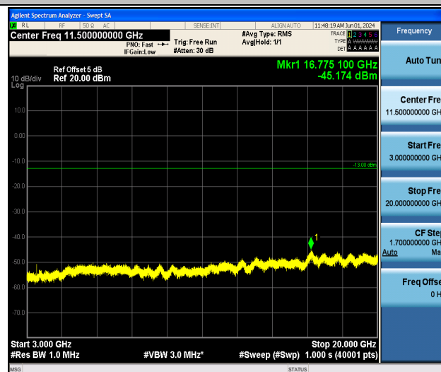
Band4_20MHz_16QAM_20300_1RB#0_3000~20000_3000~20000
