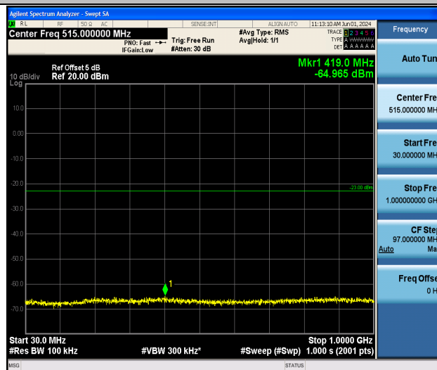
Band4_15MHz_16QAM_20025_1RB#0_30~1000_30~1000
