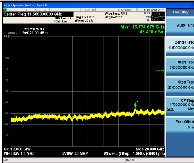
Band4_15MHz_QPSK_20025_1RB#0_3000~20000_3000~20000
