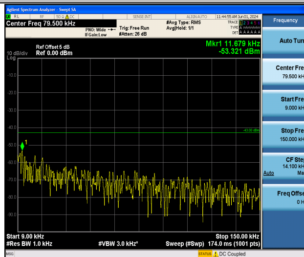
Band4_20MHz_QPSK_20175_1RB#0_0.009~0.15_0.009~0.15
