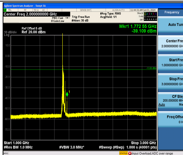
Band4_20MHz_16QAM_20050_1RB#0_1000~3000_1000~3000
