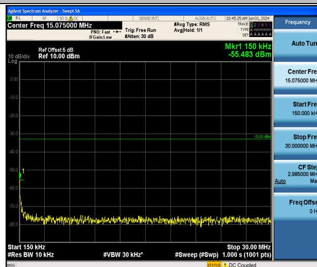
Band4_10MHz_16QAM_20350_1RB#0_0.15~30_0.15~30
