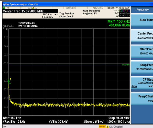
Band4_15MHz_QPSK_20175_1RB#0_0.15~30_0.15~30
