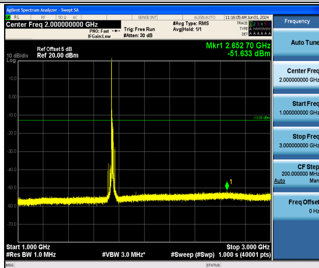
Band4_15MHz_QPSK_20325_1RB#0_1000~3000_1000~3000
