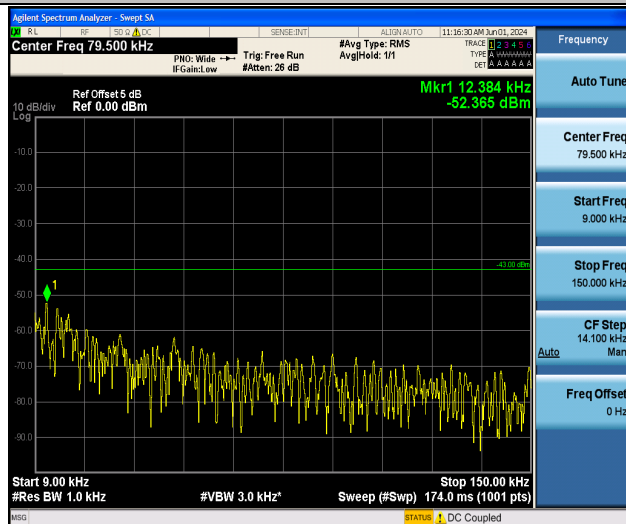
Band4_15MHz_16QAM_20325_1RB#0_0.009~0.15_0.009~0.15
