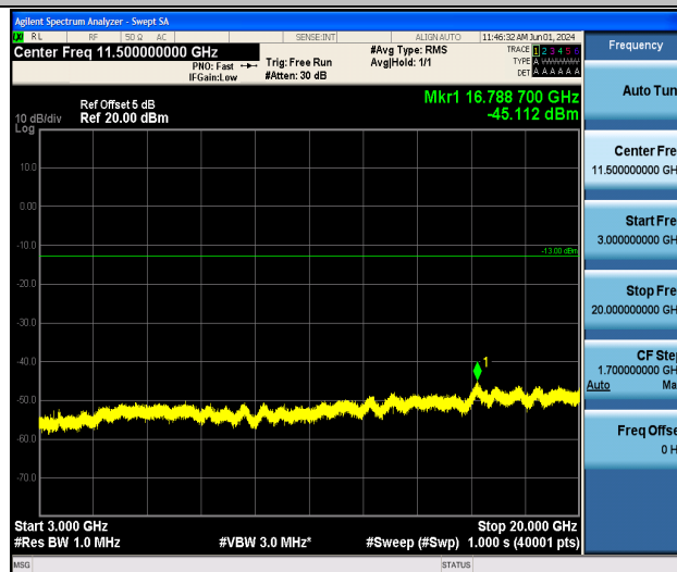
Band4_20MHz_16QAM_20175_1RB#0_3000~20000_3000~20000
