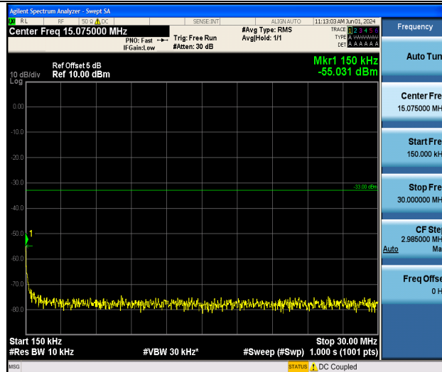
Band4_15MHz_16QAM_20025_1RB#0_0.15~30_0.15~30
