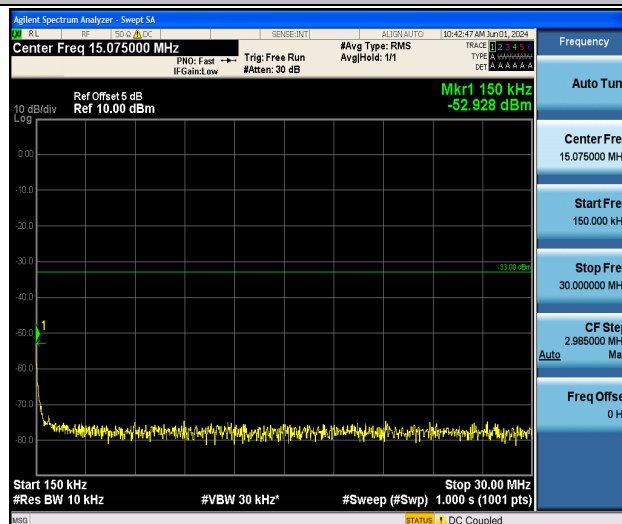
Band4_10MHz_QPSK_20175_1RB#0_0.15~30_0.15~30
