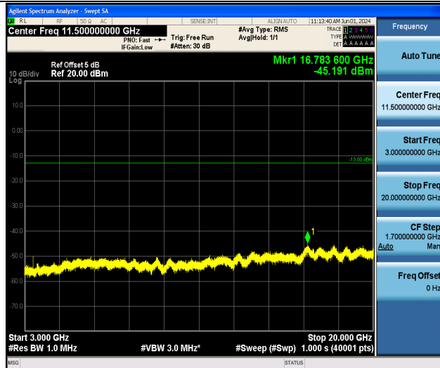
Band4_15MHz_16QAM_20025_1RB#0_3000~20000_3000~20000
