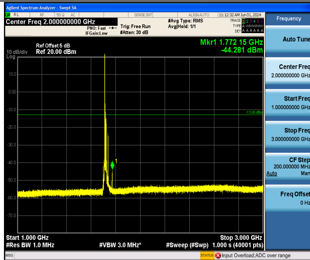
Band4_15MHz_QPSK_20025_1RB#0_1000~3000_1000~3000
