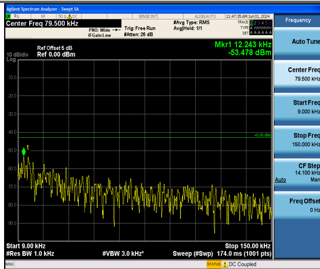
Band4_20MHz_16QAM_20300_1RB#0_0.009~0.15_0.009~0.15
