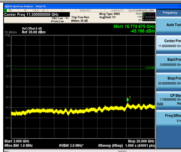
Band4_15MHz_16QAM_20325_1RB#0_3000~20000_3000~20000
