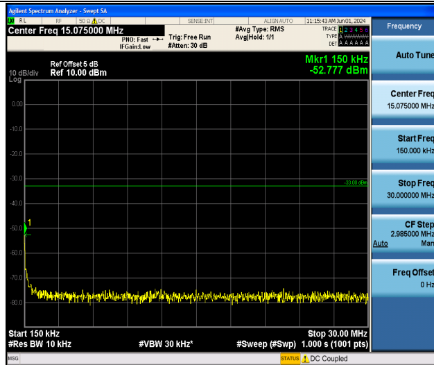
Band4_15MHz_QPSK_20325_1RB#0_0.15~30_0.15~30
