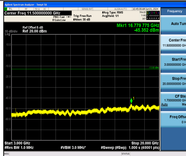
Band4_10MHz_QPSK_20350_1RB#0_3000~20000_3000~20000
