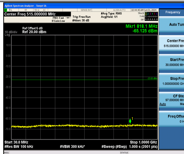
Band4_10MHz_QPSK_20350_1RB#0_30~1000_30~1000
