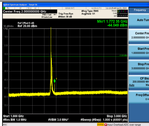
Band4_15MHz_16QAM_20025_1RB#0_1000~3000_1000~3000
