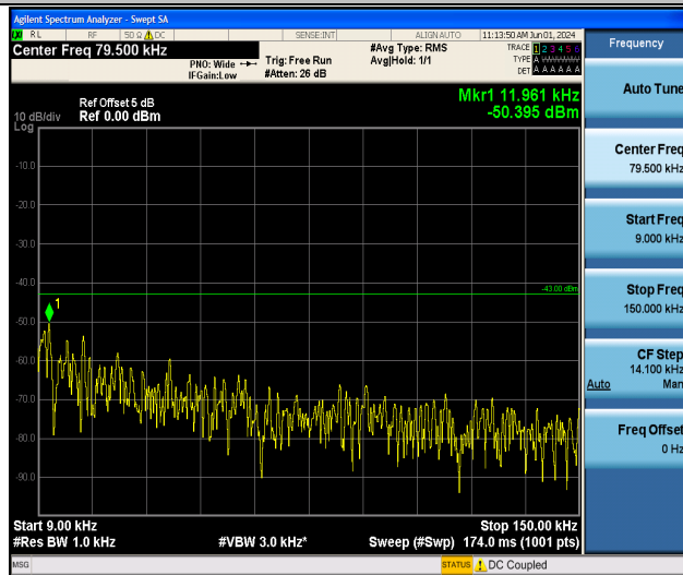
Band4_15MHz_QPSK_20175_1RB#0_0.009~0.15_0.009~0.15
