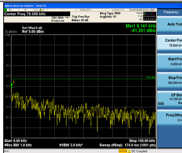
Band4_10MHz_16QAM_20350_1RB#0_0.009~0.15_0.009~0.15
