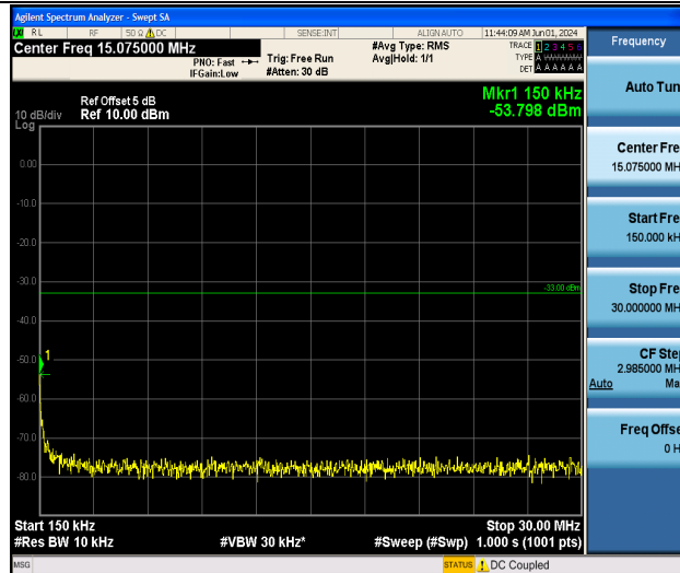
Band4_20MHz_16QAM_20050_1RB#0_0.15~30_0.15~30
