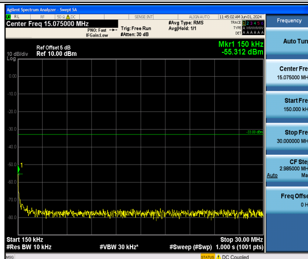
Band4_20MHz_QPSK_20175_1RB#0_0.15~30_0.15~30
