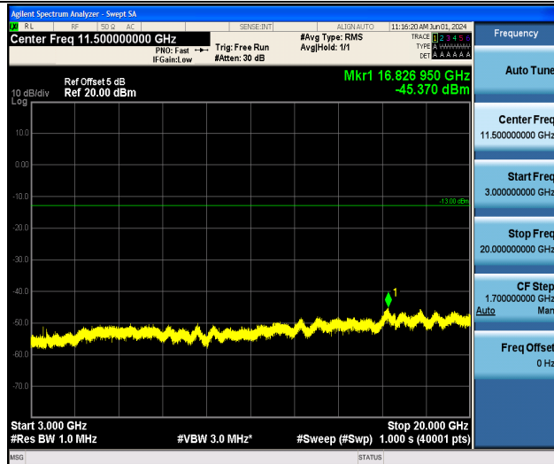
Band4_15MHz_QPSK_20325_1RB#0_3000~20000_3000~20000
