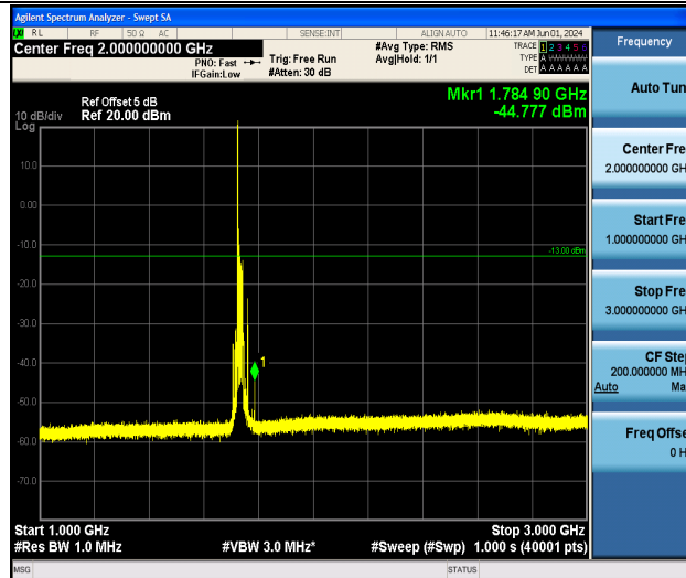
Band4_20MHz_16QAM_20175_1RB#0_1000~3000_1000~3000
