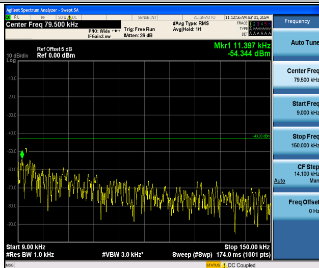
Band4_15MHz_16QAM_20025_1RB#0_0.009~0.15_0.009~0.15
