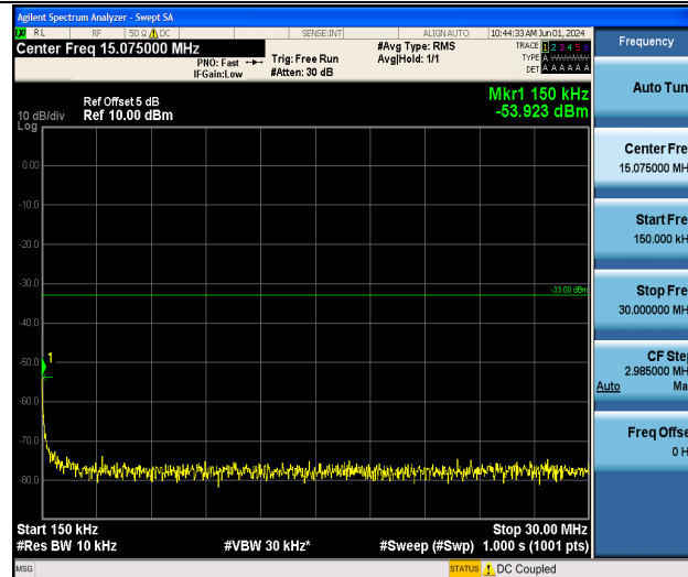
Band4_10MHz_QPSK_20350_1RB#0_0.15~30_0.15~30
