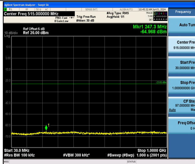
Band4_10MHz_16QAM_20350_1RB#0_30~1000_30~1000
