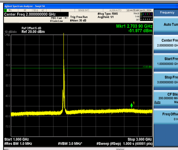
Band4_10MHz_QPSK_20350_1RB#0_1000~3000_1000~3000
