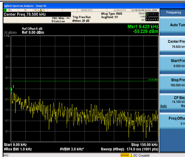
Band4_20MHz_QPSK_20300_1RB#0_0.009~0.15_0.009~0.15
