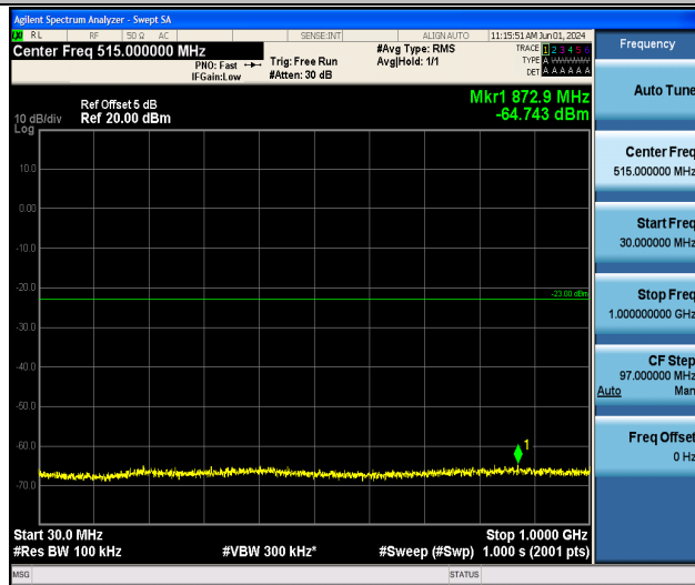
Band4_15MHz_QPSK_20325_1RB#0_30~1000_30~1000
