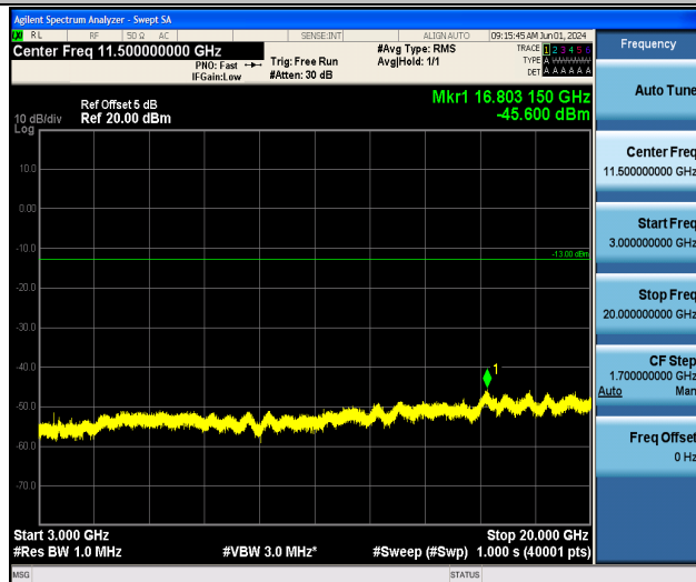
Band4_1.4MHz_16QAM_20175_1RB#0_3000~20000_3000~20000
