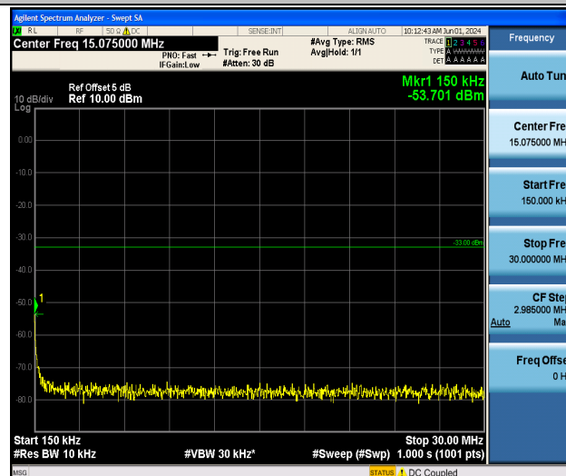
Band4_5MHz_QPSK_20175_1RB#0_0.15~30_0.15~30
