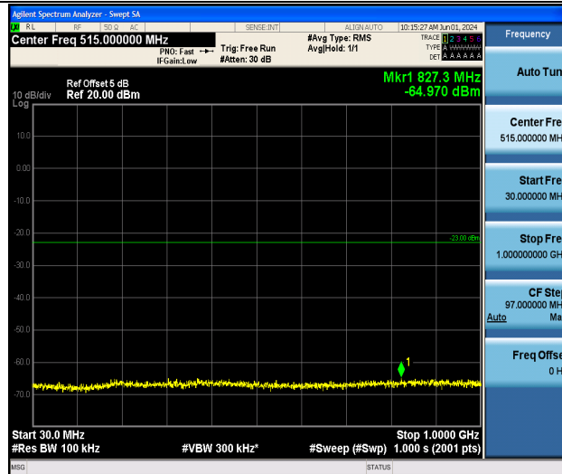
Band4_5MHz_16QAM_20375_1RB#0_30~1000_30~1000
