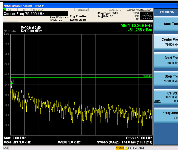
Band4_3MHz_16QAM_20385_1RB#0_0.009~0.15_0.009~0.15
