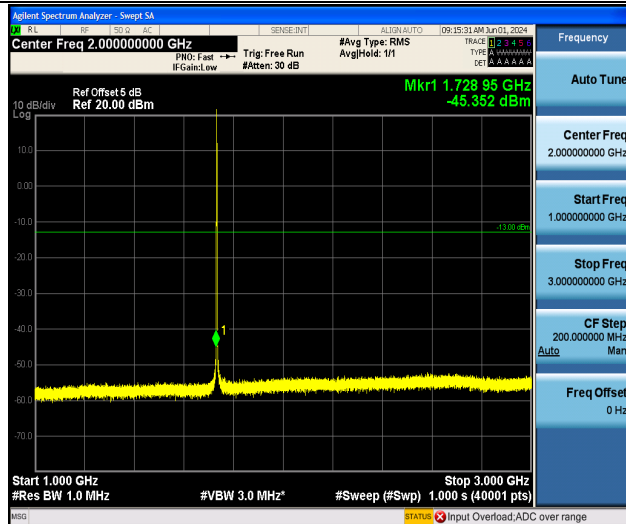
Band4_1.4MHz_16QAM_20175_1RB#0_1000~3000_1000~3000
