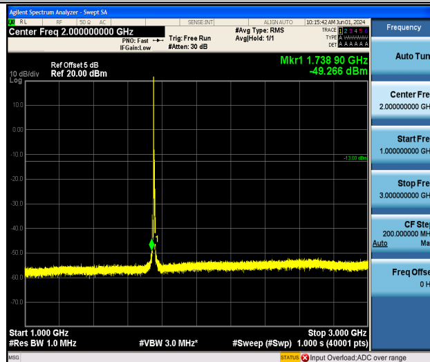
Band4_5MHz_16QAM_20375_1RB#0_1000~3000_1000~3000
