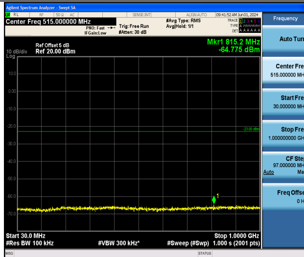
Band4_3MHz_QPSK_20175_1RB#0_30~1000_30~1000
