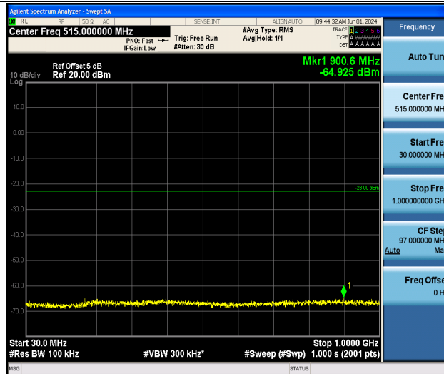
Band4_3MHz_16QAM_20385_1RB#0_30~1000_30~1000
