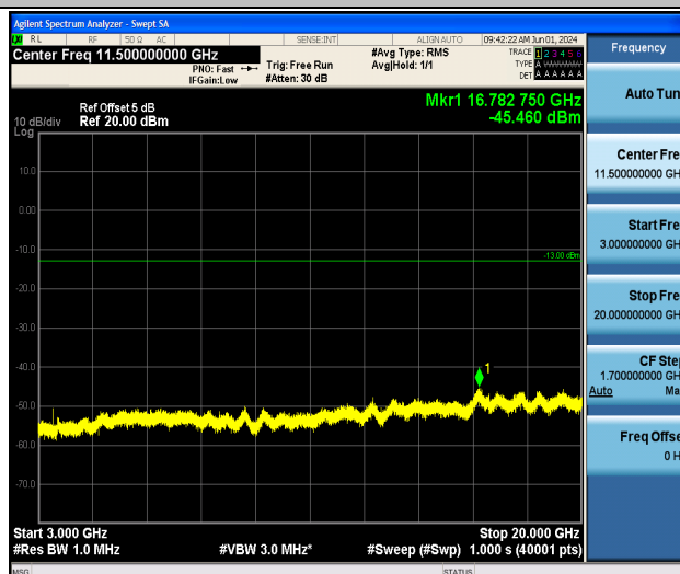
Band4_3MHz_QPSK_20175_1RB#0_3000~20000_3000~20000
