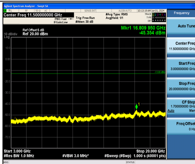
Band4_5MHz_QPSK_20175_1RB#0_3000~20000_3000~20000
