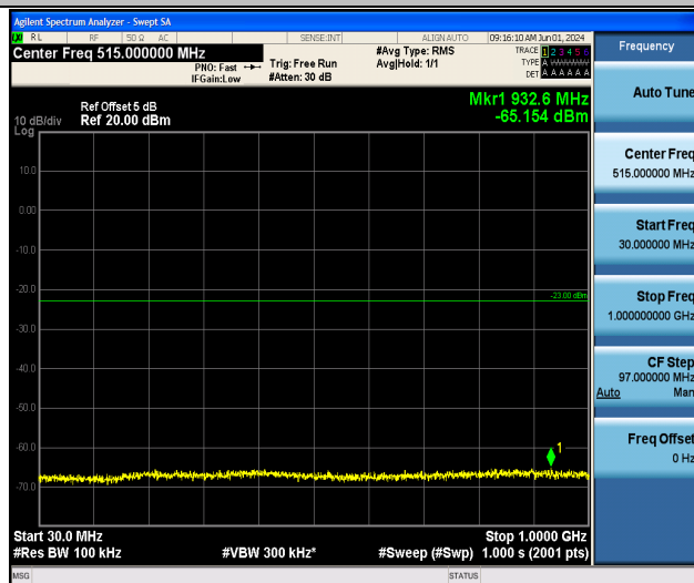
Band4_1.4MHz_QPSK_20393_1RB#0_30~1000_30~1000
