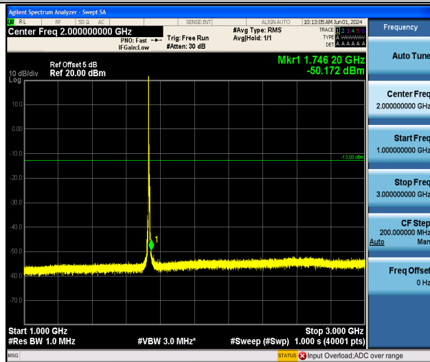
Band4_5MHz_QPSK_20175_1RB#0_1000~3000_1000~3000
