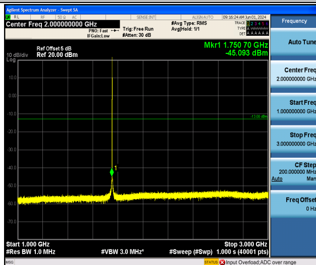
Band4_1.4MHz_QPSK_20393_1RB#0_1000~3000_1000~3000
