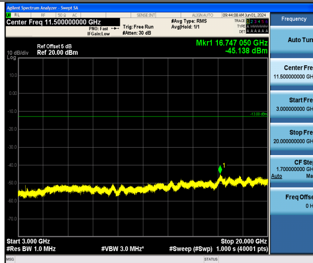
Band4_3MHz_QPSK_20385_1RB#0_3000~20000_3000~20000
