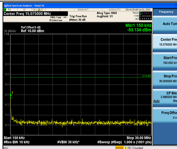
Band4_3MHz_16QAM_20385_1RB#0_0.15~30_0.15~30
