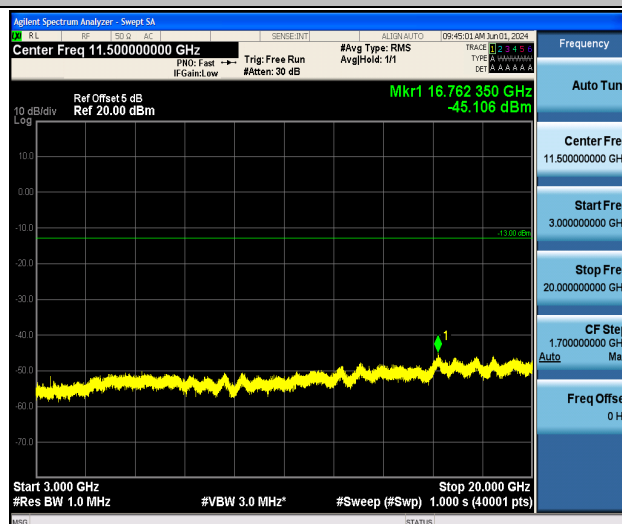
Band4_3MHz_16QAM_20385_1RB#0_3000~20000_3000~20000
