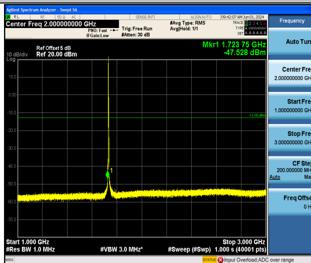
Band4_3MHz_QPSK_20175_1RB#0_1000~3000_1000~3000
