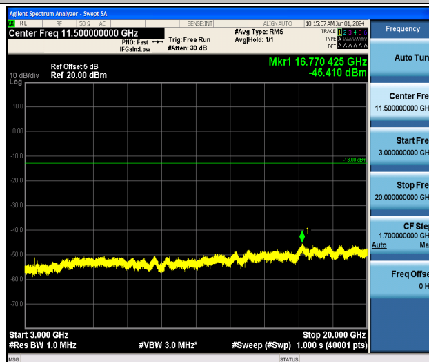
Band4_5MHz_16QAM_20375_1RB#0_3000~20000_3000~20000
