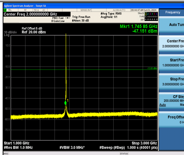
Band4_3MHz_16QAM_20385_1RB#0_1000~3000_1000~3000
