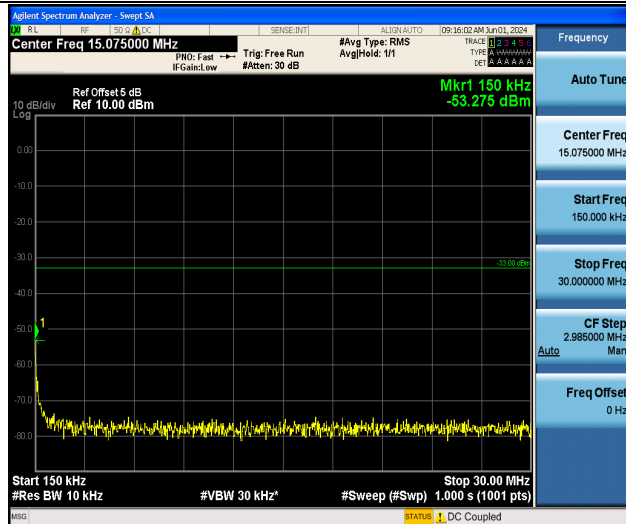
Band4_1.4MHz_QPSK_20393_1RB#0_0.15~30_0.15~30
