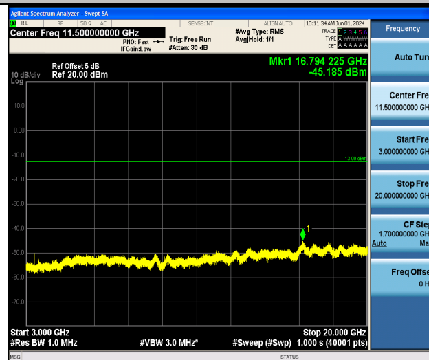
Band4_5MHz_QPSK_19975_1RB#0_3000~20000_3000~20000
