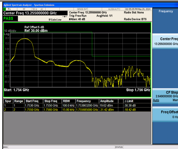
Band4_1.4MHz_16QAM_20393_1RB#0
