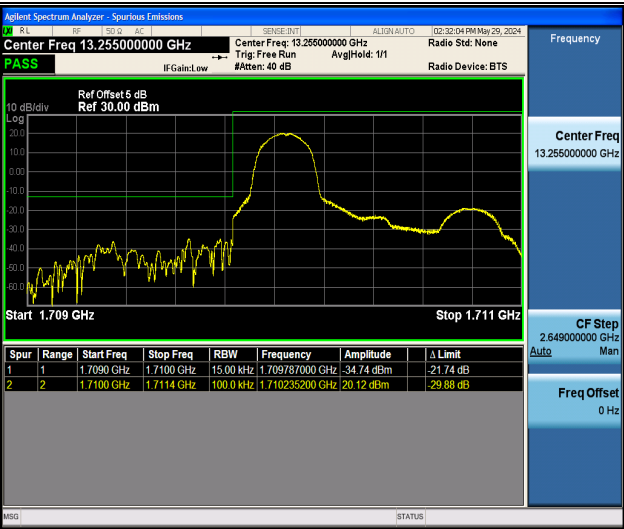
Band4_1.4MHz_QPSK_19957_1RB#0
