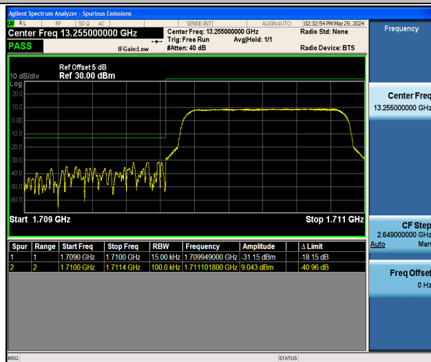
Band4_1.4MHz_16QAM_19957_6RB#0
