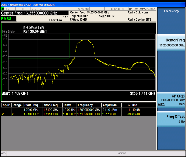
Band4_1.4MHz_16QAM_19957_1RB#0
