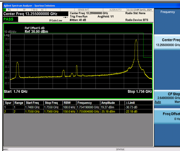
Band4_15MHz_QPSK_20325_1RB#74
