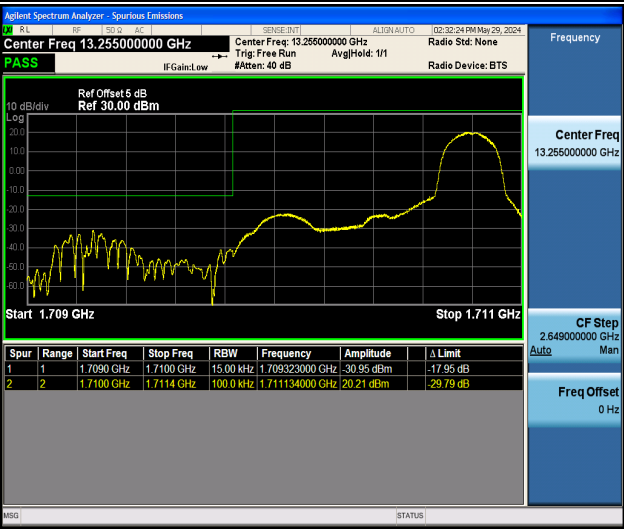
Band4_1.4MHz_QPSK_19957_1RB#5
