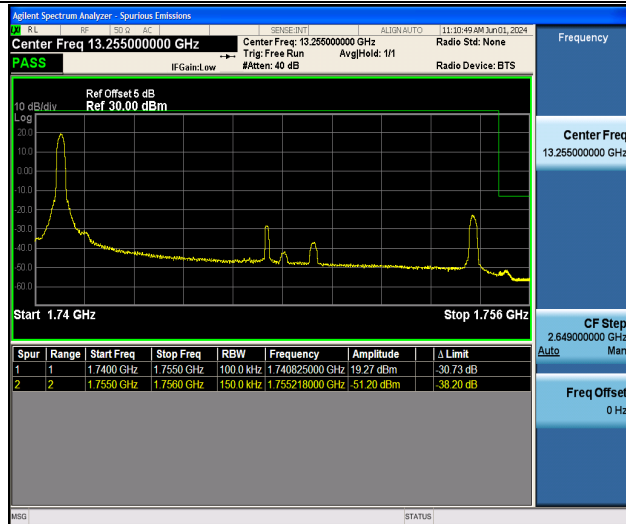
Band4_15MHz_QPSK_20325_1RB#0
