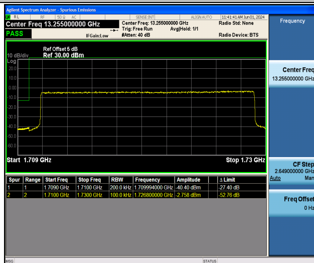
Band4_20MHz_16QAM_20050_100RB#0
