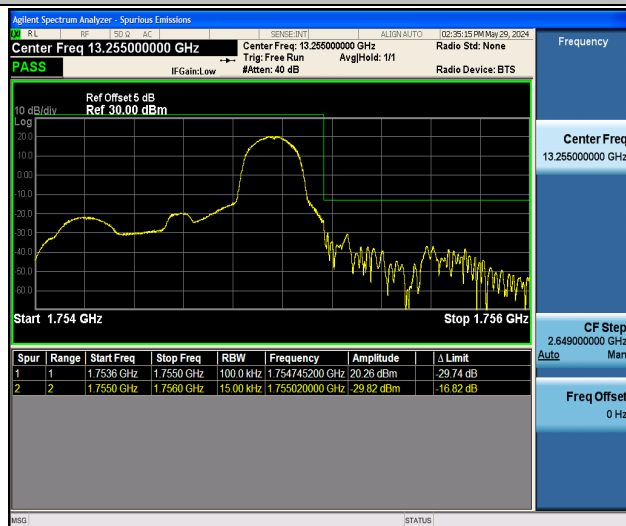
Band4_1.4MHz_QPSK_20393_1RB#5
