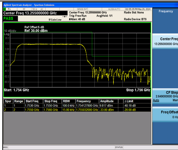
Band4_1.4MHz_QPSK_20393_6RB#0
