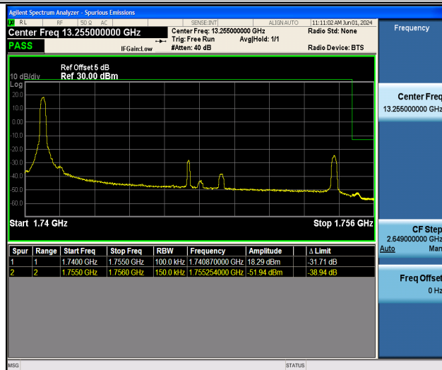
Band4_15MHz_16QAM_20325_1RB#0
