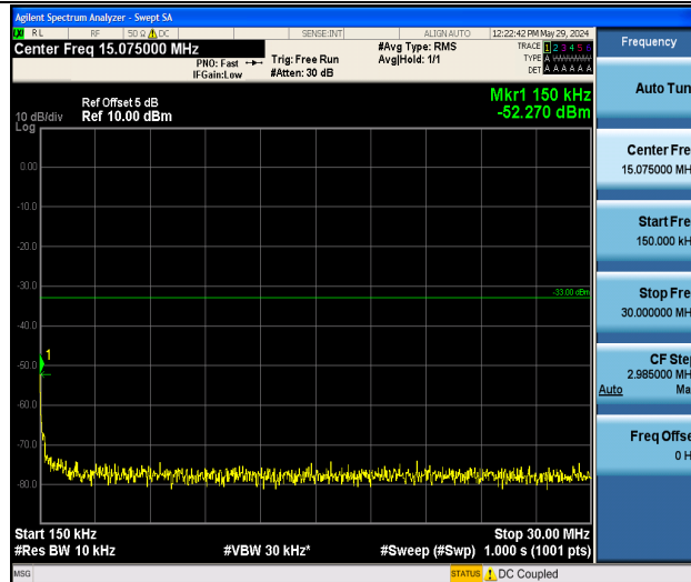
Band2_15MHz_QPSK_19125_1RB#0_0.15~30_0.15~30
