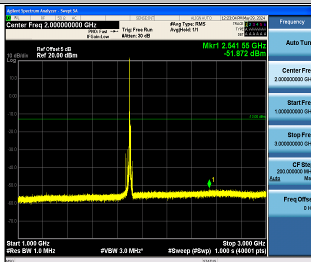
Band2_15MHz_QPSK_19125_1RB#0_1000~3000_1000~3000
