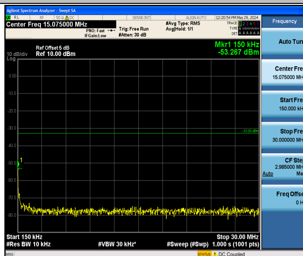
Band2_15MHz_QPSK_18900_1RB#0_0.15~30_0.15~30
