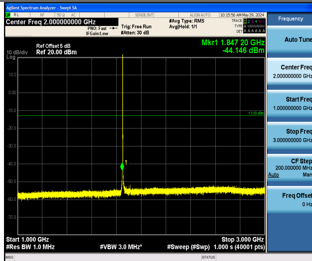
Band2_1.4MHz_QPSK_18607_1RB#0_1000~3000_1000~3000
