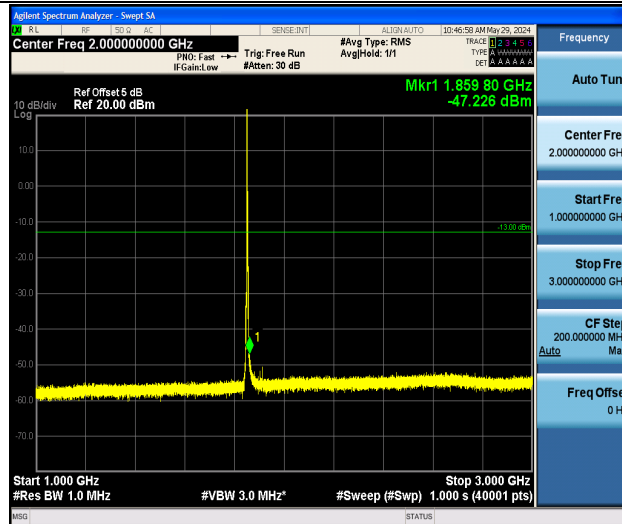
Band2_3MHz_QPSK_18615_1RB#0_1000~3000_1000~3000
