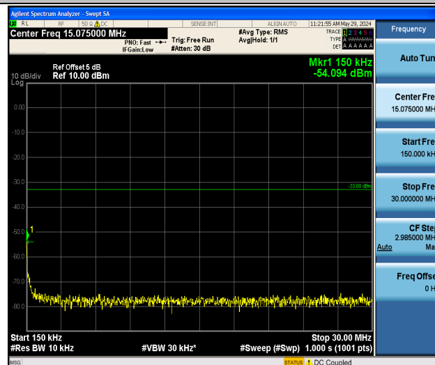
Band2_5MHz_16QAM_19175_1RB#0_0.15~30_0.15~30
