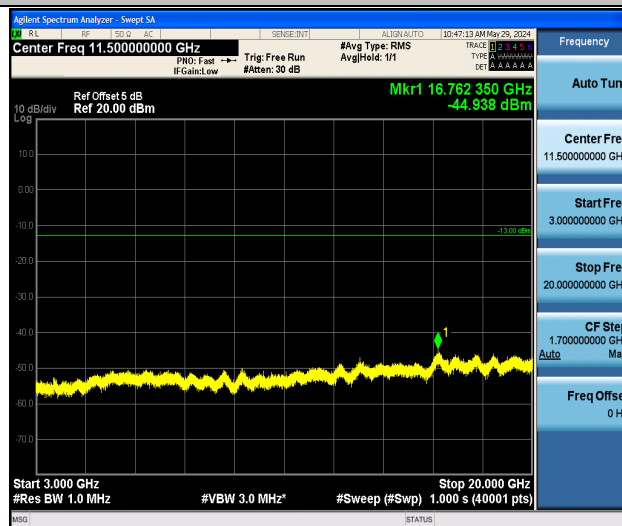
Band2_3MHz_QPSK_18615_1RB#0_3000~20000_3000~20000
