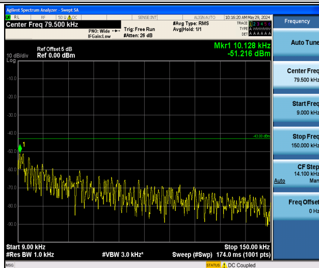
Band2_1.4MHz_16QAM_18607_1RB#0_0.009~0.15_0.009~0.15
