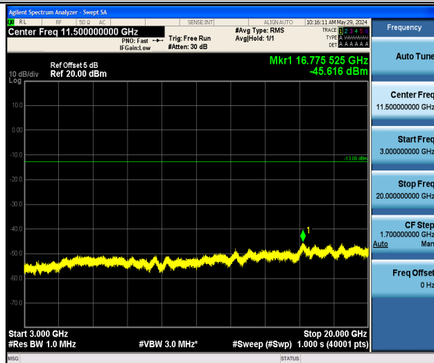
Band2_1.4MHz_QPSK_18607_1RB#0_3000~20000_3000~20000
