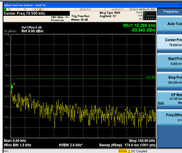
Band2_3MHz_QPSK_18900_1RB#0_0.009~0.15_0.009~0.15
