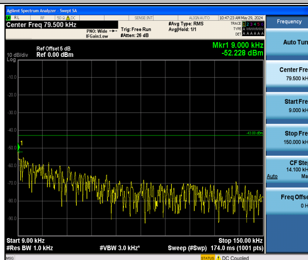
Band2_3MHz_16QAM_18615_1RB#0_0.009~0.15_0.009~0.15
