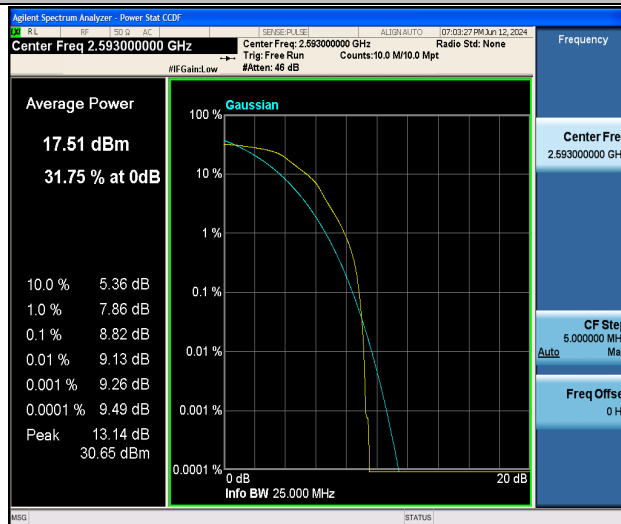
Band41-5MHz-16QAM-40620-25RB#0-PASS
