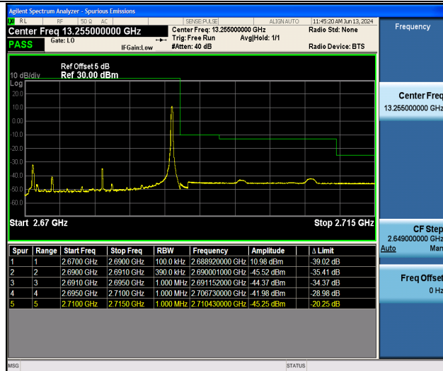
Band41_20MHz_16QAM_41490_1RB#99
