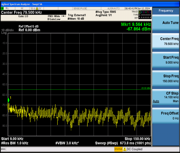
Band41_5MHz_16QAM_39675_1RB#0_0.009~0.15_0.009~0.15
