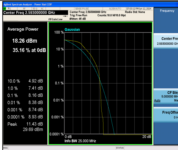
Band41-5MHz-QPSK-40620-25RB#0-PASS
