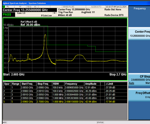
Band41_5MHz_QPSK_41565_1RB#24
