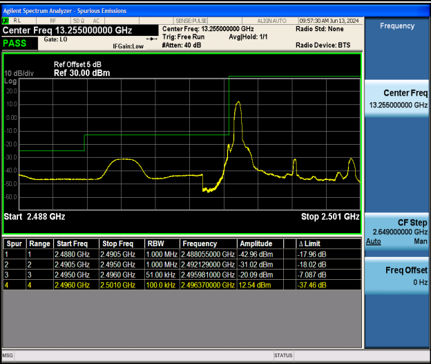
Band41_5MHz_16QAM_39675_1RB#0
