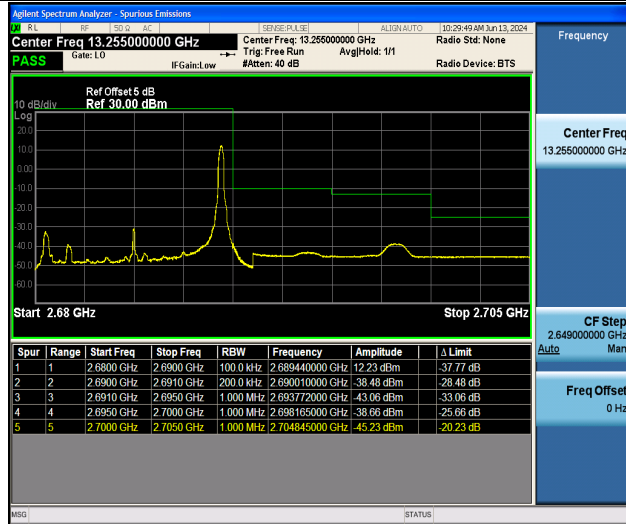
Band41_10MHz_QPSK_41540_1RB#49
