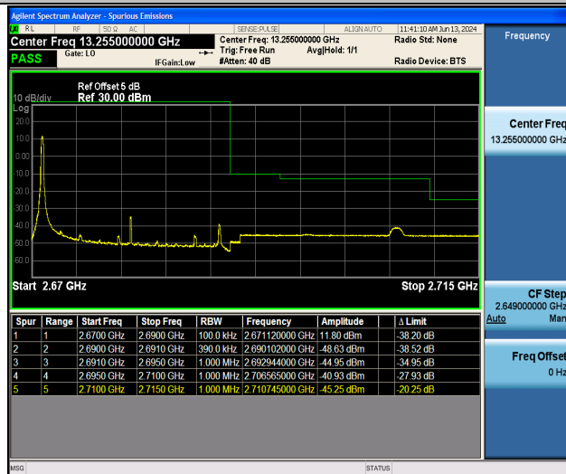
Band41_20MHz_16QAM_41490_1RB#0
