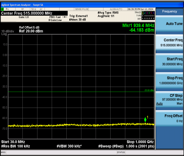
Band41_5MHz_QPSK_39675_1RB#0_30~1000_30~1000
