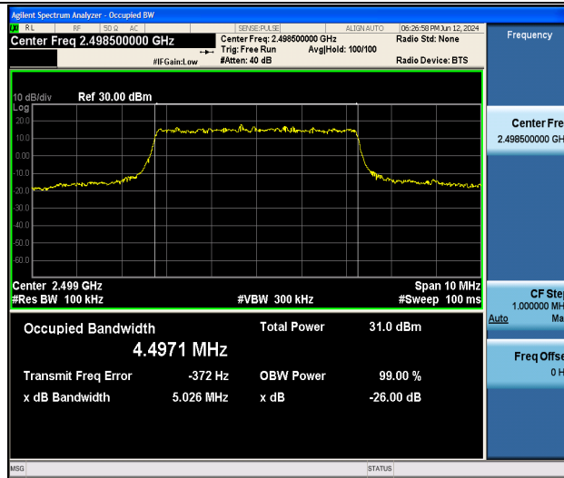
Band41-5MHz-QPSK-39675-25RB#0-PASS
