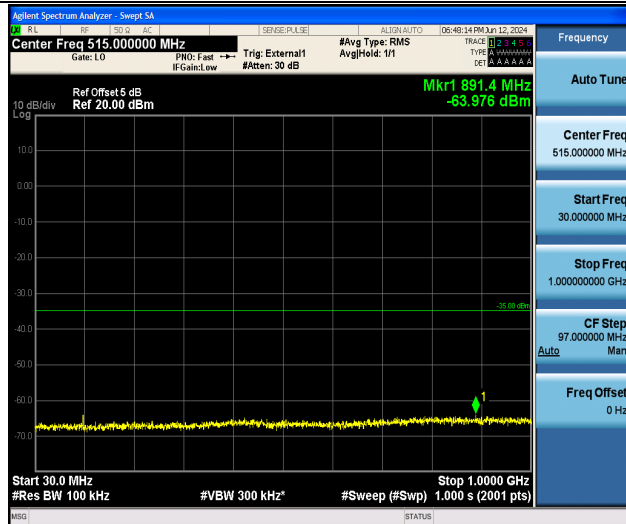
Band41_5MHz_16QAM_41565_1RB#0_30~1000_30~1000
