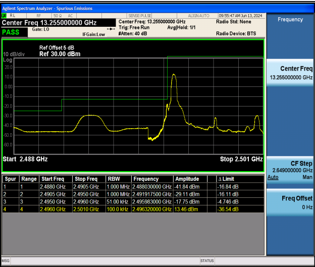
Band41_5MHz_QPSK_39675_1RB#0
