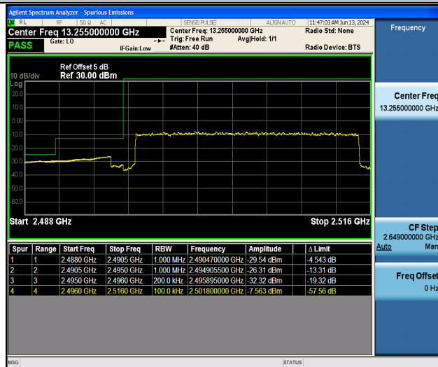
Band41_20MHz_QPSK_39750_100RB#0
