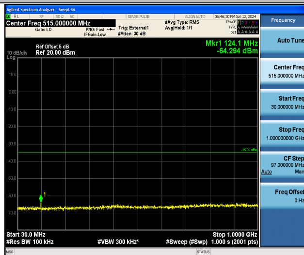
Band41_5MHz_QPSK_41565_1RB#0_30~1000_30~1000
