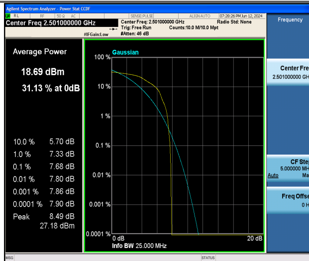
Band41-10MHz-16QAM-39700-1RB#0-PASS
