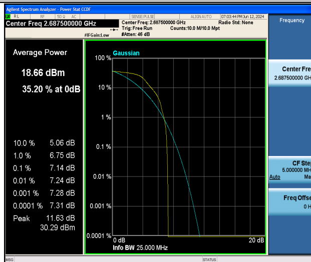
Band41-5MHz-QPSK-41565-1RB#0-PASS
