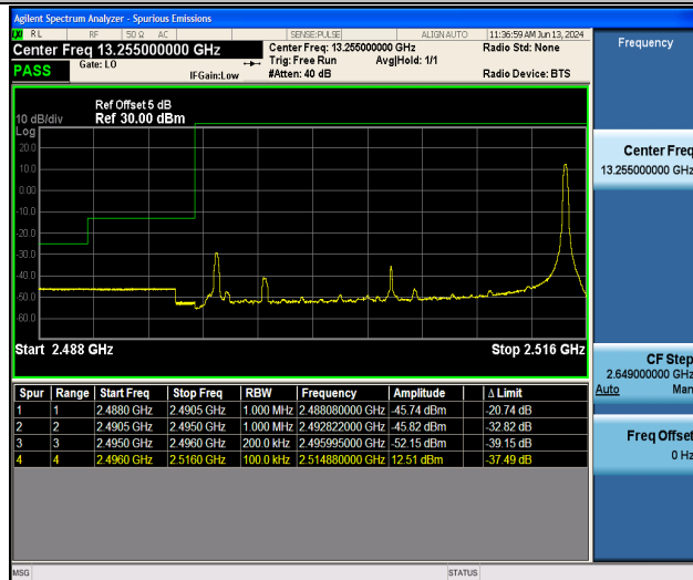
Band41_20MHz_16QAM_39750_1RB#99
