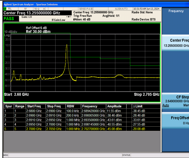
Band41_10MHz_16QAM_41540_1RB#49
