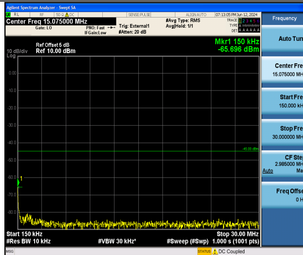
Band41_10MHz_QPSK_39700_1RB#0_0.15~30_0.15~30
