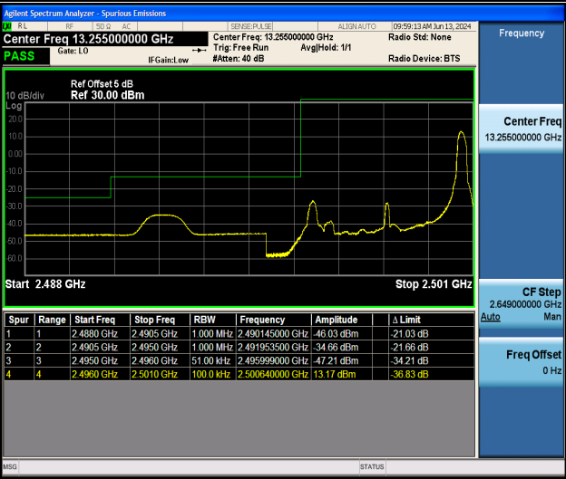
Band41_5MHz_QPSK_39675_1RB#24
