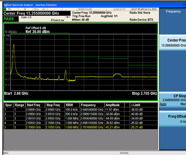
Band41_10MHz_16QAM_41540_1RB#0
