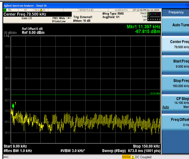
Band41_10MHz_QPSK_39700_1RB#0_0.009~0.15_0.009~0.15
