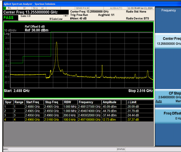
Band41_20MHz_16QAM_39750_1RB#0
