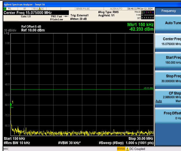
Band41_5MHz_QPSK_41565_1RB#0_0.15~30_0.15~30
