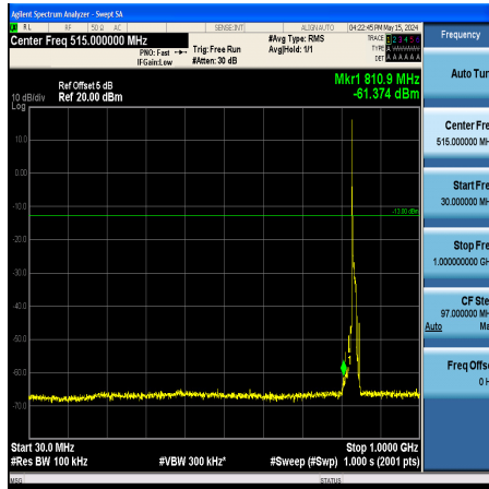
Band26_10MHz_QPSK_26915_1RB#0_30~1000_30~1000
