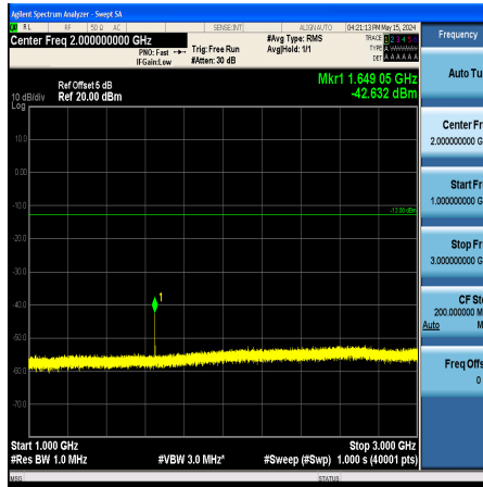
Band26_10MHz_QPSK_26840_1RB#0_1000~3000_1000~3000
