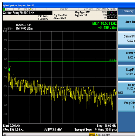
Band26_10MHz_16QAM_26840_1RB#0_0.009~0.15_0.009~0.15
