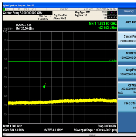
Band26_10MHz_QPSK_26915_1RB#0_1000~3000_1000~3000
