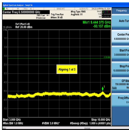
Band26_10MHz_QPSK_26915_1RB#0_3000~10000_3000~10000
