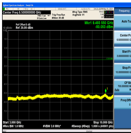
Band26_10MHz_QPSK_26840_1RB#0_3000~10000_3000~10000
