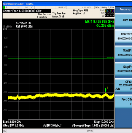
Band26_5MHz_QPSK_27015_1RB#0_3000~10000_3000~10000
