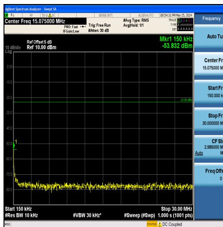
Band26_5MHz_16QAM_27015_1RB#0_0.15~30_0.15~30
