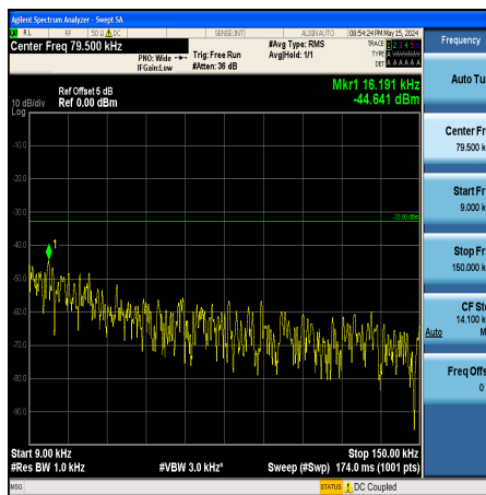
Band26_5MHz_16QAM_27015_1RB#0_0.009~0.15_0.009~0.15
