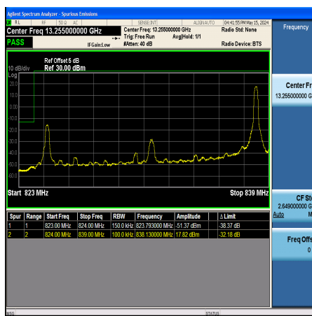
Band26_15MHz_16QAM_26865_1RB#74
