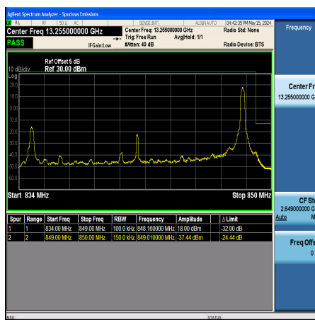
Band26_15MHz_QPSK_26965_1RB#74
