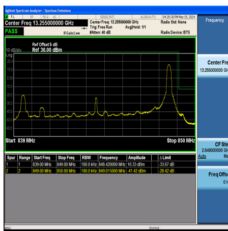
Band26_10MHz_16QAM_26990_1RB#49
