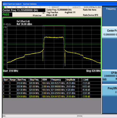
Band26_3MHz_QPSK_26775_15RB#0
