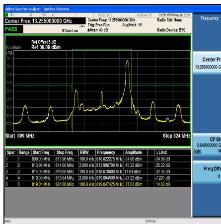
Band26_5MHz_16QAM_26715_1RB#24
