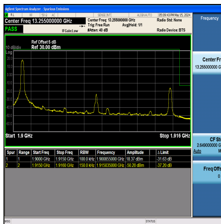
Band25_15MHz_16QAM_26615_1RB#0
