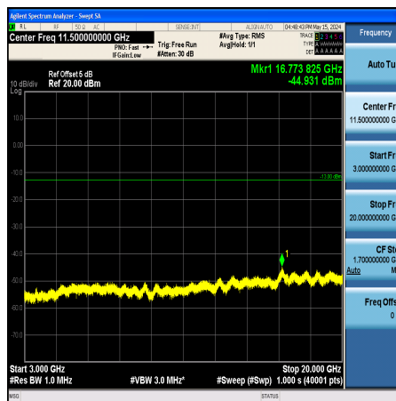
Band25_10MHz_QPSK_26090_1RB#0_3000~20000_3000~20000
