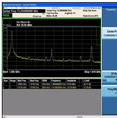
Band25_20MHz_QPSK_26590_1RB#0
