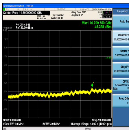
Band25_1.4MHz_QPSK_26365_1RB#0_3000~20000_3000~20000
