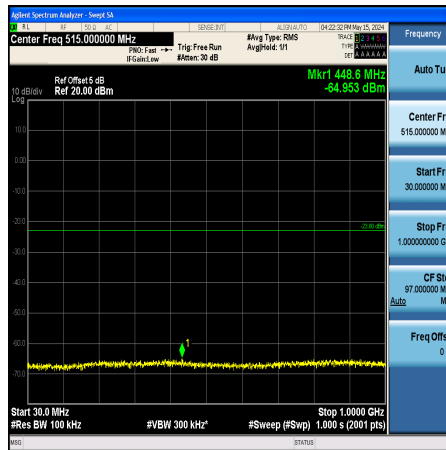
Band25_5MHz_QPSK_26365_1RB#0_30~1000_30~1000
