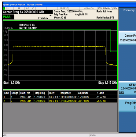
Band25_15MHz_QPSK_26615_75RB#0
