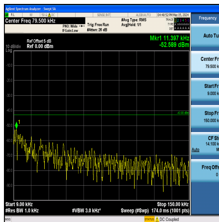
Band25_10MHz_16QAM_26090_1RB#0_0.009~0.15_0.009~0.15
