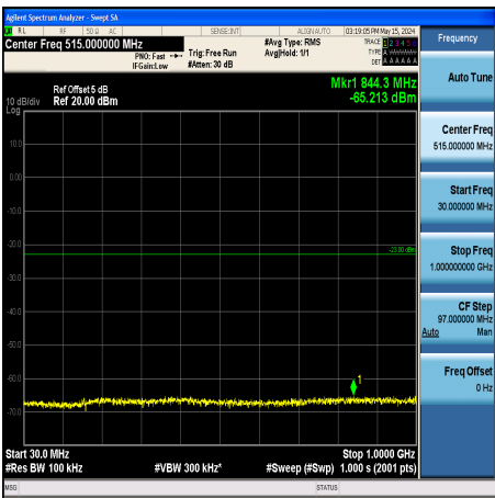
Band25_1.4MHz_QPSK_26047_1RB#0_30~1000_30~1000
