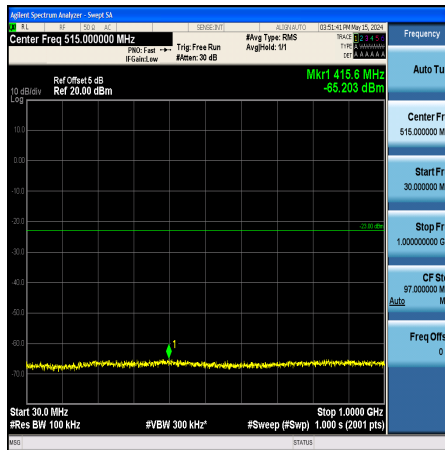
Band25_3MHz_QPSK_26365_1RB#0_30~1000_30~1000
