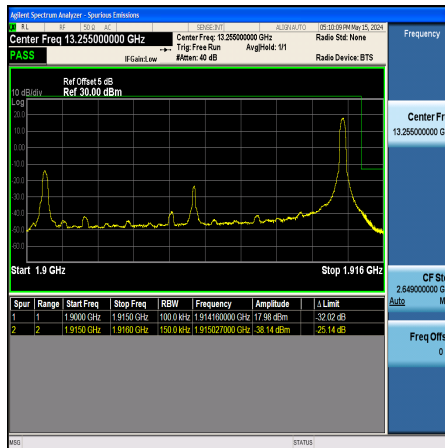
Band25_15MHz_16QAM_26615_1RB#74
