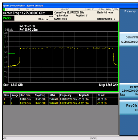
Band25_15MHz_QPSK_26115_75RB#0
