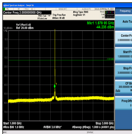
Band25_1.4MHz_QPSK_26365_1RB#0_1000~3000_1000~3000
