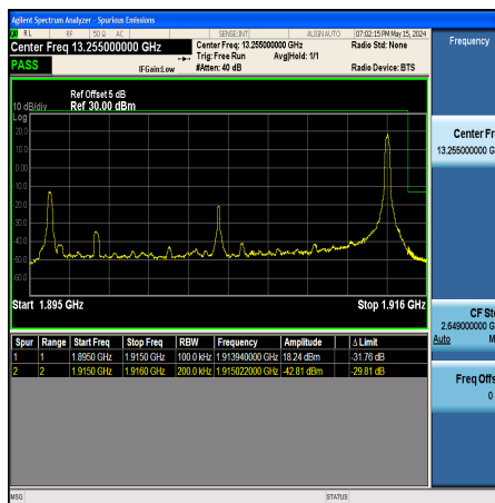
Band25_20MHz_16QAM_26590_1RB#99
