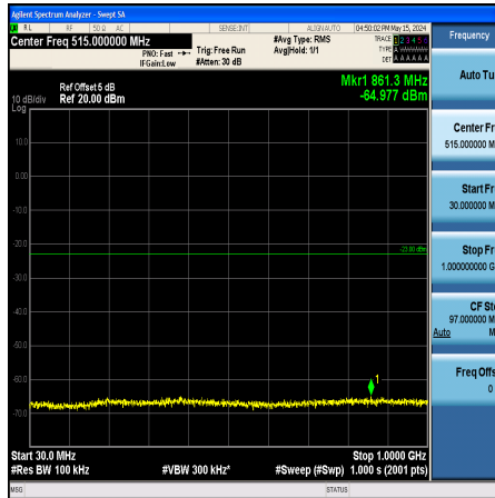
Band25_10MHz_QPSK_26365_1RB#0_30~1000_30~1000
