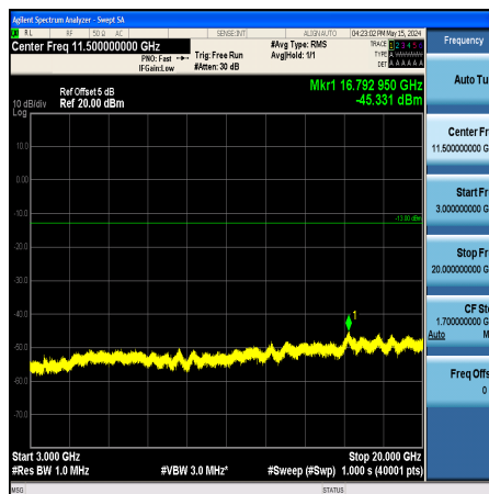
Band25_5MHz_QPSK_26365_1RB#0_3000~20000_3000~20000
