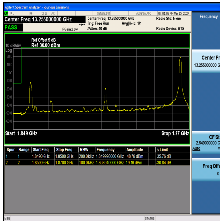
Band25_20MHz_QPSK_26140_1RB#99
