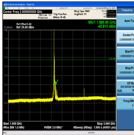
Band25_10MHz_QPSK_26090_1RB#0_1000~3000_1000~3000
