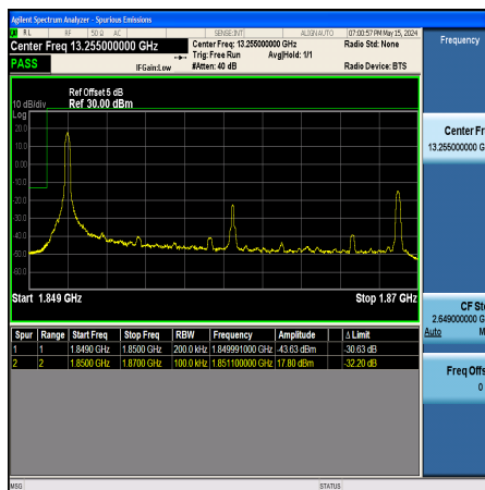
Band25_20MHz_16QAM_26140_1RB#0
