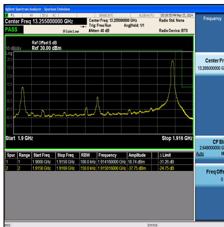
Band25_15MHz_QPSK_26615_1RB#74
