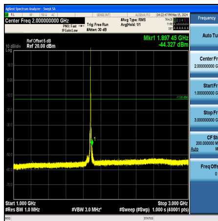
Band25_5MHz_QPSK_26365_1RB#0_1000~3000_1000~3000
