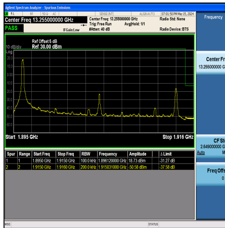
Band25_20MHz_16QAM_26590_1RB#0
