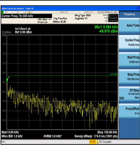
Band25_1.4MHz_QPSK_26047_1RB#0_0.009~0.15_0.009~0.15
