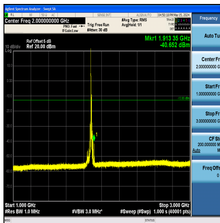
Band25_10MHz_QPSK_26365_1RB#0_1000~3000_1000~3000
