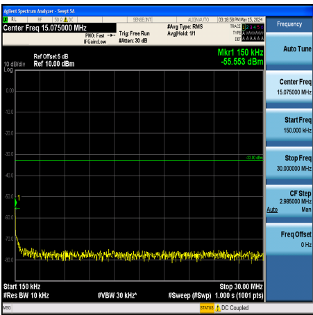
Band25_1.4MHz_QPSK_26047_1RB#0_0.15~30_0.15~30
