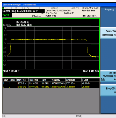
Band25_10MHz_QPSK_26640_50RB#0
