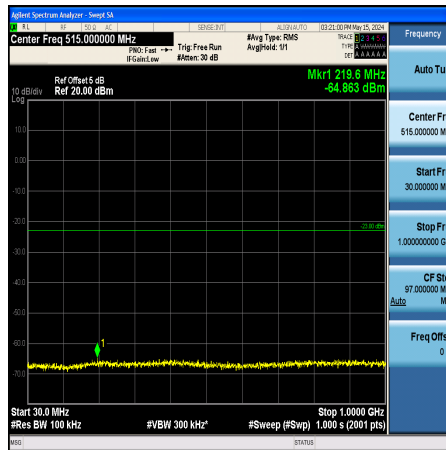
Band25_1.4MHz_QPSK_26365_1RB#0_30~1000_30~1000
