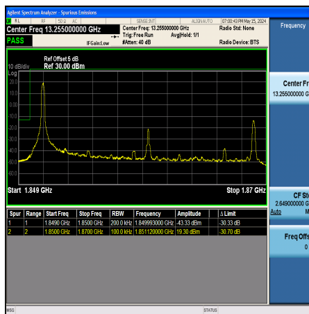
Band25_20MHz_QPSK_26140_1RB#0
