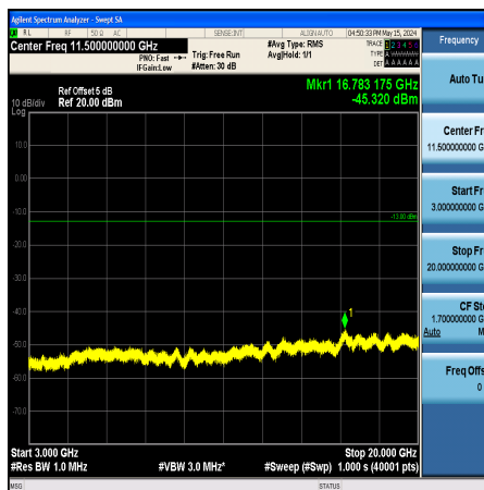
Band25_10MHz_QPSK_26365_1RB#0_3000~20000_3000~20000
