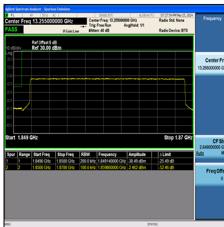
Band25_20MHz_QPSK_26140_100RB#0
