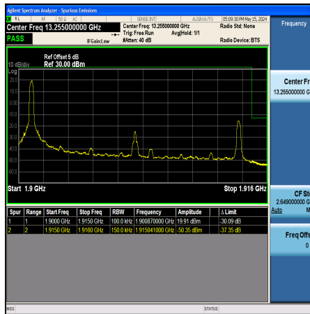
Band25_15MHz_QPSK_26615_1RB#0
