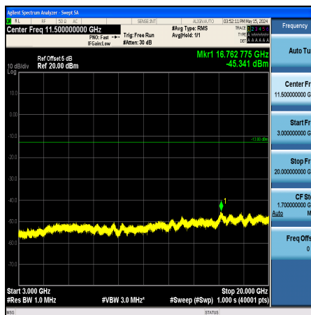
Band25_3MHz_QPSK_26365_1RB#0_3000~20000_3000~20000
