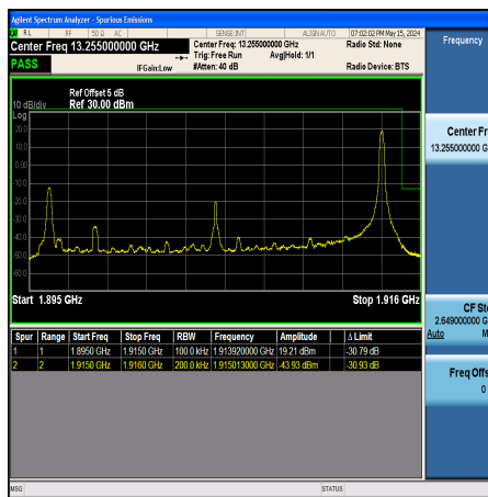
Band25_20MHz_QPSK_26590_1RB#99
