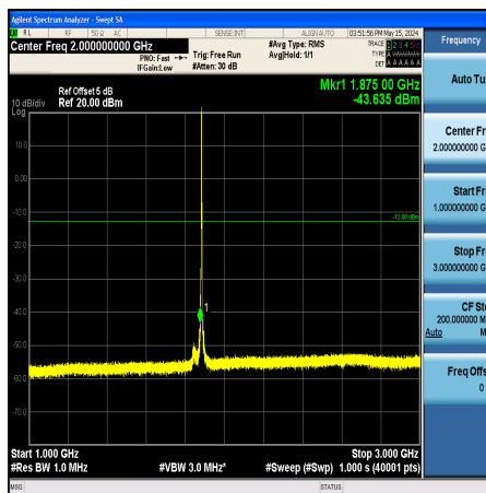
Band25_3MHz_QPSK_26365_1RB#0_1000~3000_1000~3000
