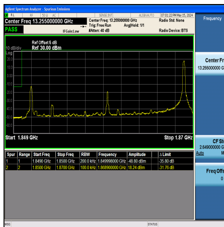
Band25_20MHz_16QAM_26140_1RB#99
