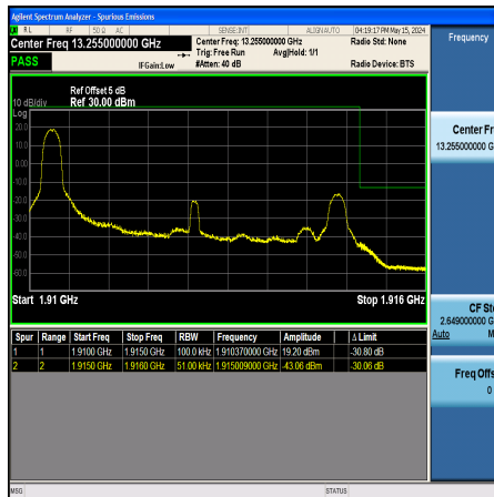
Band25_5MHz_QPSK_26665_1RB#0
