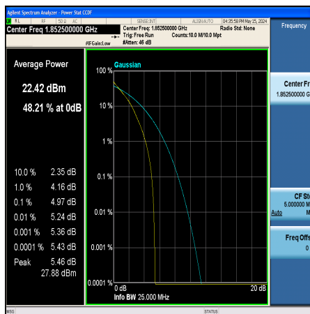
Band25-5MHz-QPSK-26065-25RB#0-PASS
