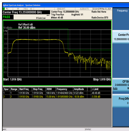
Band25_1.4MHz_QPSK_26683_6RB#0
