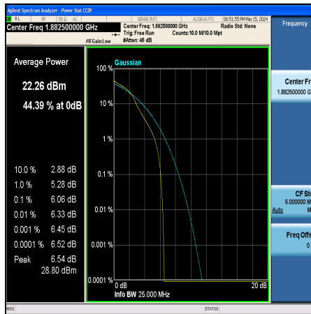
Band25-15MHz-16QAM-26365-1RB#0-PASS
