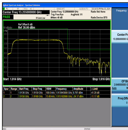
Band25_1.4MHz_16QAM_26683_6RB#0
