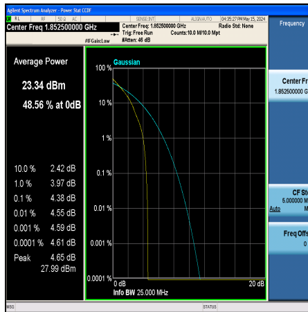
Band25-5MHz-QPSK-26065-1RB#0-PASS
