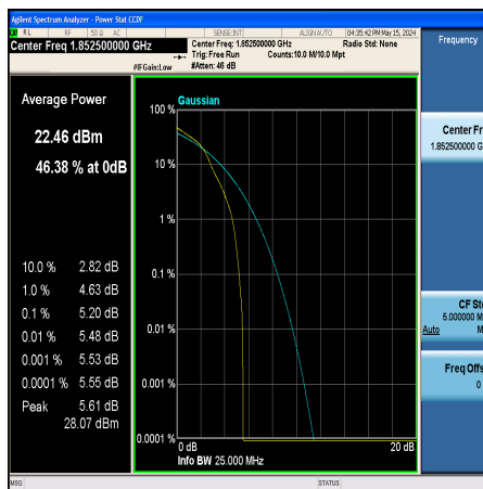
Band25-5MHz-16QAM-26065-1RB#0-PASS
