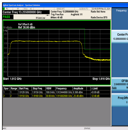
Band25_3MHz_QPSK_26675_15RB#0
