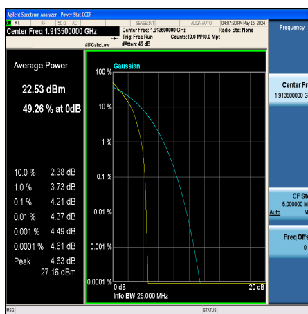
Band25-3MHz-QPSK-26675-15RB#0-PASS
