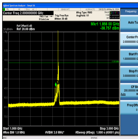
Band2_15MHz_QPSK_19125_1RB#0_1000~3000_1000~3000
