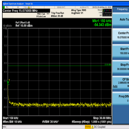
Band2_15MHz_QPSK_19125_1RB#0_0.15~30_0.15~30
