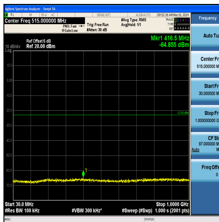
Band2_15MHz_QPSK_19125_1RB#0_30~1000_30~1000
