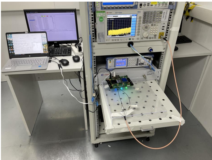
Conducted Test-WIFI
