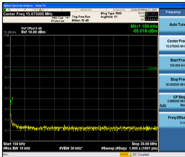
Band26_3MHz_QPSK_26775_1RB#0_0.15~30_0.15~30
