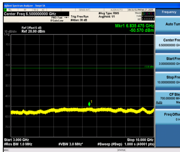
Band26_1.4MHz_QPSK_26697_1RB#0_3000~10000_3000~10000
