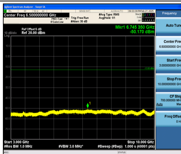
Band26_1.4MHz_QPSK_26740_1RB#0_3000~10000_3000~10000
