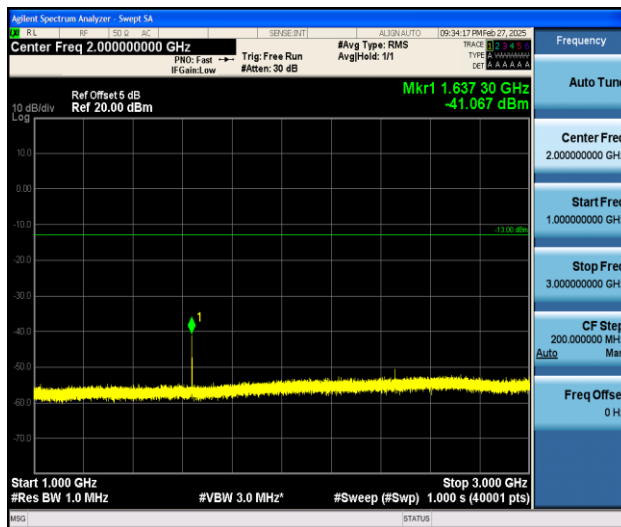
Band26_1.4MHz_16QAM_26740_1RB#0_1000~3000_1000~3000
