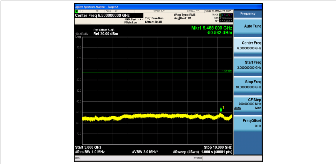
Band26_3MHz_16QAM_26705_1RB#0_3000~10000_3000~10000
