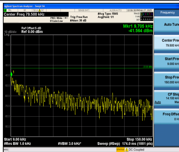
Band26_3MHz_QPSK_26775_1RB#0_0.009~0.15_0.009~0.15
