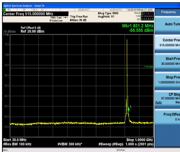
Band26_3MHz_QPSK_26775_1RB#0_30~1000_30~1000
