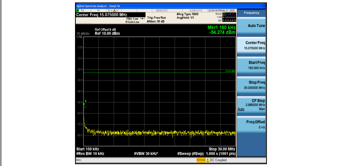
Band26_3MHz_16QAM_26740_1RB#0_0.15~30_0.15~30
