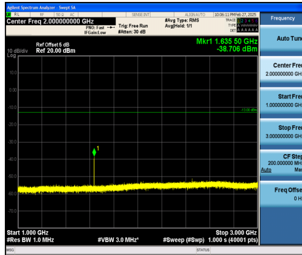
Band26_3MHz_16QAM_26740_1RB#0_1000~3000_1000~3000
