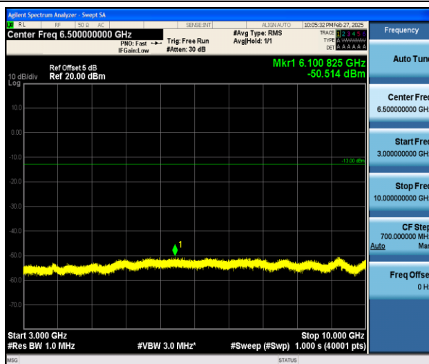
Band26_3MHz_QPSK_26740_1RB#0_3000~10000_3000~10000
