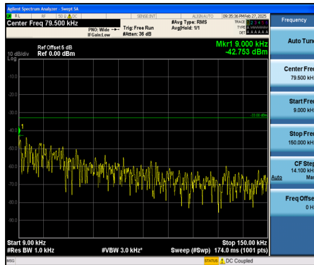
Band26_1.4MHz_16QAM_26783_1RB#0_0.009~0.15_0.009~0.15
