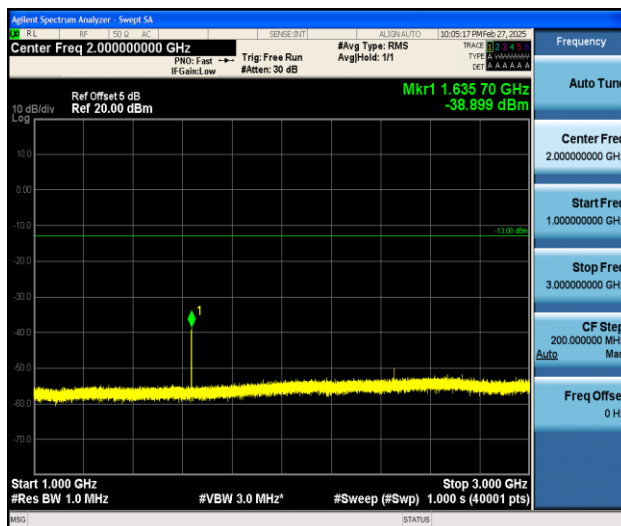
Band26_3MHz_QPSK_26740_1RB#0_1000~3000_1000~3000
