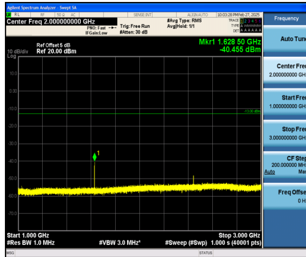
Band26_3MHz_QPSK_26705_1RB#0_1000~3000_1000~3000
