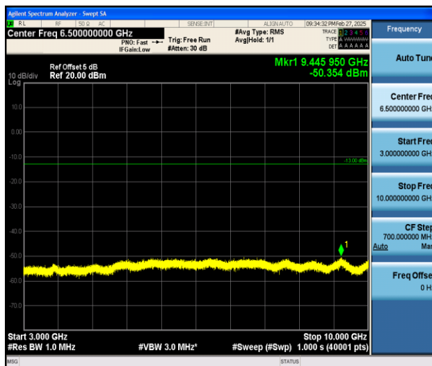
Band26_1.4MHz_16QAM_26740_1RB#0_3000~10000_3000~10000
