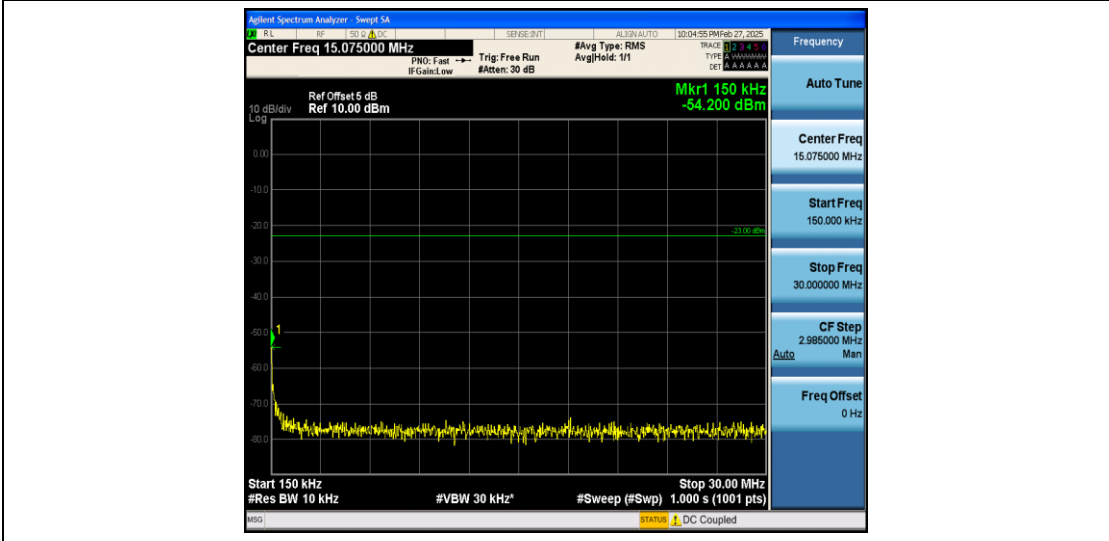
Band26_3MHz_QPSK_26740_1RB#0_0.15~30_0.15~30
