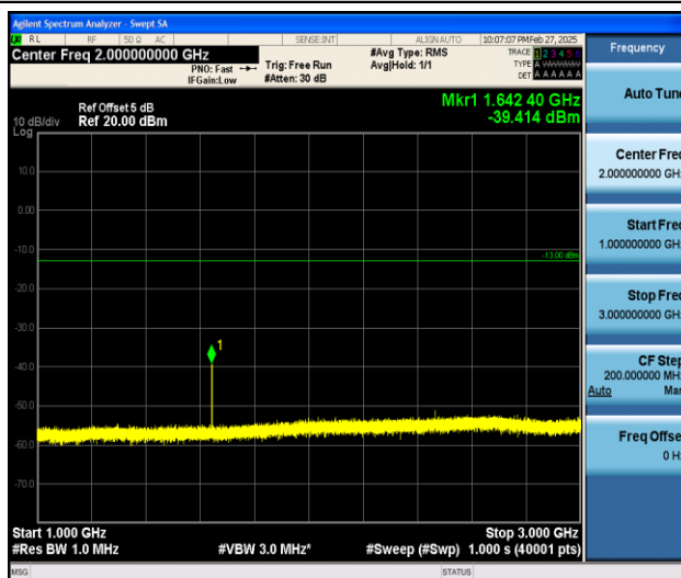
Band26_3MHz_QPSK_26775_1RB#0_1000~3000_1000~3000
