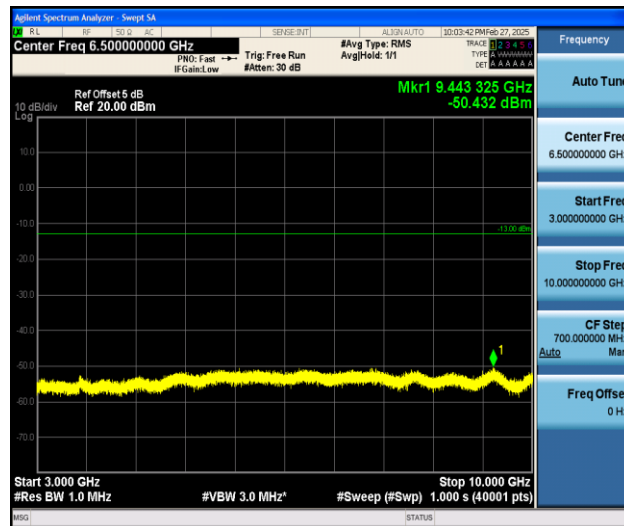
Band26_3MHz_QPSK_26705_1RB#0_3000~10000_3000~10000
