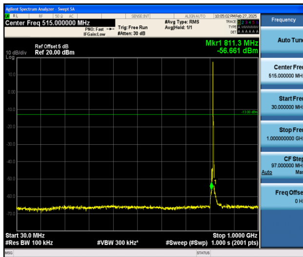
Band26_3MHz_QPSK_26740_1RB#0_30~1000_30~1000
