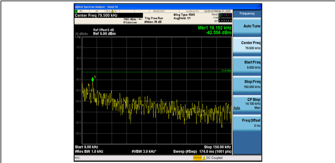
Band26_3MHz_16QAM_26740_1RB#0_0.009~0.15_0.009~0.15
