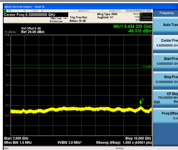
Band26_1.4MHz_16QAM_26783_1RB#0_3000~10000_3000~10000
