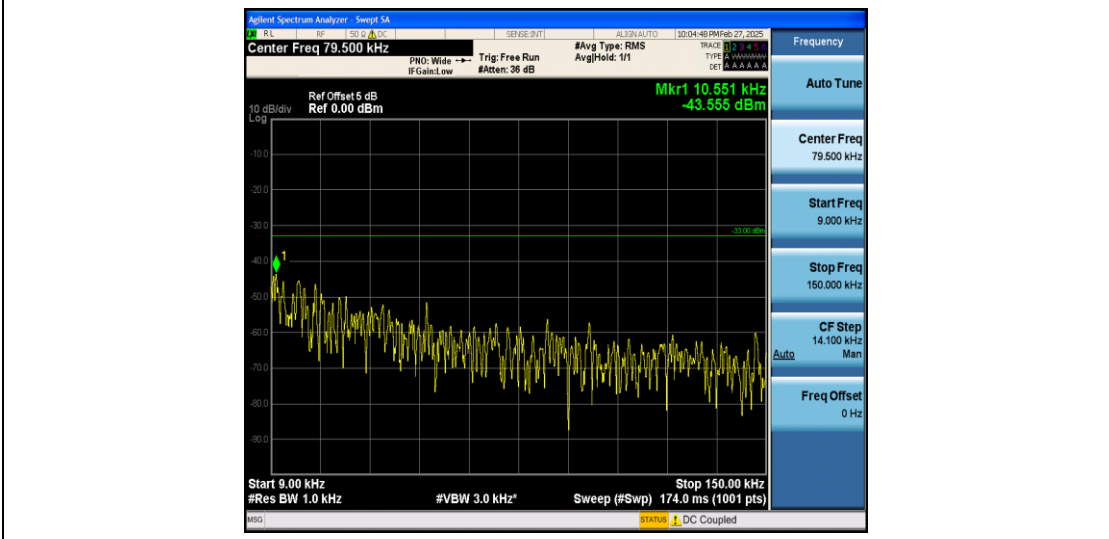
Band26_3MHz_QPSK_26740_1RB#0_0.009~0.15_0.009~0.15
