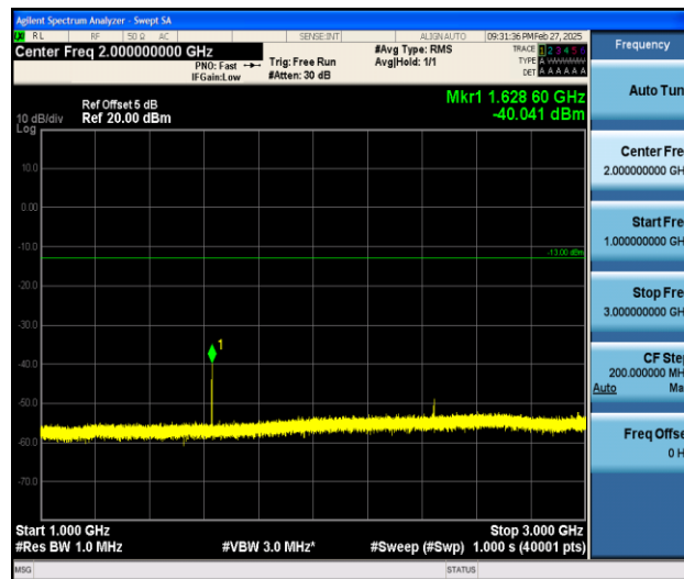
Band26_1.4MHz_QPSK_26697_1RB#0_1000~3000_1000~3000
