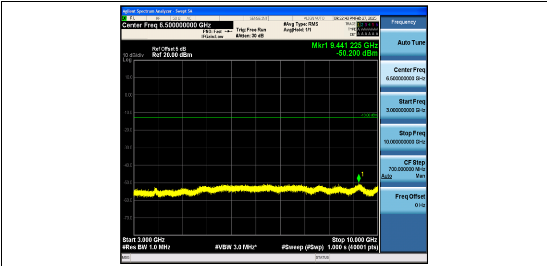
Band26_1.4MHz_16QAM_26697_1RB#0_3000~10000_3000~10000
