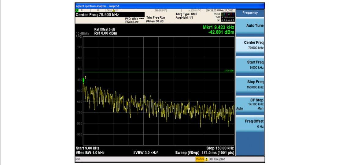
Band26_1.4MHz_QPSK_26740_1RB#0_0.009~0.15_0.009~0.15
