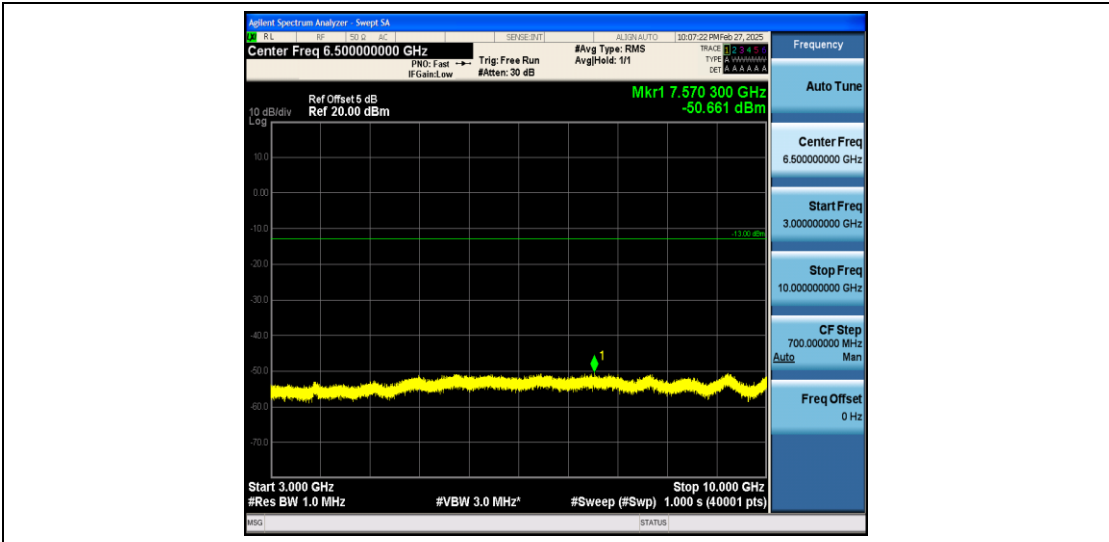
Band26_3MHz_QPSK_26775_1RB#0_3000~10000_3000~10000
