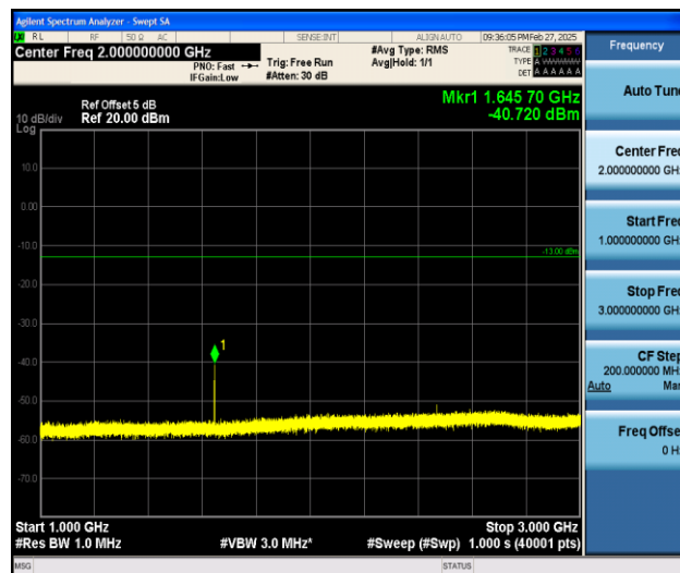
Band26_1.4MHz_16QAM_26783_1RB#0_1000~3000_1000~3000
