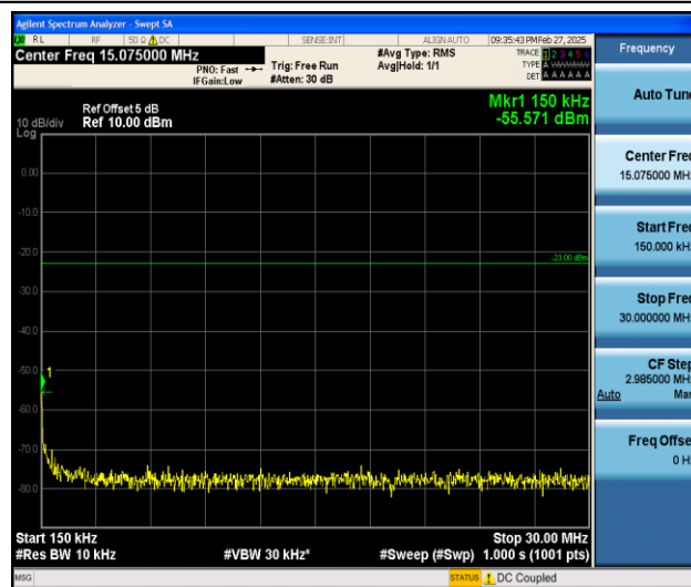
Band26_1.4MHz_16QAM_26783_1RB#0_0.15~30_0.15~30
