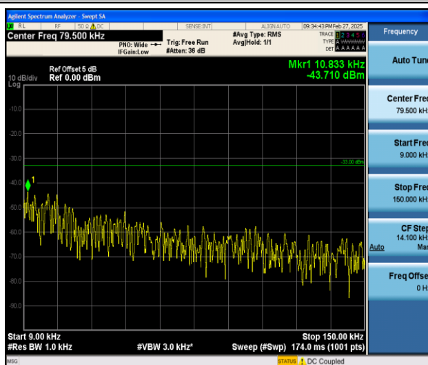
Band26_1.4MHz_QPSK_26783_1RB#0_0.009~0.15_0.009~0.15
