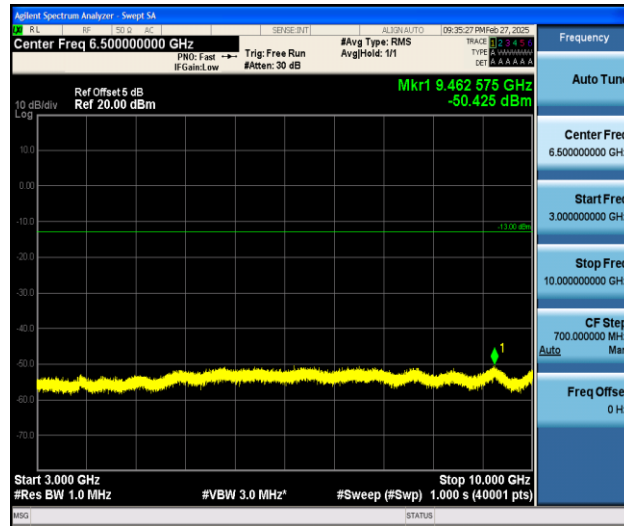
Band26_1.4MHz_QPSK_26783_1RB#0_3000~10000_3000~10000
