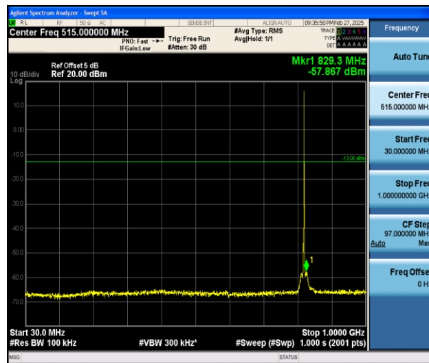
Band26_1.4MHz_16QAM_26783_1RB#0_30~1000_30~1000
