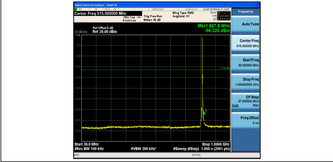
Band26_3MHz_16QAM_26740_1RB#0_30~1000_30~1000
