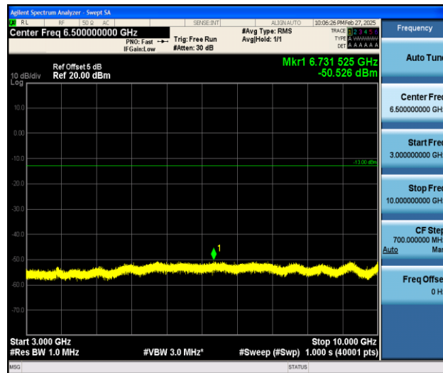
Band26_3MHz_16QAM_26740_1RB#0_3000~10000_3000~10000
