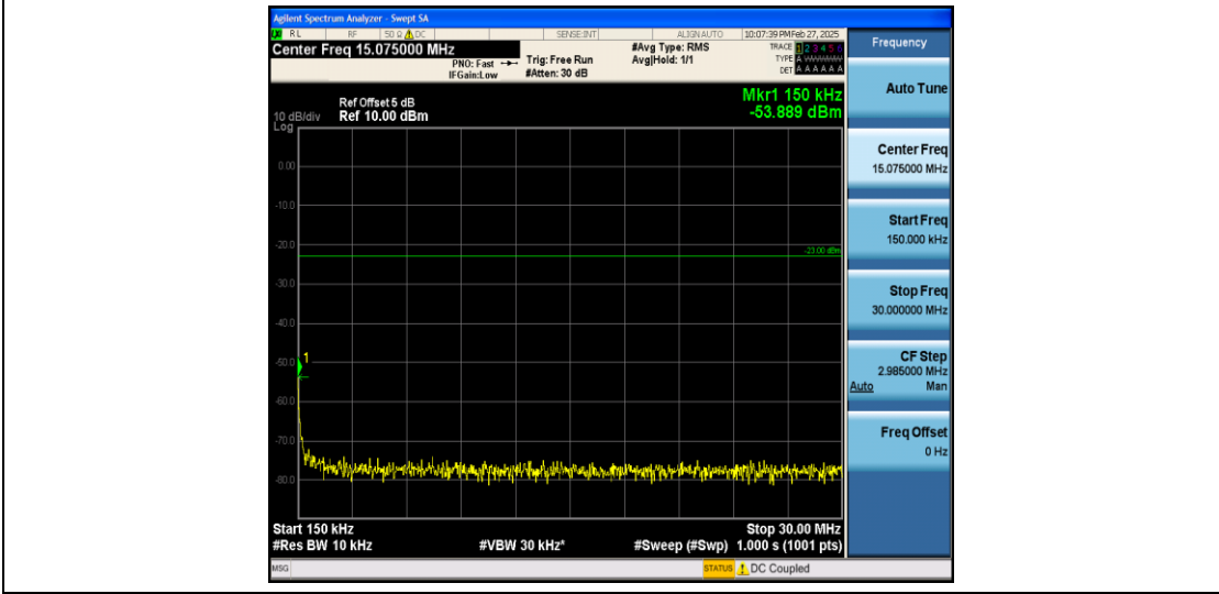
Band26_3MHz_16QAM_26775_1RB#0_0.15~30_0.15~30
