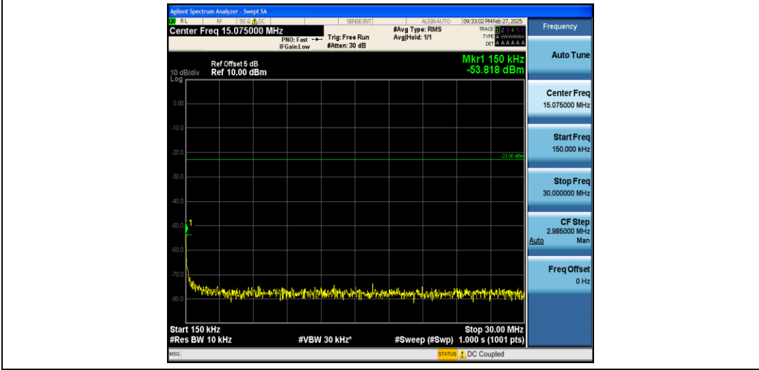
Band26_1.4MHz_QPSK_26740_1RB#0_0.15~30_0.15~30
