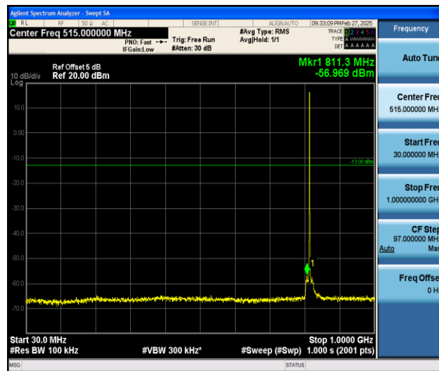
Band26_1.4MHz_QPSK_26740_1RB#0_30~1000_30~1000
