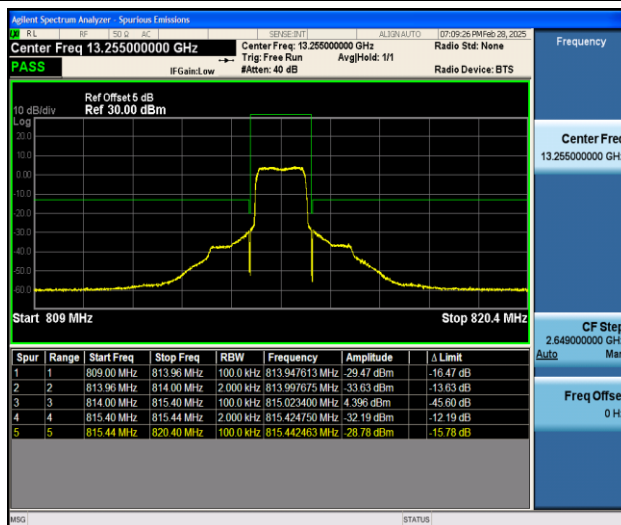
Band26_1.4MHz_QPSK_26697_6RB#0
