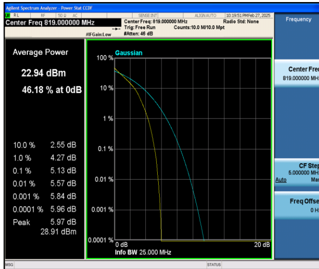
26(814-824)-3MHz-QPSK-26740-15RB#0-PASS
