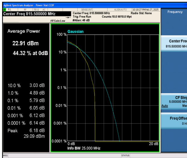
26(814-824)-3MHz-16QAM-26705-1RB#0-PASS
