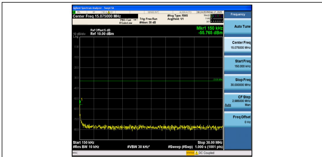
Band66_1.4MHz_16QAM_132322_1RB#0_0.15~30_0.15~30
