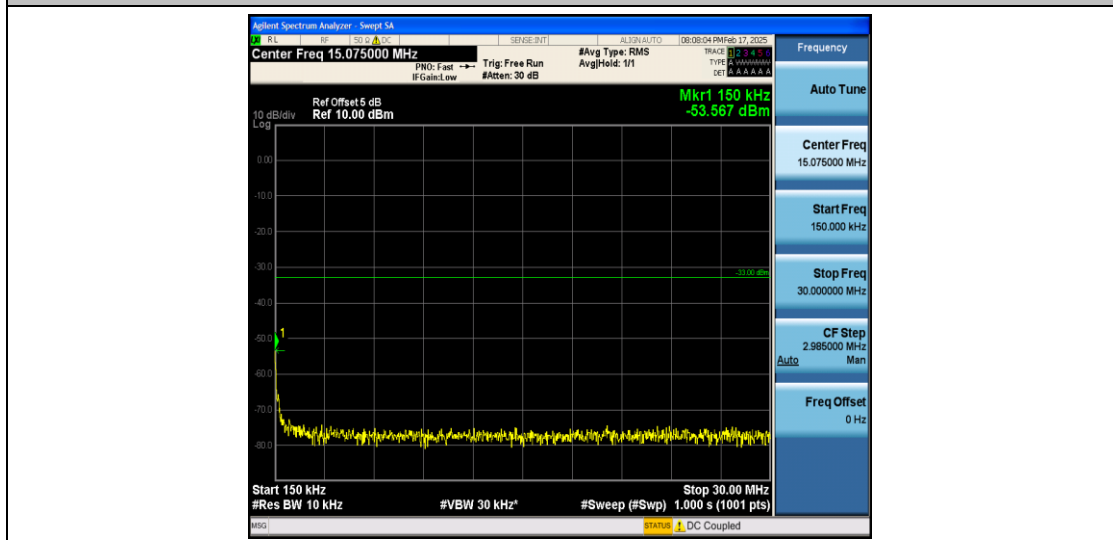
Band66_20MHz_QPSK_132572_1RB#0_0.15~30_0.15~30
