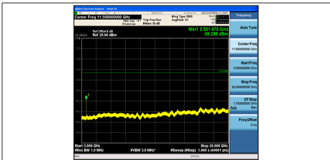
Band66_15MHz_16QAM_132597_1RB#0_3000~131022_3000~131022
