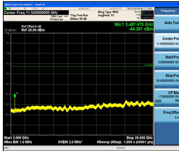
Band66_3MHz_QPSK_132322_1RB#0_3000~131022_3000~131022
