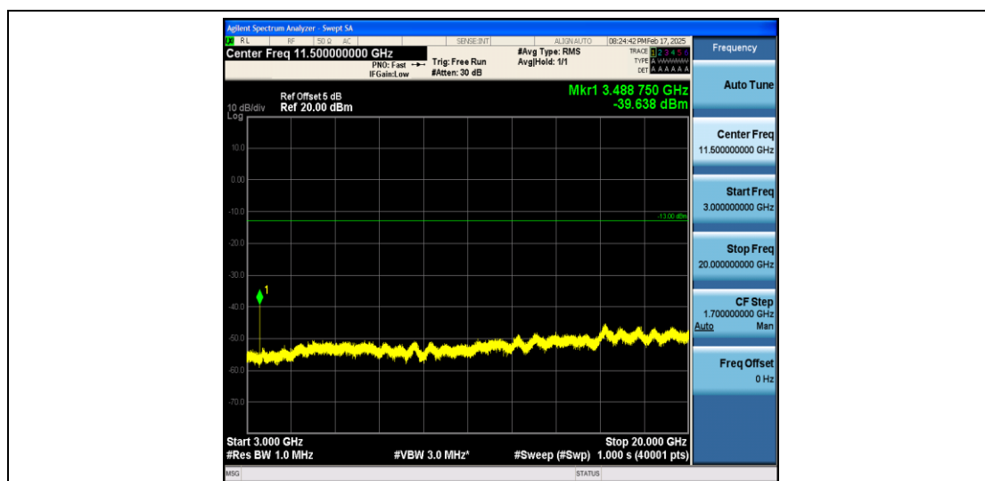
Band66_1.4MHz_16QAM_132322_1RB#0_3000~131022_3000~131022
