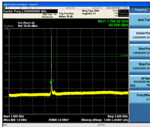
Band66_3MHz_16QAM_131987_1RB#0_1000~3000_1000~3000
