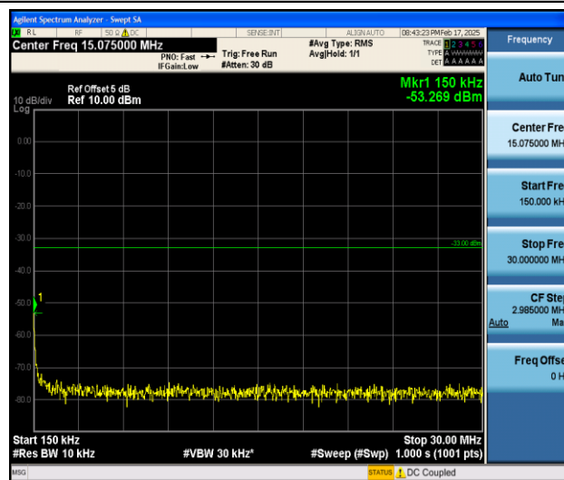
Band66_3MHz_16QAM_132322_1RB#0_0.15~30_0.15~30
