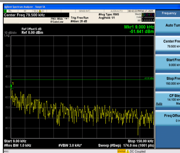
Band66_3MHz_QPSK_132322_1RB#0_0.009~0.15_0.009~0.15
