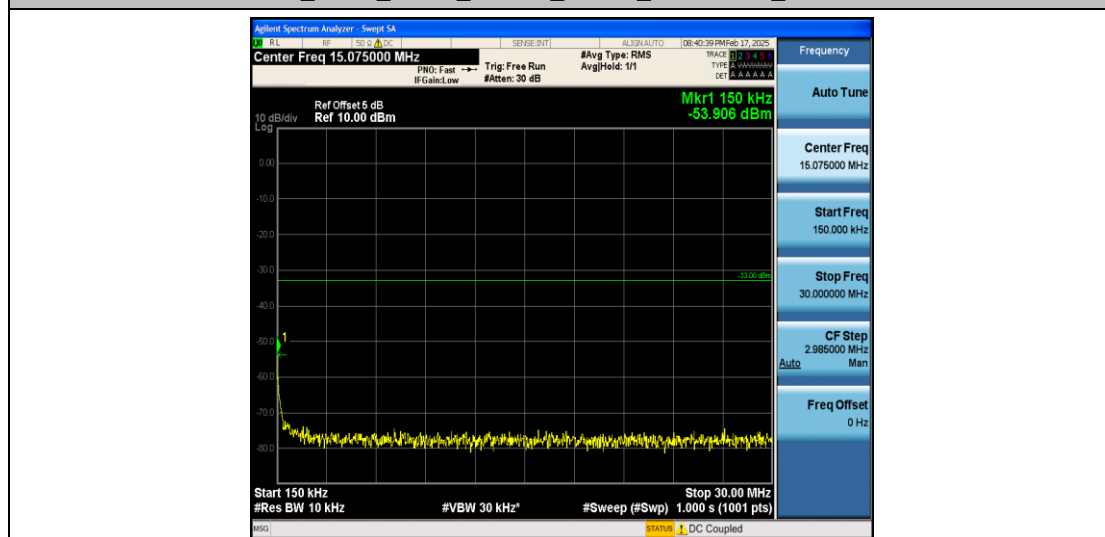
Band66_3MHz_QPSK_131987_1RB#0_0.15~30_0.15~30
