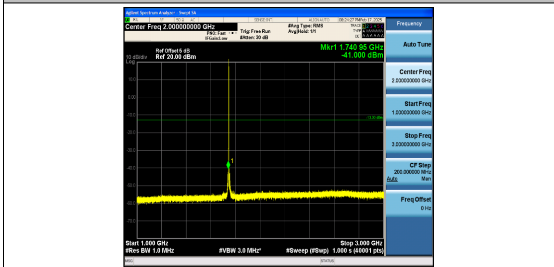
Band66_1.4MHz_16QAM_132322_1RB#0_1000~3000_1000~3000
