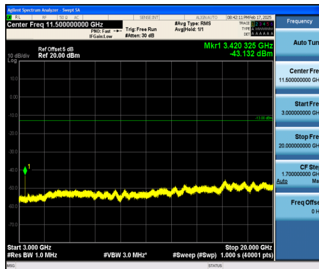
Band66_3MHz_16QAM_131987_1RB#0_3000~131022_3000~131022
