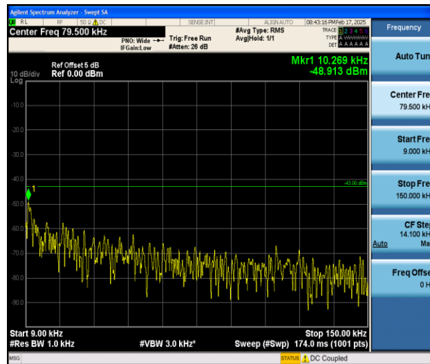
Band66_3MHz_16QAM_132322_1RB#0_0.009~0.15_0.009~0.15
