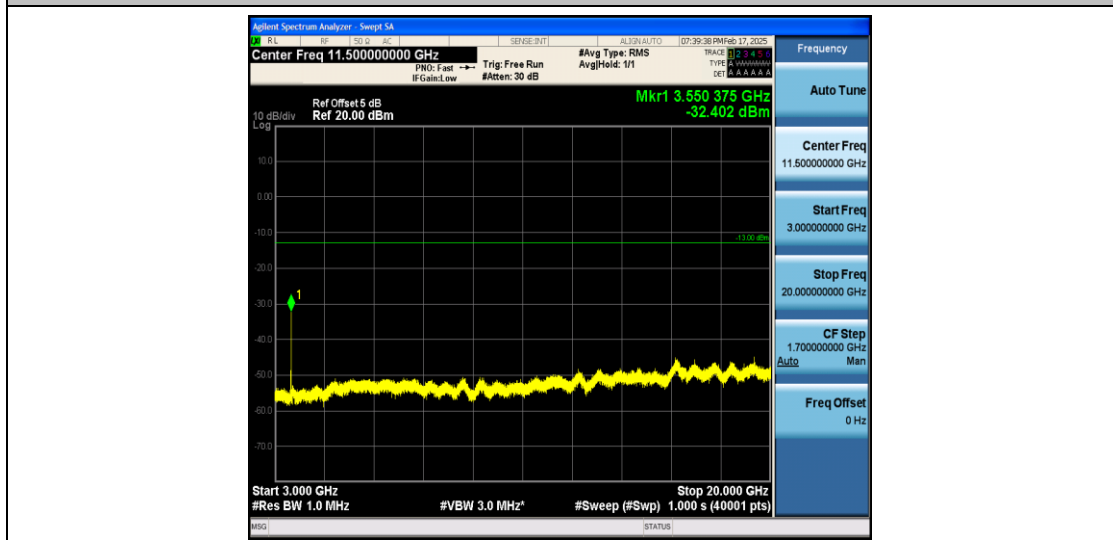
Band66_5MHz_16QAM_132647_1RB#0_3000~131022_3000~131022
