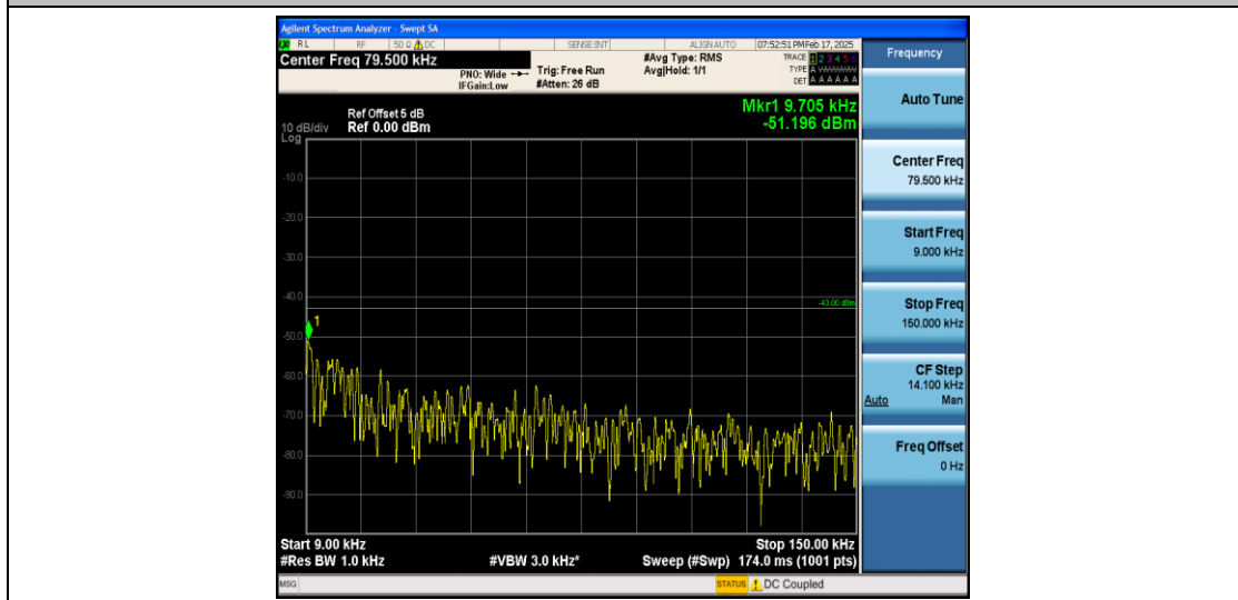
Band66_10MHz_QPSK_132622_1RB#0_0.009~0.15_0.009~0.15
