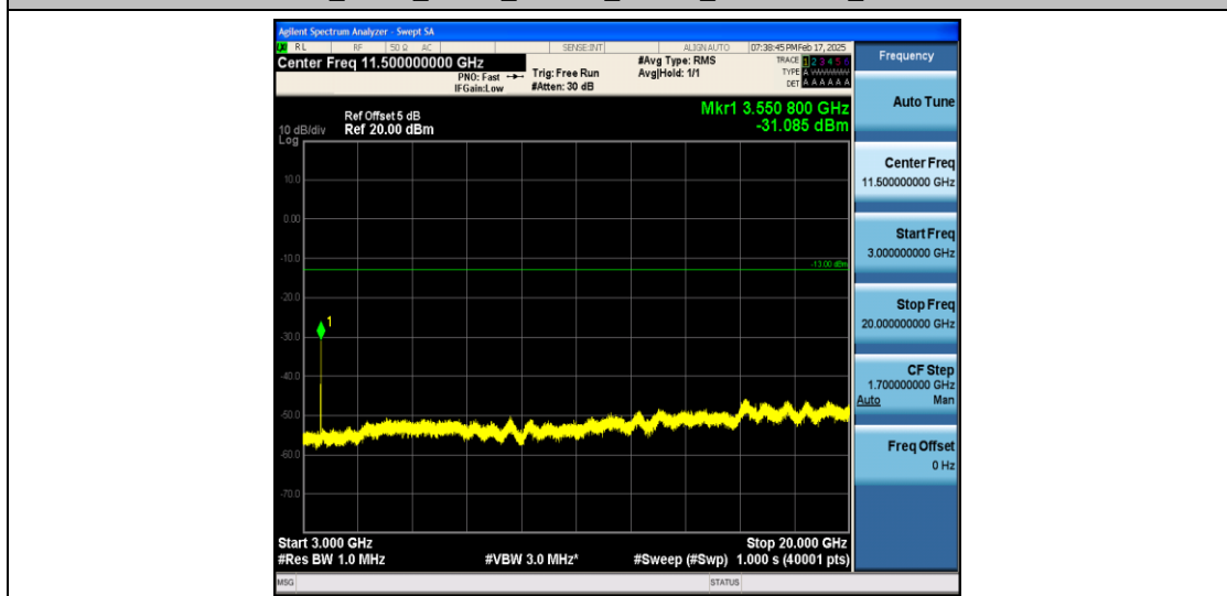
Band66_5MHz_QPSK_132647_1RB#0_3000~131022_3000~131022
