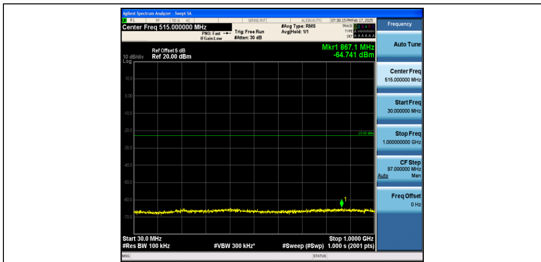
Band66_5MHz_QPSK_132647_1RB#0_30~1000_30~1000
