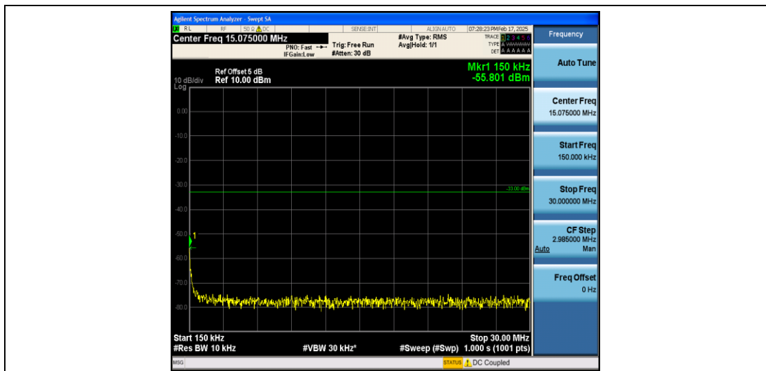
Band66_1.4MHz_QPSK_132665_1RB#0_0.15~30_0.15~30
