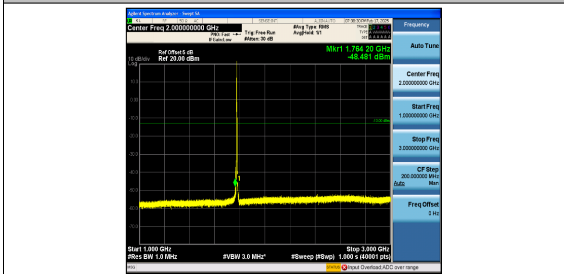
Band66_5MHz_QPSK_132647_1RB#0_1000~3000_1000~3000
