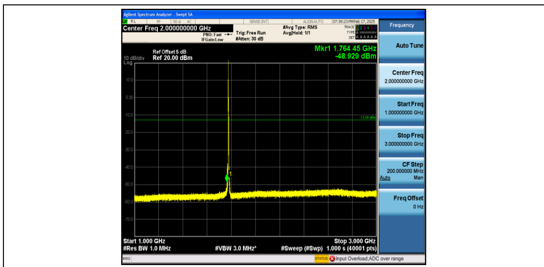
Band66_5MHz_16QAM_132647_1RB#0_1000~3000_1000~3000
