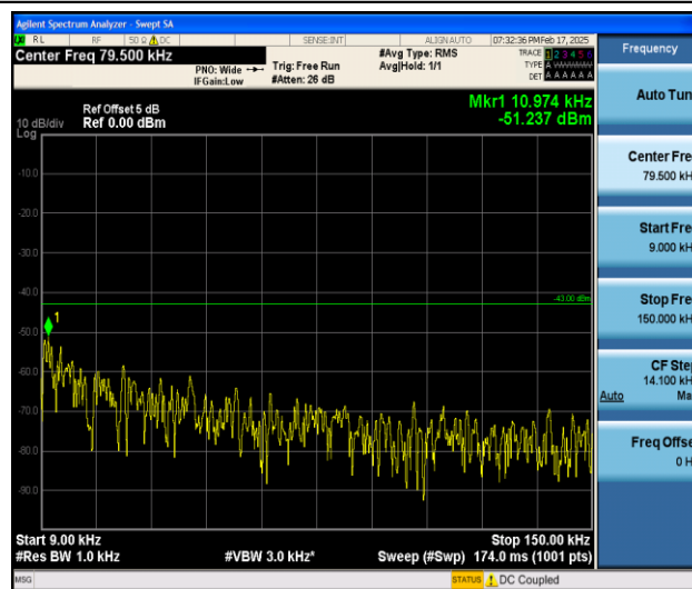
Band66_3MHz_16QAM_132657_1RB#0_0.009~0.15_0.009~0.15
