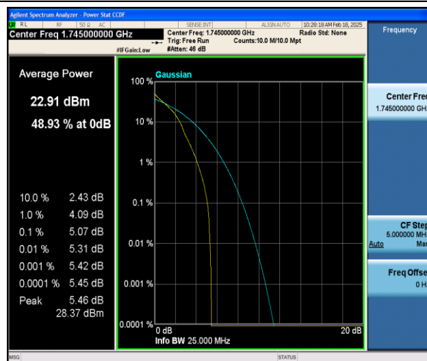
Band66-20MHz-QPSK-132322-1RB#0-PASS
