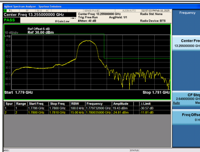
Band66_1.4MHz_QPSK_132665_1RB#5
