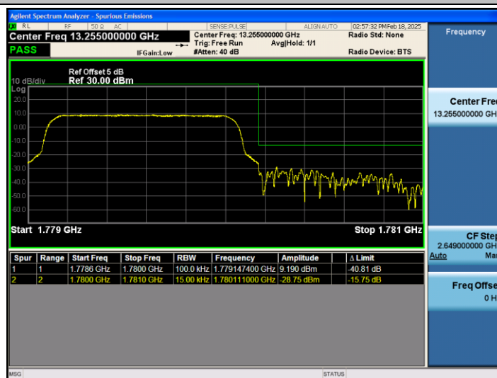
Band66_1.4MHz_16QAM_132665_6RB#0
