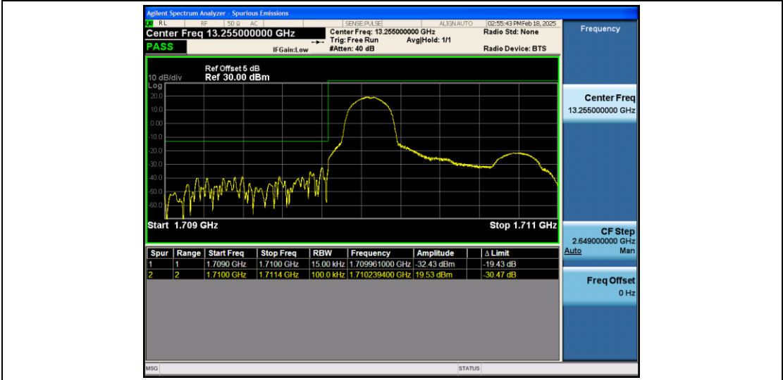
Band66_1.4MHz_QPSK_131979_1RB#0
