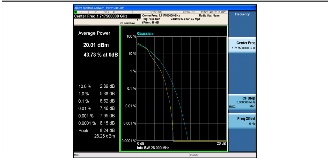
Band66-15MHz-16QAM-131047-1RB#0-PASS
