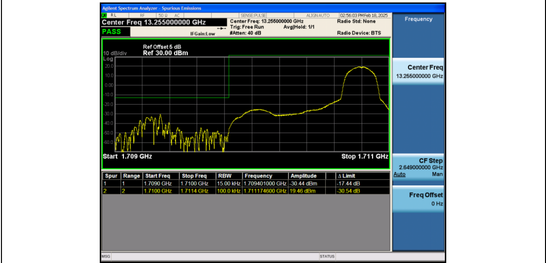
Band66_1.4MHz_QPSK_131979_1RB#5
