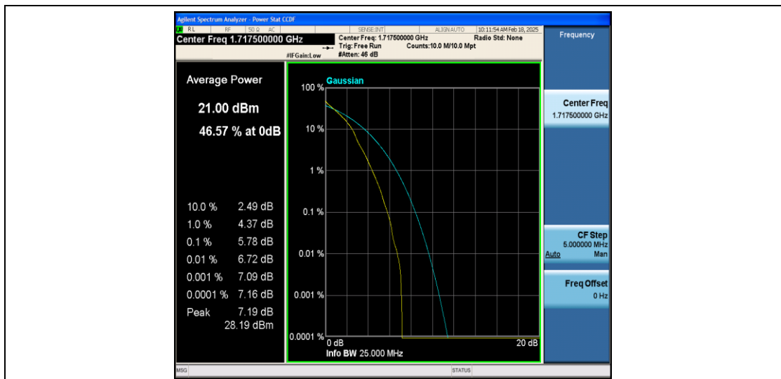
Band66-15MHz-QPSK-131047-1RB#0-PASS
