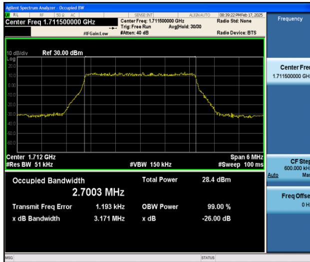
Band66-3MHz-QPSK-131987-15RB#0-PASS
