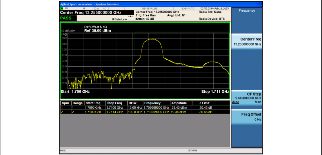
Band66_1.4MHz_16QAM_131979_1RB#0
