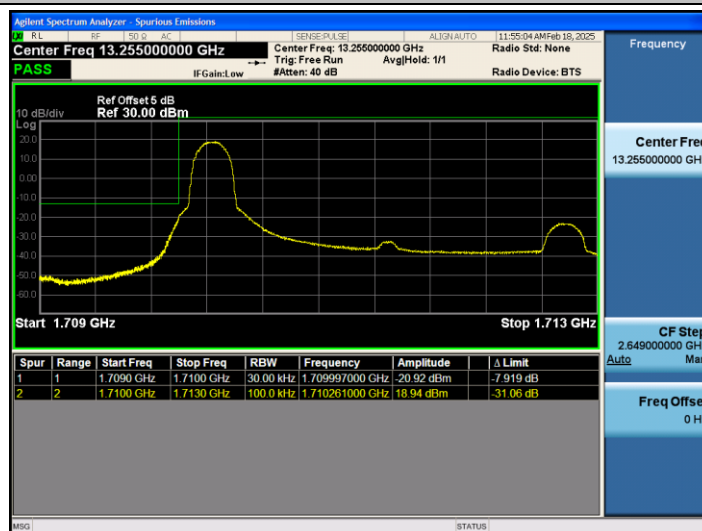
Band66_3MHz_16QAM_131987_1RB#0
