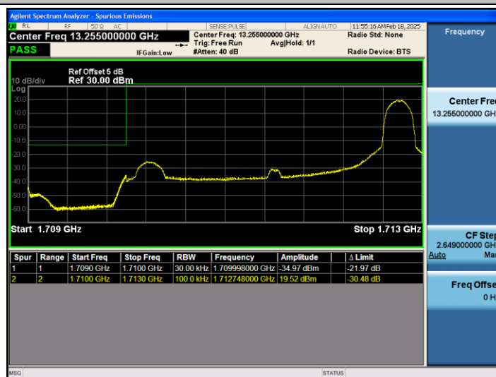
Band66_3MHz_QPSK_131987_1RB#14
