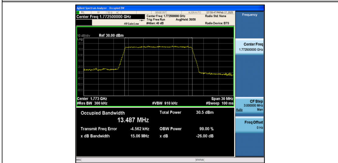
Band66-15MHz-QPSK-132597-75RB#0-PASS
