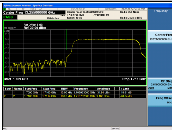
Band66_1.4MHz_16QAM_131979_6RB#0
