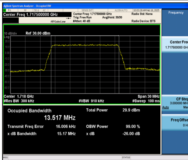
Band66-15MHz-QPSK-131047-75RB#0-PASS
