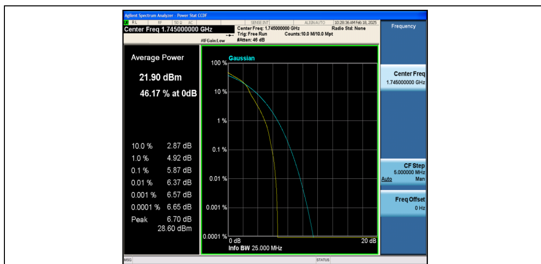
Band66-20MHz-16QAM-132322-1RB#0-PASS
