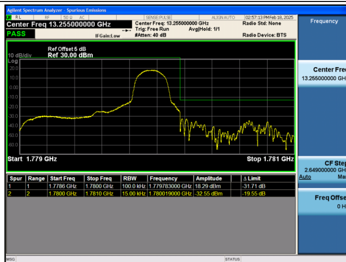
Band66_1.4MHz_16QAM_132665_1RB#5
