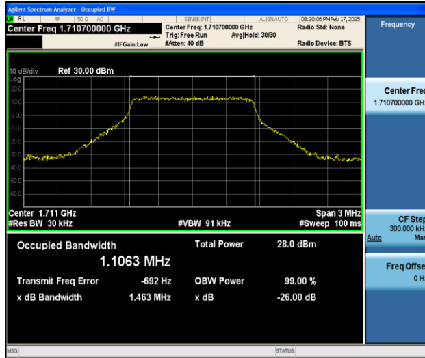
Band66-1.4MHz-QPSK-131979-6RB#0-PASS
