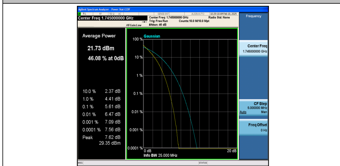
Band66-20MHz-QPSK-132322-100RB#0-PASS
