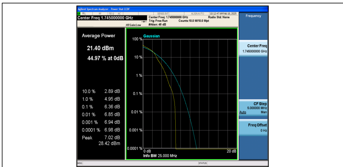
Band66-15MHz-16QAM-132322-1RB#0-PASS
