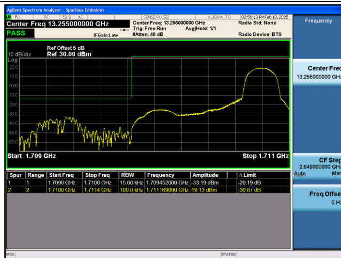
Band66_1.4MHz_16QAM_131979_1RB#5
