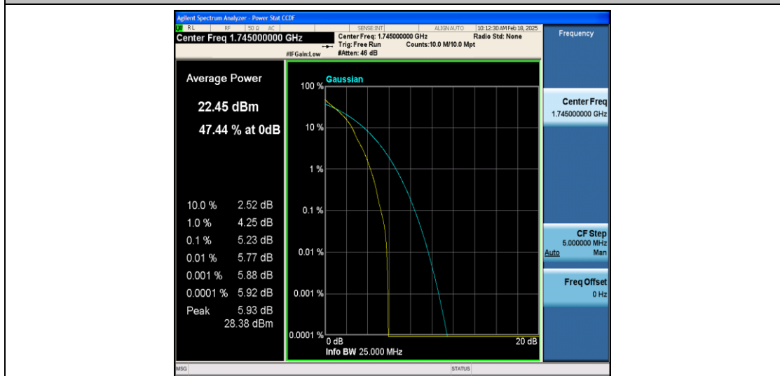
Band66-15MHz-QPSK-132322-1RB#0-PASS
