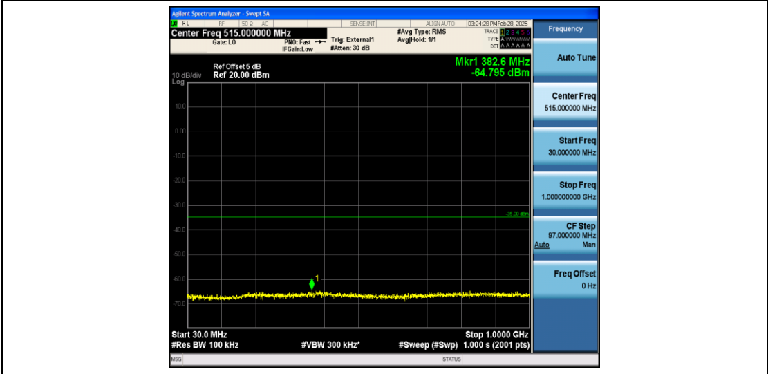
Band41_15MHz_16QAM_40620_1RB#0_30~1000_30~1000
