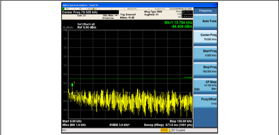
Band41_15MHz_16QAM_40620_1RB#0_0.009~0.15_0.009~0.15
