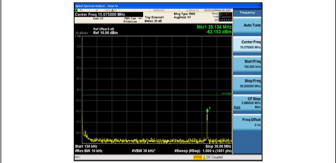
Band41_15MHz_16QAM_40620_1RB#0_0.15~30_0.15~30
