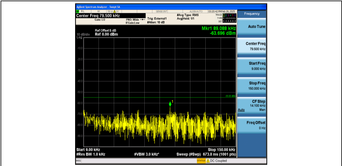
Band41_15MHz_QPSK_39725_1RB#0_0.009~0.15_0.009~0.15
