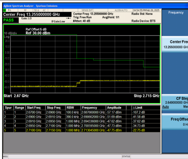
Band41_20MHz_16QAM_41490_100RB#0
