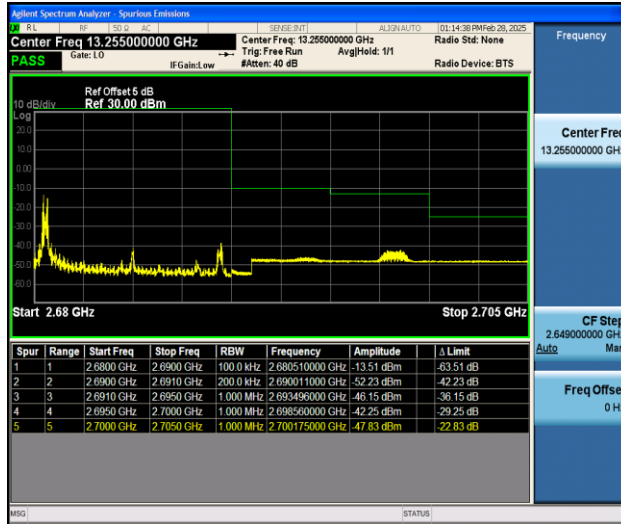
Band41_10MHz_16QAM_41540_1RB#0
