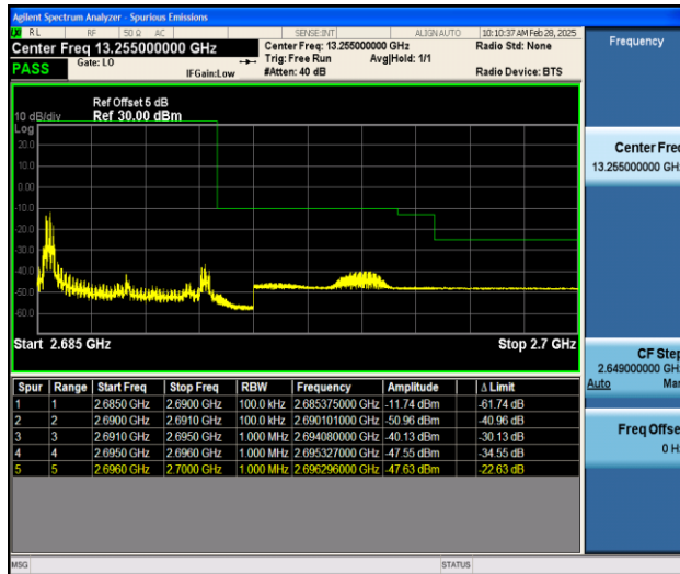
Band41_5MHz_QPSK_41565_1RB#0
