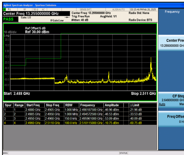
Band41_15MHz_QPSK_39725_1RB#74
