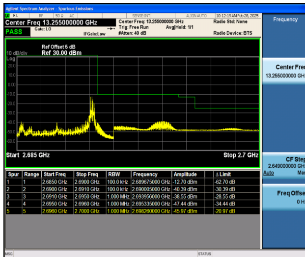
Band41_5MHz_16QAM_41565_1RB#24
