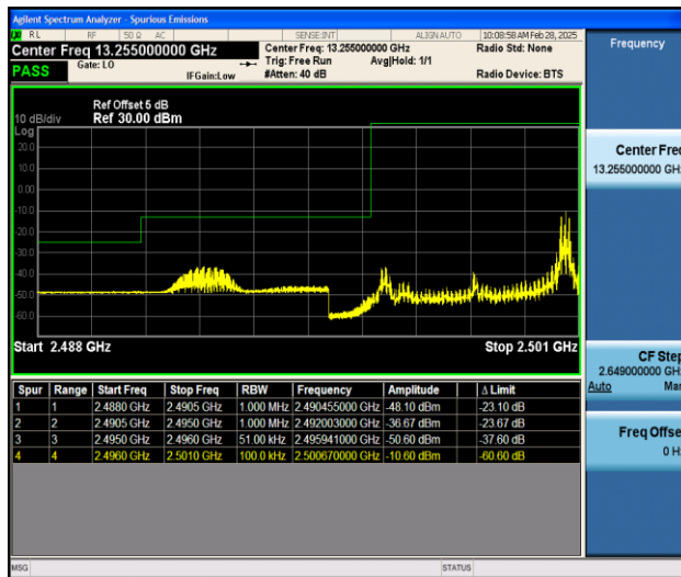
Band41_5MHz_16QAM_39675_1RB#24
