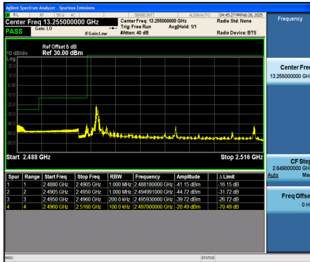
Band41_20MHz_16QAM_39750_1RB#0
