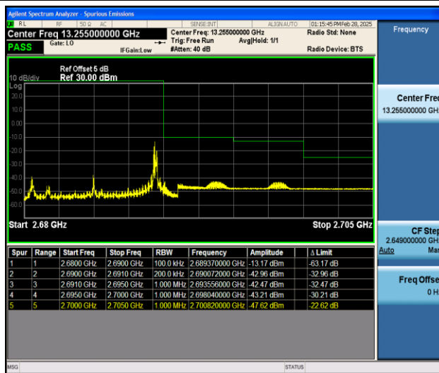
Band41_10MHz_16QAM_41540_1RB#49
