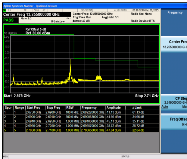
Band41_15MHz_QPSK_41515_1RB#74
