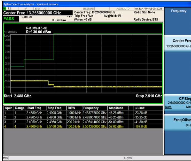
Band41_20MHz_16QAM_39750_100RB#0
