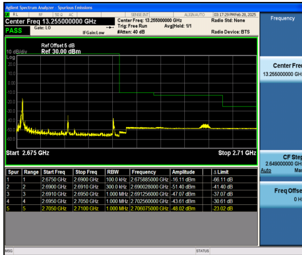
Band41_15MHz_16QAM_41515_1RB#0
