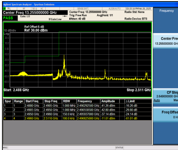
Band41_15MHz_16QAM_39725_1RB#0
