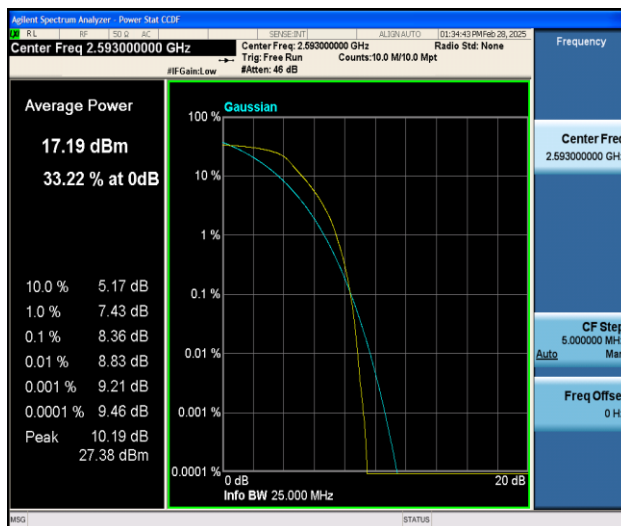
Band41-10MHz-QPSK-40620-50RB#0-PASS
