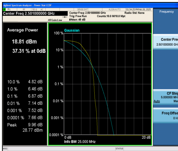
Band41-10MHz-QPSK-39700-50RB#0-PASS
