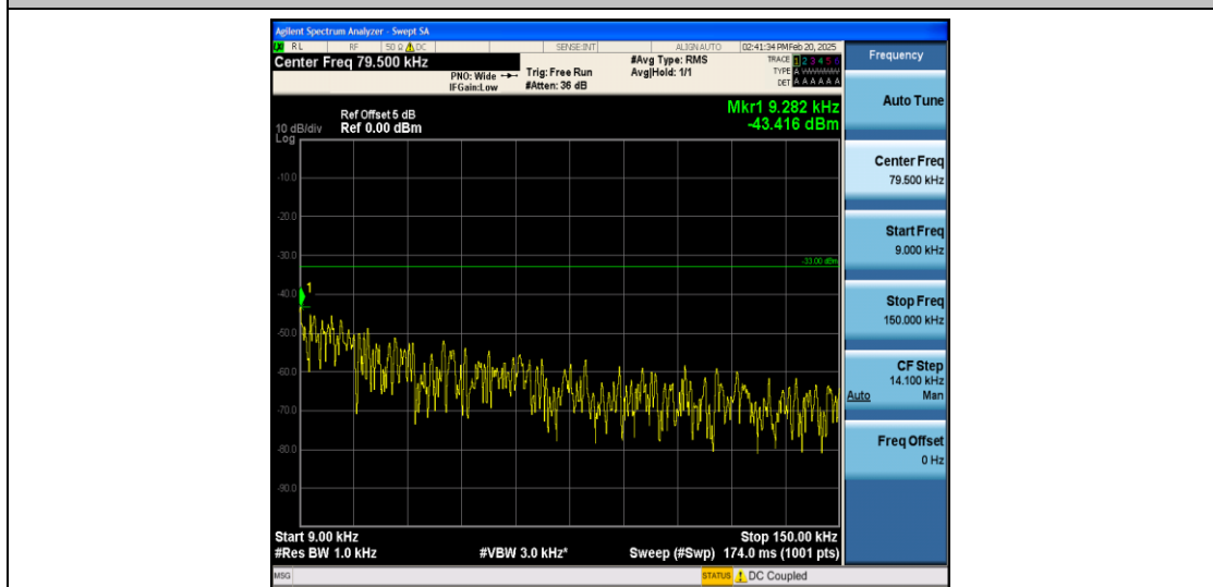
Band26_5MHz_QPSK_26915_1RB#0_0.009~0.15_0.009~0.15
