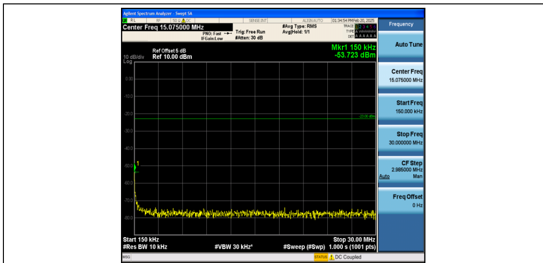
Band26_3MHz_QPSK_27025_1RB#0_0.15~30_0.15~30
