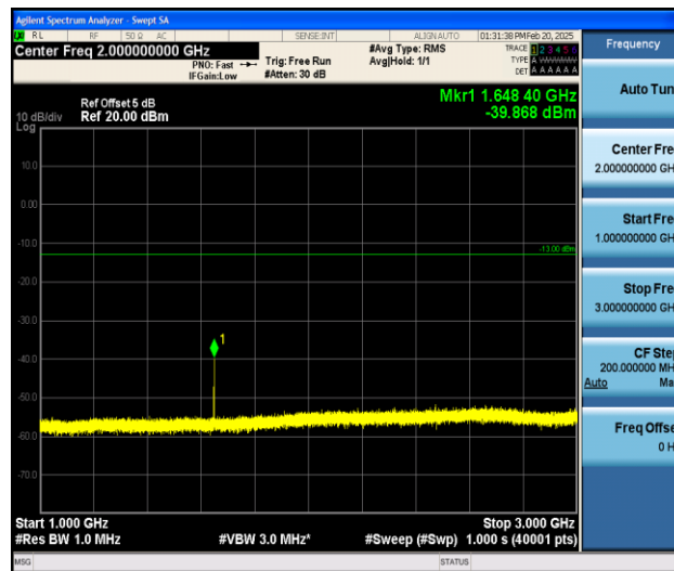
Band26_3MHz_QPSK_26805_1RB#0_1000~3000_1000~3000
