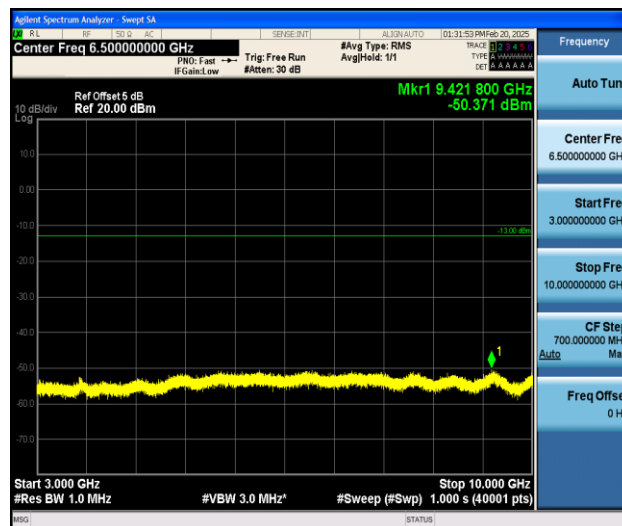
Band26_3MHz_QPSK_26805_1RB#0_3000~10000_3000~10000
