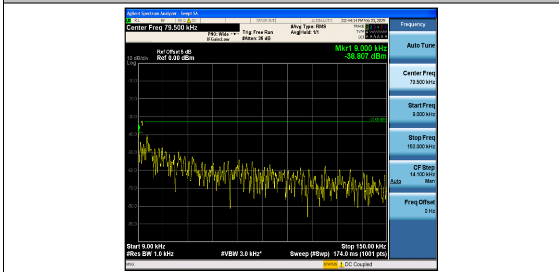
Band26_5MHz_16QAM_27015_1RB#0_0.009~0.15_0.009~0.15
