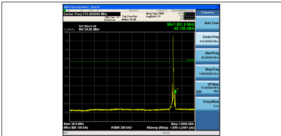
Band26_5MHz_QPSK_26915_1RB#0_30~1000_30~1000
