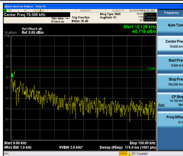
Band26_3MHz_QPSK_27025_1RB#0_0.009~0.15_0.009~0.15
