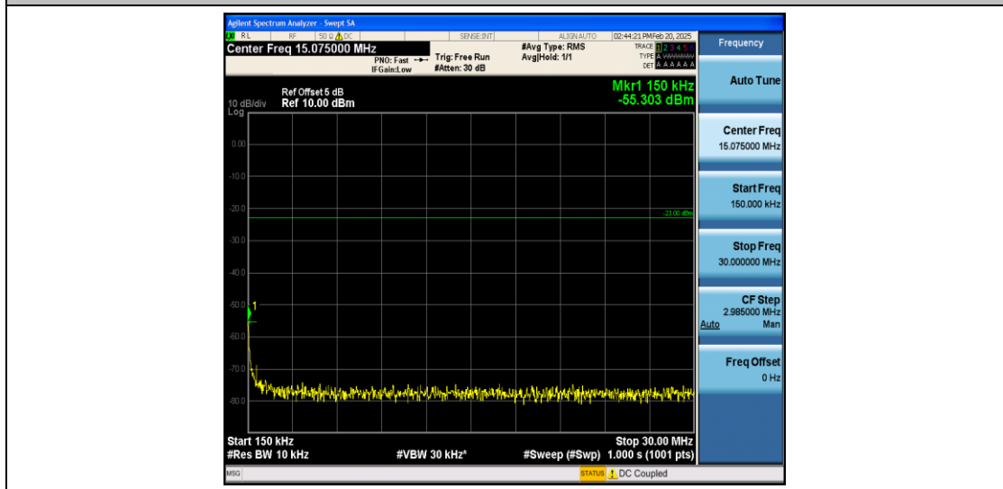
Band26_5MHz_16QAM_27015_1RB#0_0.15~30_0.15~30
