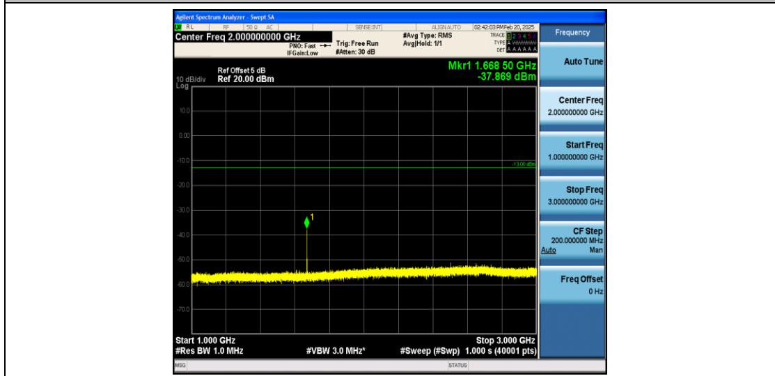
Band26_5MHz_QPSK_26915_1RB#0_1000~3000_1000~3000
