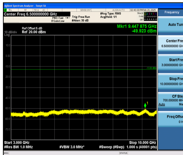
Band26_5MHz_QPSK_26815_1RB#0_3000~10000_3000~10000
