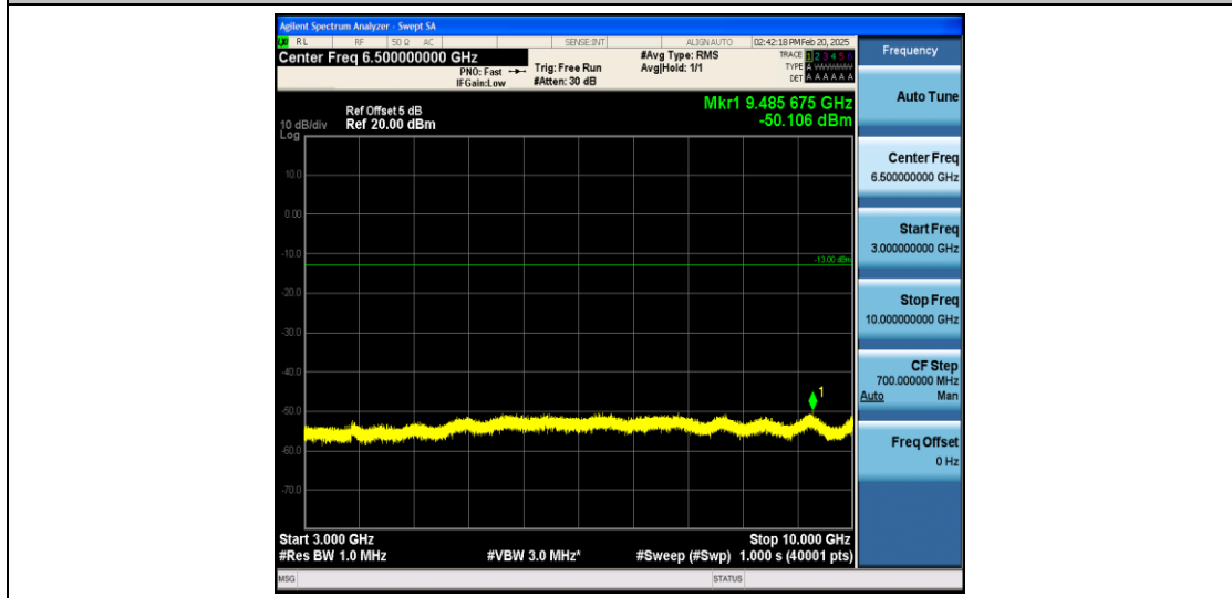
Band26_5MHz_QPSK_26915_1RB#0_3000~10000_3000~10000
