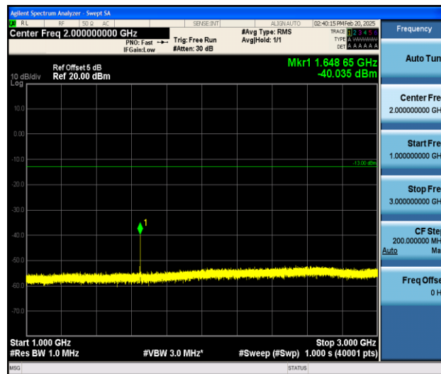
Band26_5MHz_QPSK_26815_1RB#0_1000~3000_1000~3000
