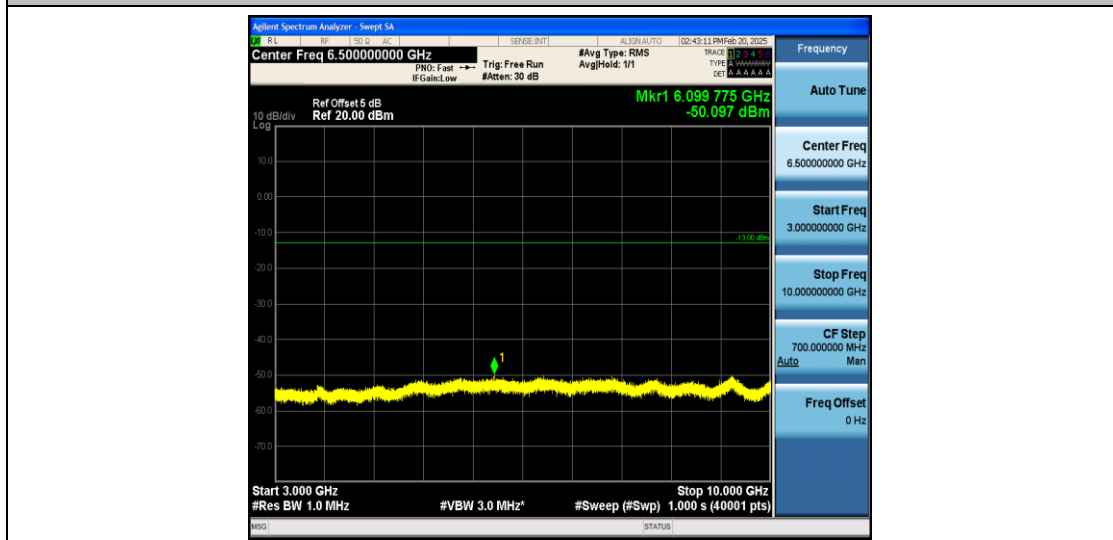
Band26_5MHz_16QAM_26915_1RB#0_3000~10000_3000~10000
