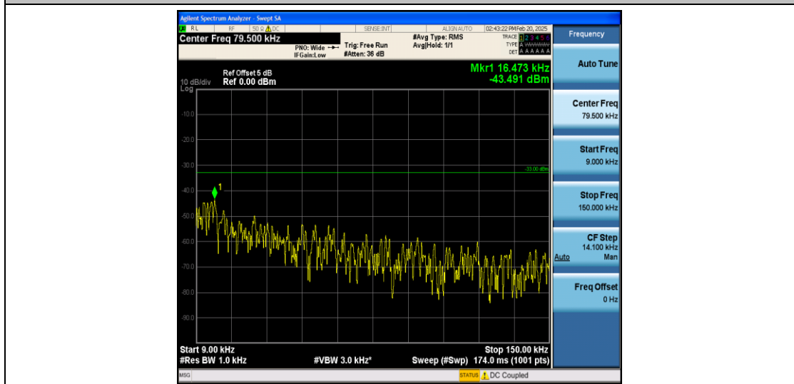
Band26_5MHz_QPSK_27015_1RB#0_0.009~0.15_0.009~0.15
