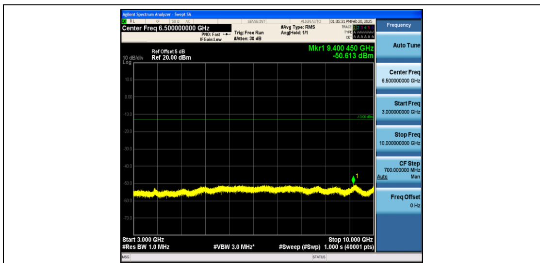
Band26_3MHz_QPSK_27025_1RB#0_3000~10000_3000~10000
