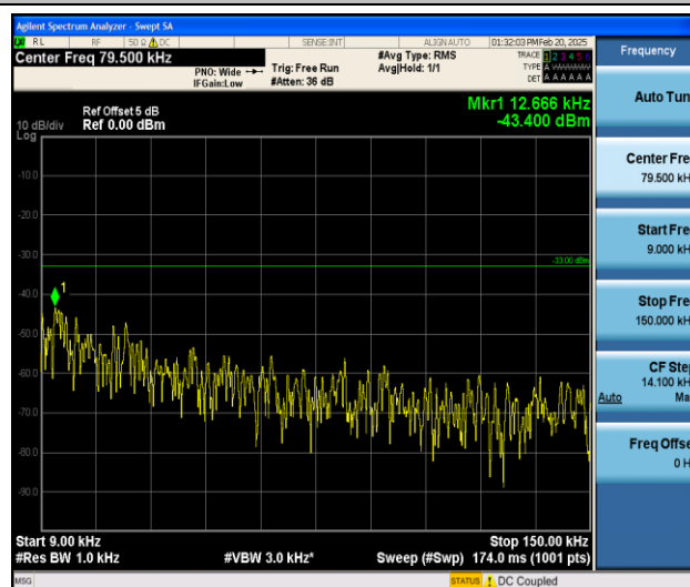
Band26_3MHz_16QAM_26805_1RB#0_0.009~0.15_0.009~0.15
