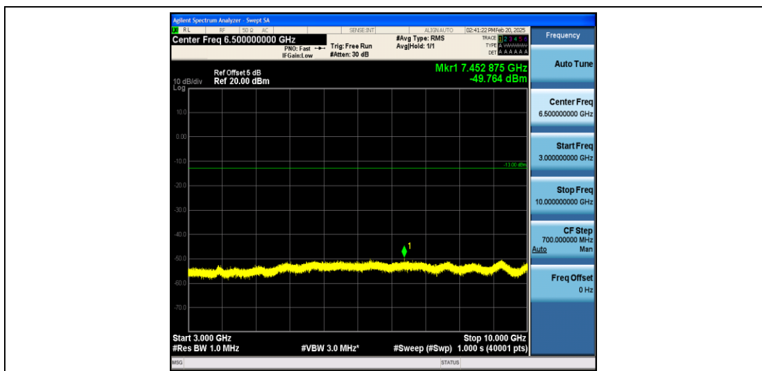
Band26_5MHz_16QAM_26815_1RB#0_3000~10000_3000~10000
