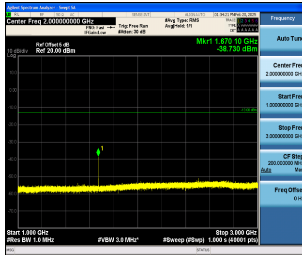
Band26_3MHz_16QAM_26915_1RB#0_1000~3000_1000~3000
