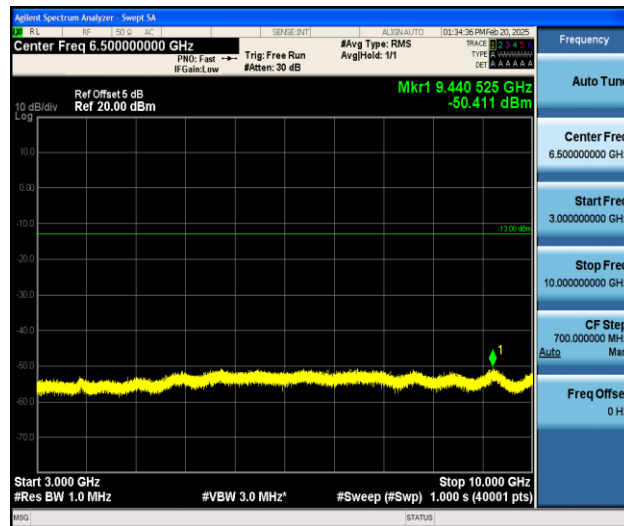
Band26_3MHz_16QAM_26915_1RB#0_3000~10000_3000~10000
