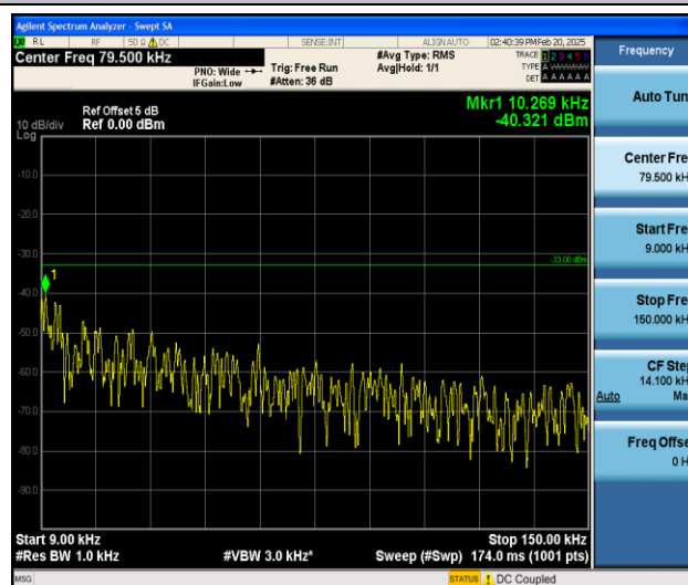
Band26_5MHz_16QAM_26815_1RB#0_0.009~0.15_0.009~0.15
