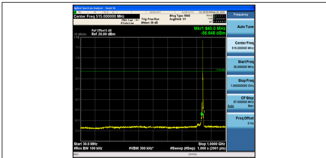
Band26_3MHz_16QAM_27025_1RB#0_30~1000_30~1000
