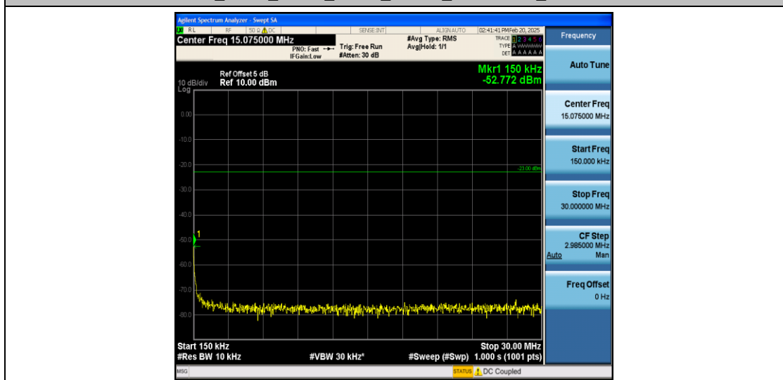
Band26_5MHz_QPSK_26915_1RB#0_0.15~30_0.15~30
