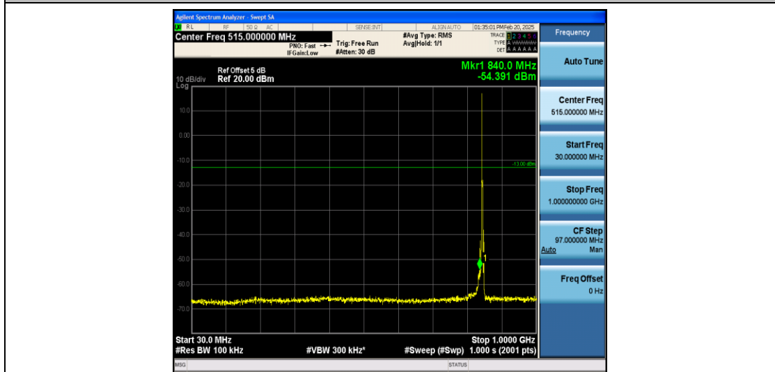
Band26_3MHz_QPSK_27025_1RB#0_30~1000_30~1000
