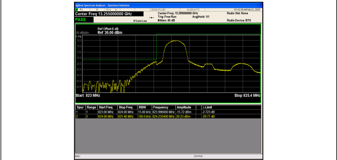
Band26_1.4MHz_QPSK_26797_1RB#0
