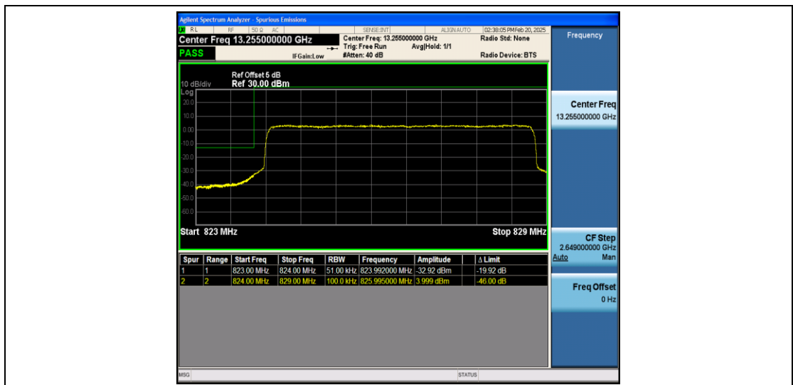
Band26_5MHz_QPSK_26815_25RB#0
