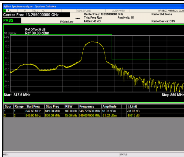
Band26_1.4MHz_16QAM_27033_1RB#5
