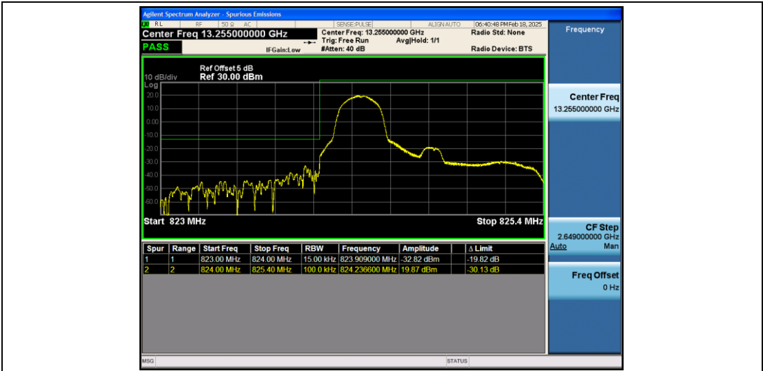
Band26_1.4MHz_QPSK_26797_1RB#0_Final1
