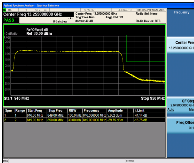
Band26_3MHz_16QAM_27025_15RB#0
