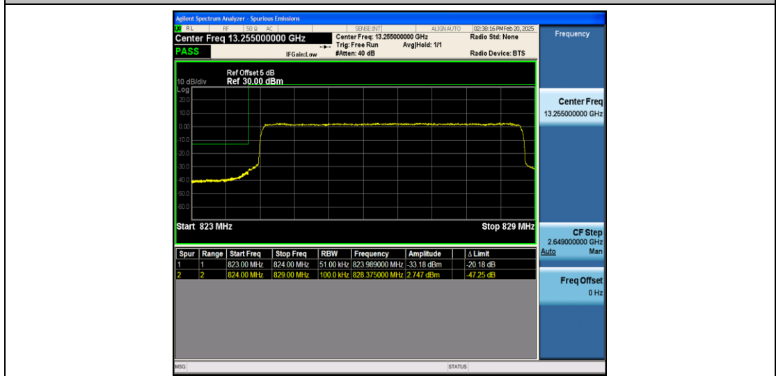
Band26_5MHz_16QAM_26815_25RB#0
