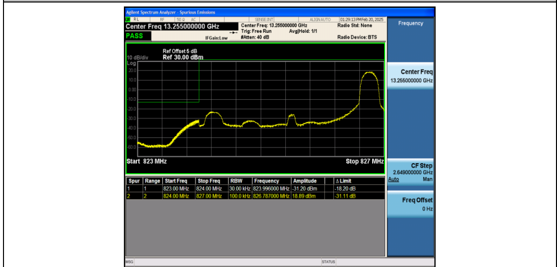
Band26_3MHz_16QAM_26805_1RB#14
