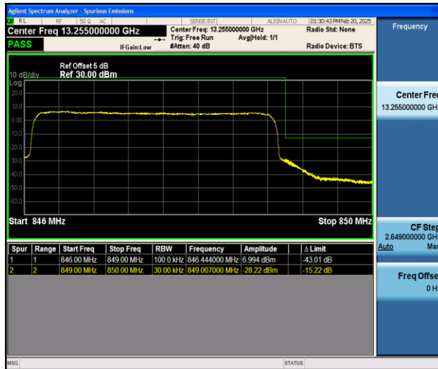
Band26_3MHz_QPSK_27025_15RB#0
