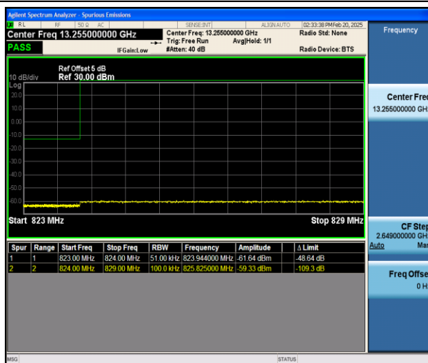
Band26_5MHz_QPSK_26815_1RB#0
