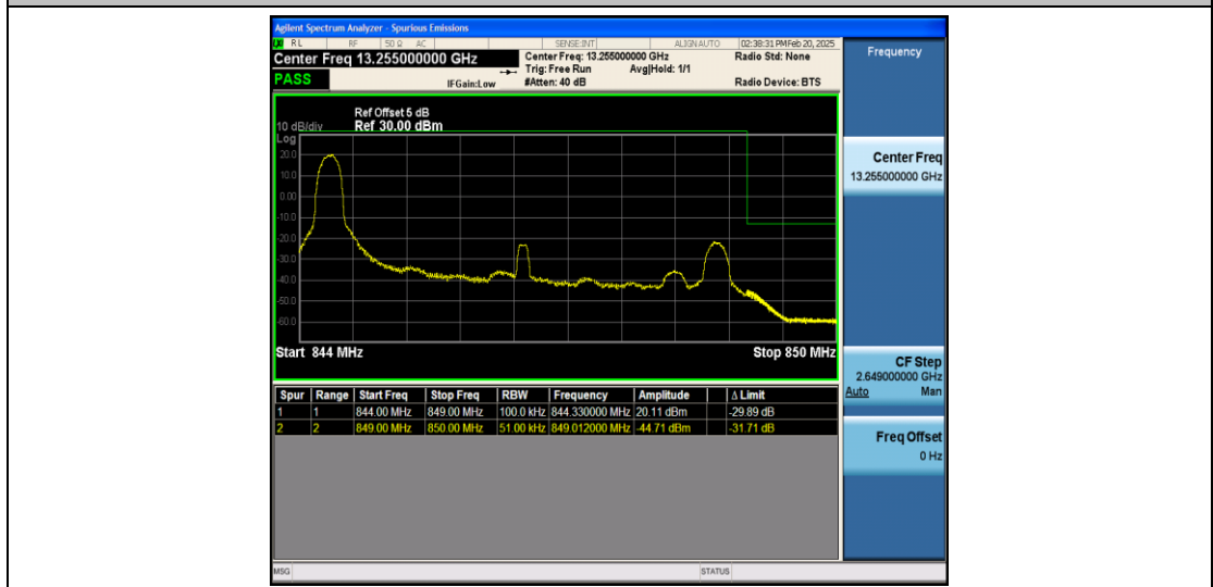
Band26_5MHz_QPSK_27015_1RB#0
