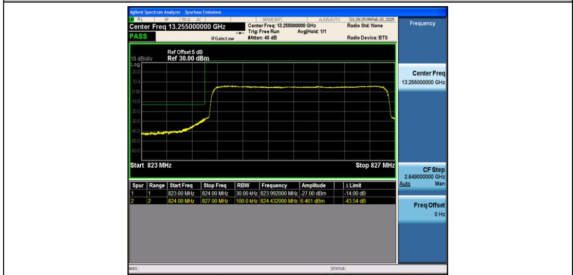
Band26_3MHz_QPSK_26805_15RB#0
