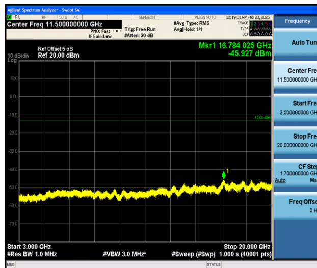
Band25_10MHz_16QAM_26640_1RB#0_3000~20000_3000~20000
