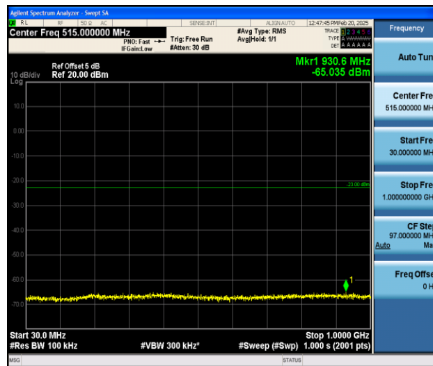
Band25_20MHz_16QAM_26140_1RB#0_30~1000_30~1000
