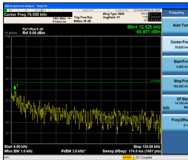
Band25_15MHz_QPSK_26615_1RB#0_0.009~0.15_0.009~0.15
