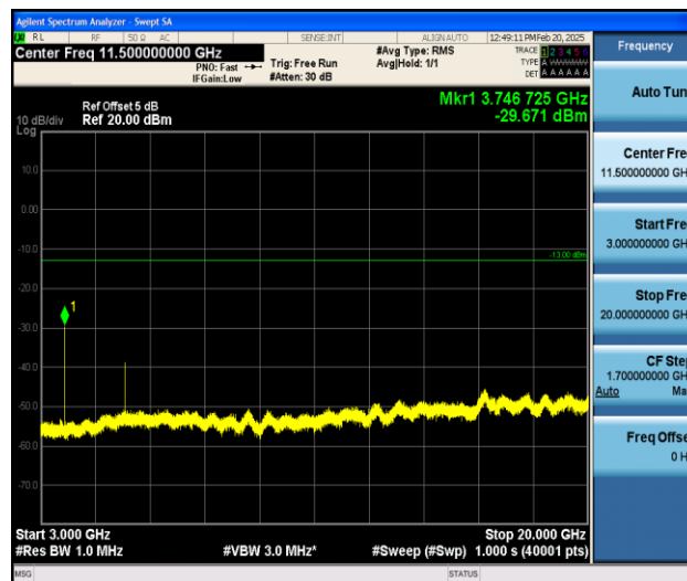
Band25_20MHz_QPSK_26365_1RB#0_3000~20000_3000~20000
