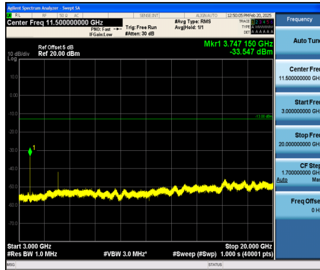
Band25_20MHz_16QAM_26365_1RB#0_3000~20000_3000~20000
