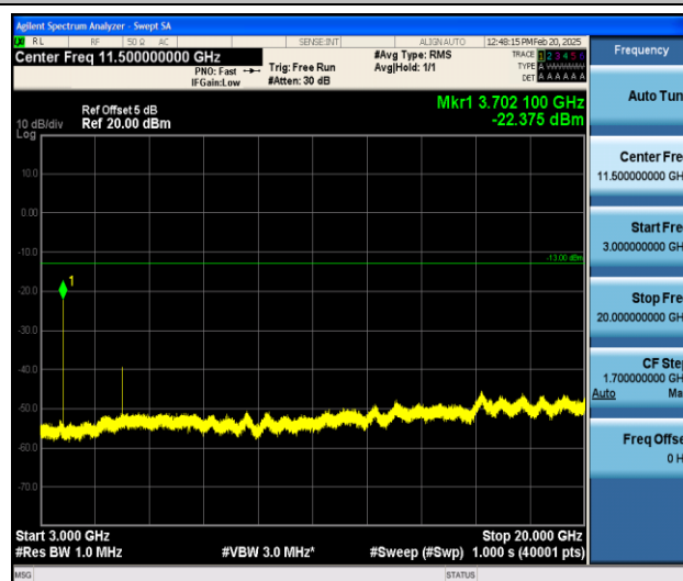
Band25_20MHz_16QAM_26140_1RB#0_3000~20000_3000~20000
