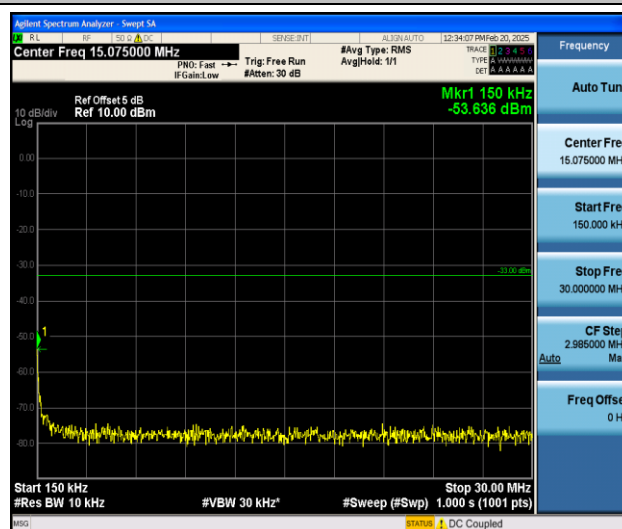
Band25_15MHz_QPSK_26615_1RB#0_0.15~30_0.15~30
