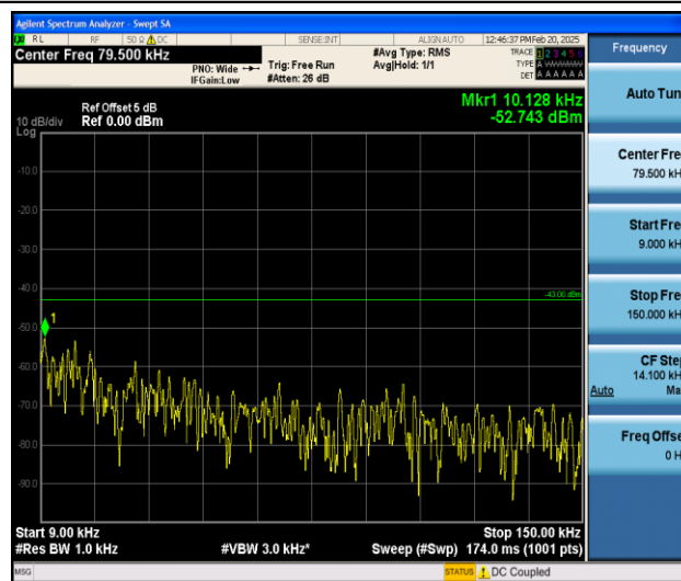
Band25_20MHz_QPSK_26140_1RB#0_0.009~0.15_0.009~0.15
