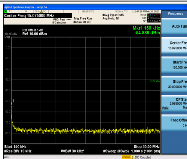
Band25_20MHz_16QAM_26140_1RB#0_0.15~30_0.15~30
