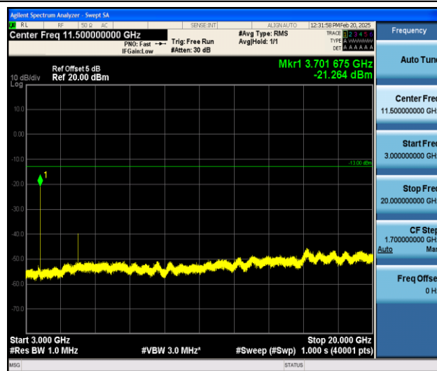
Band25_15MHz_16QAM_26115_1RB#0_3000~20000_3000~20000
