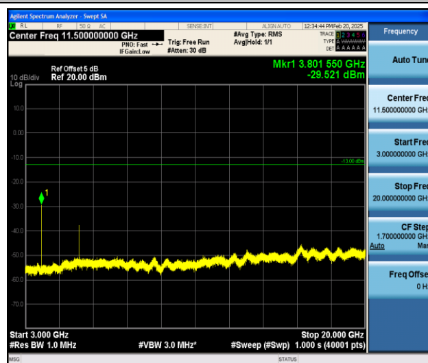
Band25_15MHz_QPSK_26615_1RB#0_3000~20000_3000~20000
