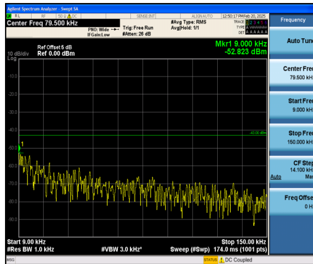
Band25_20MHz_QPSK_26590_1RB#0_0.009~0.15_0.009~0.15
