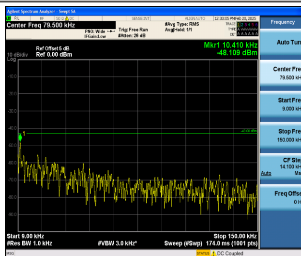
Band25_15MHz_16QAM_26365_1RB#0_0.009~0.15_0.009~0.15
