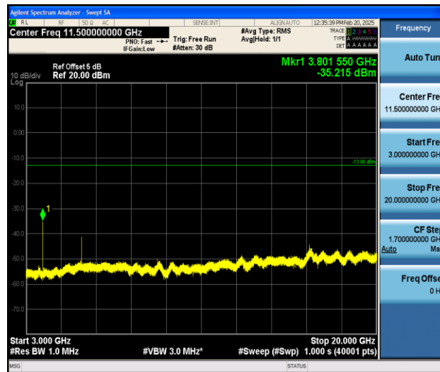
Band25_15MHz_16QAM_26615_1RB#0_3000~20000_3000~20000
