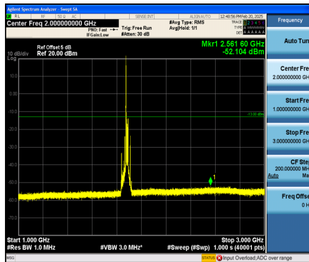
Band25_20MHz_QPSK_26365_1RB#0_1000~3000_1000~3000
