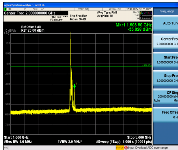
Band25_15MHz_16QAM_26115_1RB#0_1000~3000_1000~3000
