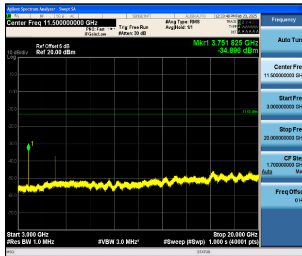
Band25_15MHz_16QAM_26365_1RB#0_3000~20000_3000~20000
