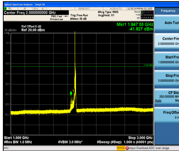
Band25_15MHz_16QAM_26615_1RB#0_1000~3000_1000~3000
