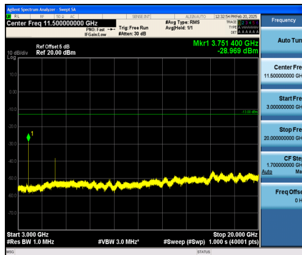
Band25_15MHz_QPSK_26365_1RB#0_3000~20000_3000~20000
