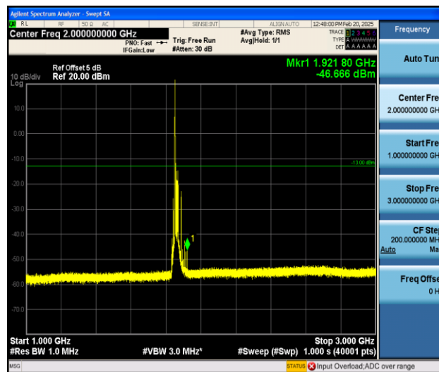
Band25_20MHz_16QAM_26140_1RB#0_1000~3000_1000~3000
