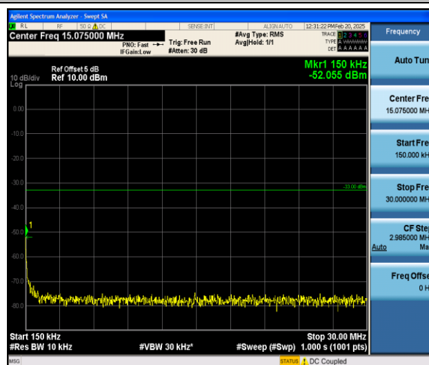
Band25_15MHz_16QAM_26115_1RB#0_0.15~30_0.15~30
