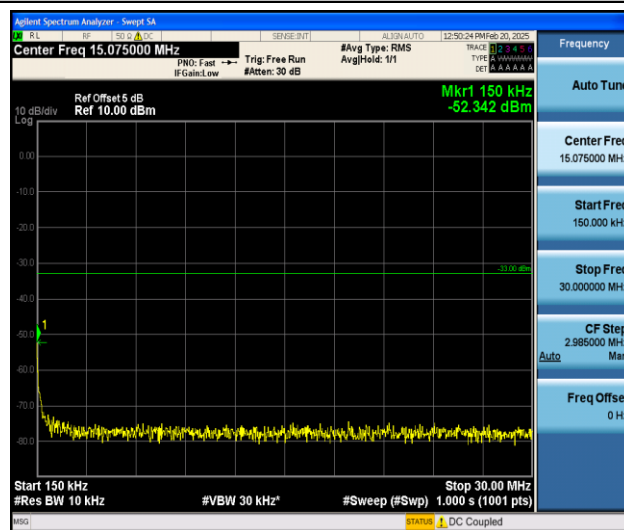
Band25_20MHz_QPSK_26590_1RB#0_0.15~30_0.15~30
