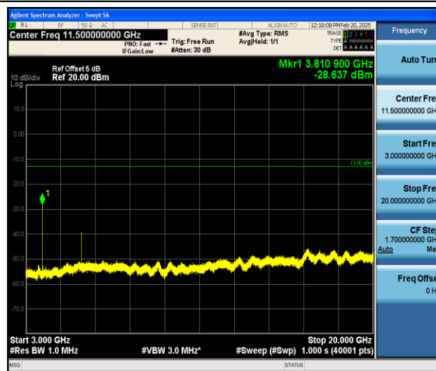
Band25_10MHz_QPSK_26640_1RB#0_3000~20000_3000~20000
