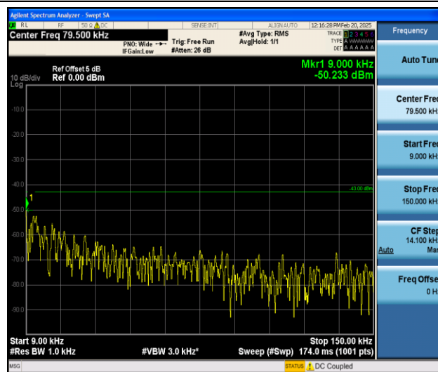
Band25_10MHz_16QAM_26365_1RB#0_0.009~0.15_0.009~0.15
