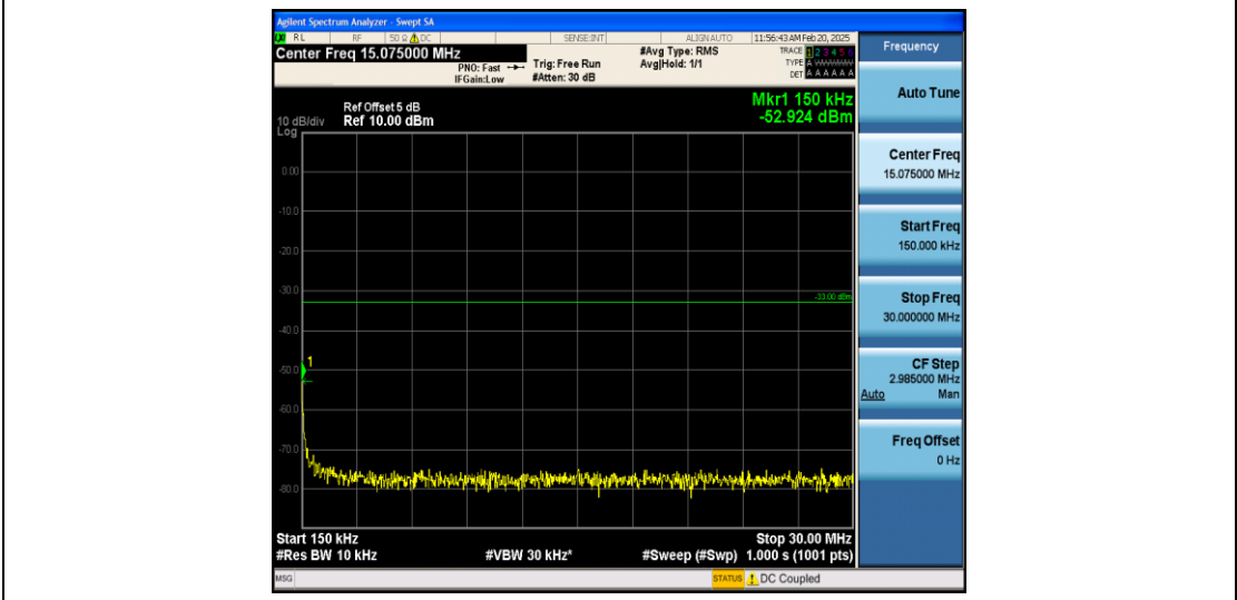
Band25_5MHz_16QAM_26665_1RB#0_0.15~30_0.15~30
