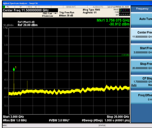
Band25_10MHz_16QAM_26365_1RB#0_3000~20000_3000~20000
