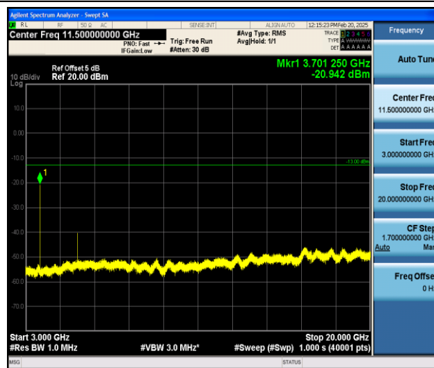
Band25_10MHz_16QAM_26090_1RB#0_3000~20000_3000~20000
