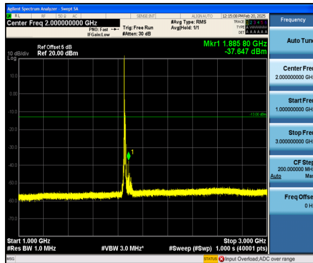
Band25_10MHz_16QAM_26090_1RB#0_1000~3000_1000~3000
