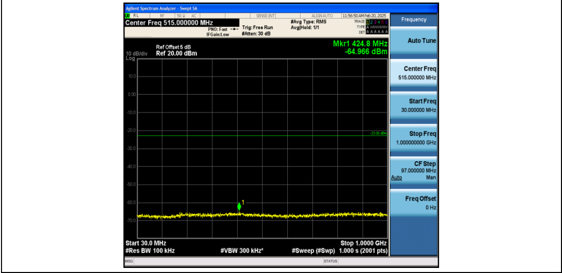
Band25_5MHz_16QAM_26665_1RB#0_30~1000_30~1000
