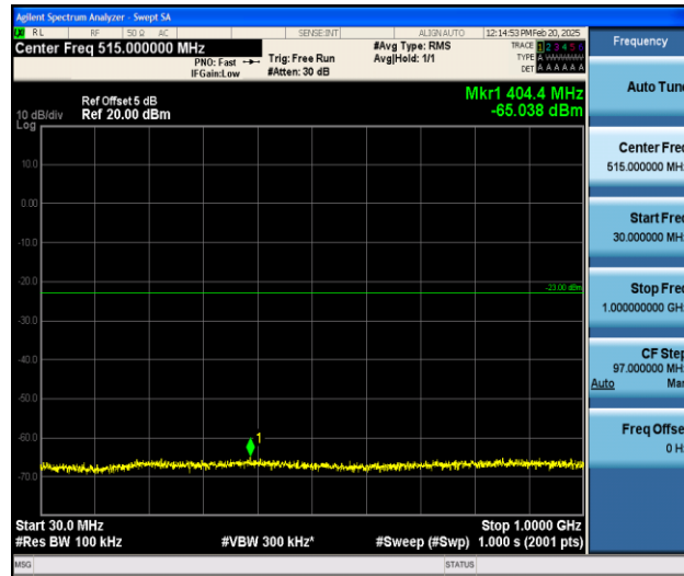
Band25_10MHz_16QAM_26090_1RB#0_30~1000_30~1000
