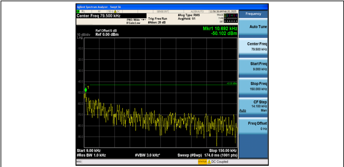
Band25_5MHz_16QAM_26665_1RB#0_0.009~0.15_0.009~0.15
