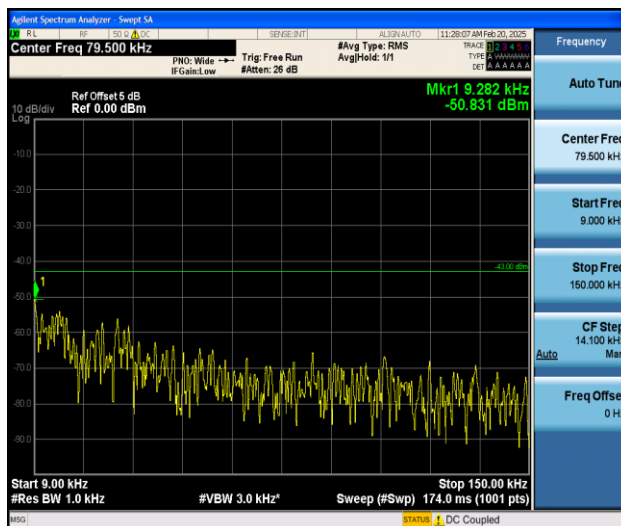
Band25_3MHz_16QAM_26055_1RB#0_0.009~0.15_0.009~0.15
