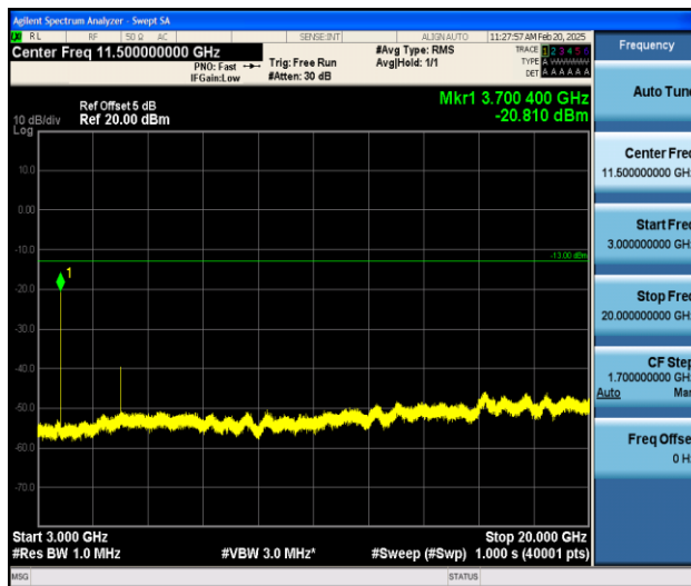
Band25_3MHz_QPSK_26055_1RB#0_3000~20000_3000~20000
