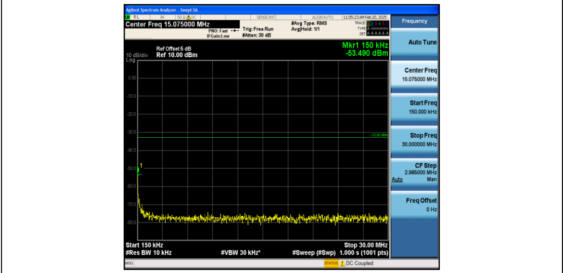
Band25_1.4MHz_QPSK_26365_1RB#0_0.15~30_0.15~30
