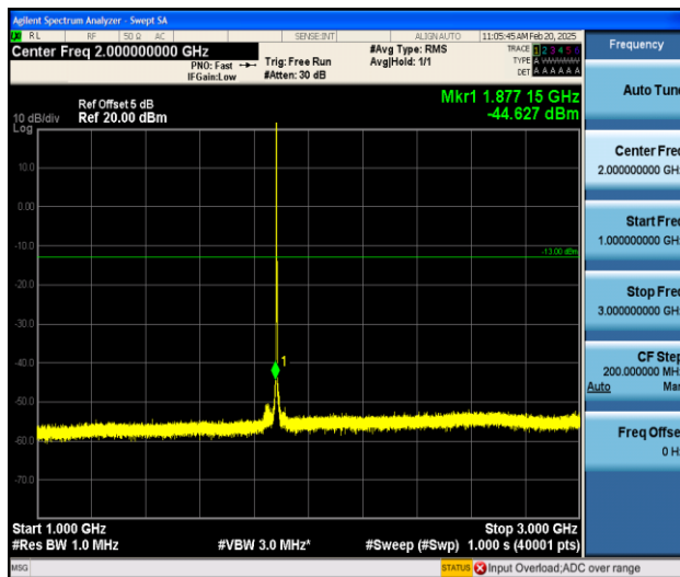
Band25_1.4MHz_QPSK_26365_1RB#0_1000~3000_1000~3000
