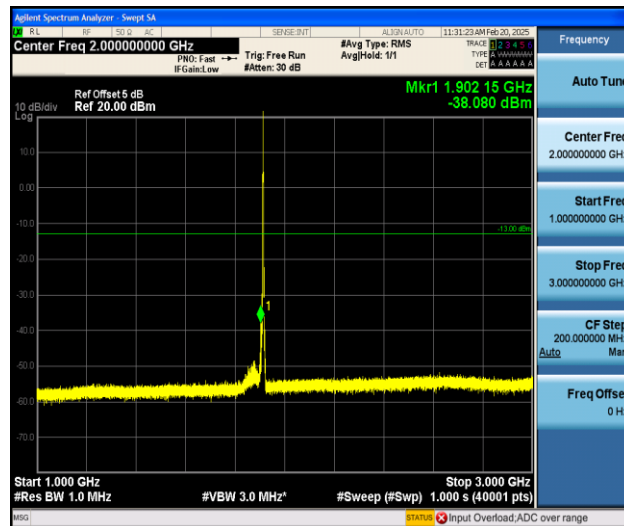
Band25_3MHz_QPSK_26675_1RB#0_1000~3000_1000~3000
