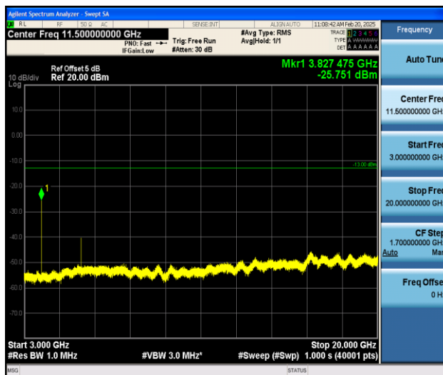
Band25_1.4MHz_16QAM_26683_1RB#0_3000~20000_3000~20000
