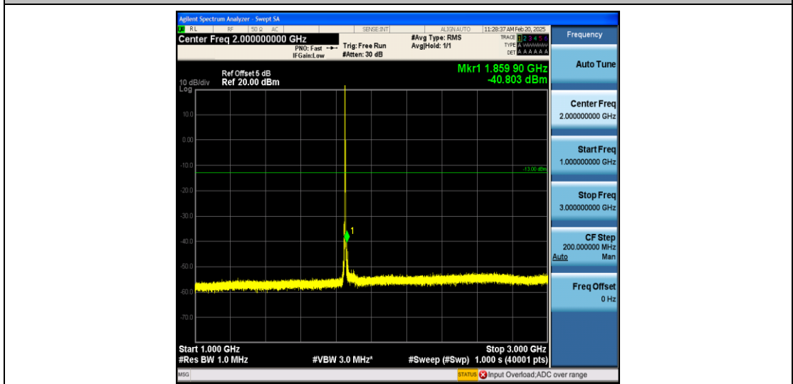
Band25_3MHz_16QAM_26055_1RB#0_1000~3000_1000~3000
