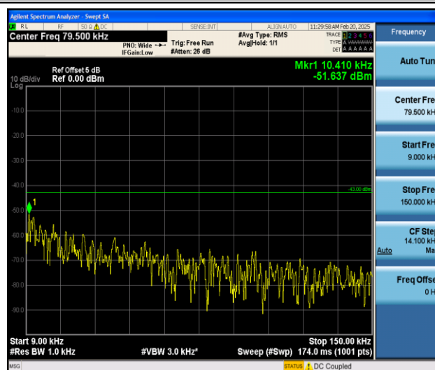
Band25_3MHz_16QAM_26365_1RB#0_0.009~0.15_0.009~0.15
