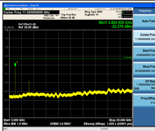
Band25_3MHz_QPSK_26675_1RB#0_3000~20000_3000~20000
