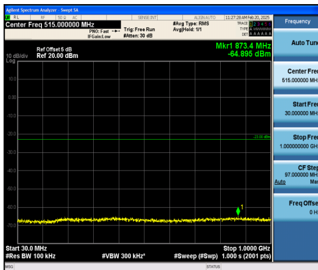
Band25_3MHz_QPSK_26055_1RB#0_30~1000_30~1000
