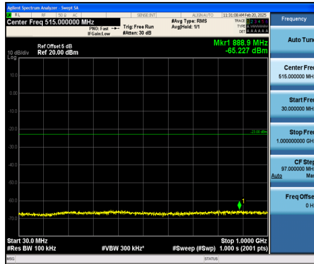
Band25_3MHz_QPSK_26675_1RB#0_30~1000_30~1000
