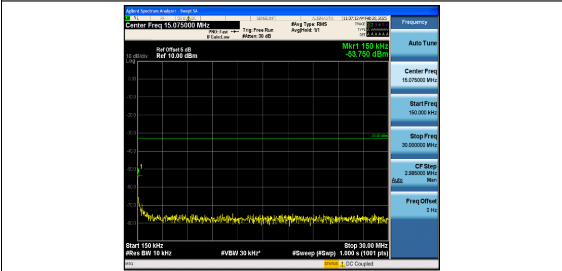
Band25_1.4MHz_QPSK_26683_1RB#0_0.15~30_0.15~30
