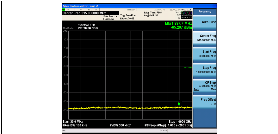
Band25_3MHz_16QAM_26055_1RB#0_30~1000_30~1000
