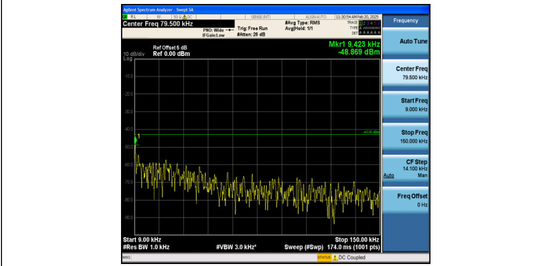
Band25_3MHz_QPSK_26675_1RB#0_0.009~0.15_0.009~0.15
