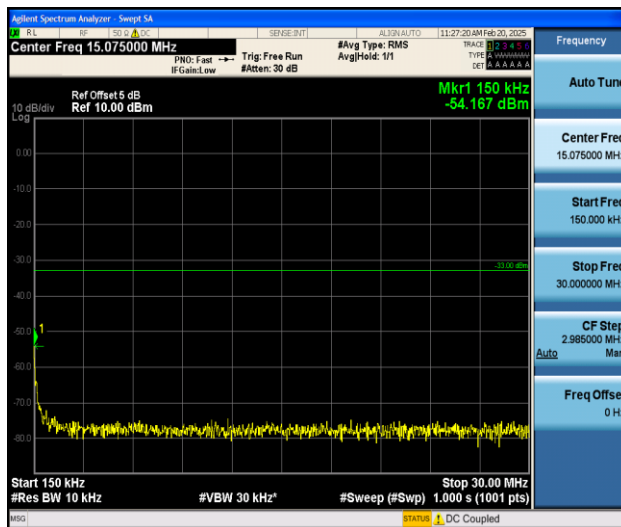
Band25_3MHz_QPSK_26055_1RB#0_0.15~30_0.15~30
