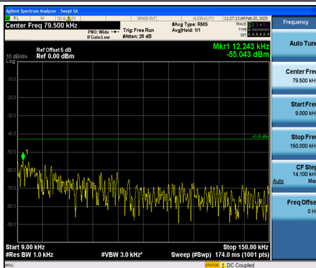
Band25_3MHz_QPSK_26055_1RB#0_0.009~0.15_0.009~0.15
