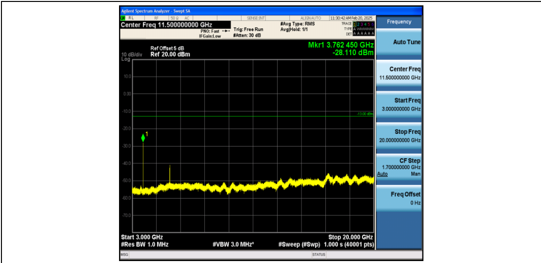
Band25_3MHz_16QAM_26365_1RB#0_3000~20000_3000~20000
