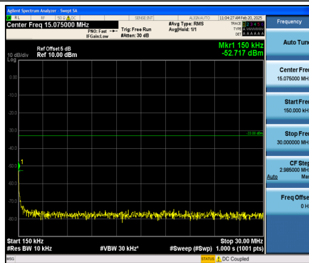
Band25_1.4MHz_16QAM_26047_1RB#0_0.15~30_0.15~30
