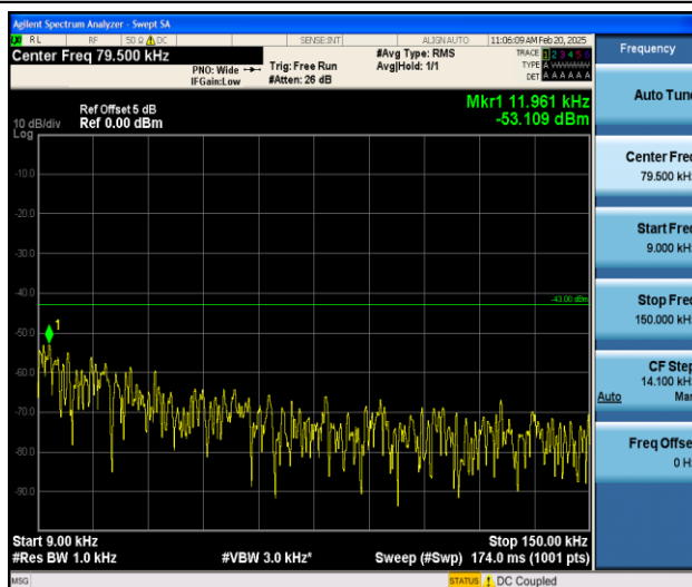
Band25_1.4MHz_16QAM_26365_1RB#0_0.009~0.15_0.009~0.15
