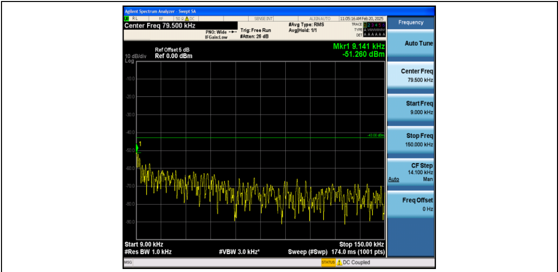
Band25_1.4MHz_QPSK_26365_1RB#0_0.009~0.15_0.009~0.15
