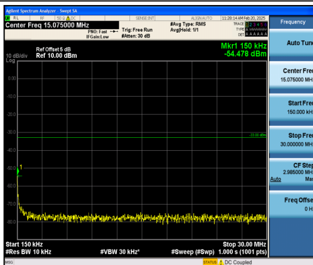
Band25_3MHz_16QAM_26055_1RB#0_0.15~30_0.15~30
