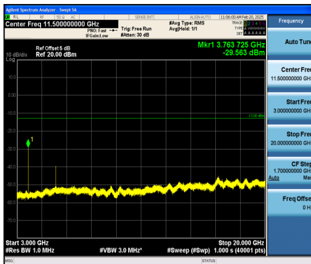
Band25_1.4MHz_QPSK_26365_1RB#0_3000~20000_3000~20000
