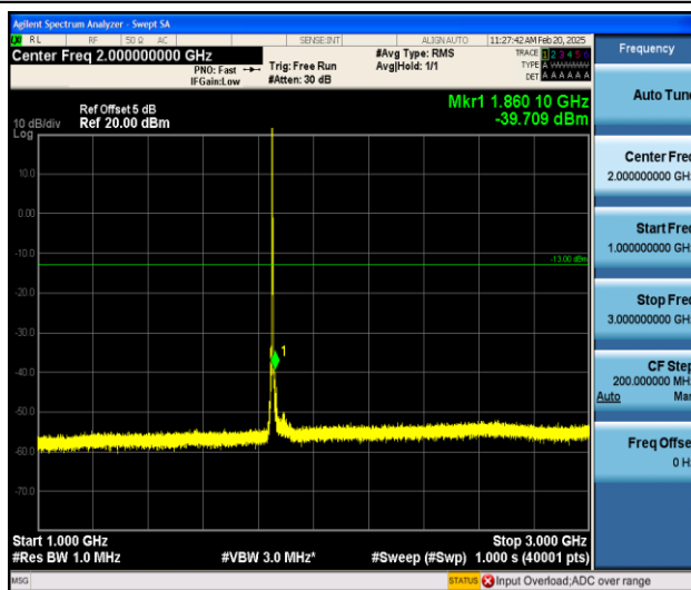
Band25_3MHz_QPSK_26055_1RB#0_1000~3000_1000~3000
