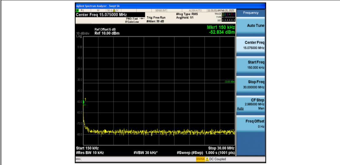
Band25_3MHz_QPSK_26675_1RB#0_0.15~30_0.15~30
