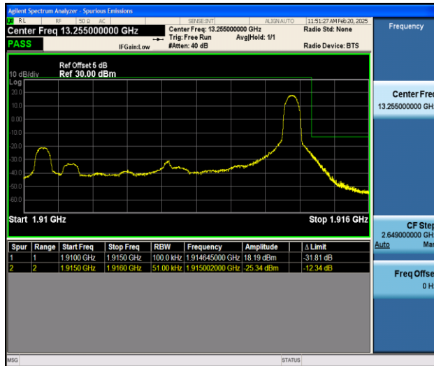
Band25_5MHz_16QAM_26665_1RB#24
