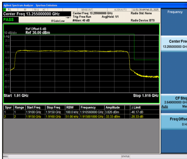
Band25_5MHz_QPSK_26665_25RB#0
