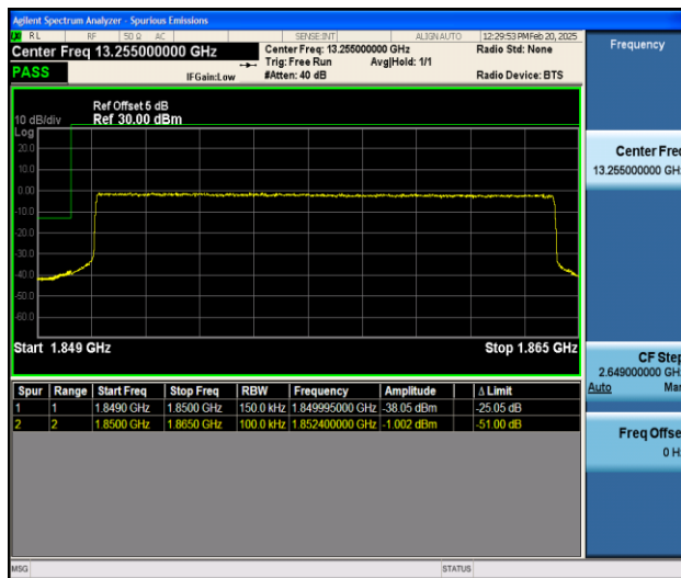
Band25_15MHz_QPSK_26115_75RB#0
