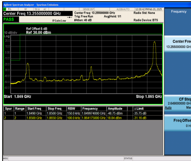
Band25_15MHz_16QAM_26115_1RB#74
