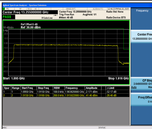
Band25_20MHz_QPSK_26590_100RB#0
