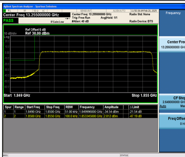
Band25_5MHz_16QAM_26065_25RB#0
