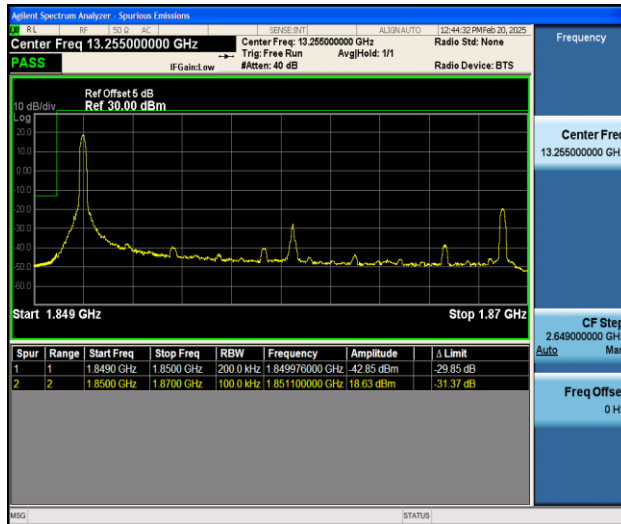
Band25_20MHz_16QAM_26140_1RB#0
