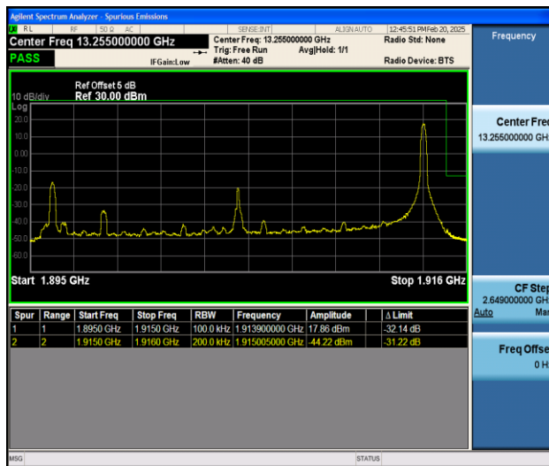
Band25_20MHz_16QAM_26590_1RB#99
