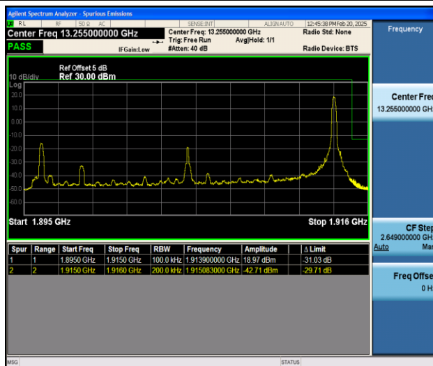
Band25_20MHz_QPSK_26590_1RB#99
