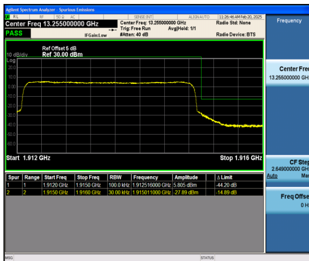
Band25_3MHz_QPSK_26675_15RB#0
