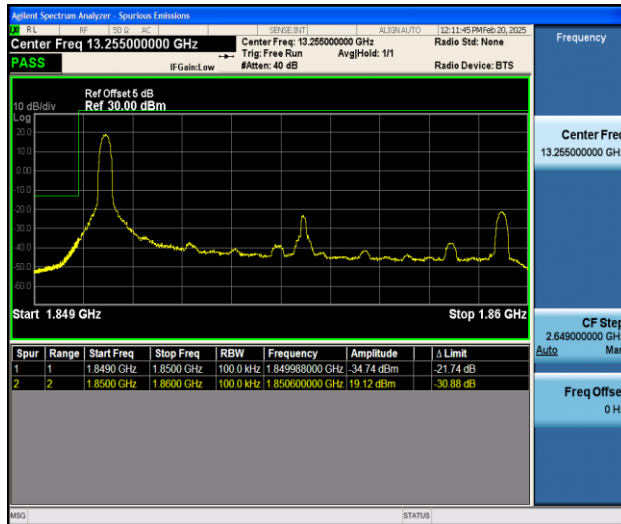
Band25_10MHz_16QAM_26090_1RB#0
