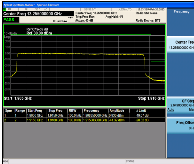
Band25_10MHz_QPSK_26640_50RB#0
