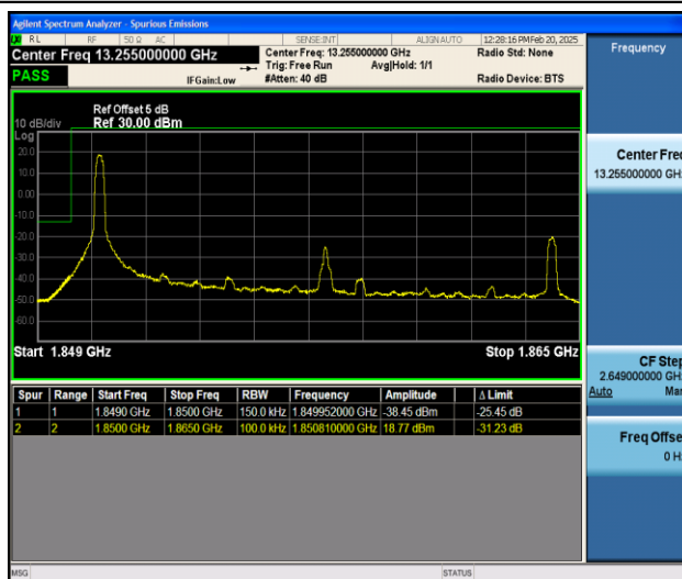
Band25_15MHz_16QAM_26115_1RB#0
