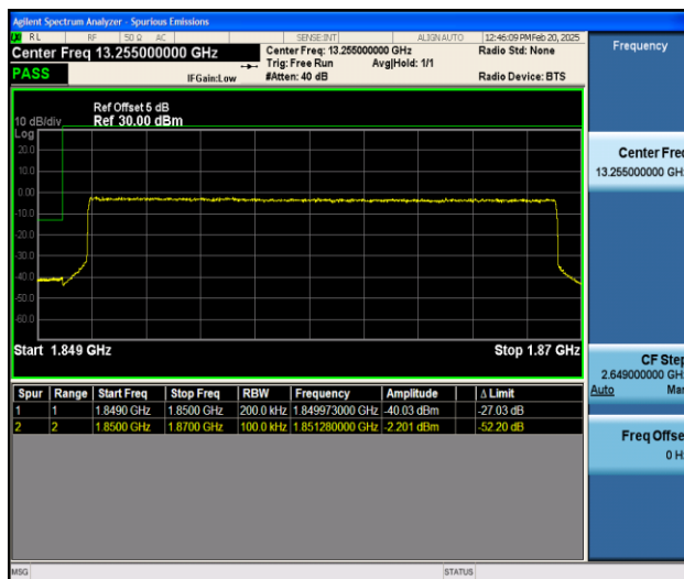
Band25_20MHz_QPSK_26140_100RB#0
