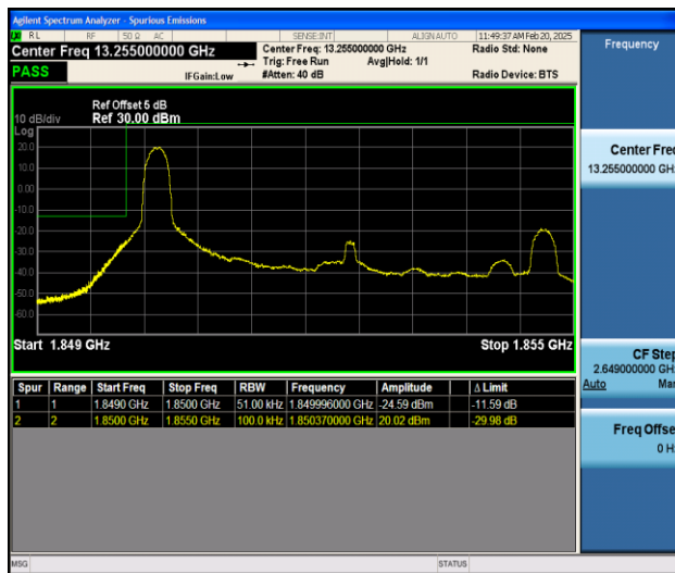
Band25_5MHz_QPSK_26065_1RB#0
