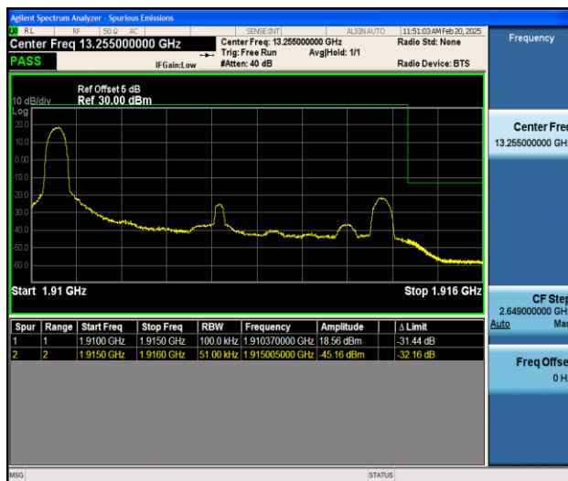
Band25_5MHz_16QAM_26665_1RB#0
