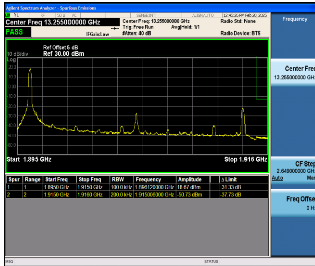
Band25_20MHz_16QAM_26590_1RB#0
