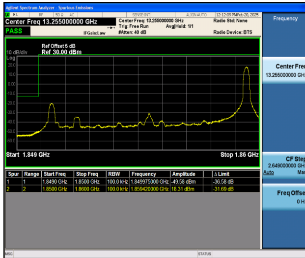
Band25_10MHz_16QAM_26090_1RB#49
