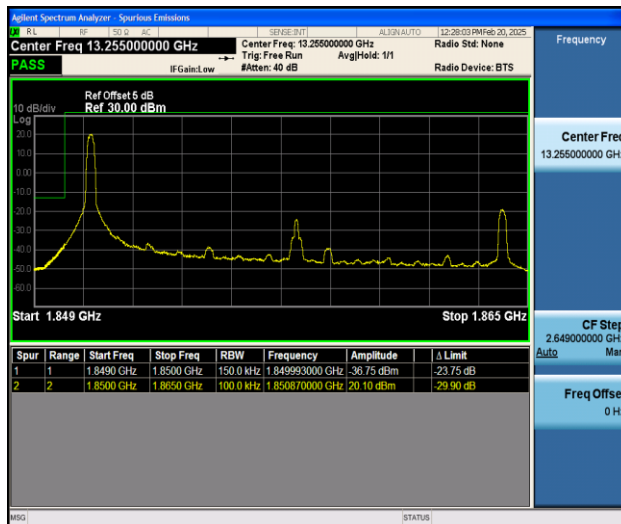
Band25_15MHz_QPSK_26115_1RB#0
