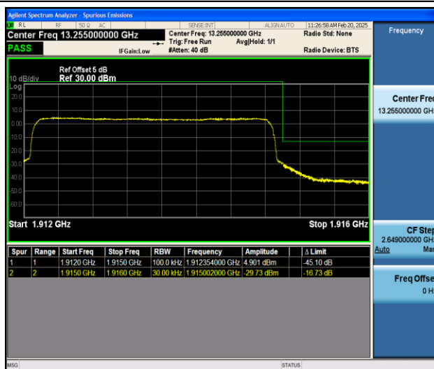
Band25_3MHz_16QAM_26675_15RB#0
