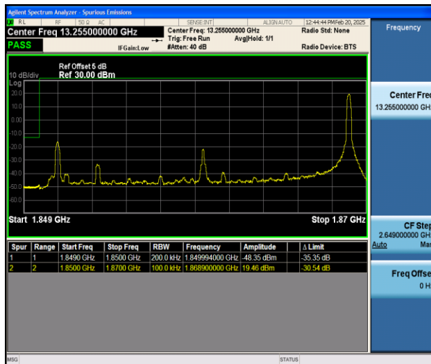
Band25_20MHz_QPSK_26140_1RB#99
