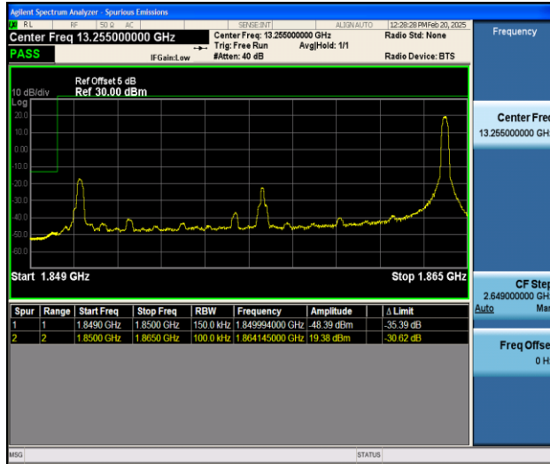
Band25_15MHz_QPSK_26115_1RB#74
