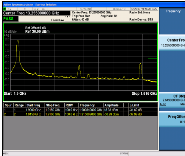
Band25_15MHz_16QAM_26615_1RB#0
