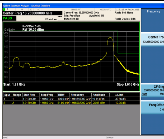
Band25_5MHz_QPSK_26665_1RB#24
