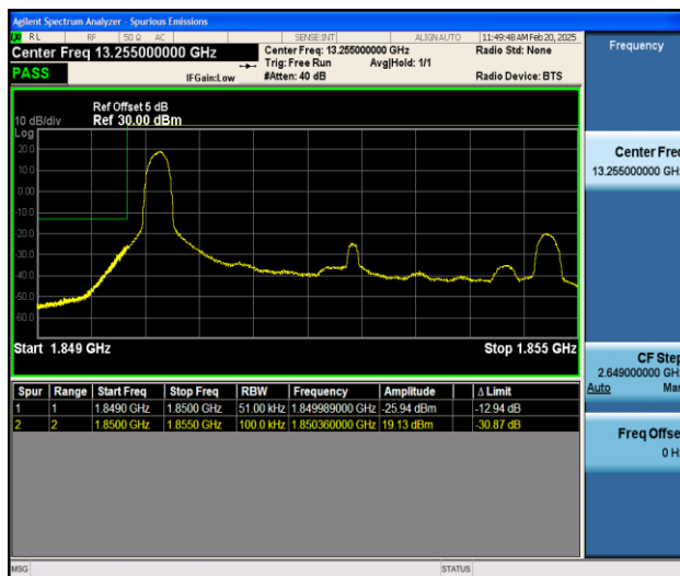
Band25_5MHz_16QAM_26065_1RB#0
