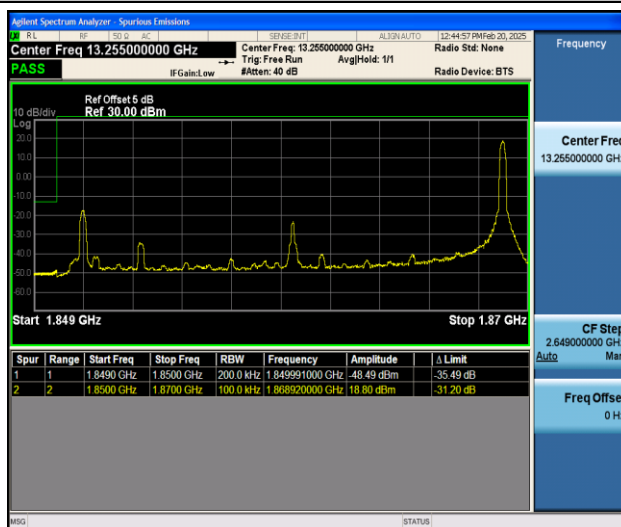
Band25_20MHz_16QAM_26140_1RB#99
