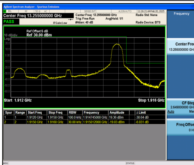
Band25_3MHz_QPSK_26675_1RB#14
