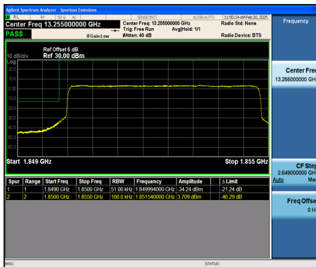
Band25_5MHz_QPSK_26065_25RB#0
