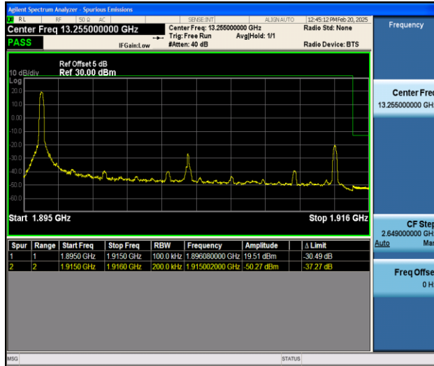
Band25_20MHz_QPSK_26590_1RB#0
