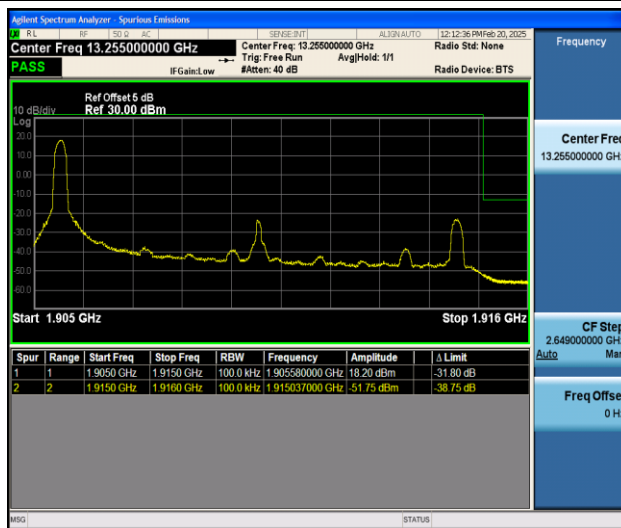
Band25_10MHz_16QAM_26640_1RB#0
