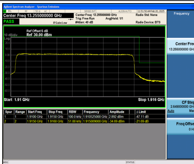
Band25_5MHz_16QAM_26665_25RB#0
