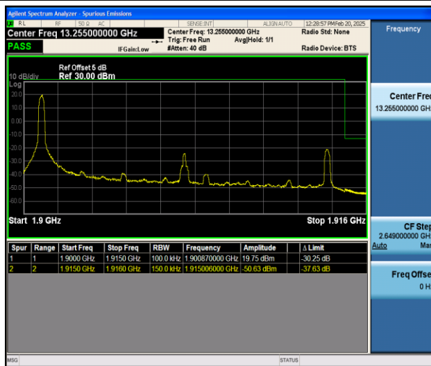
Band25_15MHz_QPSK_26615_1RB#0
