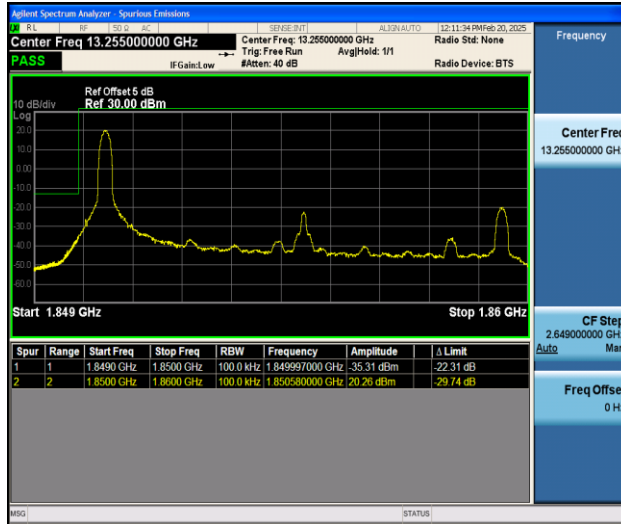
Band25_10MHz_QPSK_26090_1RB#0
