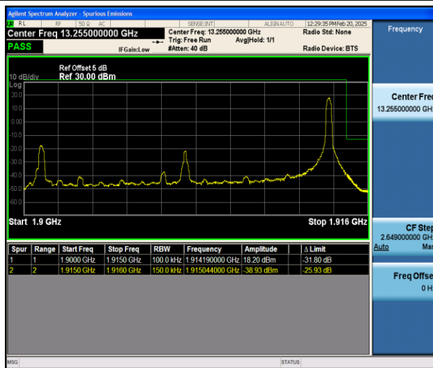
Band25_15MHz_16QAM_26615_1RB#74
