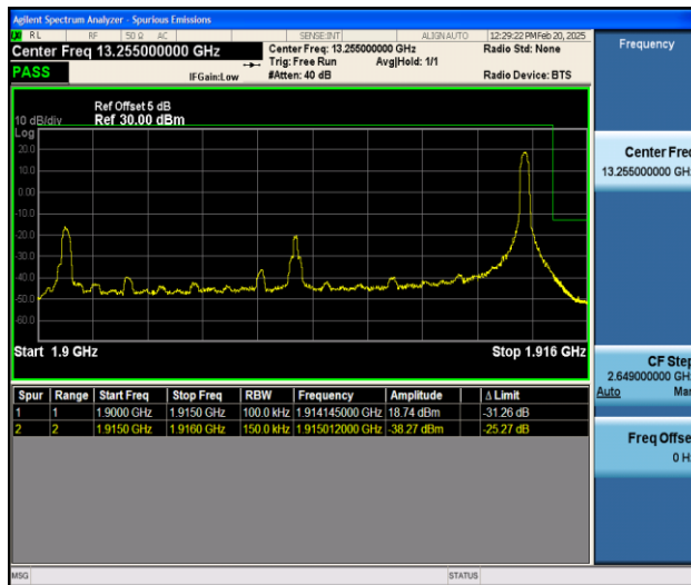
Band25_15MHz_QPSK_26615_1RB#74
