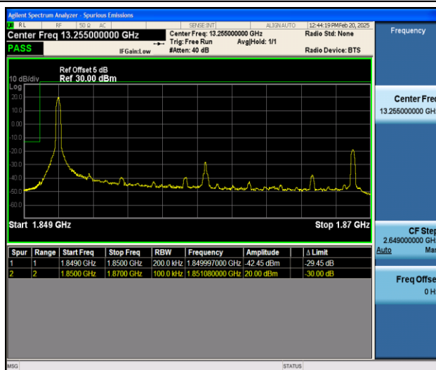
Band25_20MHz_QPSK_26140_1RB#0
