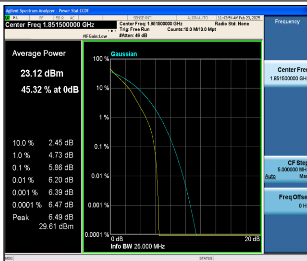
Band25-3MHz-QPSK-26055-15RB#0-PASS
