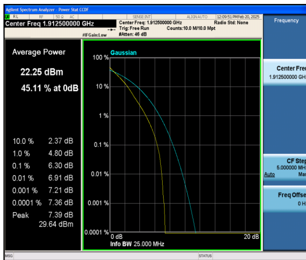
Band25-5MHz-QPSK-26665-25RB#0-PASS
