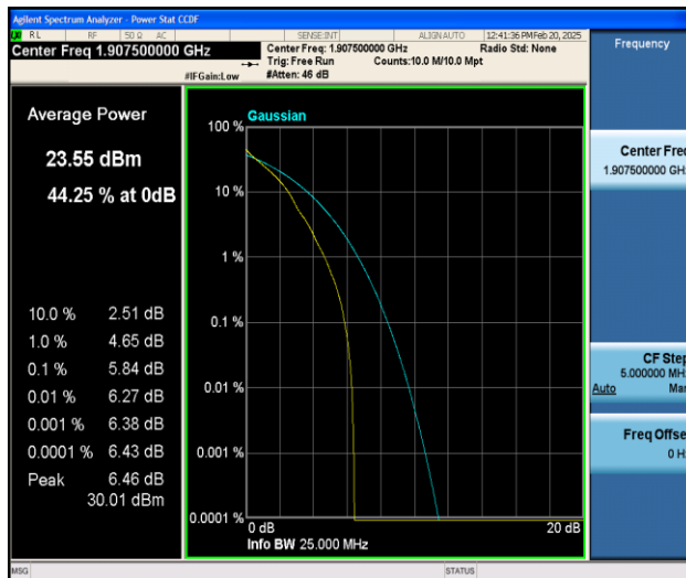
Band25-15MHz-QPSK-26615-1RB#0-PASS
