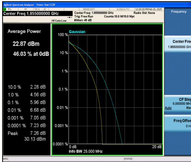
Band25-10MHz-QPSK-26090-50RB#0-PASS
