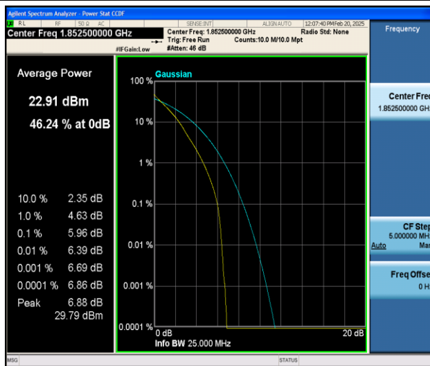
Band25-5MHz-QPSK-26065-25RB#0-PASS
