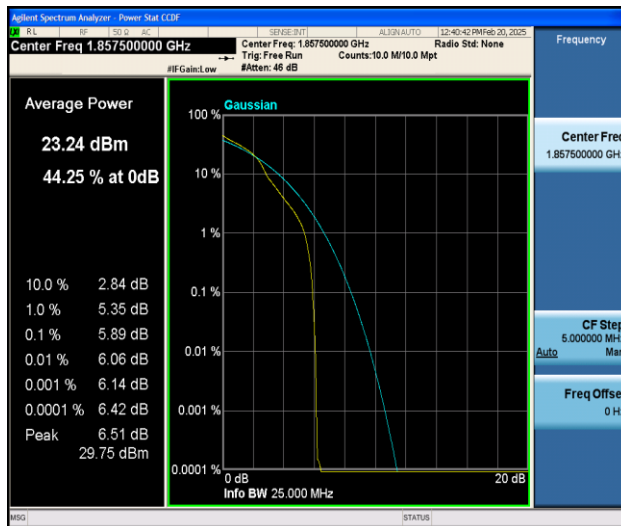
Band25-15MHz-16QAM-26115-1RB#0-PASS
