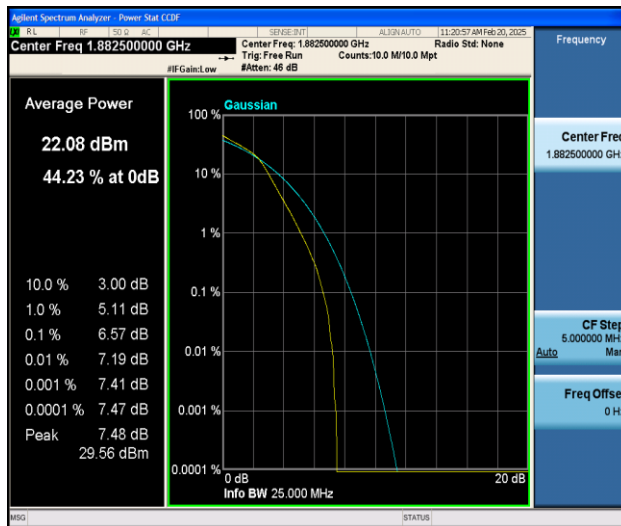
Band25-1.4MHz-16QAM-26365-6RB#0-PASS
