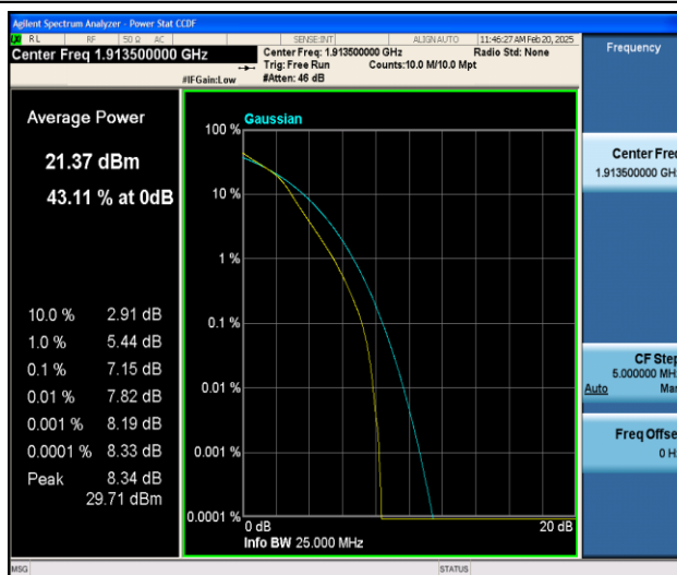
Band25-3MHz-16QAM-26675-15RB#0-PASS
