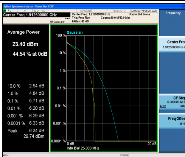
Band25-5MHz-QPSK-26665-1RB#0-PASS
