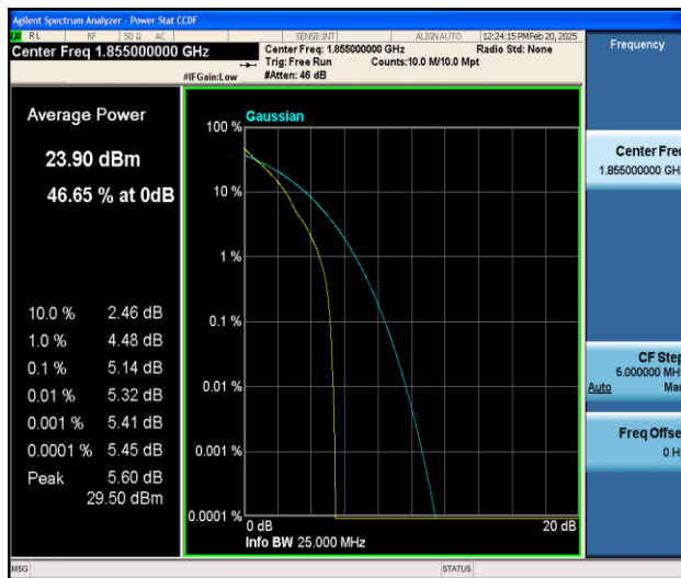
Band25-10MHz-QPSK-26090-1RB#0-PASS
