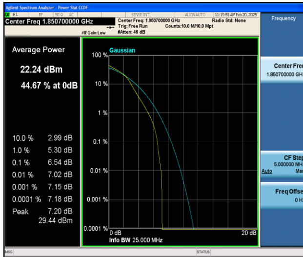
Band25-1.4MHz-16QAM-26047-6RB#0-PASS
