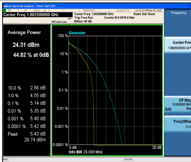
Band25-15MHz-QPSK-26365-1RB#0-PASS
