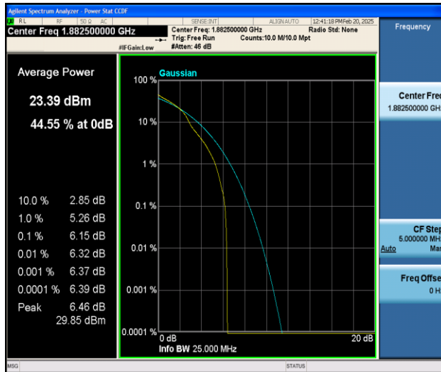
Band25-15MHz-16QAM-26365-1RB#0-PASS
