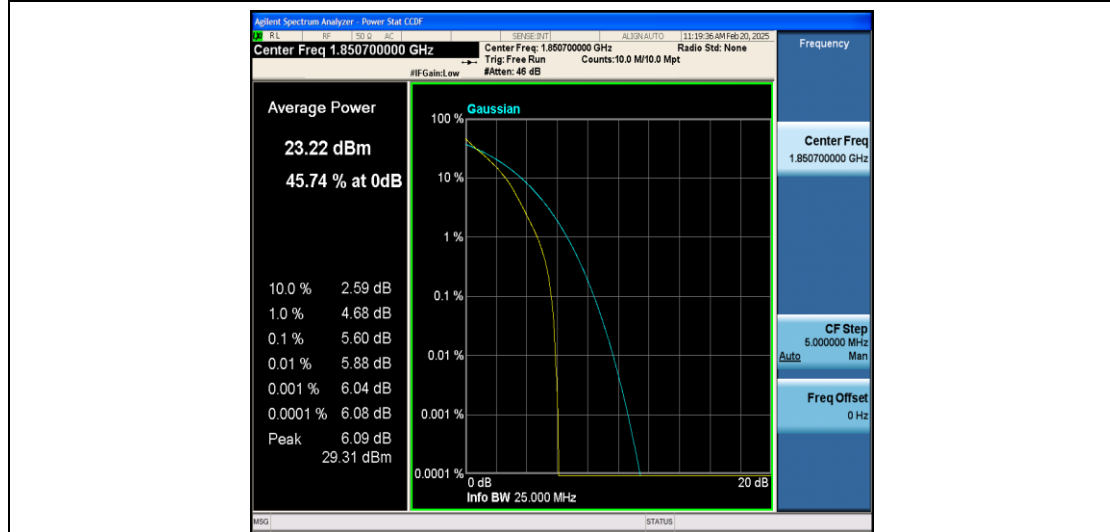
Band25-1.4MHz-QPSK-26047-6RB#0-PASS
