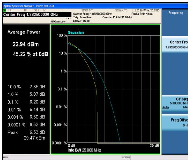
Band25-1.4MHz-16QAM-26365-1RB#0-PASS
