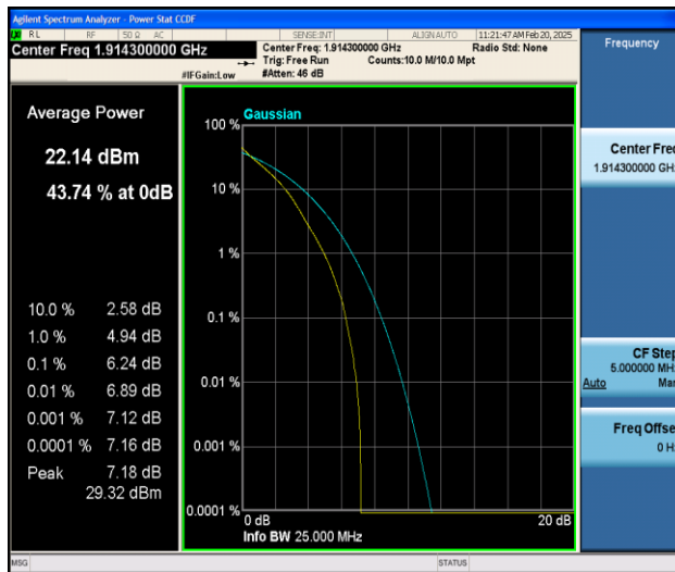
Band25-1.4MHz-QPSK-26683-6RB#0-PASS
