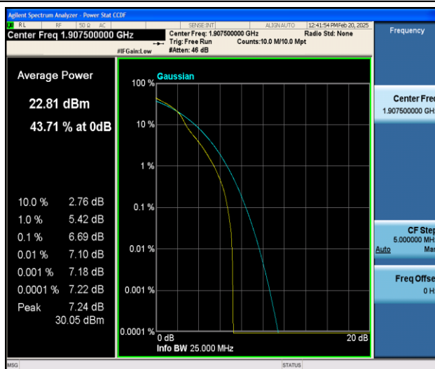
Band25-15MHz-16QAM-26615-1RB#0-PASS
