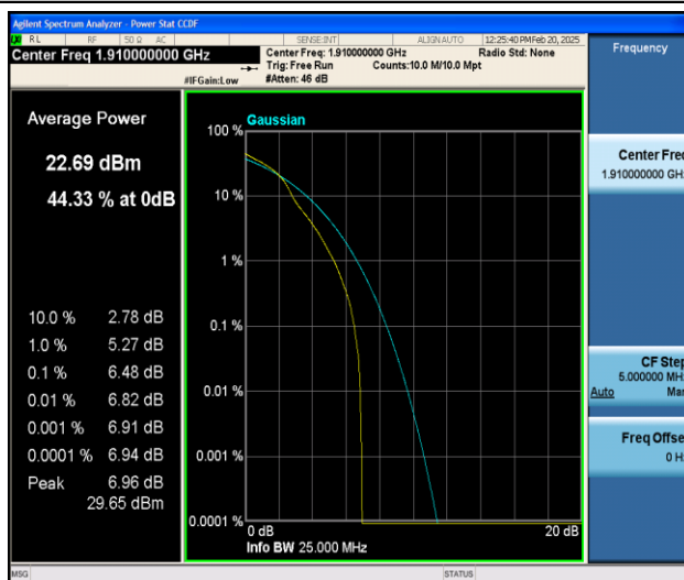
Band25-10MHz-16QAM-26640-1RB#0-PASS
