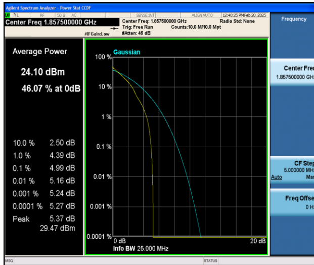
Band25-15MHz-QPSK-26115-1RB#0-PASS
