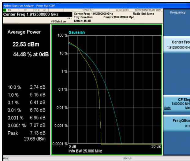
Band25-5MHz-16QAM-26665-1RB#0-PASS
