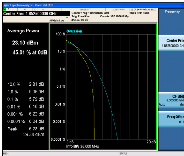
Band25-5MHz-16QAM-26065-1RB#0-PASS
