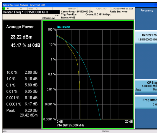
Band25-3MHz-16QAM-26055-1RB#0-PASS
