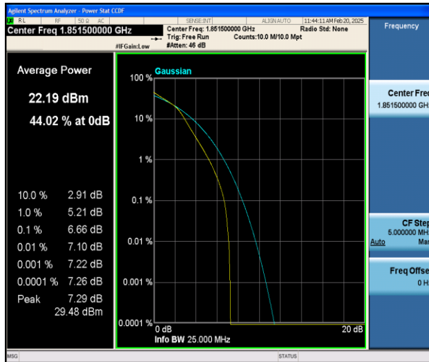
Band25-3MHz-16QAM-26055-15RB#0-PASS
