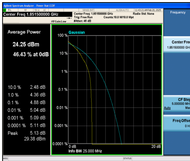
Band25-3MHz-QPSK-26055-1RB#0-PASS
