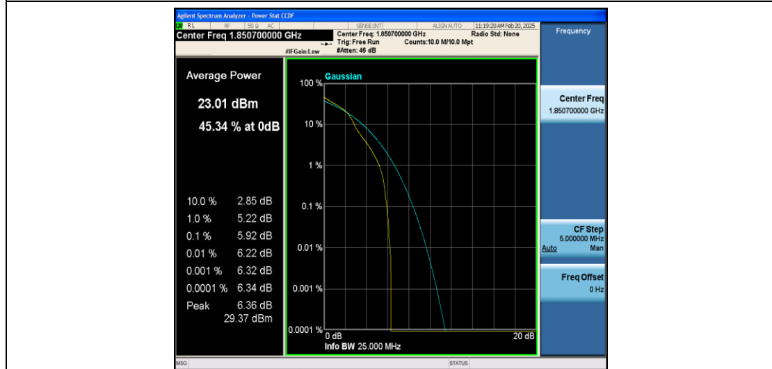
Band25-1.4MHz-16QAM-26047-1RB#0-PASS
