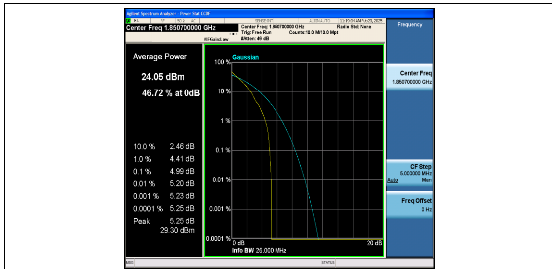
Band25-1.4MHz-QPSK-26047-1RB#0-PASS
