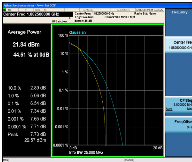
Band25-5MHz-16QAM-26365-25RB#0-PASS
