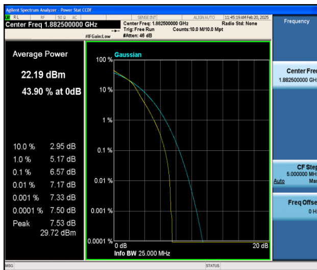
Band25-3MHz-16QAM-26365-15RB#0-PASS
