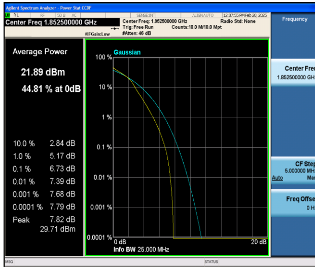
Band25-5MHz-16QAM-26065-25RB#0-PASS
