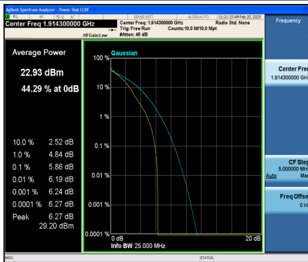
Band25-1.4MHz-QPSK-26683-1RB#0-PASS
