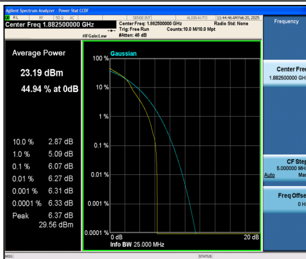
Band25-3MHz-16QAM-26365-1RB#0-PASS
