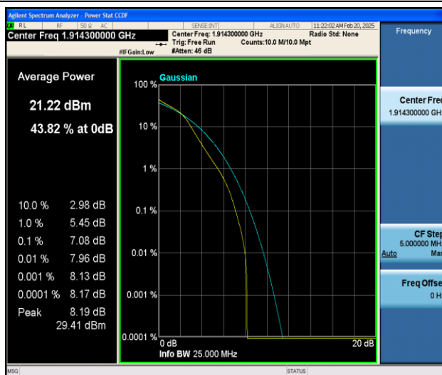
Band25-1.4MHz-16QAM-26683-6RB#0-PASS
