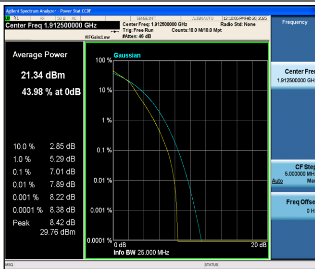
Band25-5MHz-16QAM-26665-25RB#0-PASS
