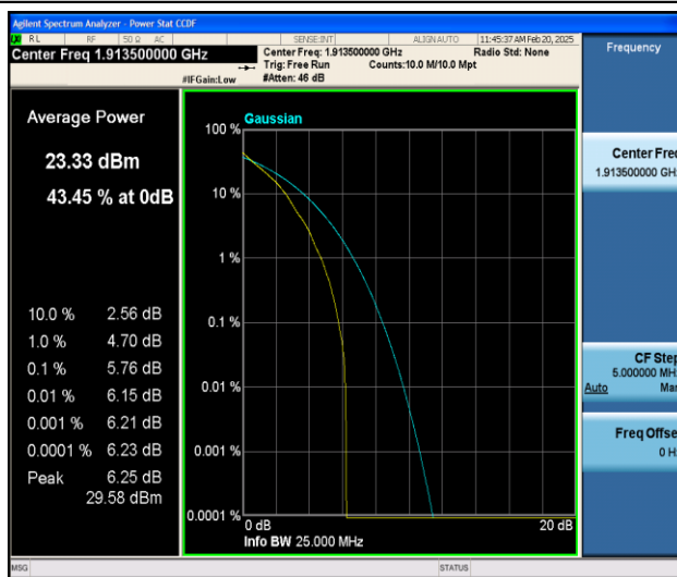
Band25-3MHz-QPSK-26675-1RB#0-PASS
