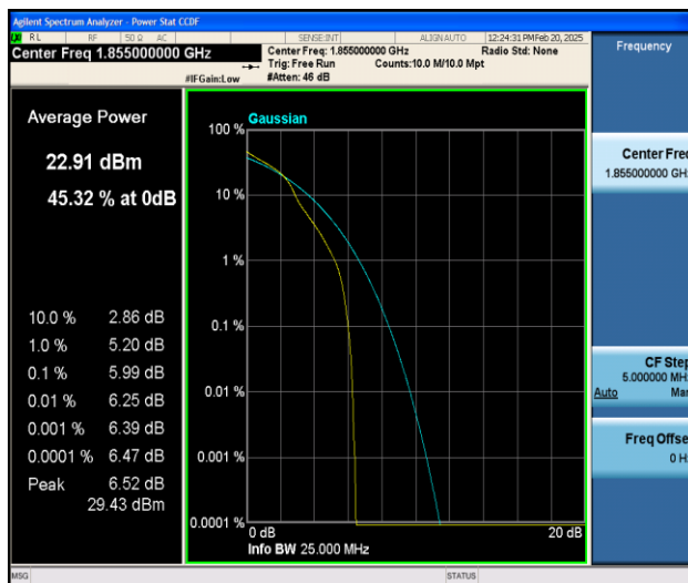
Band25-10MHz-16QAM-26090-1RB#0-PASS
