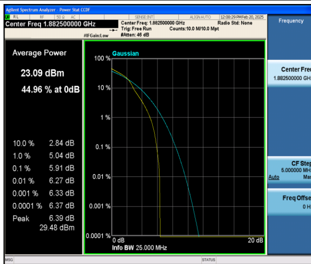
Band25-5MHz-16QAM-26365-1RB#0-PASS
