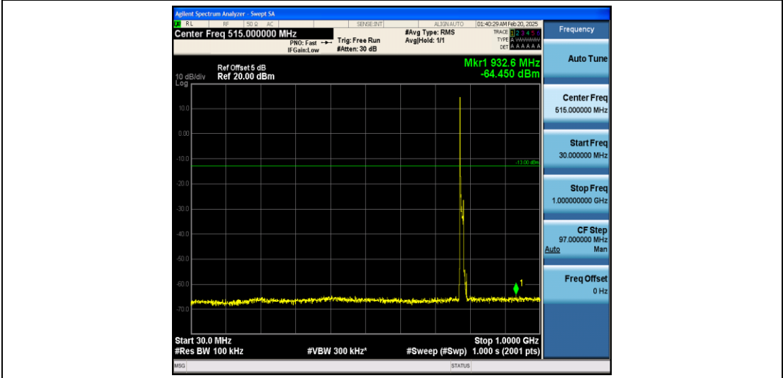
Band13_10MHz_16QAM_23230_1RB#0_30~1000_30~1000
