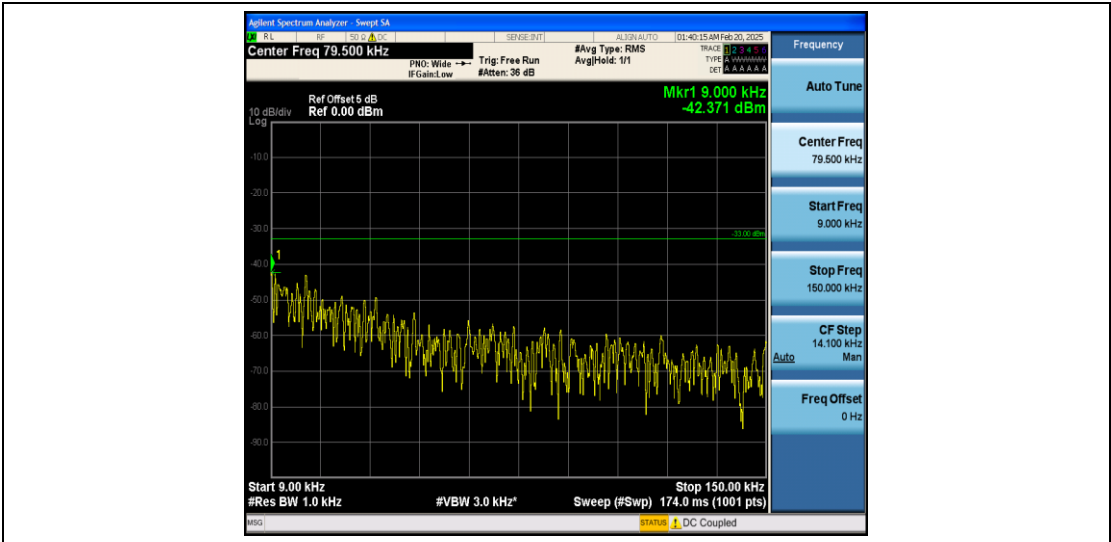
Band13_10MHz_16QAM_23230_1RB#0_0.009~0.15_0.009~0.15
