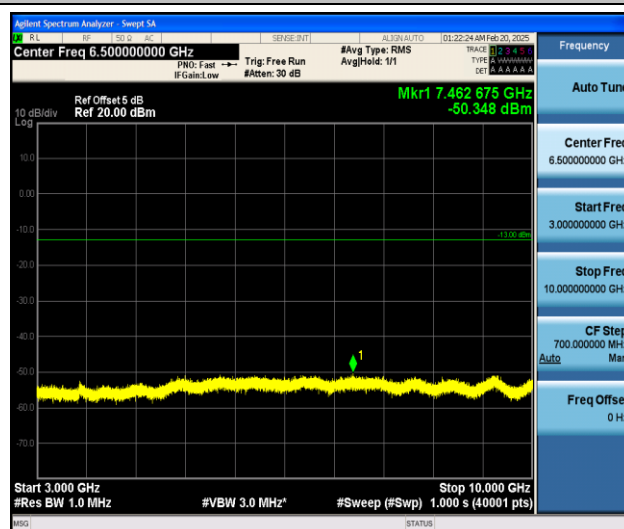
Band13_5MHz_16QAM_23230_1RB#0_3000~10000_3000~10000
