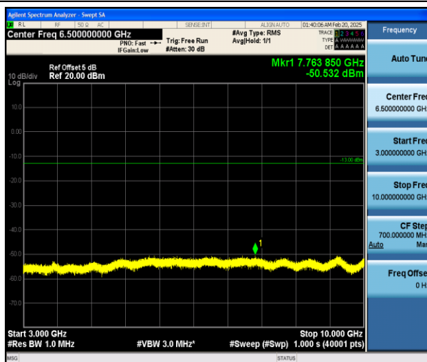
Band13_10MHz_QPSK_23230_1RB#0_3000~10000_3000~10000
