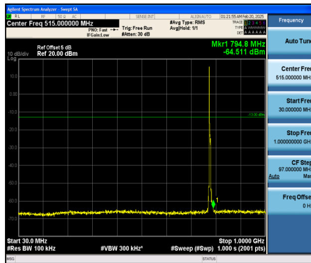
Band13_5MHz_16QAM_23230_1RB#0_30~1000_30~1000
