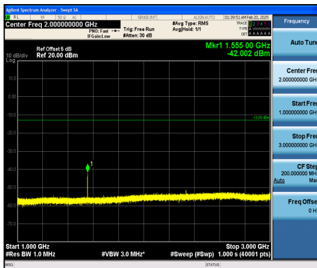
Band13_10MHz_QPSK_23230_1RB#0_1000~3000_1000~3000
