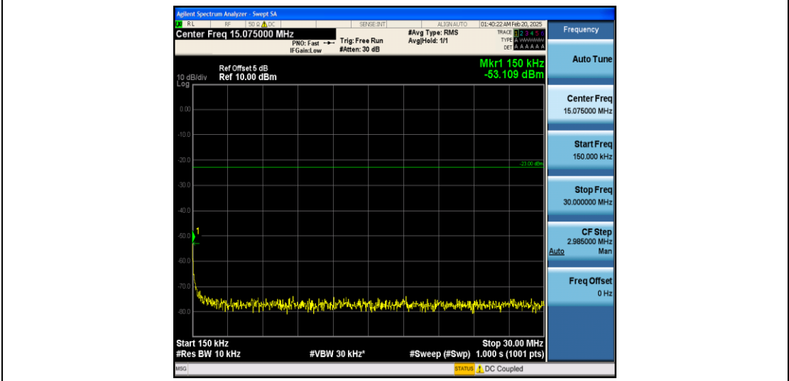
Band13_10MHz_16QAM_23230_1RB#0_0.15~30_0.15~30
