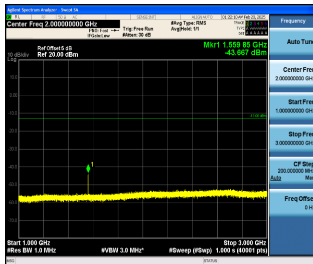
Band13_5MHz_16QAM_23230_1RB#0_1000~3000_1000~3000
