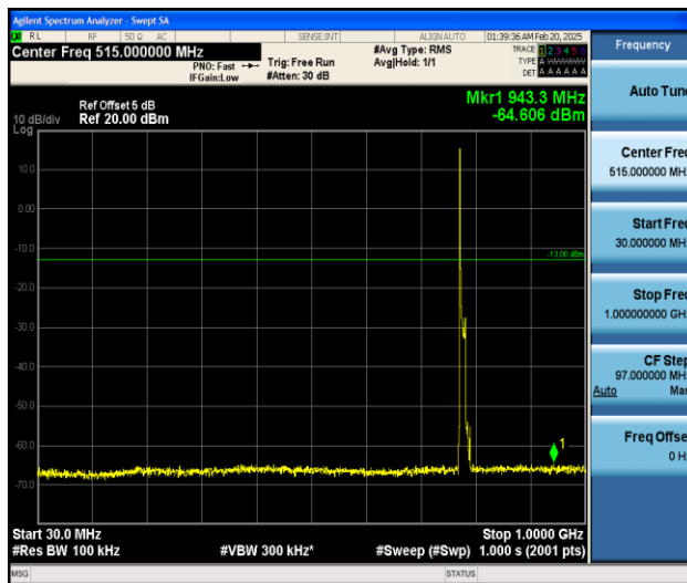
Band13_10MHz_QPSK_23230_1RB#0_30~1000_30~1000
