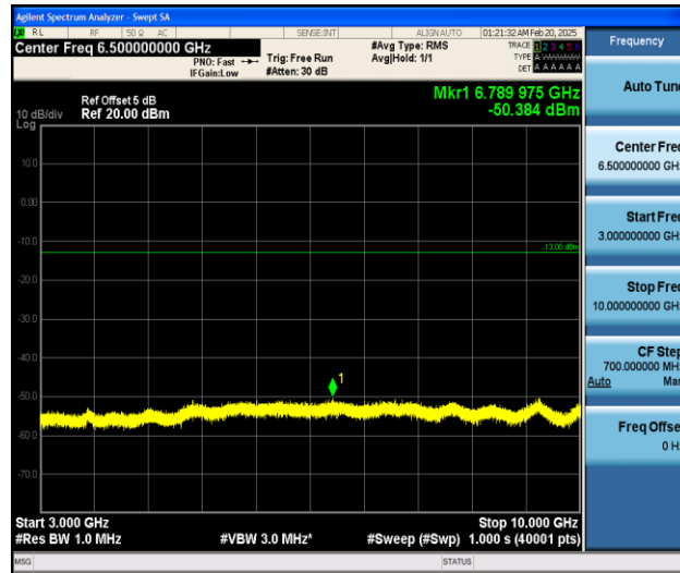
Band13_5MHz_QPSK_23230_1RB#0_3000~10000_3000~10000
