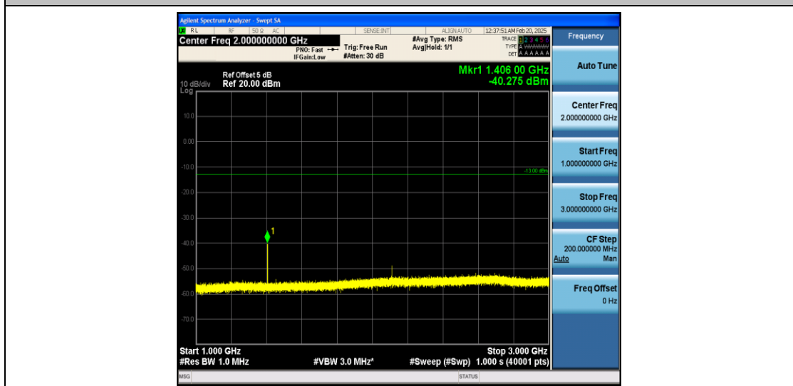
Band12_10MHz_QPSK_23095_1RB#0_1000~3000_1000~3000
