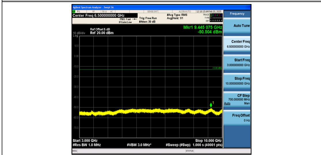
Band12_5MHz_16QAM_23155_1RB#0_3000~10000_3000~10000
