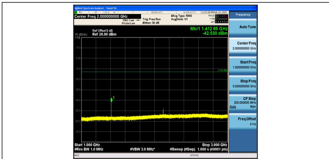
Band12_3MHz_16QAM_23095_1RB#0_1000~3000_1000~3000
