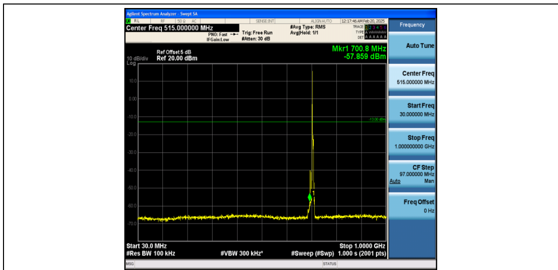
Band12_5MHz_16QAM_23155_1RB#0_30~1000_30~1000
