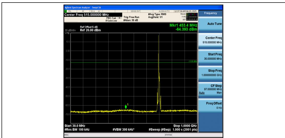
Band12_10MHz_QPSK_23095_1RB#0_30~1000_30~1000
