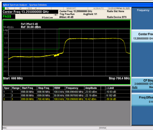
Band12_1.4MHz_QPSK_23017_6RB#0
