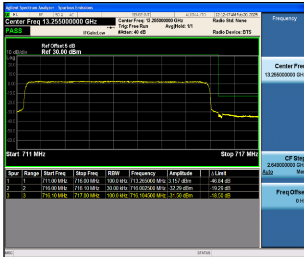
Band12_5MHz_16QAM_23155_25RB#0
