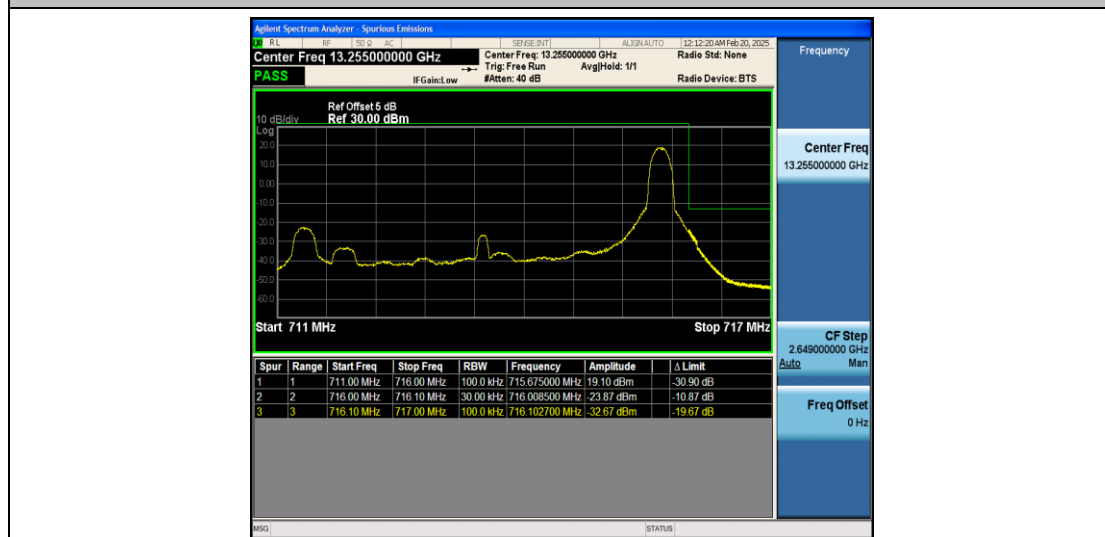
Band12_5MHz_16QAM_23155_1RB#24
