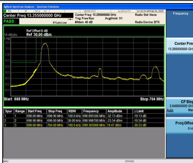
Band12_5MHz_16QAM_23035_1RB#0
