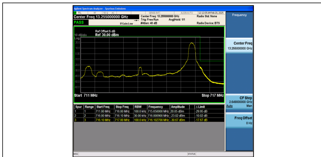
Band12_5MHz_QPSK_23155_1RB#24
