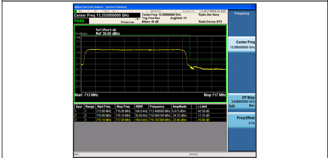
Band12_3MHz_QPSK_23165_15RB#0
