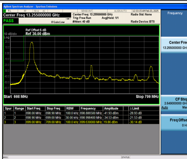
Band12_10MHz_16QAM_23060_1RB#0
