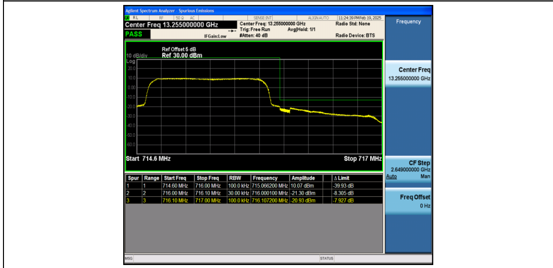
Band12_1.4MHz_QPSK_23173_6RB#0
