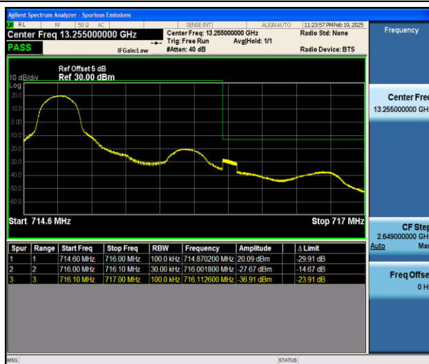
Band12_1.4MHz_16QAM_23173_1RB#0
