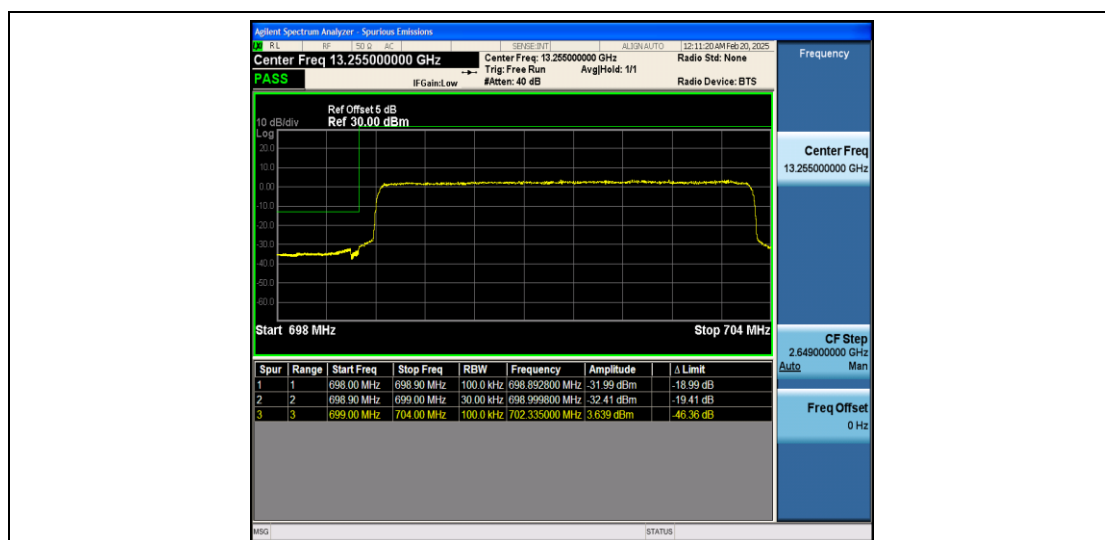
Band12_5MHz_16QAM_23035_25RB#0
