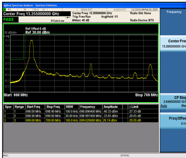
Band12_10MHz_QPSK_23060_1RB#0
