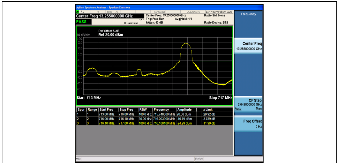
Band12_3MHz_QPSK_23165_1RB#14
