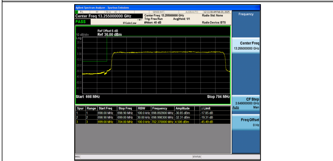
Band12_5MHz_QPSK_23035_25RB#0
