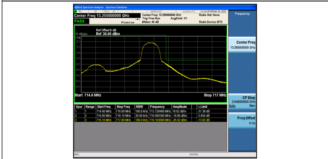
Band12_1.4MHz_16QAM_23173_1RB#5
