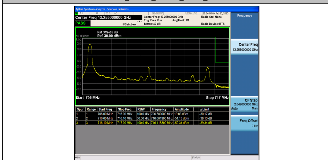
Band12_10MHz_QPSK_23130_1RB#0
