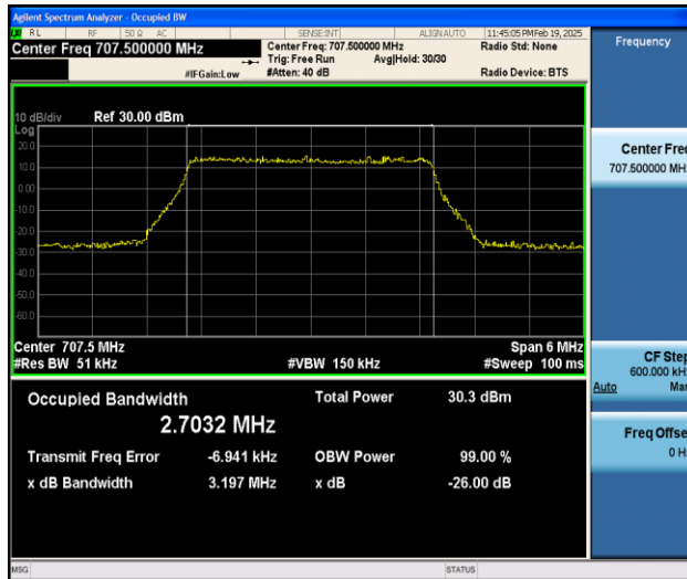
Band12-3MHz-16QAM-23095-15RB#0-PASS
