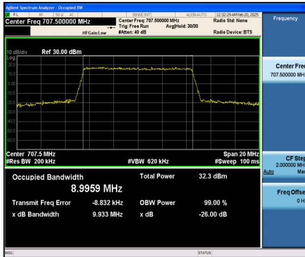
Band12-10MHz-QPSK-23095-50RB#0-PASS
