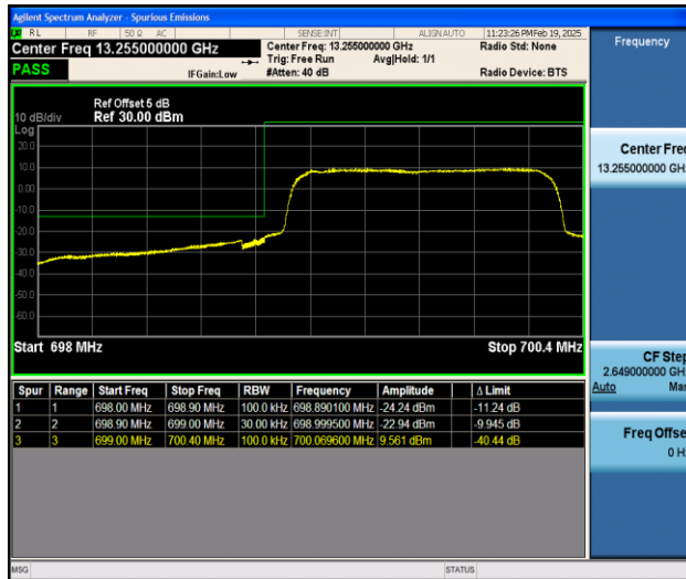
Band12_1.4MHz_16QAM_23017_6RB#0
