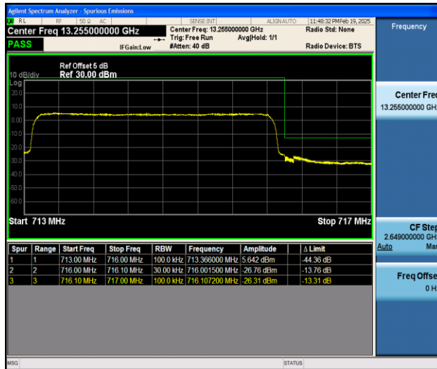
Band12_3MHz_16QAM_23165_15RB#0
