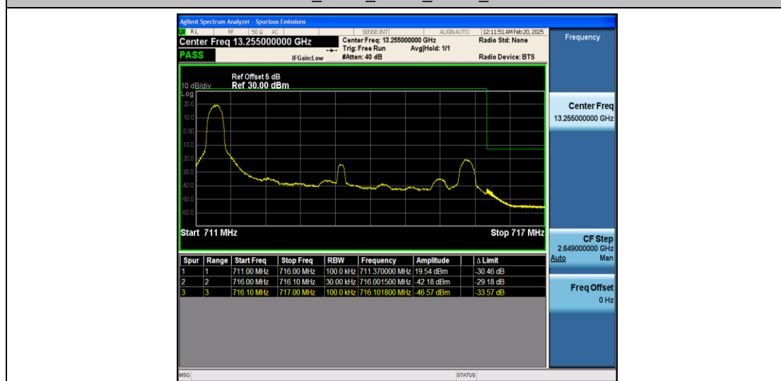
Band12_5MHz_16QAM_23155_1RB#0
