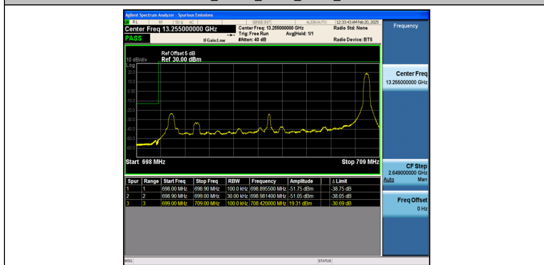
Band12_10MHz_16QAM_23060_1RB#49
