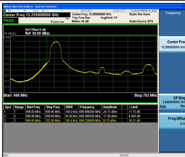
Band12_3MHz_16QAM_23025_1RB#0
