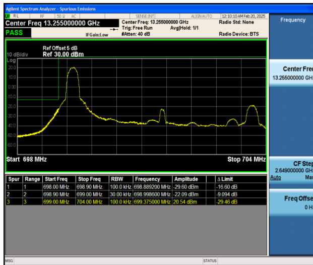
Band12_5MHz_QPSK_23035_1RB#0
