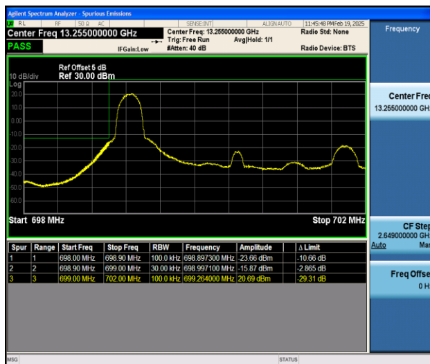
Band12_3MHz_QPSK_23025_1RB#0
