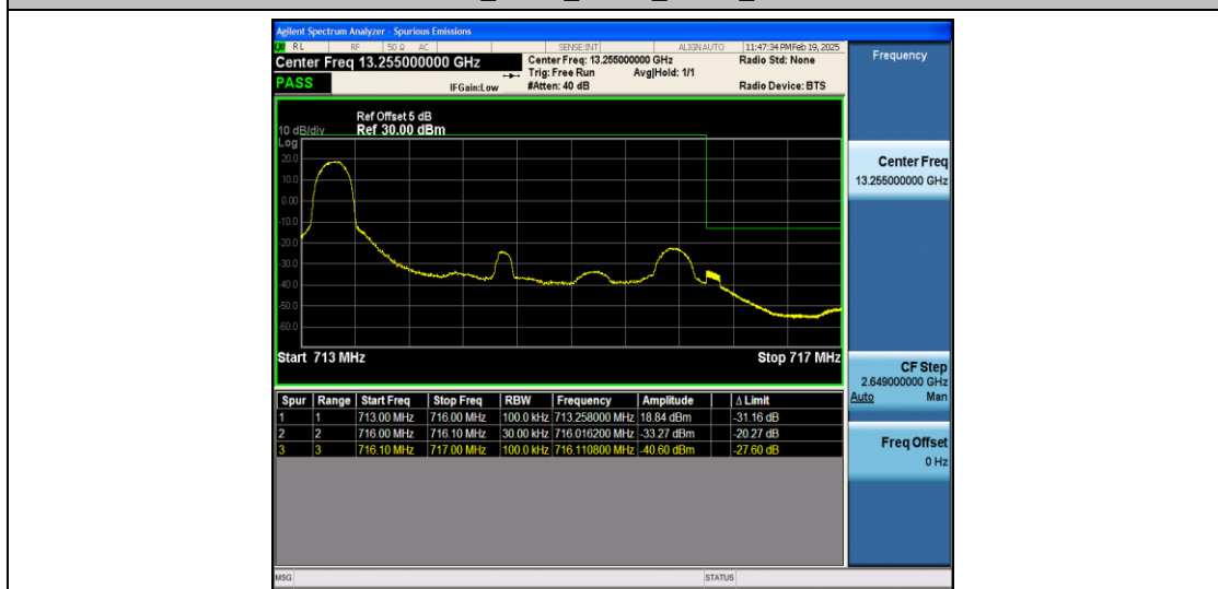
Band12_3MHz_16QAM_23165_1RB#0
