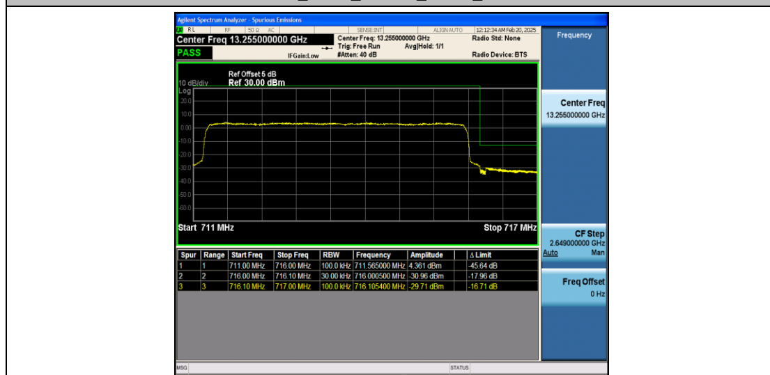
Band12_5MHz_QPSK_23155_25RB#0
