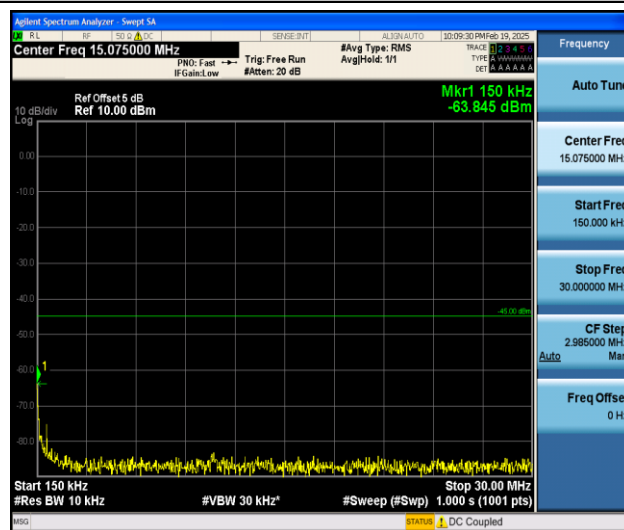
Band7_15MHz_16QAM_21375_1RB#0_0.15~30_0.15~30
