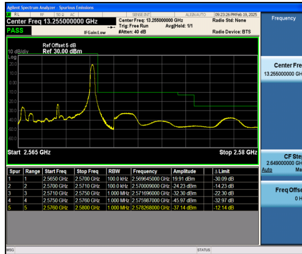
Band7_5MHz_QPSK_21425_1RB#24
