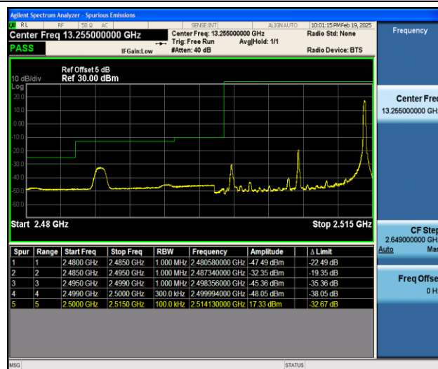
Band7_15MHz_16QAM_20825_1RB#74
