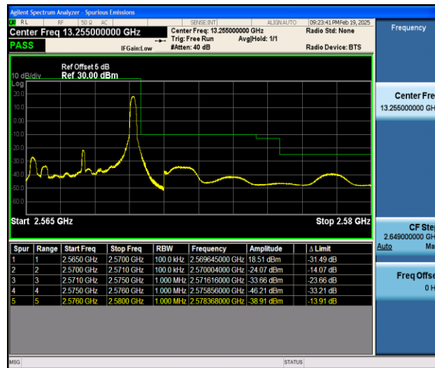
Band7_5MHz_16QAM_21425_1RB#24
