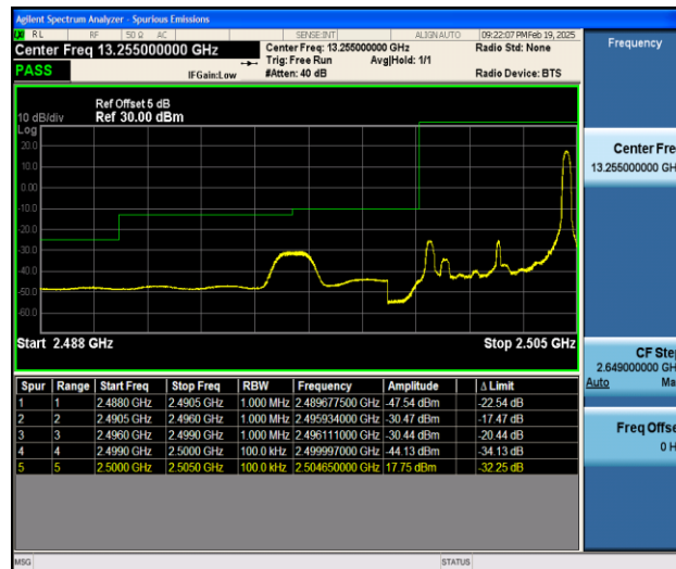
Band7_5MHz_16QAM_20775_1RB#24
