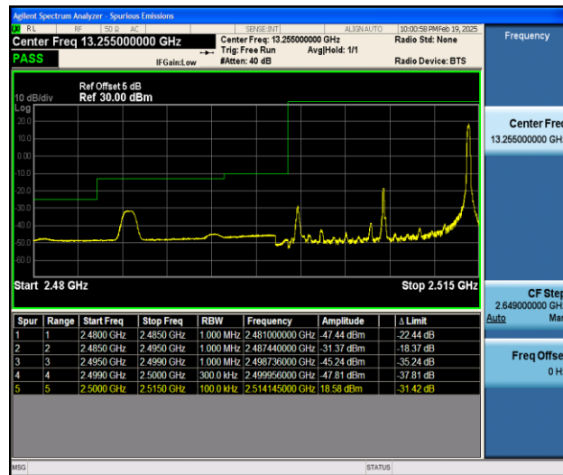
Band7_15MHz_QPSK_20825_1RB#74
