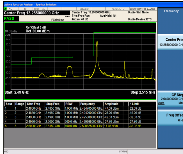
Band7_15MHz_16QAM_20825_1RB#0
