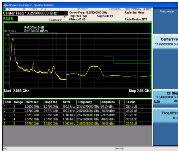
Band7_5MHz_QPSK_21425_1RB#0
