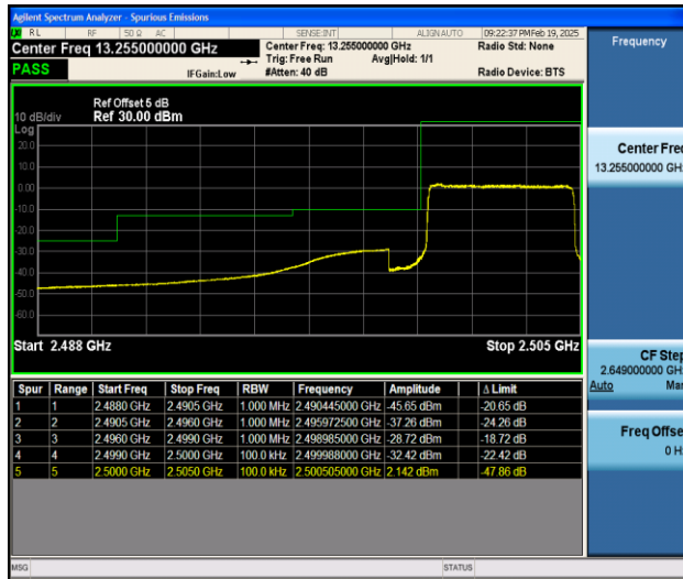
Band7_5MHz_16QAM_20775_25RB#0
