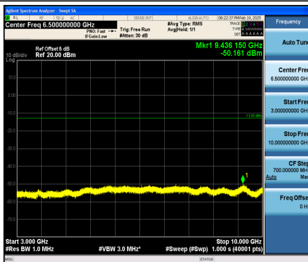
Band5_10MHz_16QAM_20600_1RB#0_3000~10000_3000~10000
