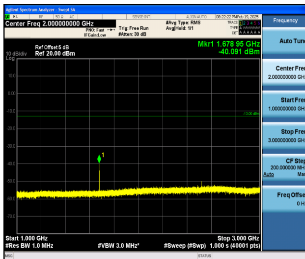
Band5_10MHz_16QAM_20600_1RB#0_1000~3000_1000~3000
