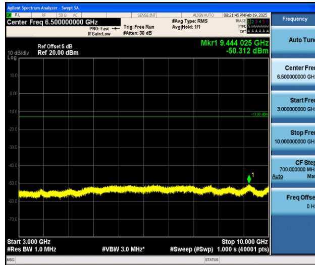
Band5_10MHz_QPSK_20600_1RB#0_3000~10000_3000~10000
