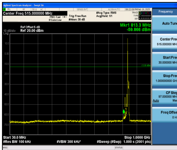
Band5_10MHz_16QAM_20600_1RB#0_30~1000_30~1000
