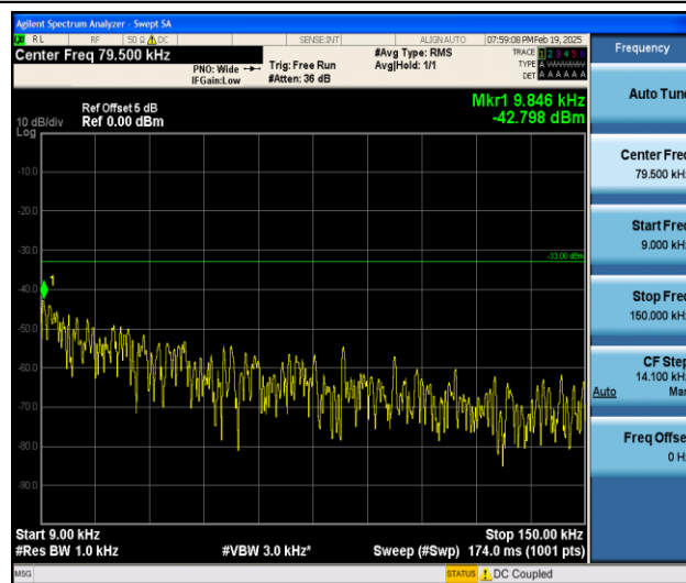
Band5_5MHz_QPSK_20625_1RB#0_0.009~0.15_0.009~0.15
