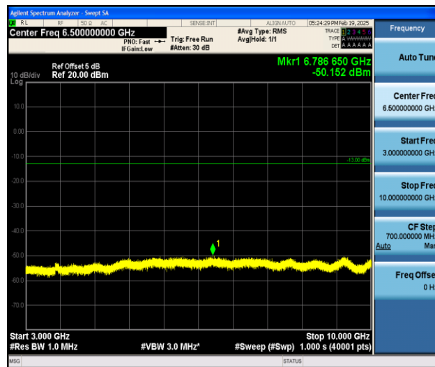
Band5_3MHz_QPSK_20635_1RB#0_3000~10000_3000~10000
