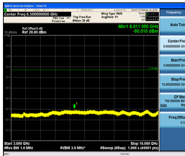
Band5_1.4MHz_QPSK_20407_1RB#0_3000~10000_3000~10000
