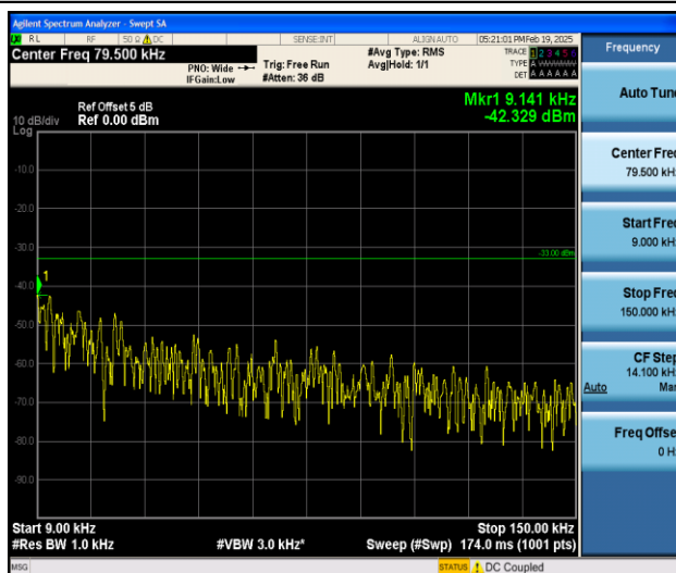
Band5_3MHz_16QAM_20415_1RB#0_0.009~0.15_0.009~0.15
