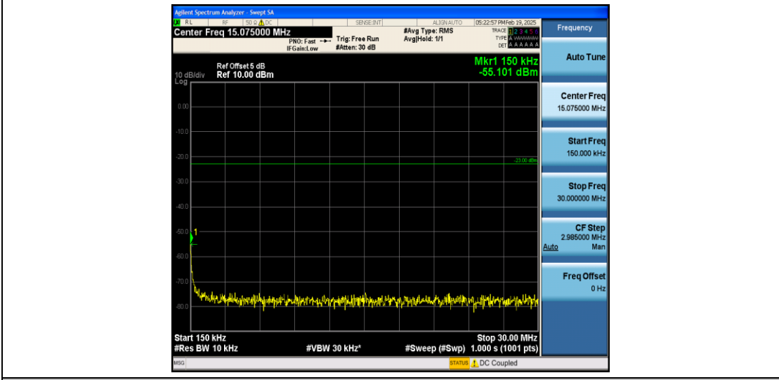
Band5_3MHz_16QAM_20525_1RB#0_0.15~30_0.15~30
