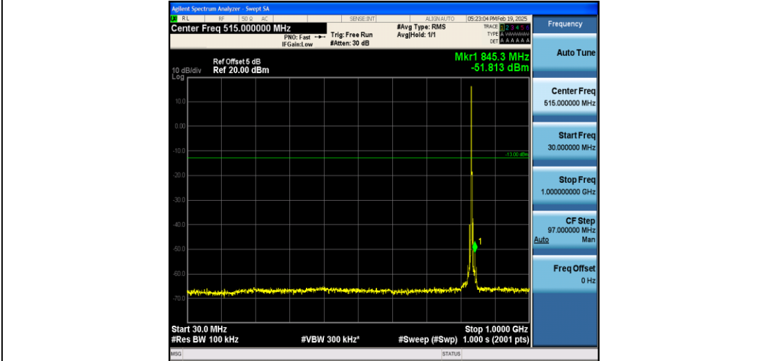
Band5_3MHz_16QAM_20525_1RB#0_30~1000_30~1000
