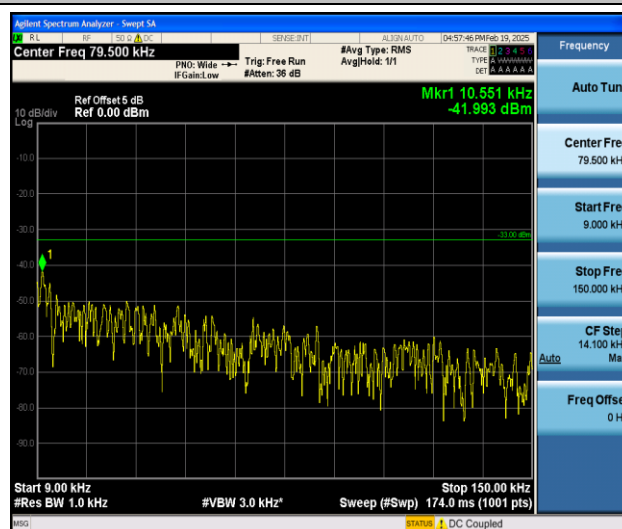
Band5_1.4MHz_16QAM_20407_1RB#0_0.009~0.15_0.009~0.15
