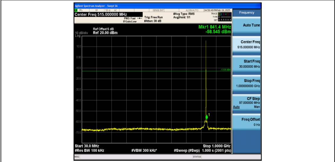
Band5_1.4MHz_16QAM_20525_1RB#0_30~1000_30~1000
