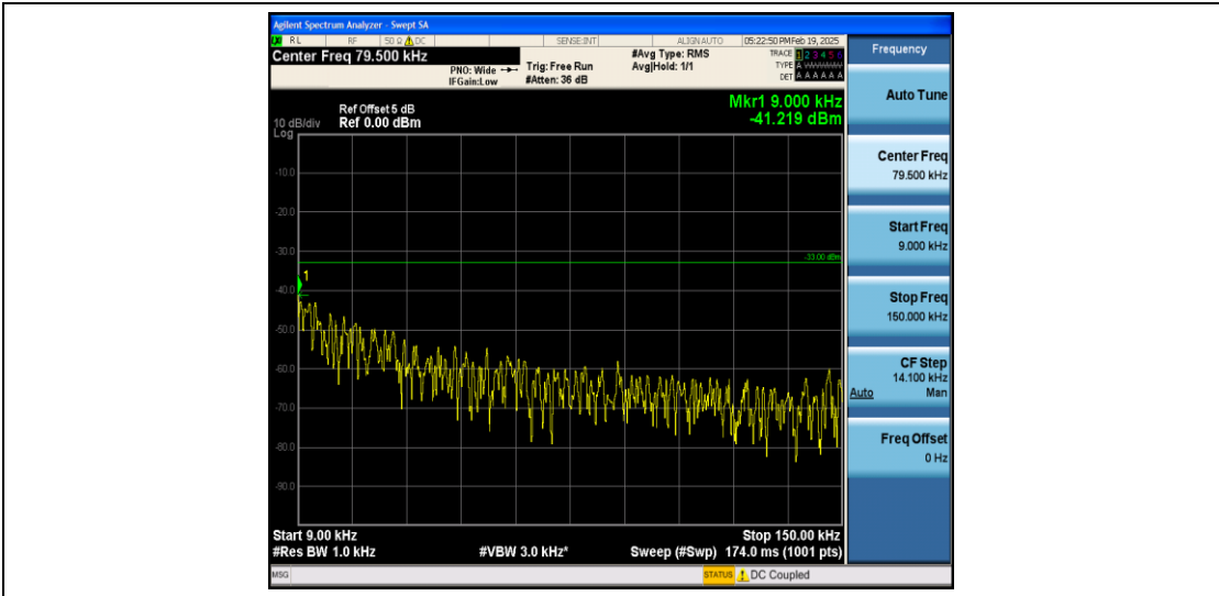
Band5_3MHz_16QAM_20525_1RB#0_0.009~0.15_0.009~0.15
