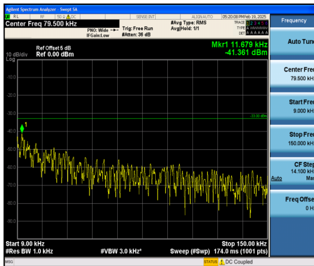
Band5_3MHz_QPSK_20415_1RB#0_0.009~0.15_0.009~0.15
