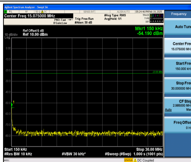
Band5_3MHz_16QAM_20635_1RB#0_0.15~30_0.15~30
