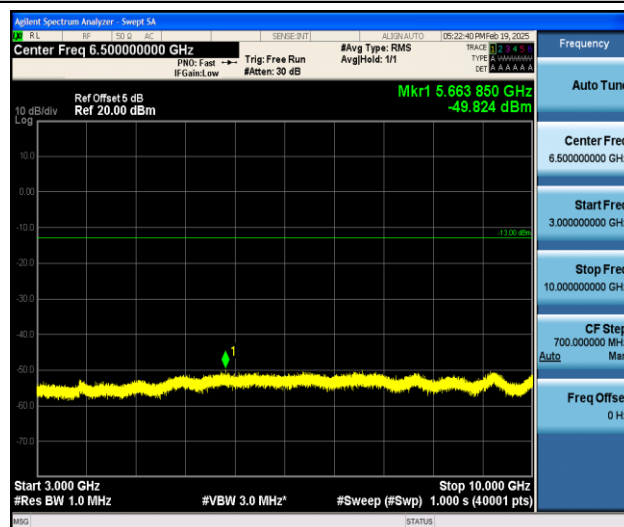
Band5_3MHz_QPSK_20525_1RB#0_3000~10000_3000~10000
