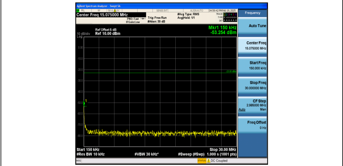
Band5_1.4MHz_16QAM_20525_1RB#0_0.15~30_0.15~30
