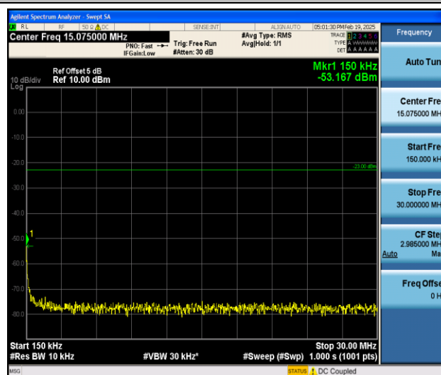
Band5_1.4MHz_16QAM_20643_1RB#0_0.15~30_0.15~30
