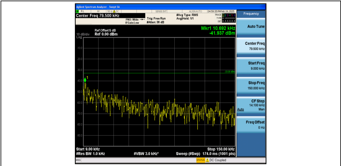
Band5_1.4MHz_16QAM_20525_1RB#0_0.009~0.15_0.009~0.15
