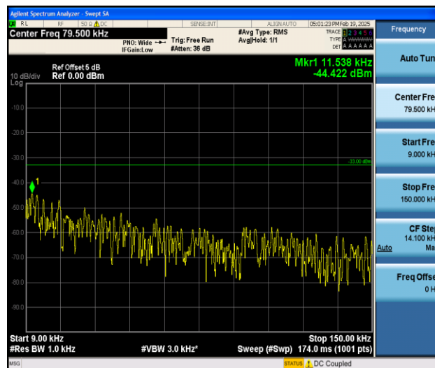
Band5_1.4MHz_16QAM_20643_1RB#0_0.009~0.15_0.009~0.15
