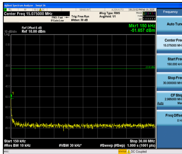
Band5_3MHz_QPSK_20635_1RB#0_0.15~30_0.15~30
