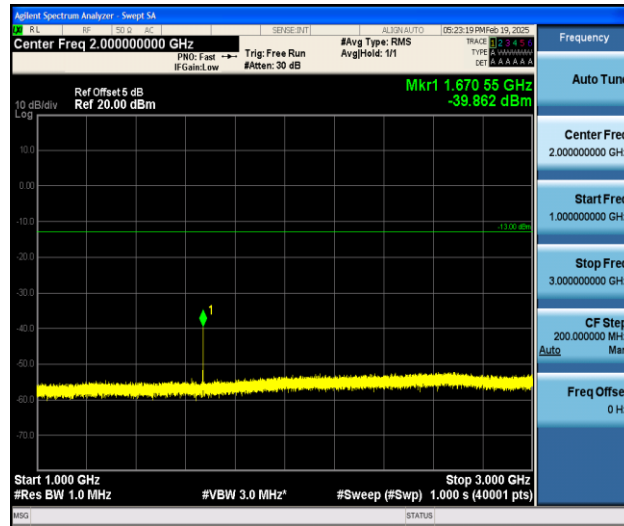
Band5_3MHz_16QAM_20525_1RB#0_1000~3000_1000~3000
