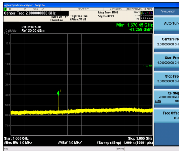
Band5_3MHz_QPSK_20525_1RB#0_1000~3000_1000~3000
