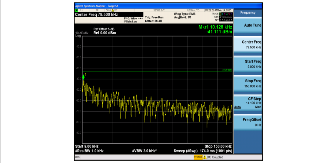
Band5_3MHz_QPSK_20525_1RB#0_0.009~0.15_0.009~0.15
