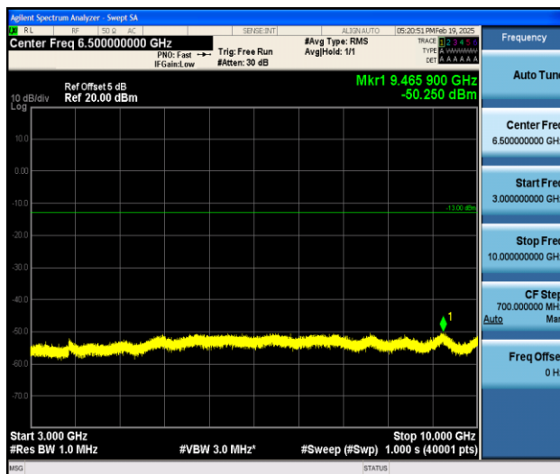
Band5_3MHz_QPSK_20415_1RB#0_3000~10000_3000~10000
