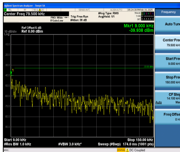
Band5_3MHz_16QAM_20635_1RB#0_0.009~0.15_0.009~0.15
