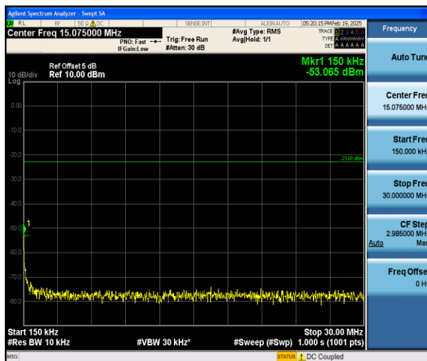
Band5_3MHz_QPSK_20415_1RB#0_0.15~30_0.15~30
