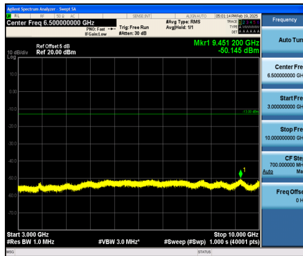
Band5_1.4MHz_QPSK_20643_1RB#0_3000~10000_3000~10000
