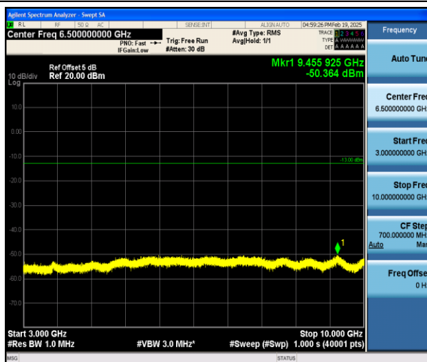
Band5_1.4MHz_QPSK_20525_1RB#0_3000~10000_3000~10000
