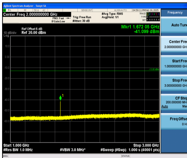
Band5_1.4MHz_QPSK_20525_1RB#0_1000~3000_1000~3000
