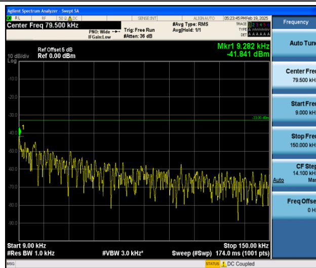
Band5_3MHz_QPSK_20635_1RB#0_0.009~0.15_0.009~0.15
