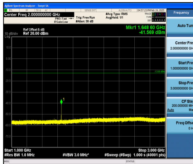
Band5_1.4MHz_QPSK_20407_1RB#0_1000~3000_1000~3000
