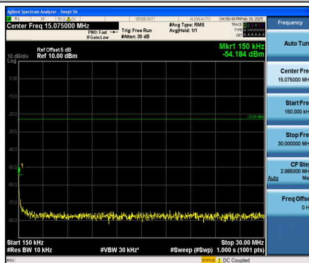
Band5_1.4MHz_QPSK_20525_1RB#0_0.15~30_0.15~30
