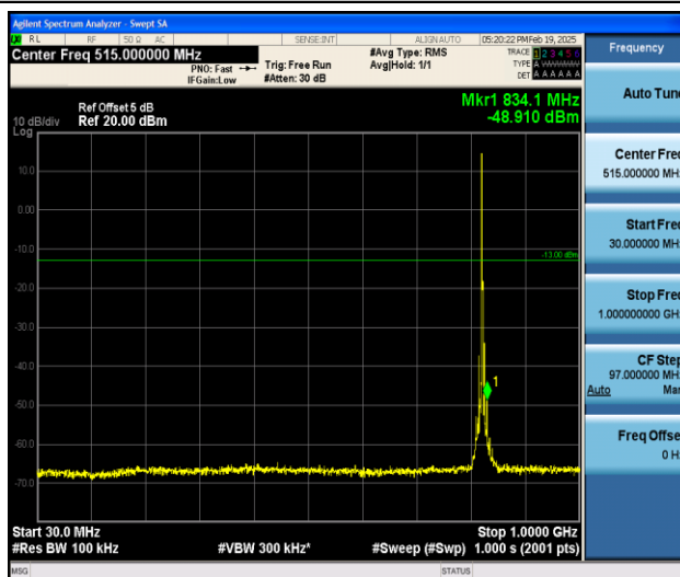
Band5_3MHz_QPSK_20415_1RB#0_30~1000_30~1000
