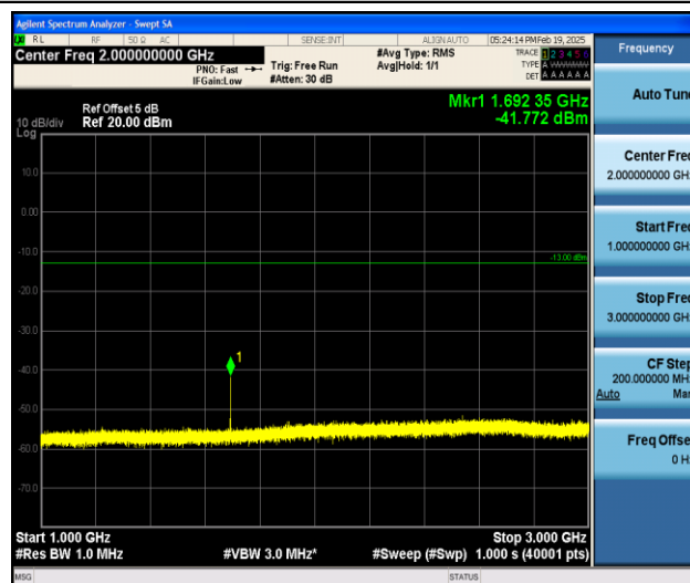
Band5_3MHz_QPSK_20635_1RB#0_1000~3000_1000~3000
