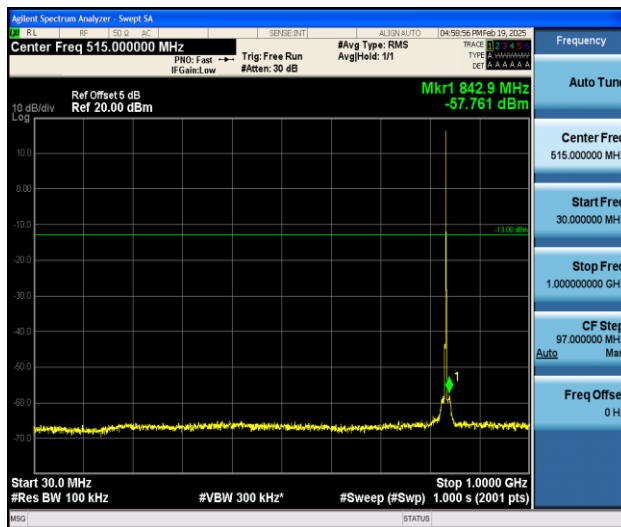
Band5_1.4MHz_QPSK_20525_1RB#0_30~1000_30~1000
