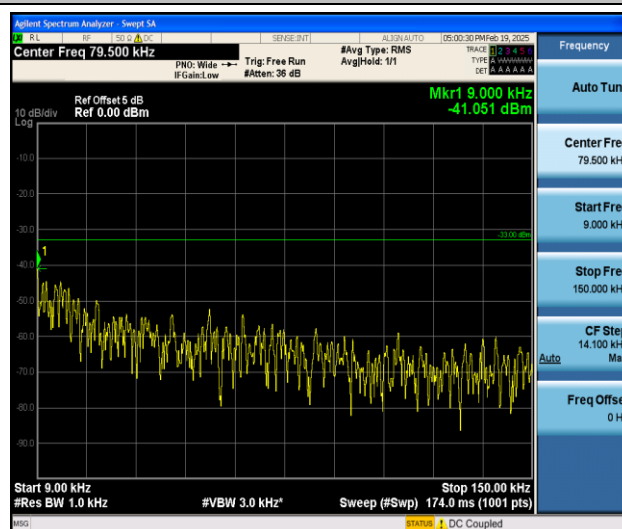
Band5_1.4MHz_QPSK_20643_1RB#0_0.009~0.15_0.009~0.15
