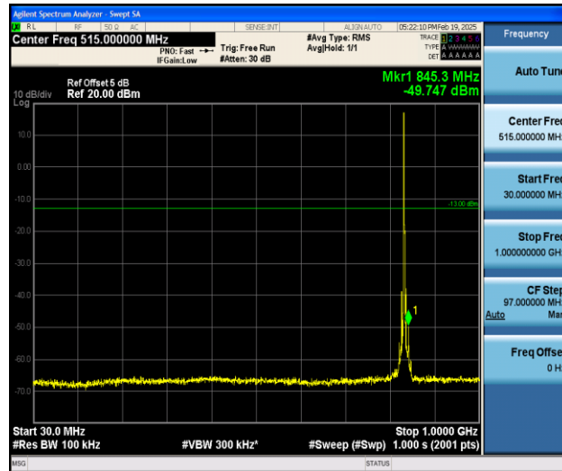
Band5_3MHz_QPSK_20525_1RB#0_30~1000_30~1000
