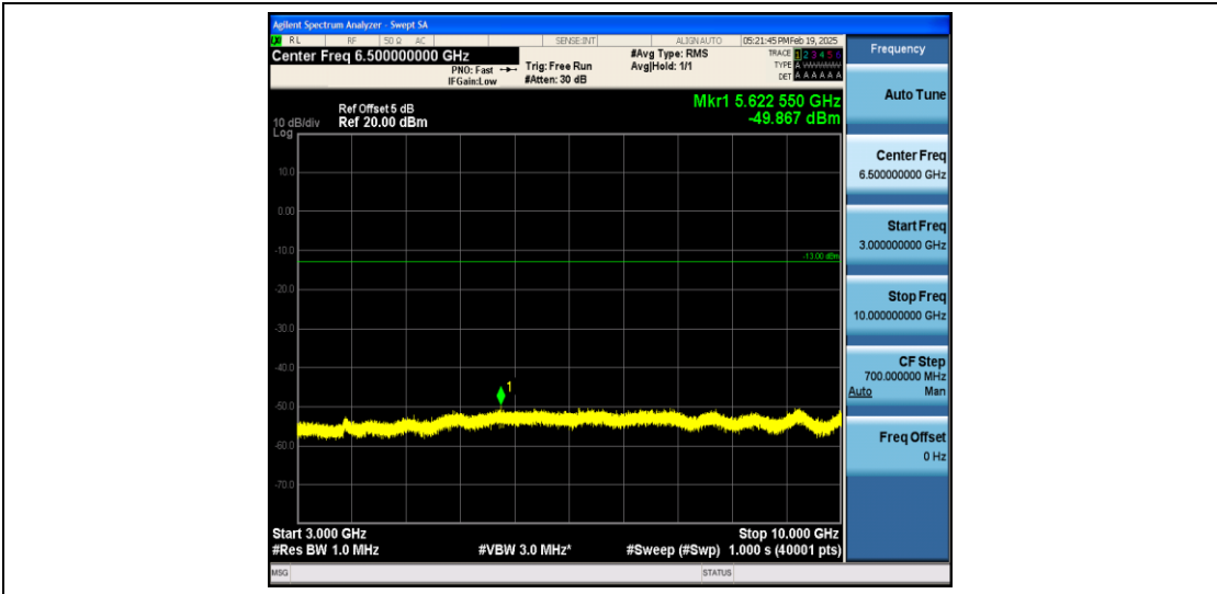
Band5_3MHz_16QAM_20415_1RB#0_3000~10000_3000~10000
