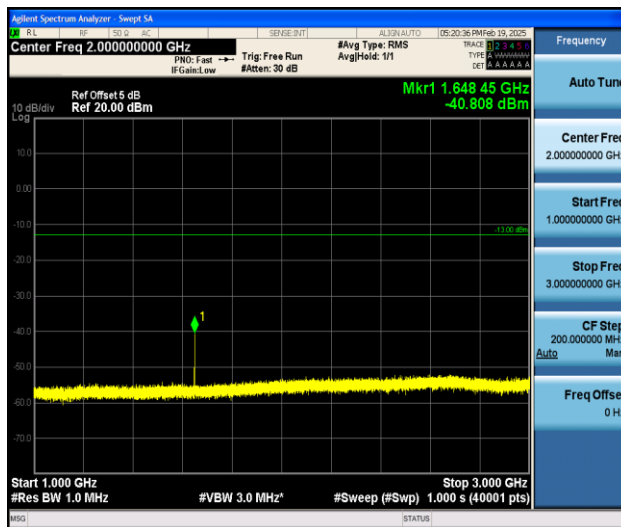
Band5_3MHz_QPSK_20415_1RB#0_1000~3000_1000~3000
