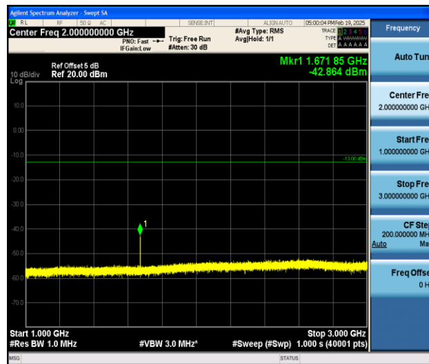
Band5_1.4MHz_16QAM_20525_1RB#0_1000~3000_1000~3000
