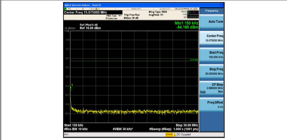
Band5_3MHz_QPSK_20525_1RB#0_0.15~30_0.15~30
