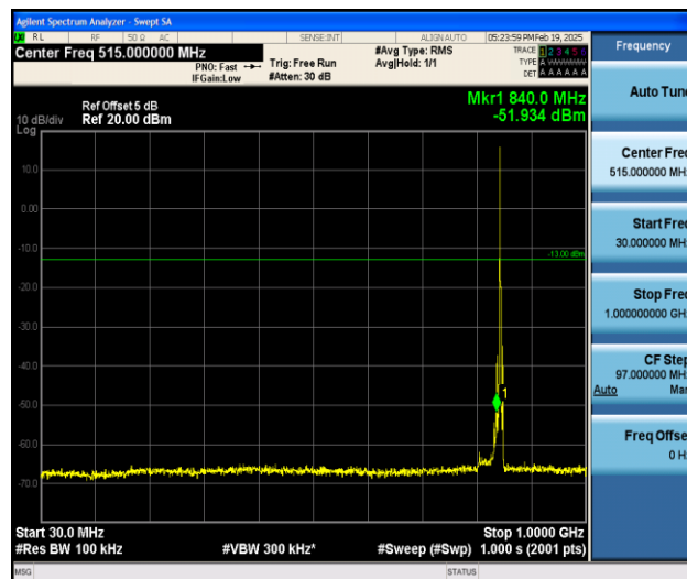
Band5_3MHz_QPSK_20635_1RB#0_30~1000_30~1000
