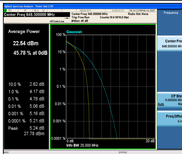
Band5-1.4MHz-QPSK-20643-1RB#0-PASS
