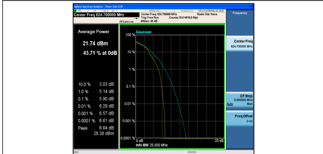
Band5-1.4MHz-16QAM-20407-1RB#0-PASS
