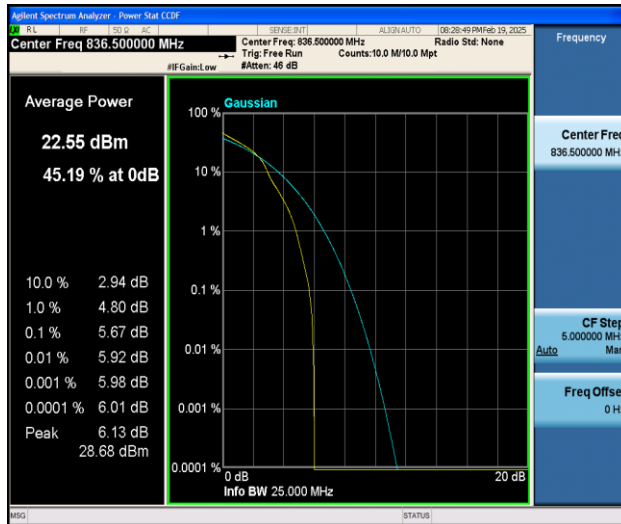
Band5-10MHz-16QAM-20525-1RB#0-PASS
