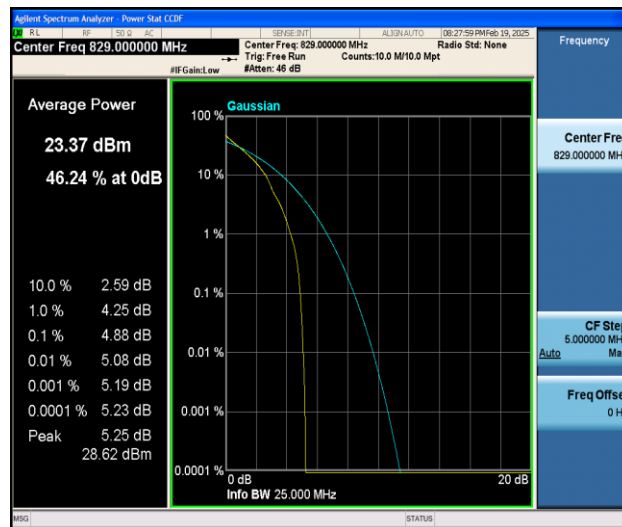
Band5-10MHz-QPSK-20450-1RB#0-PASS
