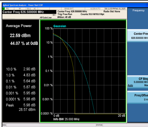
Band5-5MHz-16QAM-20425-1RB#0-PASS
