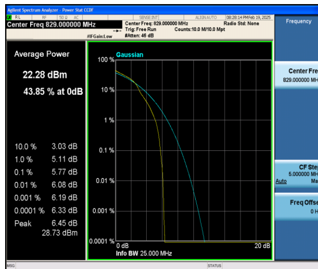
Band5-10MHz-16QAM-20450-1RB#0-PASS
