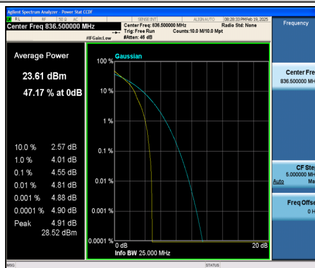
Band5-10MHz-QPSK-20525-1RB#0-PASS
