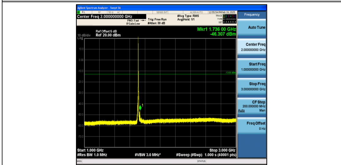
Band4_5MHz_QPSK_19975_1RB#0_1000~3000_1000~3000
