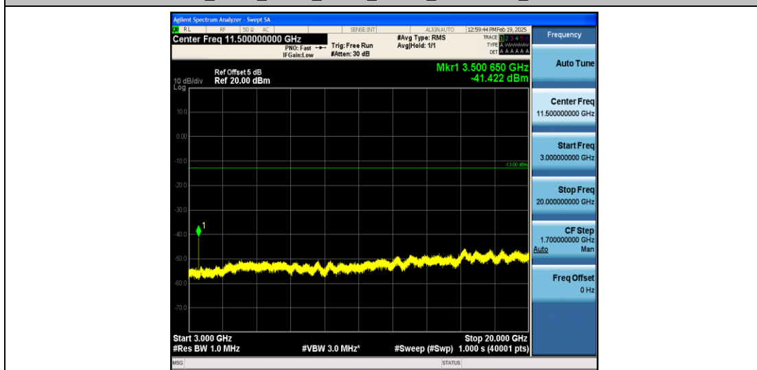
Band4_5MHz_QPSK_20375_1RB#0_3000~20000_3000~20000
