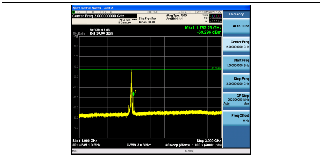
Band4_10MHz_QPSK_20175_1RB#0_1000~3000_1000~3000
