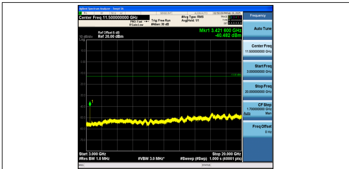
Band4_10MHz_QPSK_20000_1RB#0_3000~20000_3000~20000
