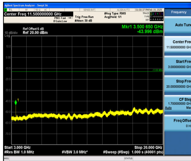
Band4_5MHz_16QAM_20375_1RB#0_3000~20000_3000~20000
