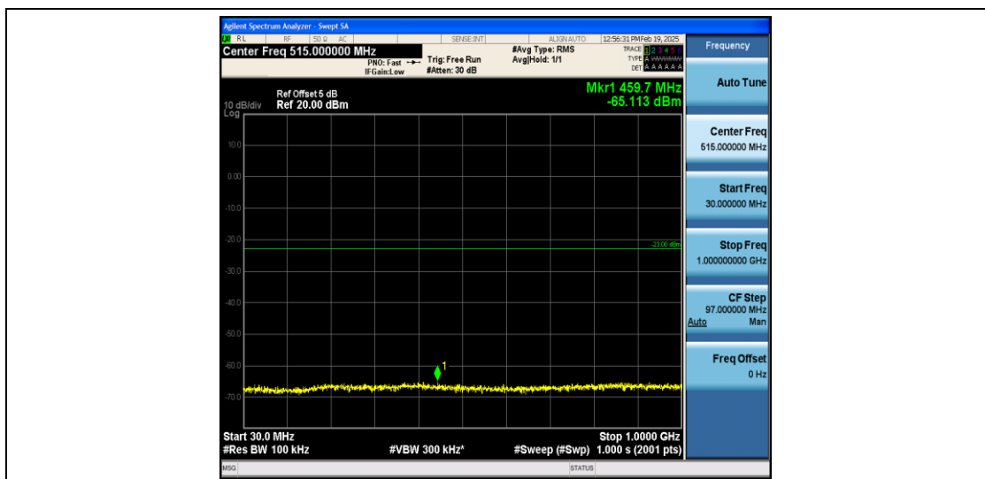
Band4_5MHz_16QAM_19975_1RB#0_30~1000_30~1000
