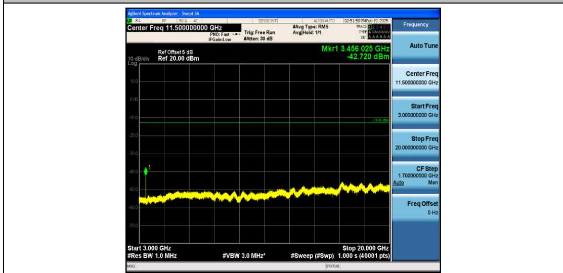
Band4_10MHz_QPSK_20175_1RB#0_3000~20000_3000~20000
