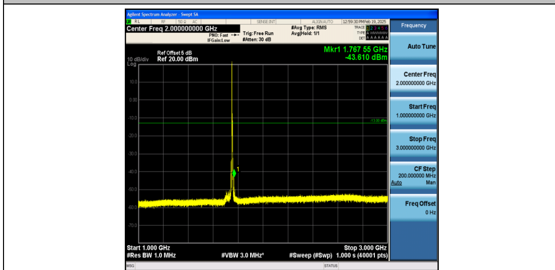
Band4_5MHz_QPSK_20375_1RB#0_1000~3000_1000~3000
