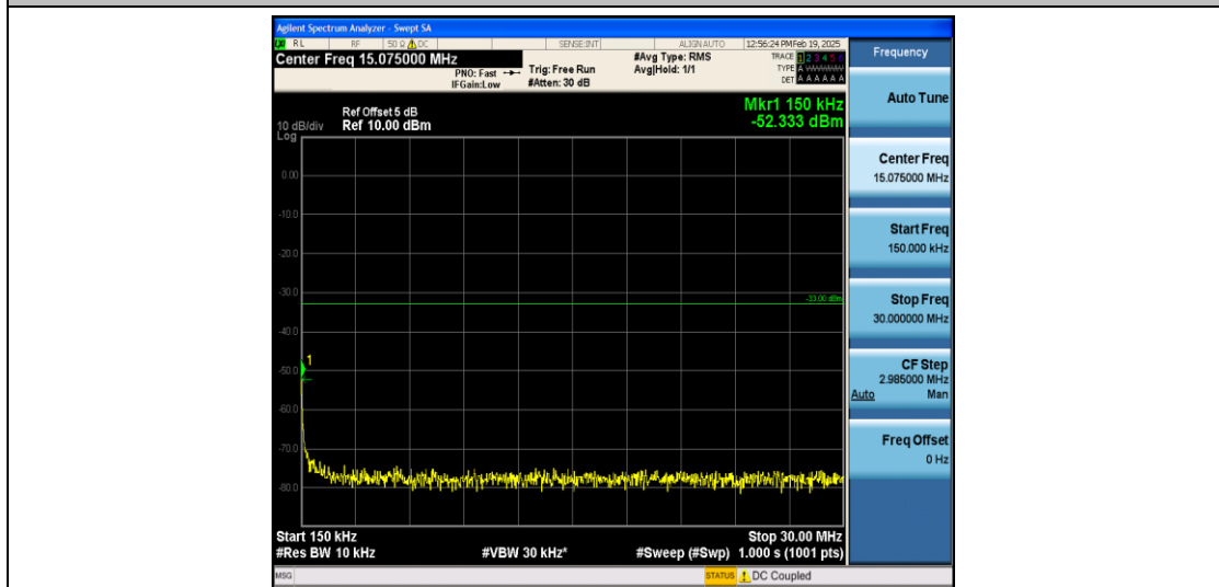
Band4_5MHz_16QAM_19975_1RB#0_0.15~30_0.15~30
