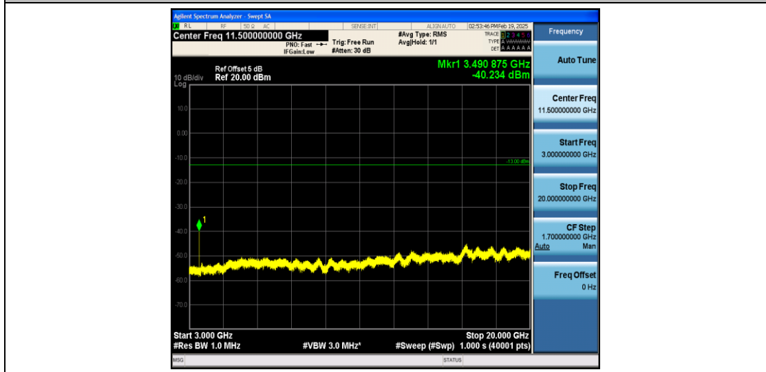
Band4_10MHz_QPSK_20350_1RB#0_3000~20000_3000~20000
