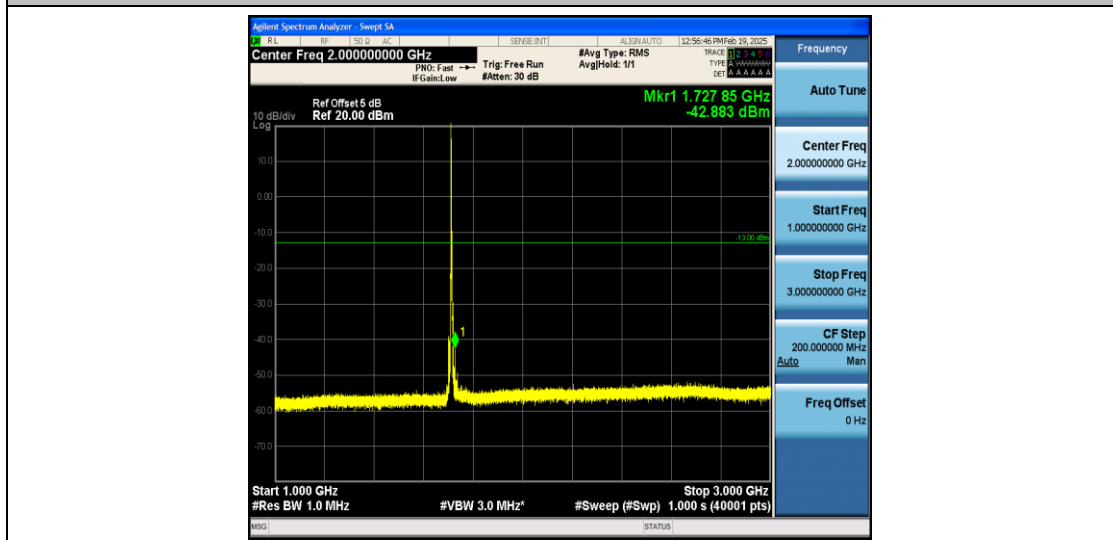
Band4_5MHz_16QAM_19975_1RB#0_1000~3000_1000~3000
