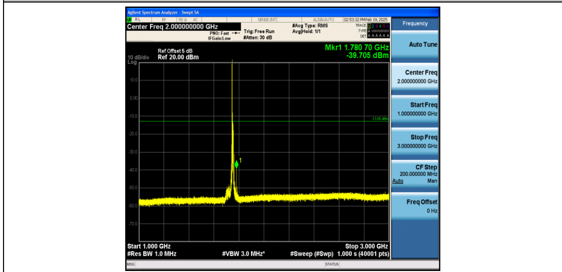
Band4_10MHz_QPSK_20350_1RB#0_1000~3000_1000~3000
