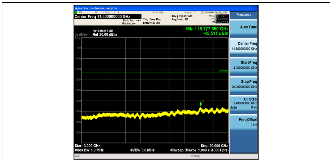
Band4_5MHz_QPSK_19975_1RB#0_3000~20000_3000~20000
