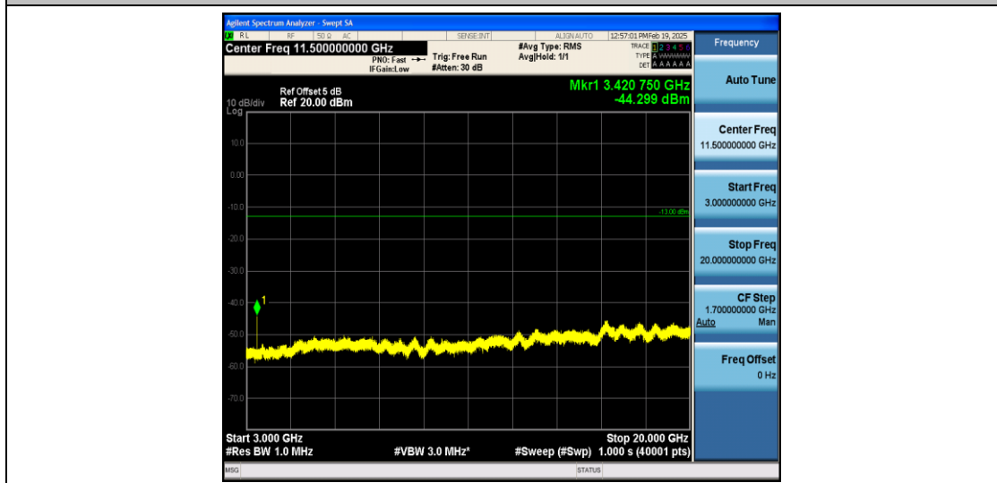
Band4_5MHz_16QAM_19975_1RB#0_3000~20000_3000~20000
