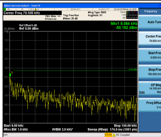
Band4_10MHz_QPSK_20000_1RB#0_0.009~0.15_0.009~0.15
