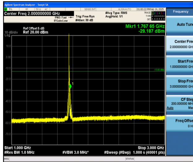
Band4_5MHz_16QAM_20375_1RB#0_1000~3000_1000~3000
