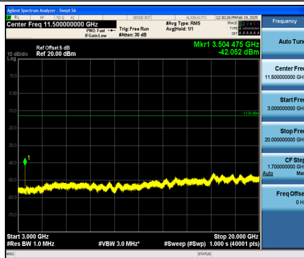
Band4_3MHz_QPSK_20385_1RB#0_3000~20000_3000~20000
