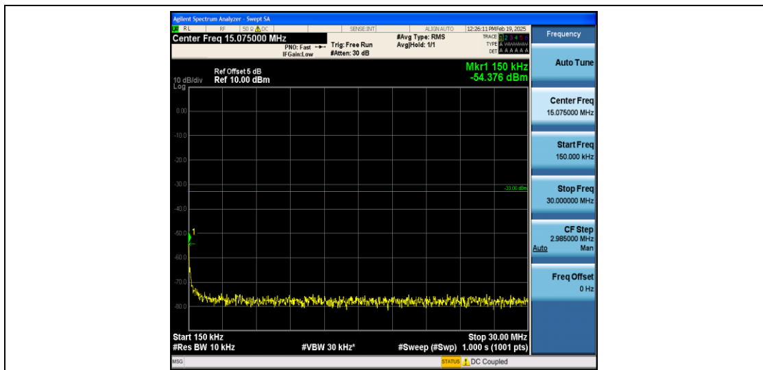
Band4_3MHz_QPSK_19965_1RB#0_0.15~30_0.15~30
