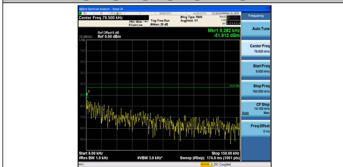
Band4_3MHz_QPSK_19965_1RB#0_0.009~0.15_0.009~0.15
