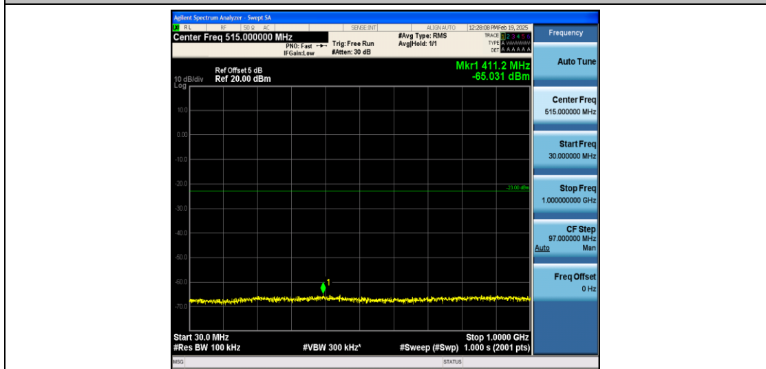
Band4_3MHz_QPSK_20175_1RB#0_30~1000_30~1000
