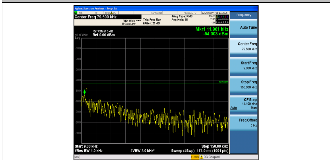
Band4_3MHz_16QAM_19965_1RB#0_0.009~0.15_0.009~0.15
