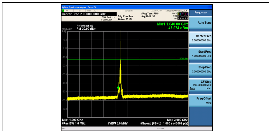
Band2_15MHz_QPSK_18900_1RB#0_1000~3000_1000~3000
