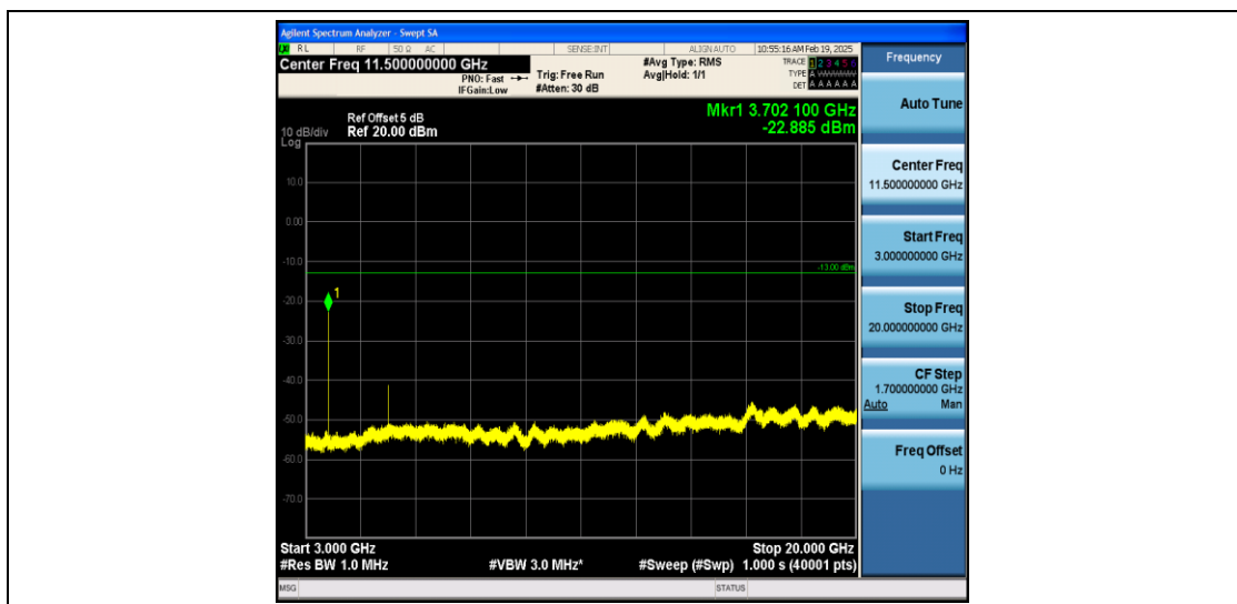
Band2_20MHz_QPSK_18700_1RB#0_3000~20000_3000~20000
