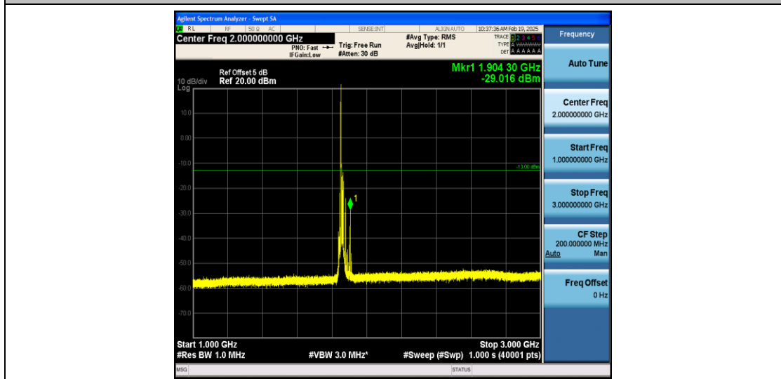
Band2_15MHz_16QAM_18675_1RB#0_1000~3000_1000~3000
