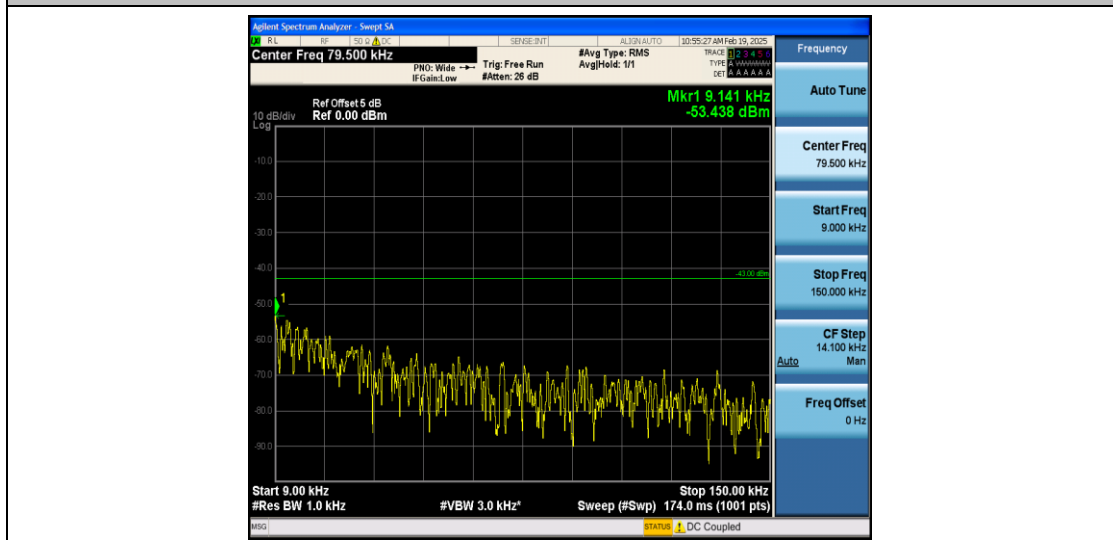
Band2_20MHz_16QAM_18700_1RB#0_0.009~0.15_0.009~0.15
