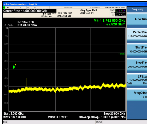
Band2_20MHz_QPSK_18900_1RB#0_3000~20000_3000~20000
