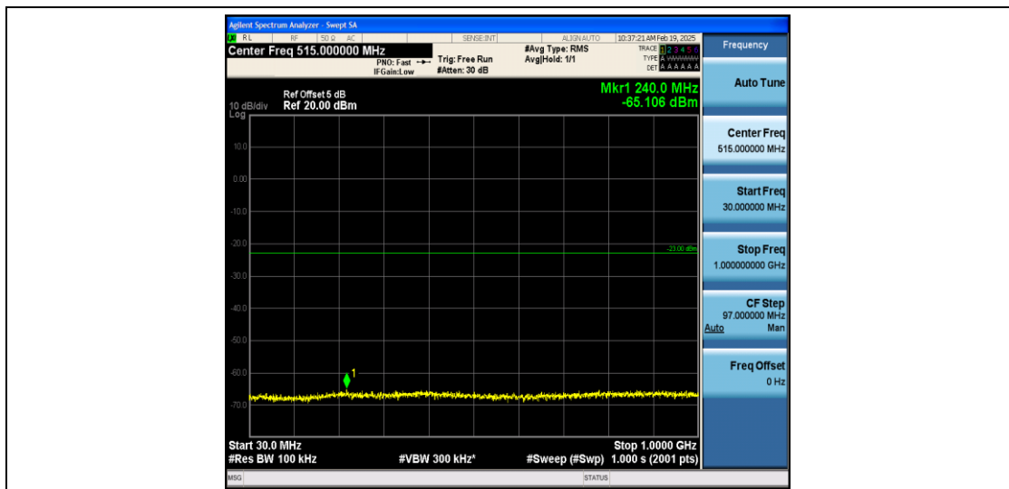
Band2_15MHz_16QAM_18675_1RB#0_30~1000_30~1000
