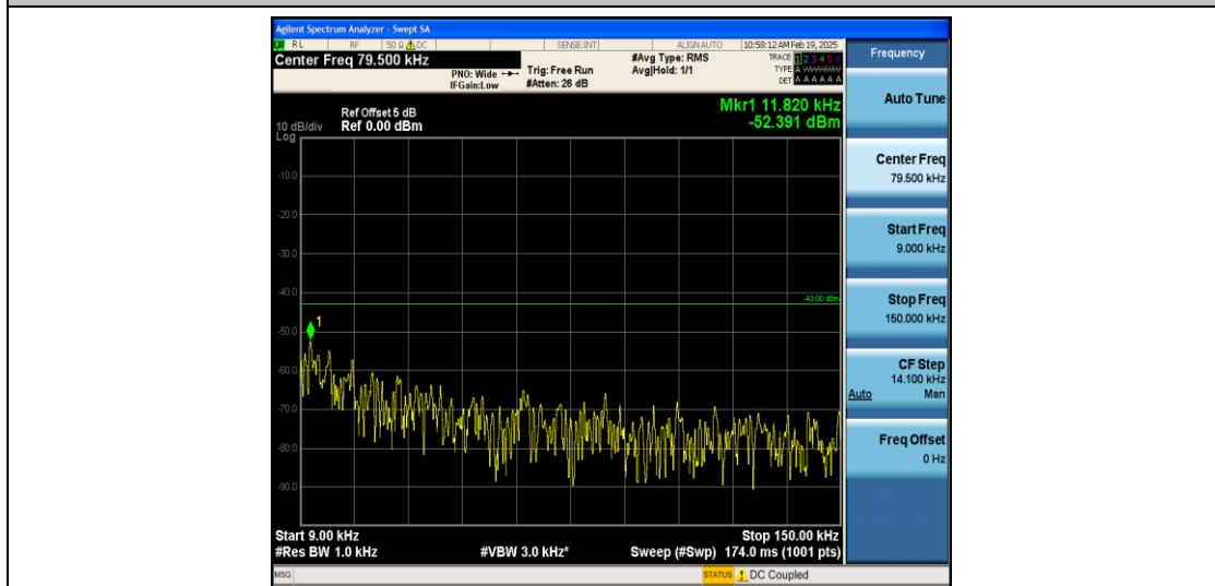
Band2_20MHz_QPSK_19100_1RB#0_0.009~0.15_0.009~0.15
