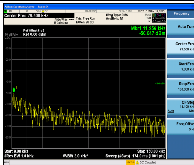
Band2_20MHz_16QAM_18900_1RB#0_0.009~0.15_0.009~0.15
