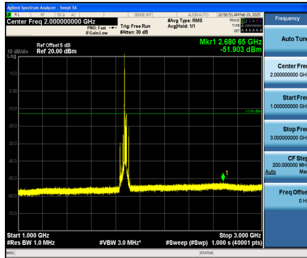
Band2_20MHz_QPSK_18900_1RB#0_1000~3000_1000~3000
