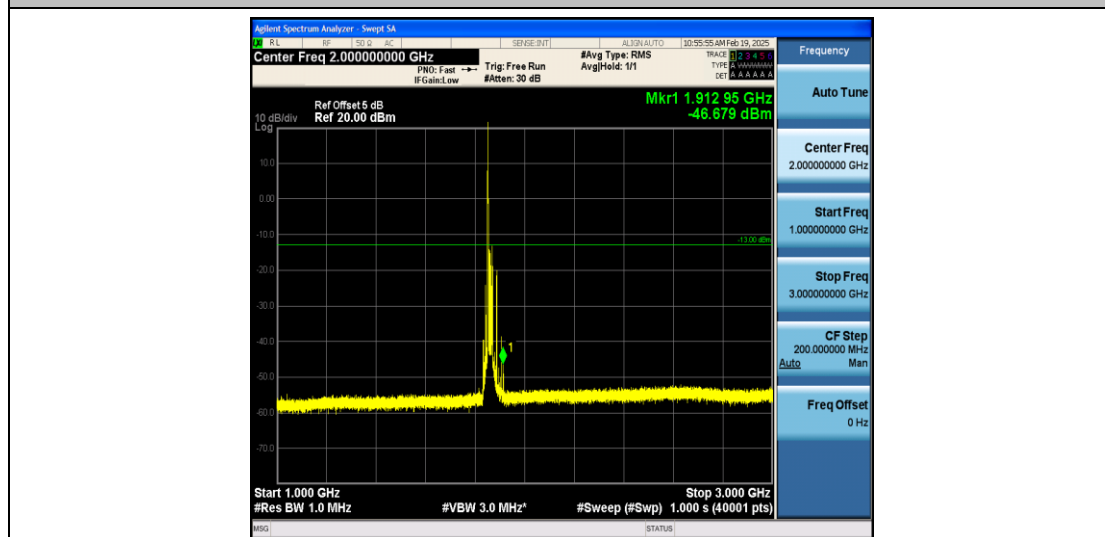
Band2_20MHz_16QAM_18700_1RB#0_1000~3000_1000~3000
