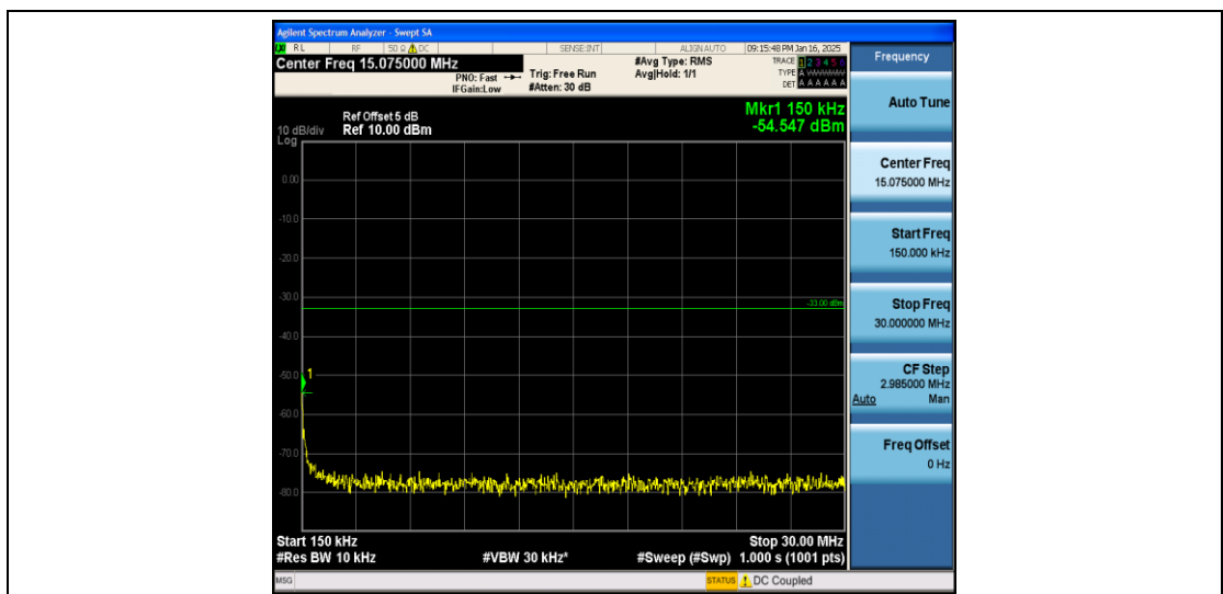
Band2_5MHz_QPSK_18625_1RB#0_0.15~30_0.15~30
