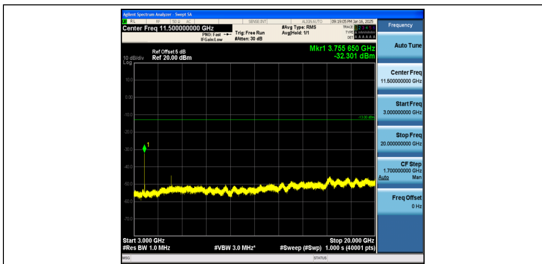
Band2_5MHz_16QAM_18900_1RB#0_3000~20000_3000~20000
