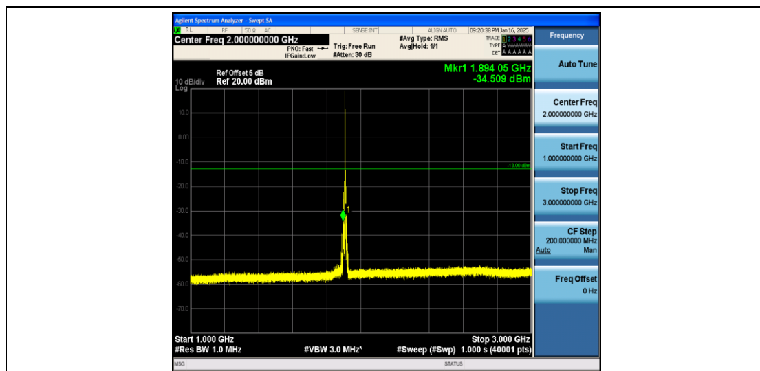
Band2_5MHz_16QAM_19175_1RB#0_1000~3000_1000~3000
