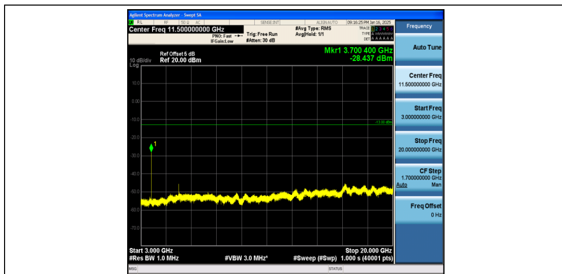
Band2_5MHz_QPSK_18625_1RB#0_3000~20000_3000~20000
