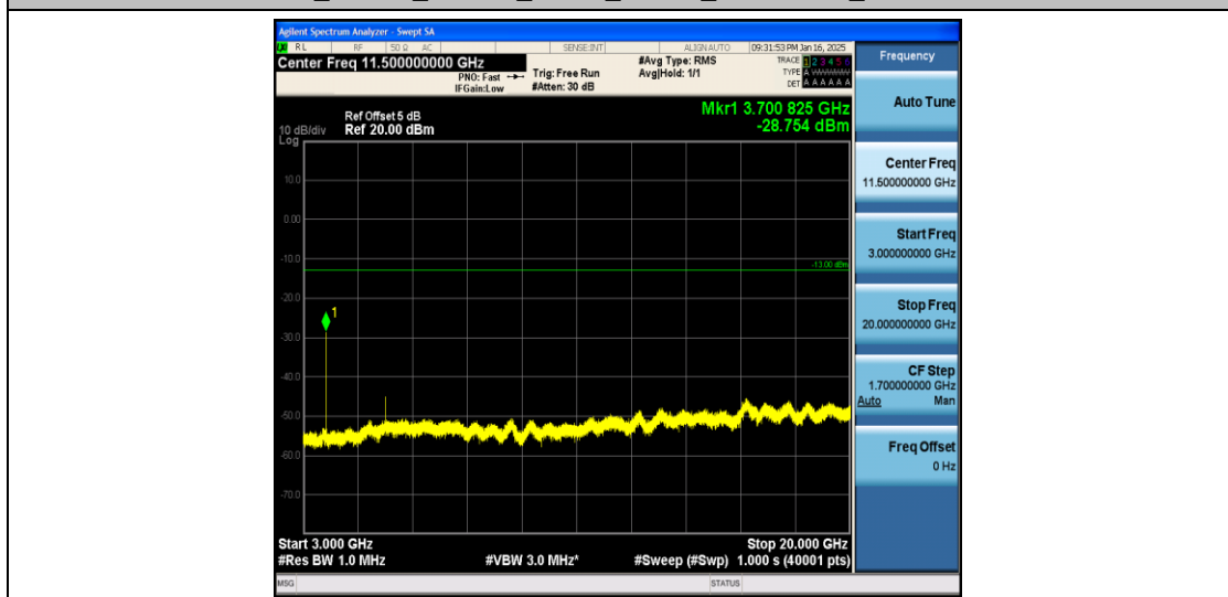
Band2_10MHz_16QAM_18650_1RB#0_3000~20000_3000~20000
