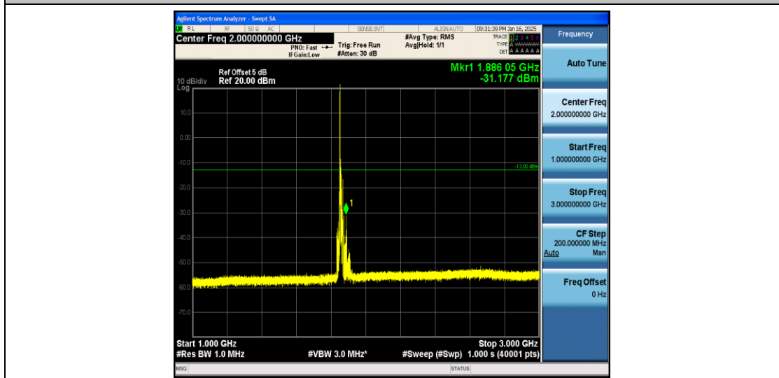
Band2_10MHz_16QAM_18650_1RB#0_1000~3000_1000~3000
