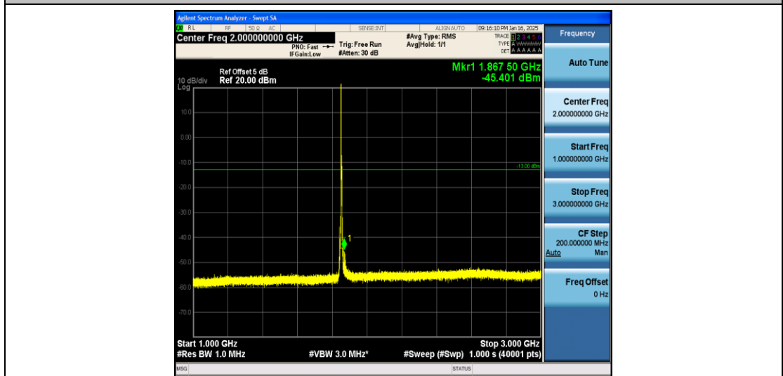
Band2_5MHz_QPSK_18625_1RB#0_1000~3000_1000~3000
