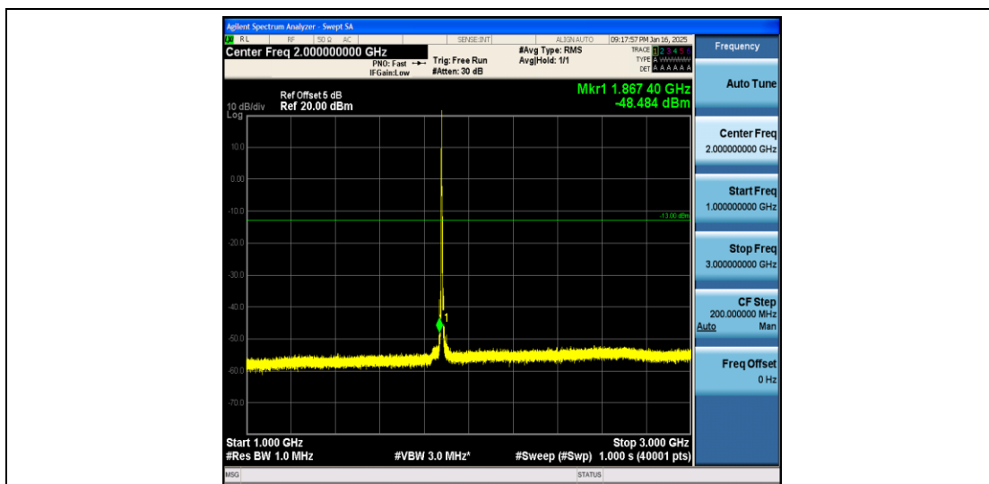
Band2_5MHz_QPSK_18900_1RB#0_1000~3000_1000~3000
