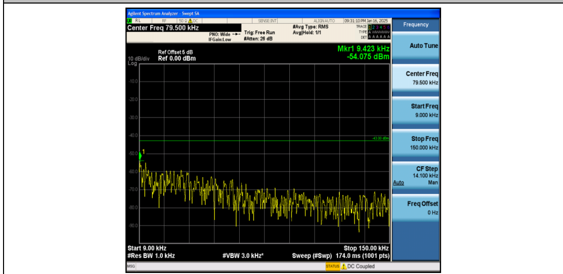
Band2_10MHz_16QAM_18650_1RB#0_0.009~0.15_0.009~0.15
