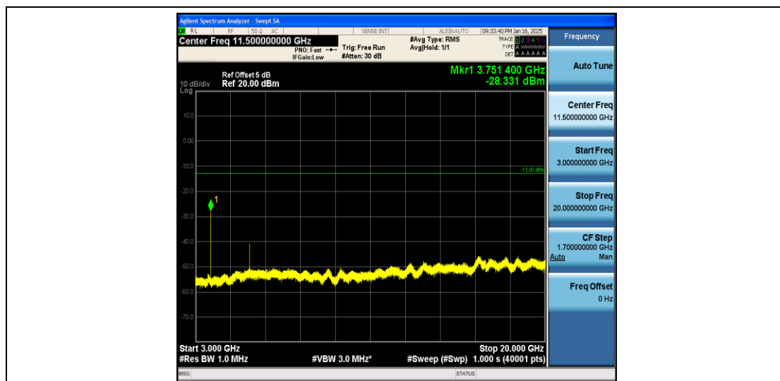
Band2_10MHz_16QAM_18900_1RB#0_3000~20000_3000~20000
