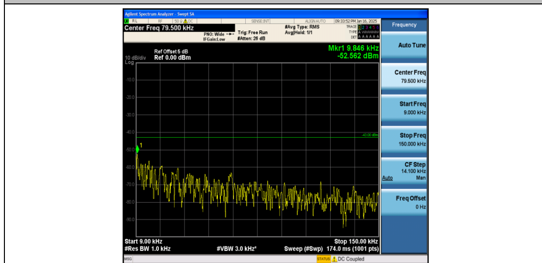
Band2_10MHz_QPSK_19150_1RB#0_0.009~0.15_0.009~0.15
