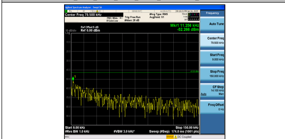
Band2_5MHz_16QAM_18900_1RB#0_0.009~0.15_0.009~0.15
