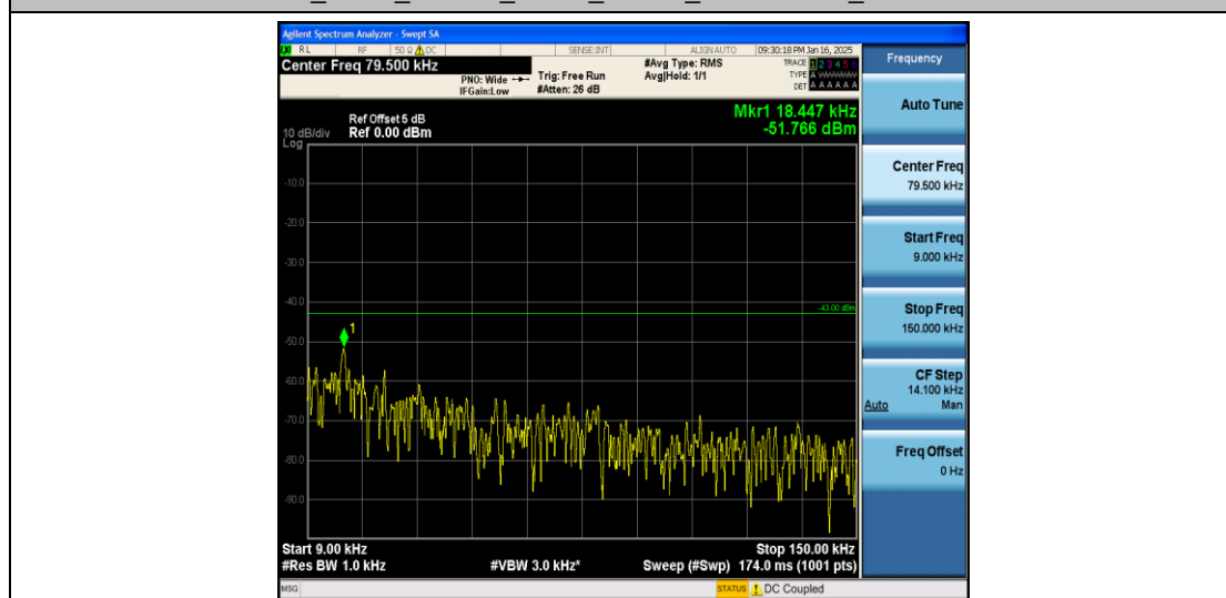
Band2_10MHz_QPSK_18650_1RB#0_0.009~0.15_0.009~0.15
