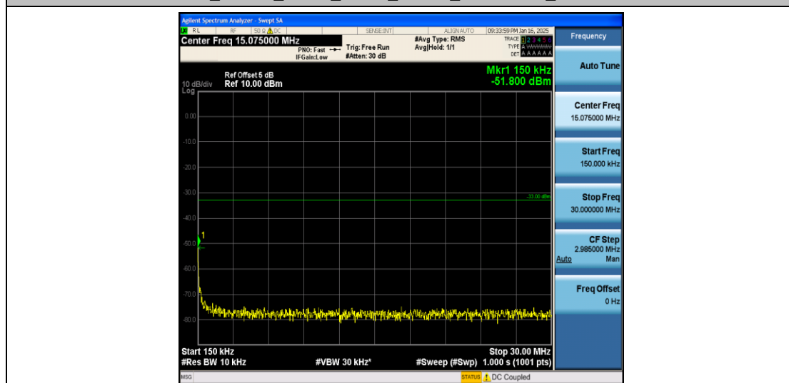
Band2_10MHz_QPSK_19150_1RB#0_0.15~30_0.15~30
