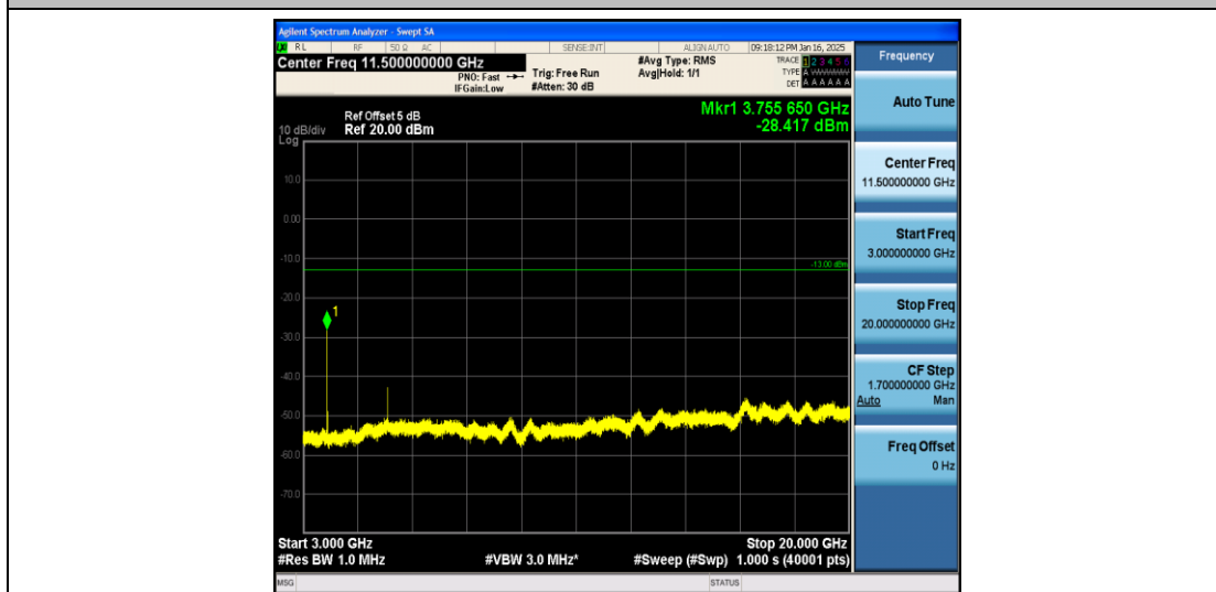
Band2_5MHz_QPSK_18900_1RB#0_3000~20000_3000~20000
