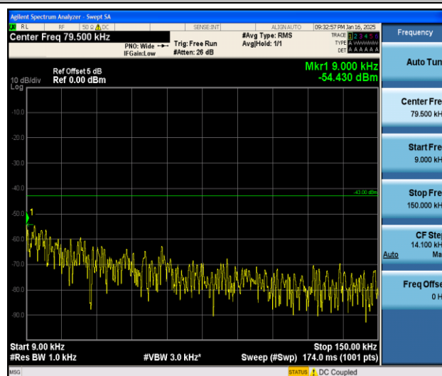
Band2_10MHz_16QAM_18900_1RB#0_0.009~0.15_0.009~0.15
