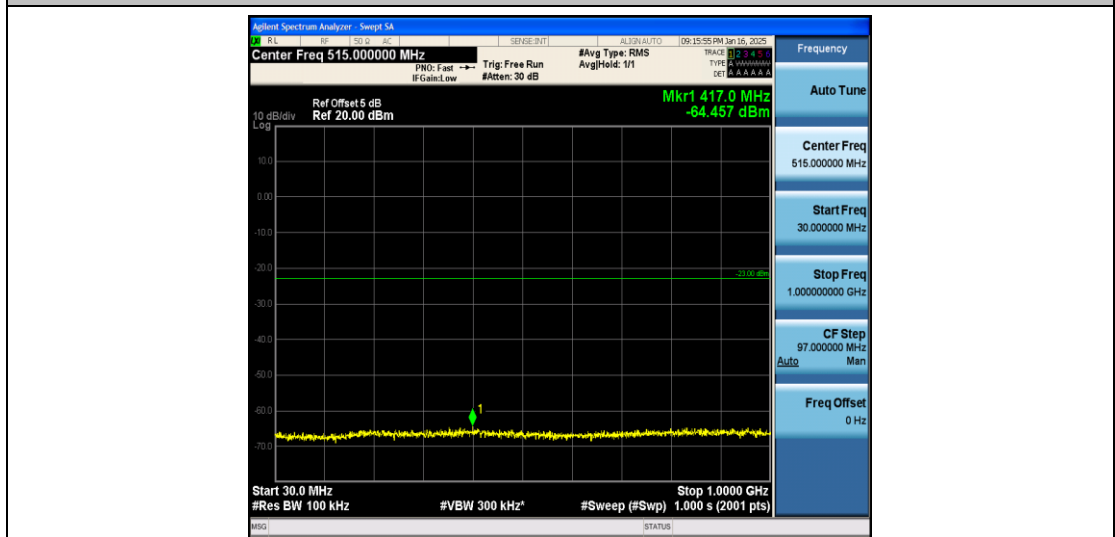
Band2_5MHz_QPSK_18625_1RB#0_30~1000_30~1000
