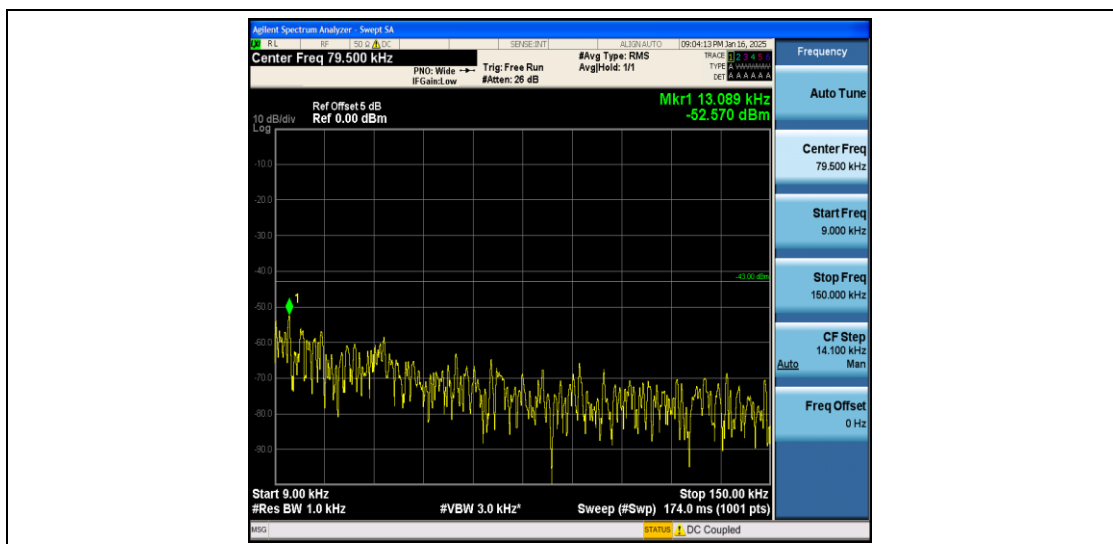
Band2_3MHz_QPSK_18900_1RB#0_0.009~0.15_0.009~0.15
