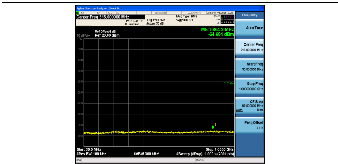
Band2_1.4MHz_QPSK_19193_1RB#0_30~1000_30~1000
