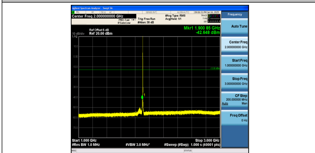
Band2_3MHz_QPSK_19185_1RB#0_1000~3000_1000~3000
