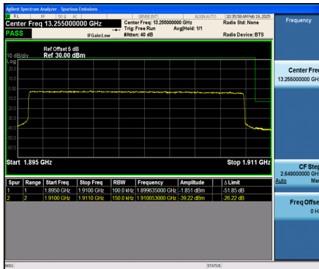
Band2_15MHz_QPSK_19125_75RB#0
