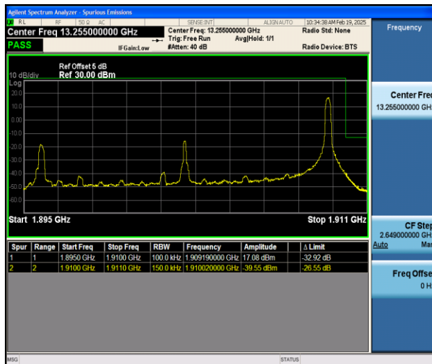
Band2_15MHz_16QAM_19125_1RB#74
