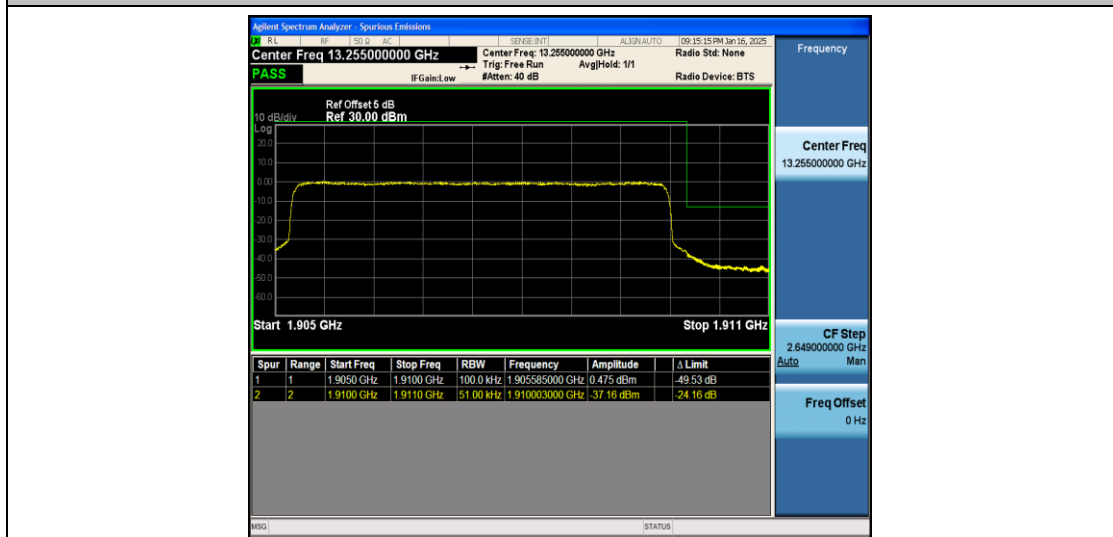
Band2_5MHz_QPSK_19175_25RB#0
