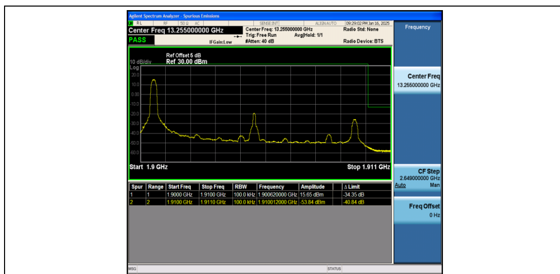
Band2_10MHz_16QAM_19150_1RB#0
