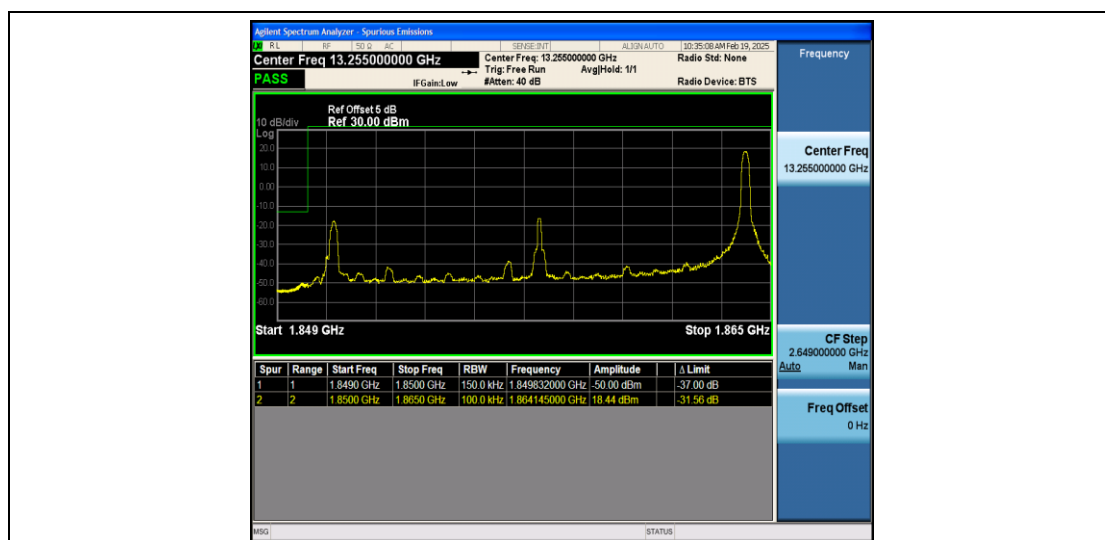
Band2_15MHz_QPSK_18675_1RB#74
