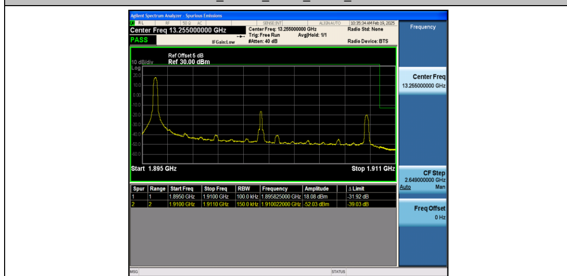
Band2_15MHz_QPSK_19125_1RB#0
