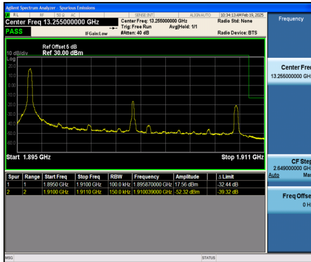
Band2_15MHz_16QAM_19125_1RB#0
