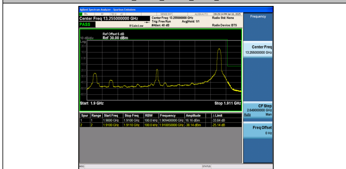
Band2_10MHz_QPSK_19150_1RB#49
