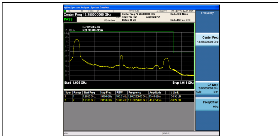
Band2_5MHz_QPSK_19175_1RB#0
