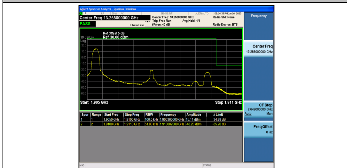
Band2_5MHz_16QAM_19175_1RB#0
