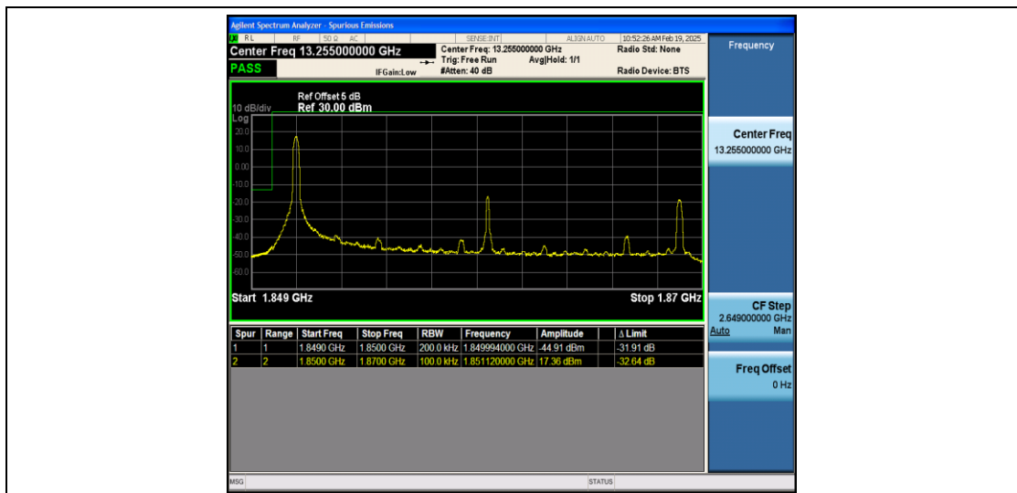
Band2_20MHz_16QAM_18700_1RB#0
