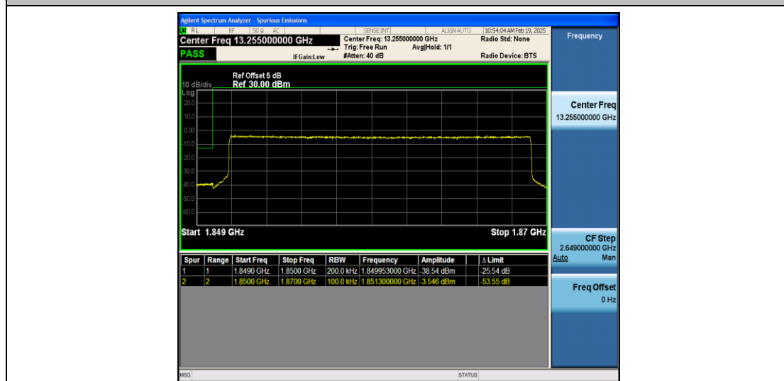
Band2_20MHz_QPSK_18700_100RB#0
