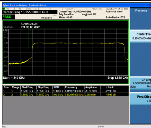
Band2_5MHz_16QAM_18625_25RB#0
