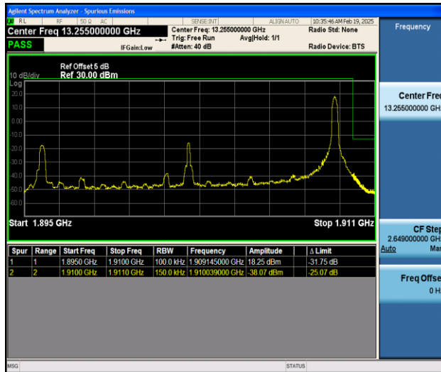
Band2_15MHz_QPSK_19125_1RB#74
