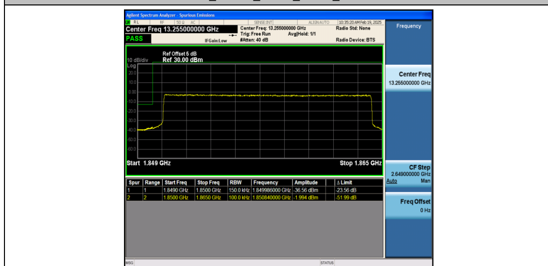
Band2_15MHz_QPSK_18675_75RB#0
