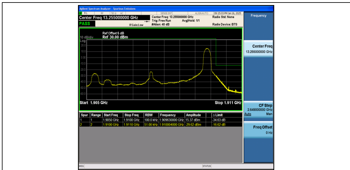
Band2_5MHz_16QAM_19175_1RB#24
